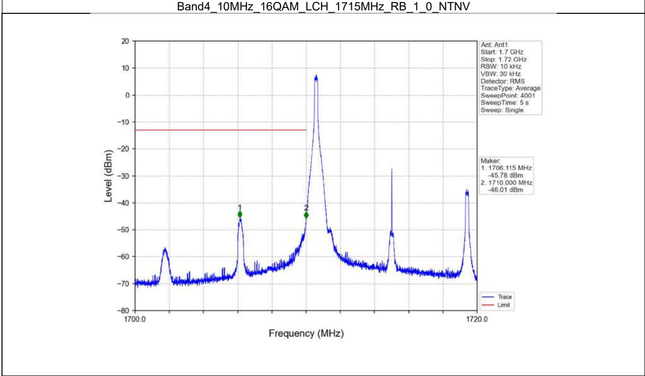
Band4_10MHz_16QAM_LCH_1715MHz_RB_1_0_NTNV
