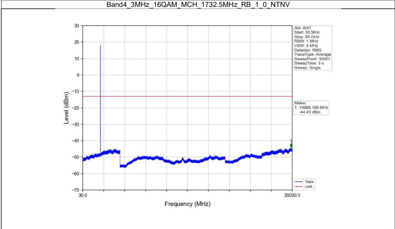
Band4_3MHz_16QAM_MCH_1732.5MHz_RB_1_0_NTNV
