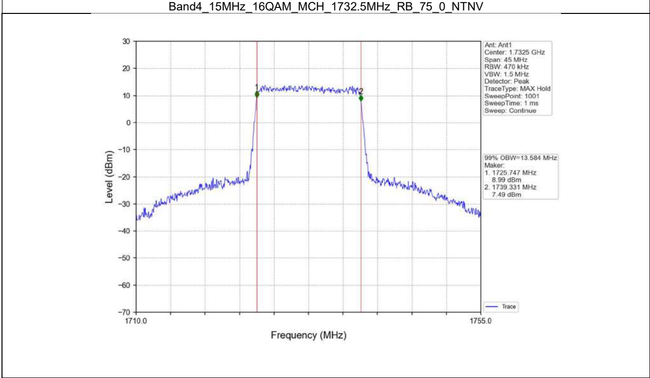
Band4_15MHz_16QAM_MCH_1732.5MHz_RB_75_0_NTNV
