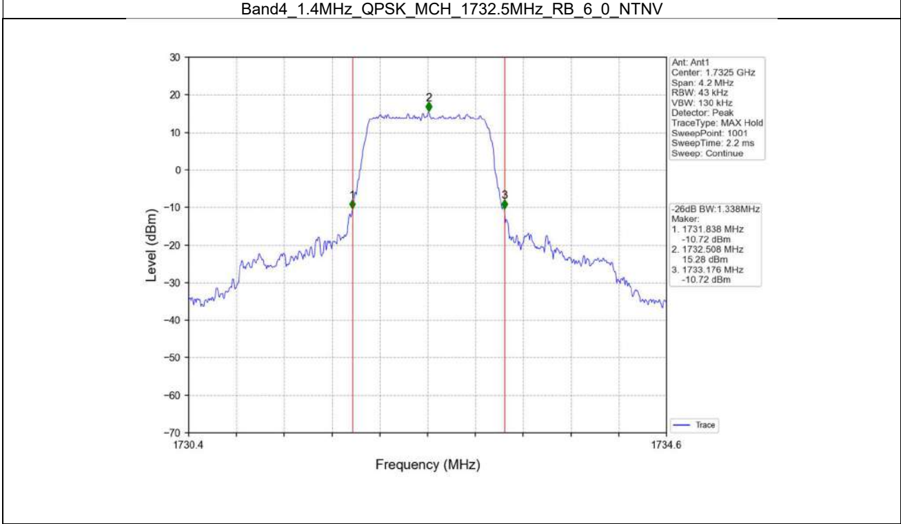
Band4_1.4MHz_QPSK_MCH_1732.5MHz_RB_6_0_NTNV
