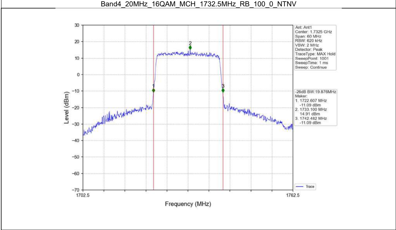
Band4_20MHz_16QAM_MCH_1732.5MHz_RB_100_0_NTNV
