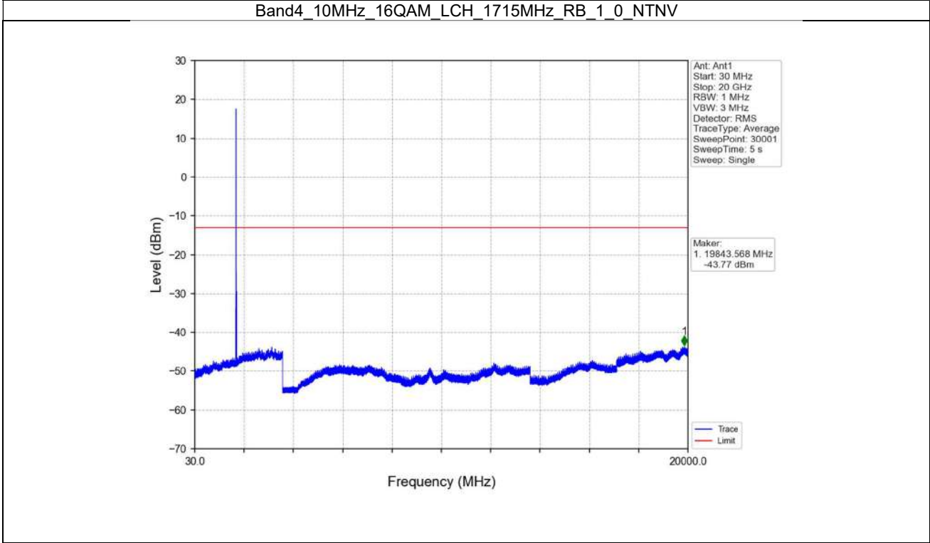
Band4_10MHz_16QAM_LCH_1715MHz_RB_1_0_NTNV
