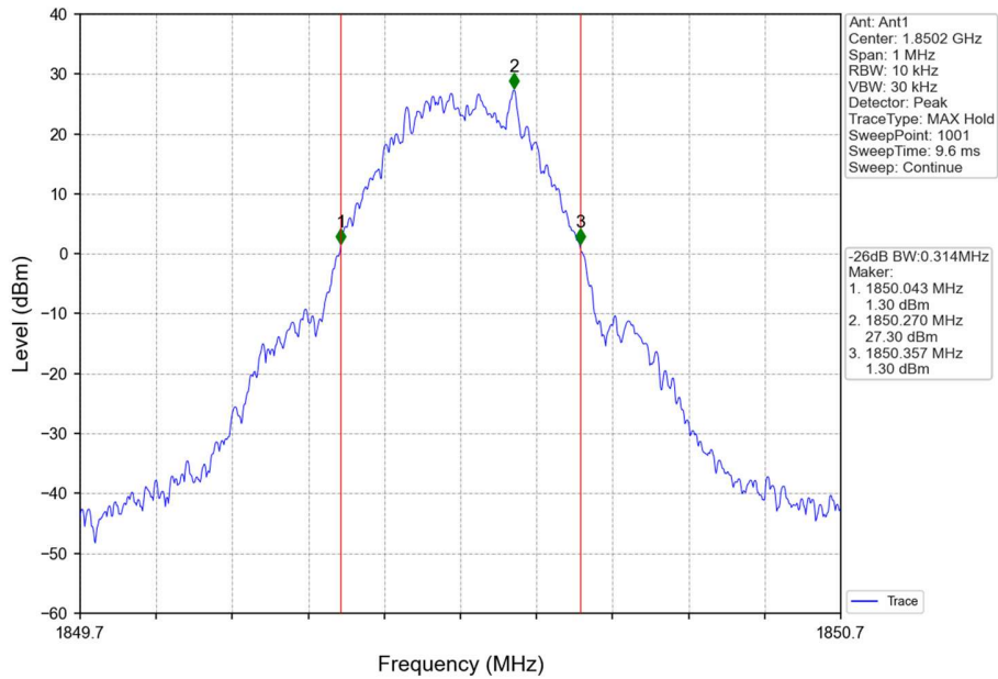
PCS1900_GSM_LCH_1850.2MHz_GSM_NTNV
