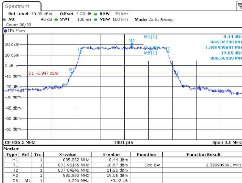
Band26-1.4MHz-QPSK-26915-6RB#0-1.091
