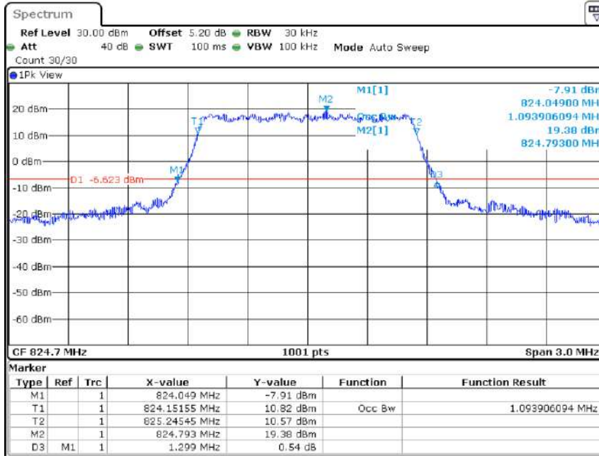
Band26-1.4MHz-QPSK-26797-6RB#0-1.094
