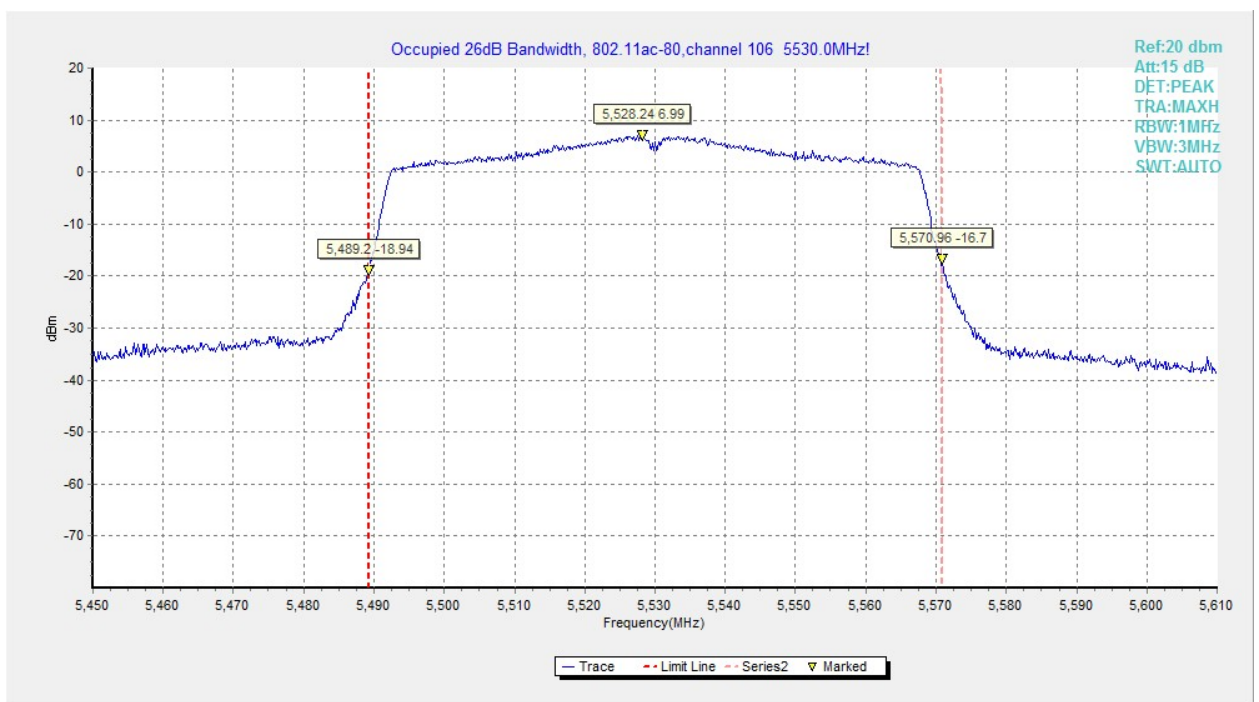
Fig.31 Occupied 26dB Bandwidth (802. 11ac-VHT80, 5530MHz)
