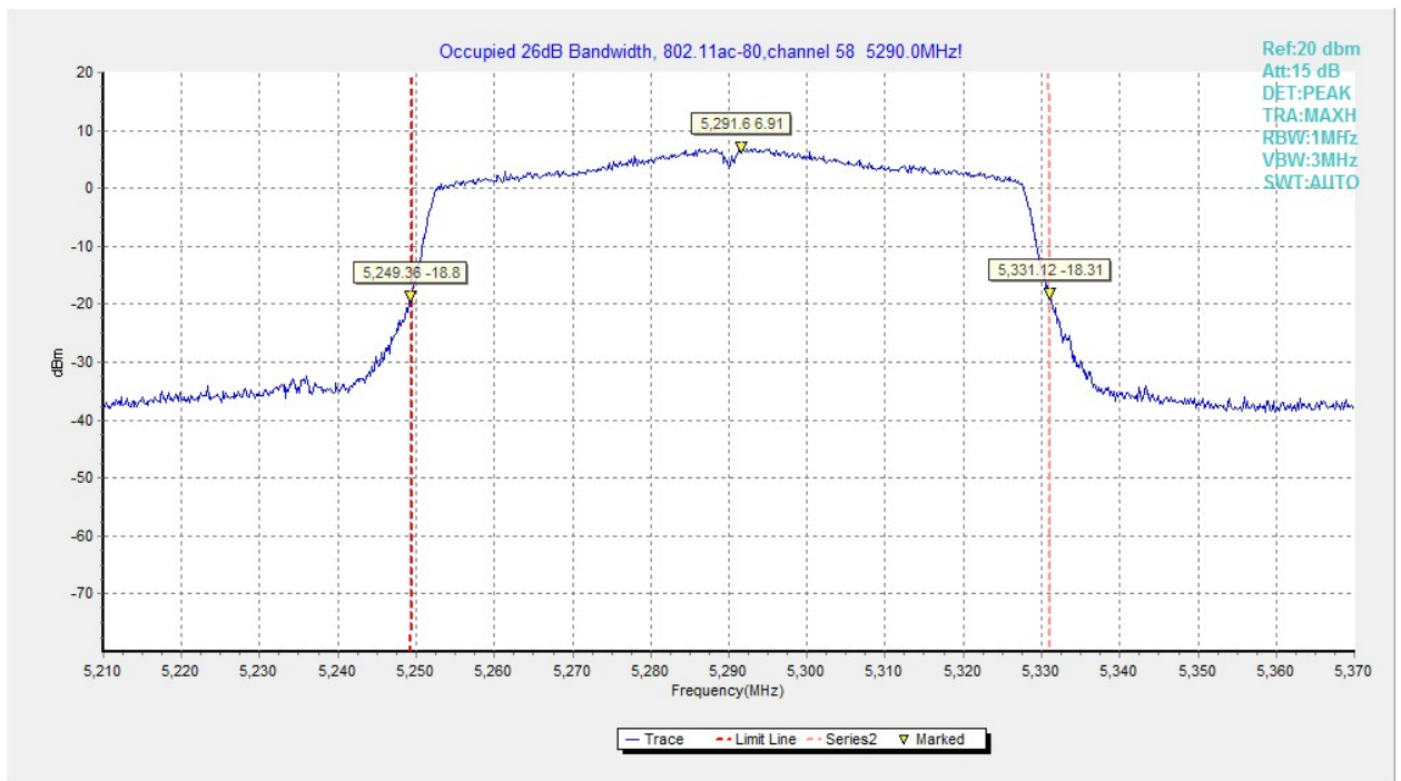
Fig.30 Occupied 26dB Bandwidth (802. 11ac-VHT80, 5290MHz)
