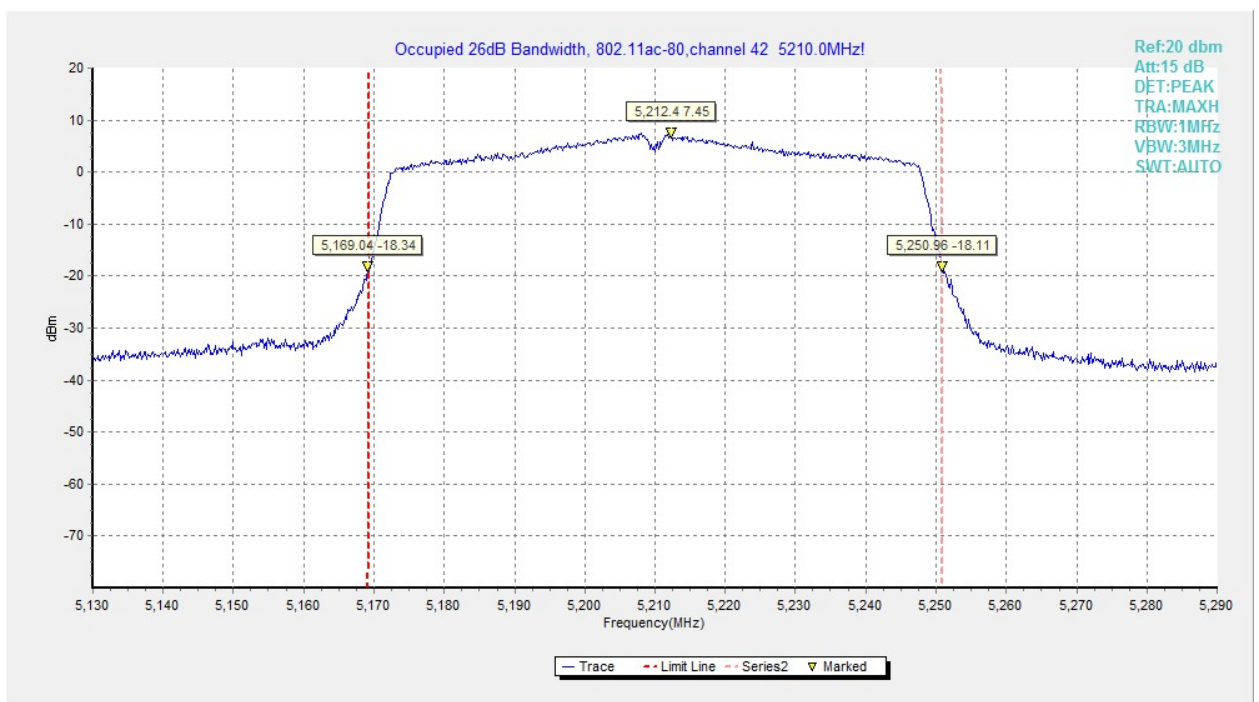
Fig.29 Occupied 26dB Bandwidth (802. 11ac-VHT80, 5210MHz)
