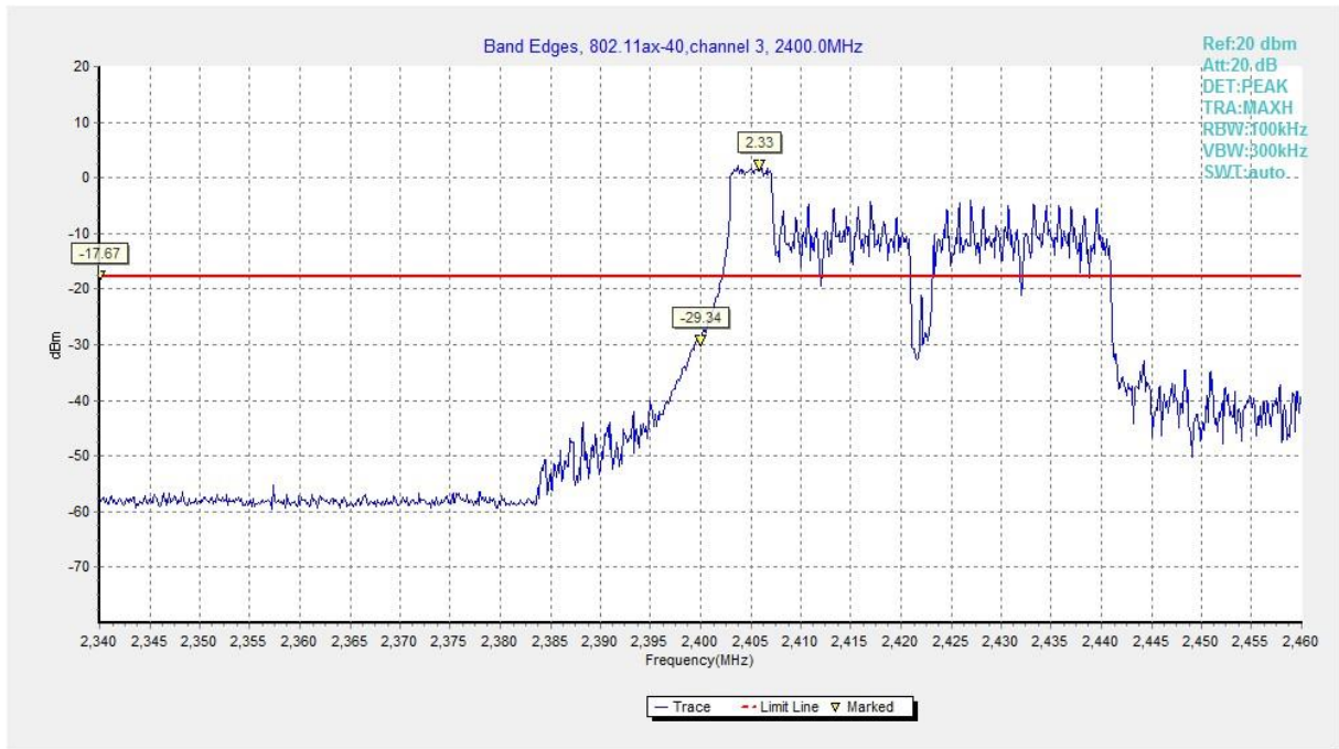
Fig.A.5.29 Band Edges (802.11ax-HE40-RU52-left, Ch 3)
