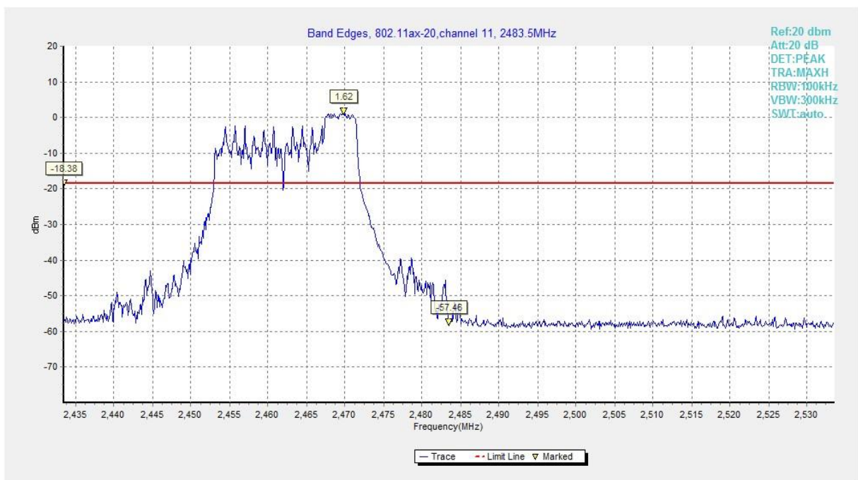
Fig.A.5.14 Band Edges (802.11ax-HE20-RU52-right, Ch 11)
