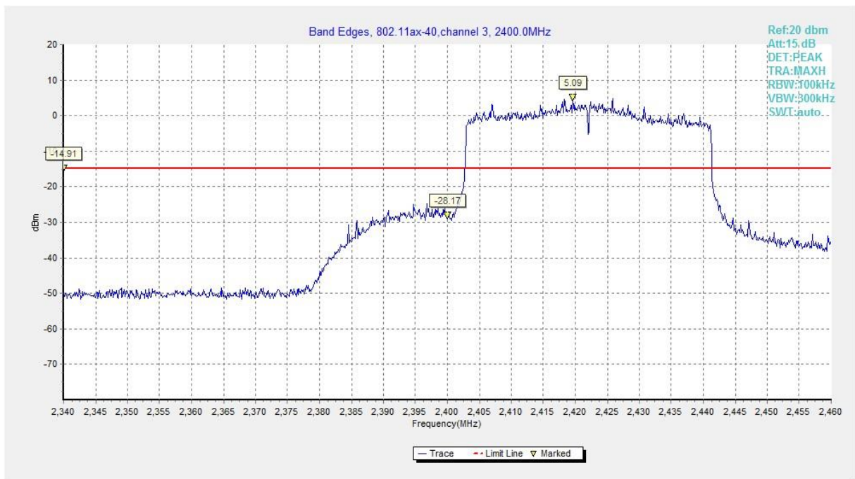
Fig.A.5.11 Band Edges (802.11ax-HE40, Ch 3)
