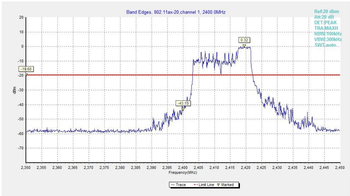
Fig.A.5.41 Band Edges (802.11ax-HE20-RU52-right, Ch 1)
