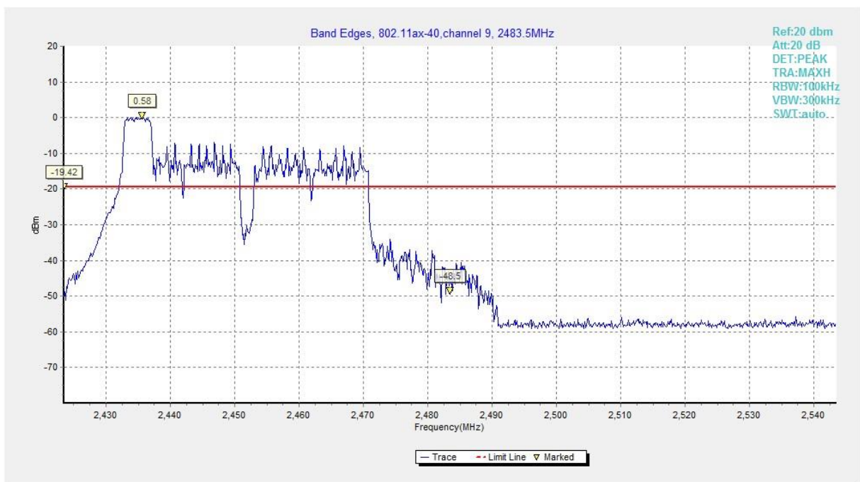
Fig.A.5.44 Band Edges (802.11ax-HE40-RU52-left, Ch 9)
