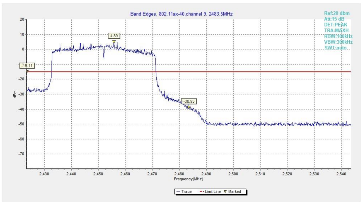
Fig.A.5.12 Band Edges (802.11ax-HE40, Ch 9)
