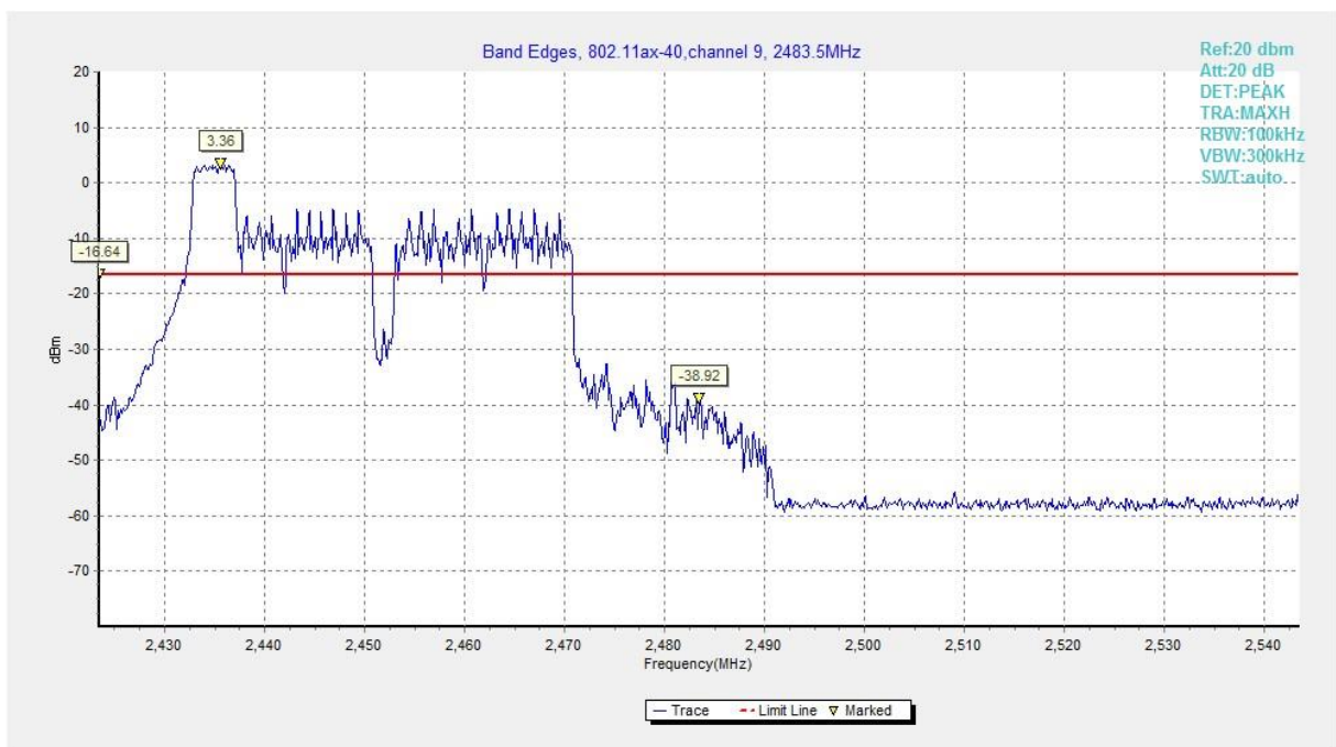
Fig.A.5.16 Band Edges (802.11ax-HE40-RU52-left, Ch 9)
