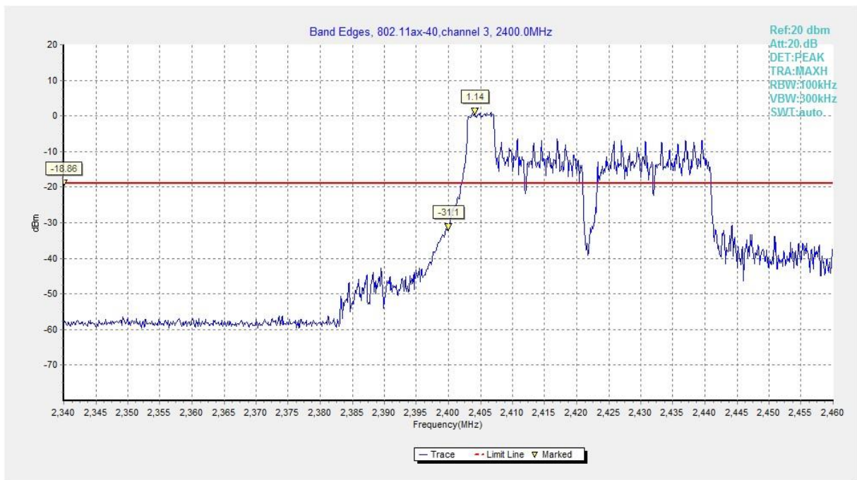
Fig.A.5.43 Band Edges (802.11ax-HE40-RU52-left, Ch 3)
