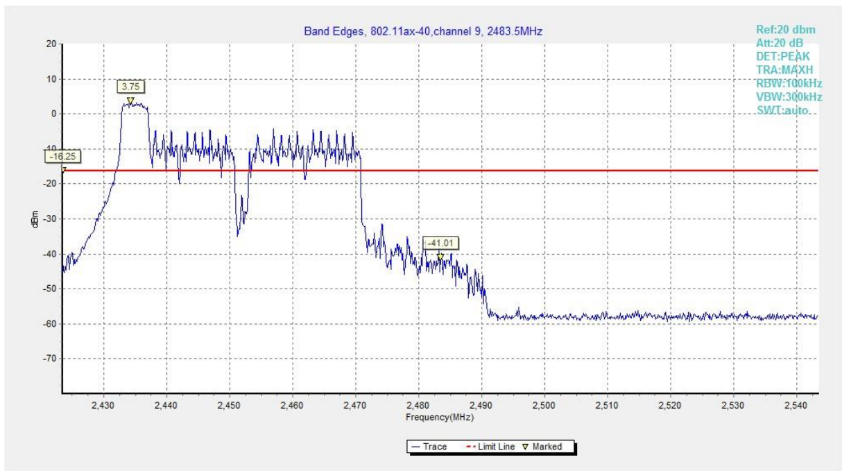
Fig.A.5.30 Band Edges (802.11ax-HE40-RU52-left, Ch 9)
