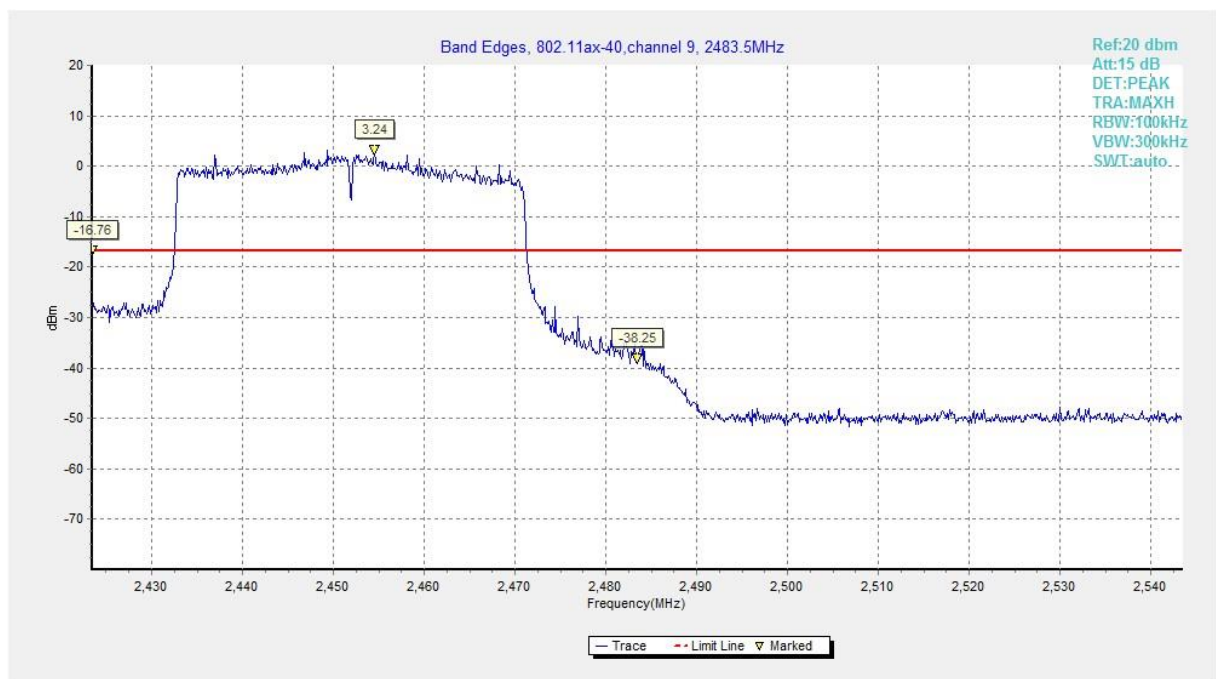
Fig.A.5.26 Band Edges (802.11ax-HE40, Ch 9)
