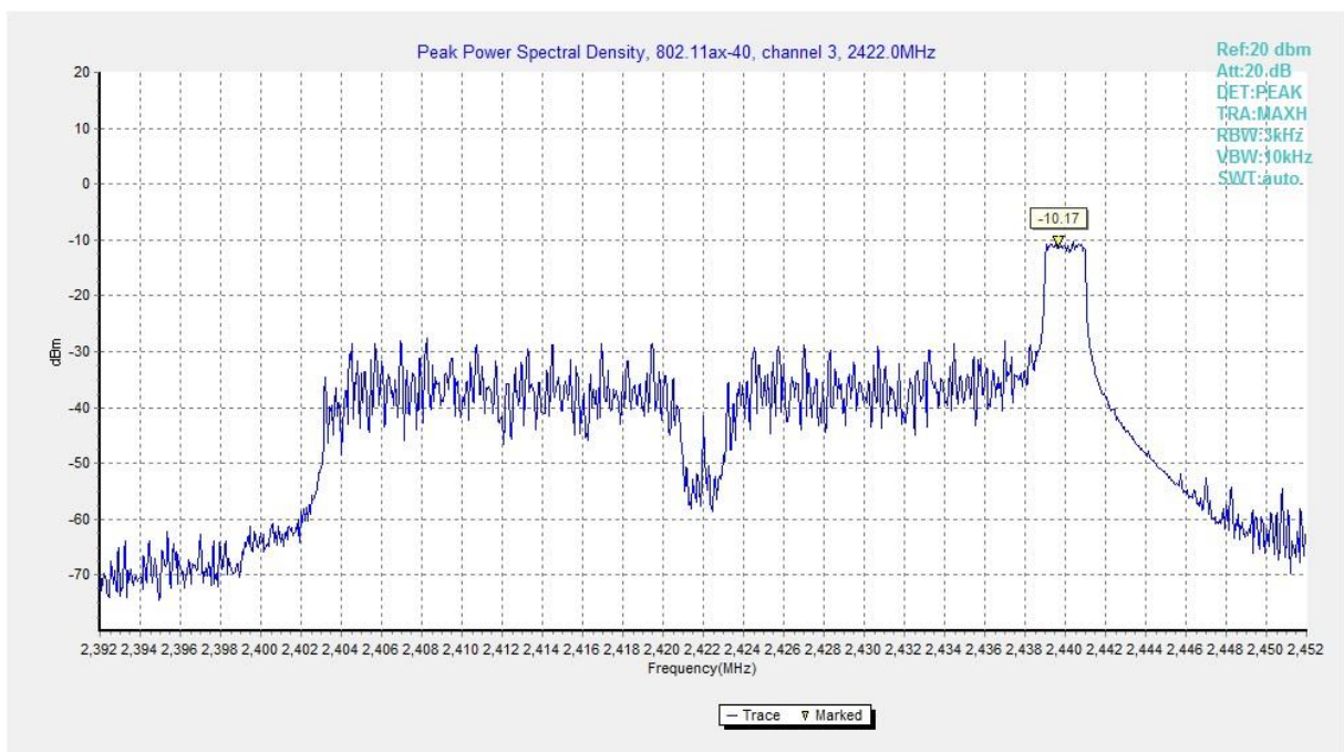
Fig.A.3.55 Power Spectral Density (802.11ax-HE40-RU26-right, Ch 3)
