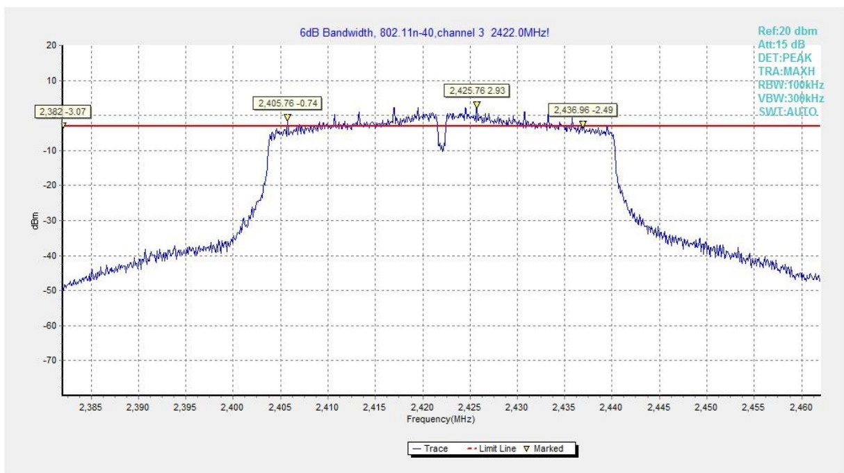
Fig.A.4.25 Occupied 6dB Bandwidth (802.11n-40MHz, Ch 3)
