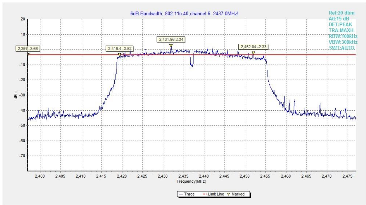
Fig.A.4.26 Occupied 6dB Bandwidth (802.11n-HT40, Ch 6)
