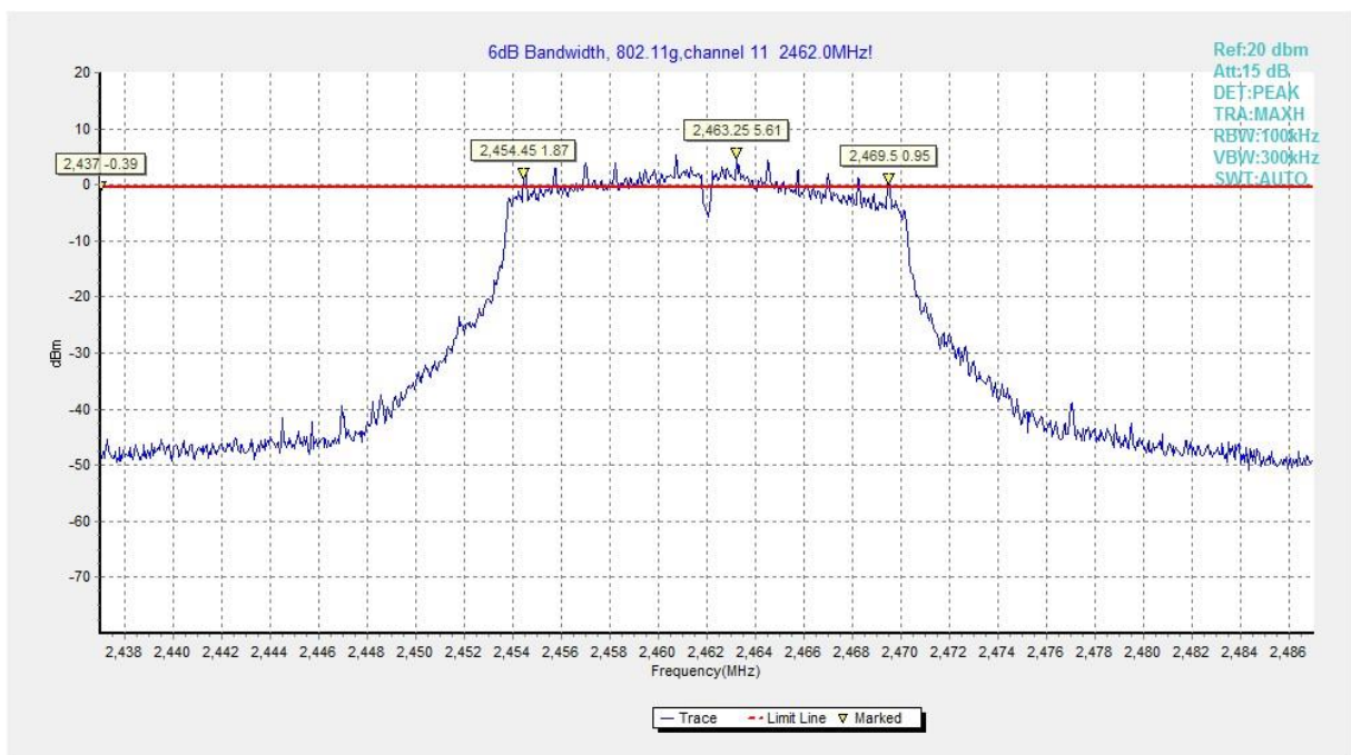
Fig.A.4.21 Occupied 6dB Bandwidth (802.11g, Ch 11)
