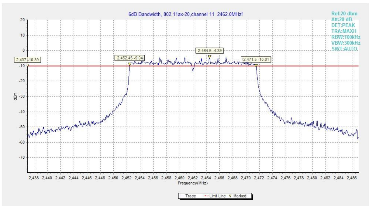
Fig.A.4.15 Occupied 6dB Bandwidth (802.11ax-HE20MHz-RU242, Ch 11)
