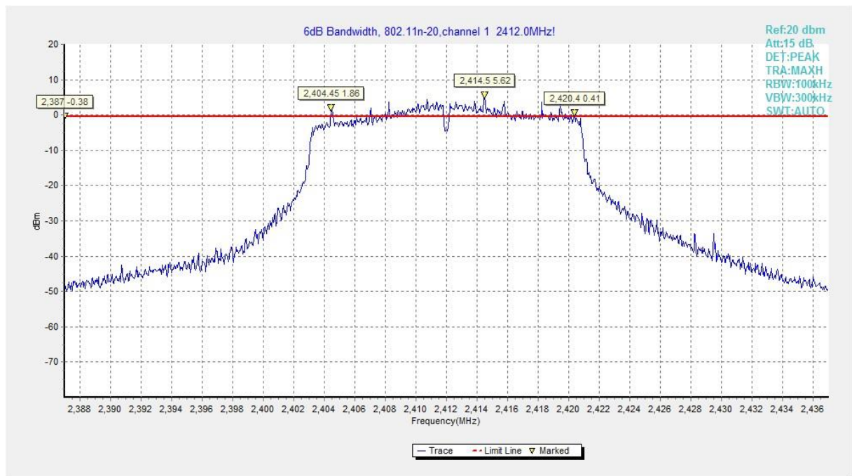
Fig.A.4.22 Occupied 6dB Bandwidth (802.11n-20MHz, Ch 1)
