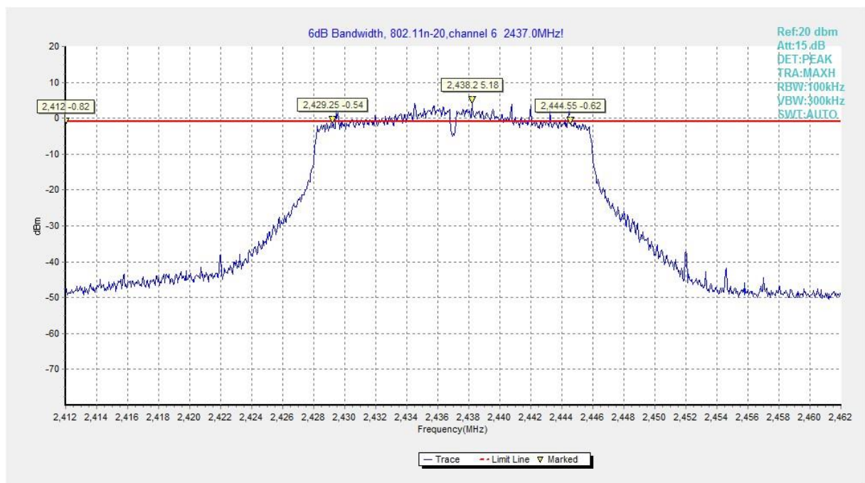
Fig.A.4.23 Occupied 6dB Bandwidth (802.11n-HT20, Ch 6)
