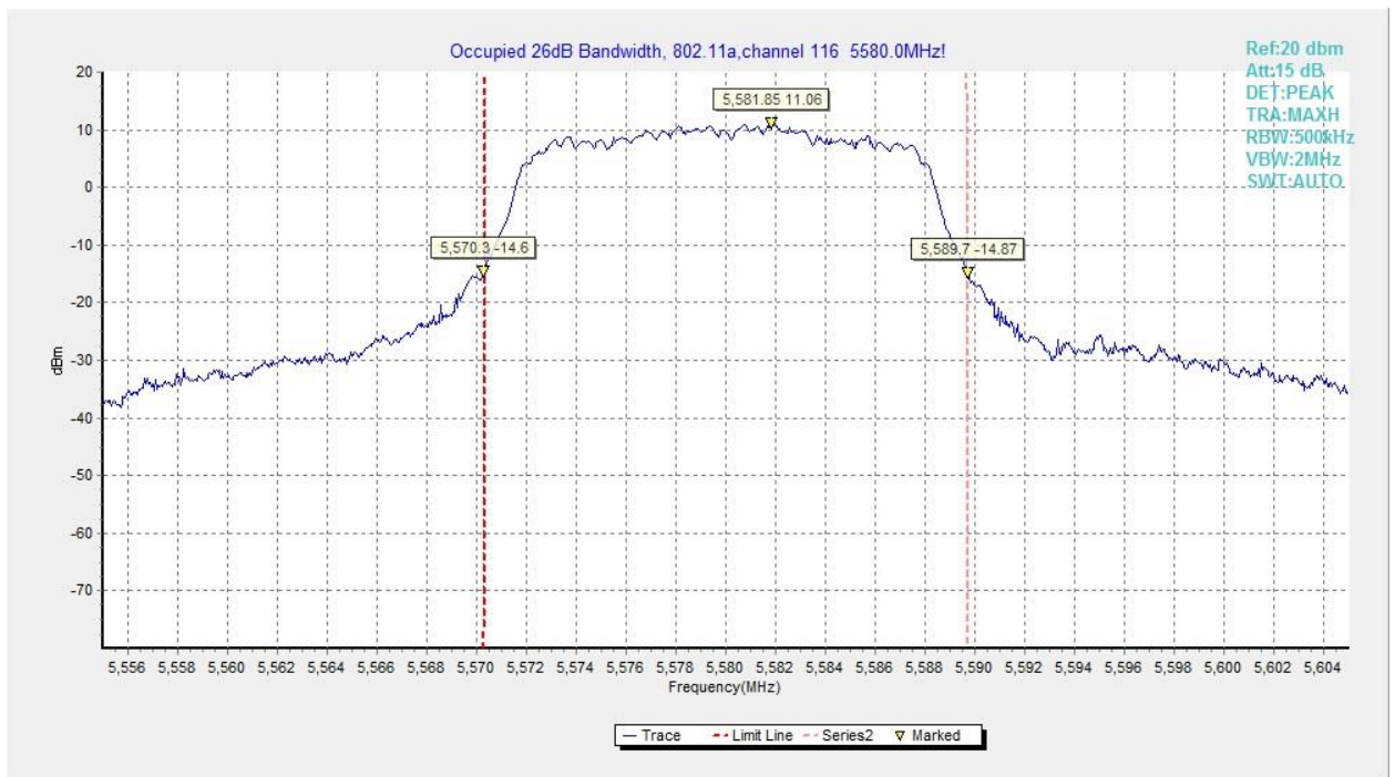
Fig.68 Occupied 26dB Bandwidth (802.11a, 5580MHz)
