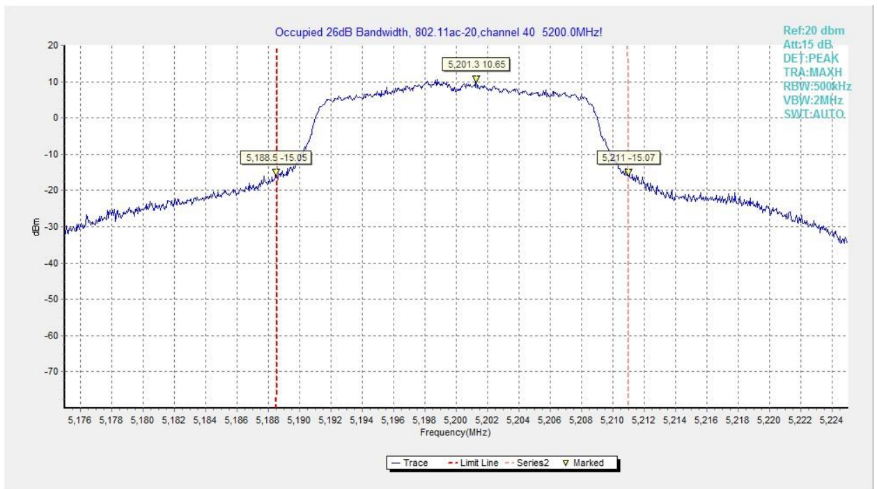
Fig.72 Occupied 26dB Bandwidth (802.11ac-VHT20, 5200MHz)
