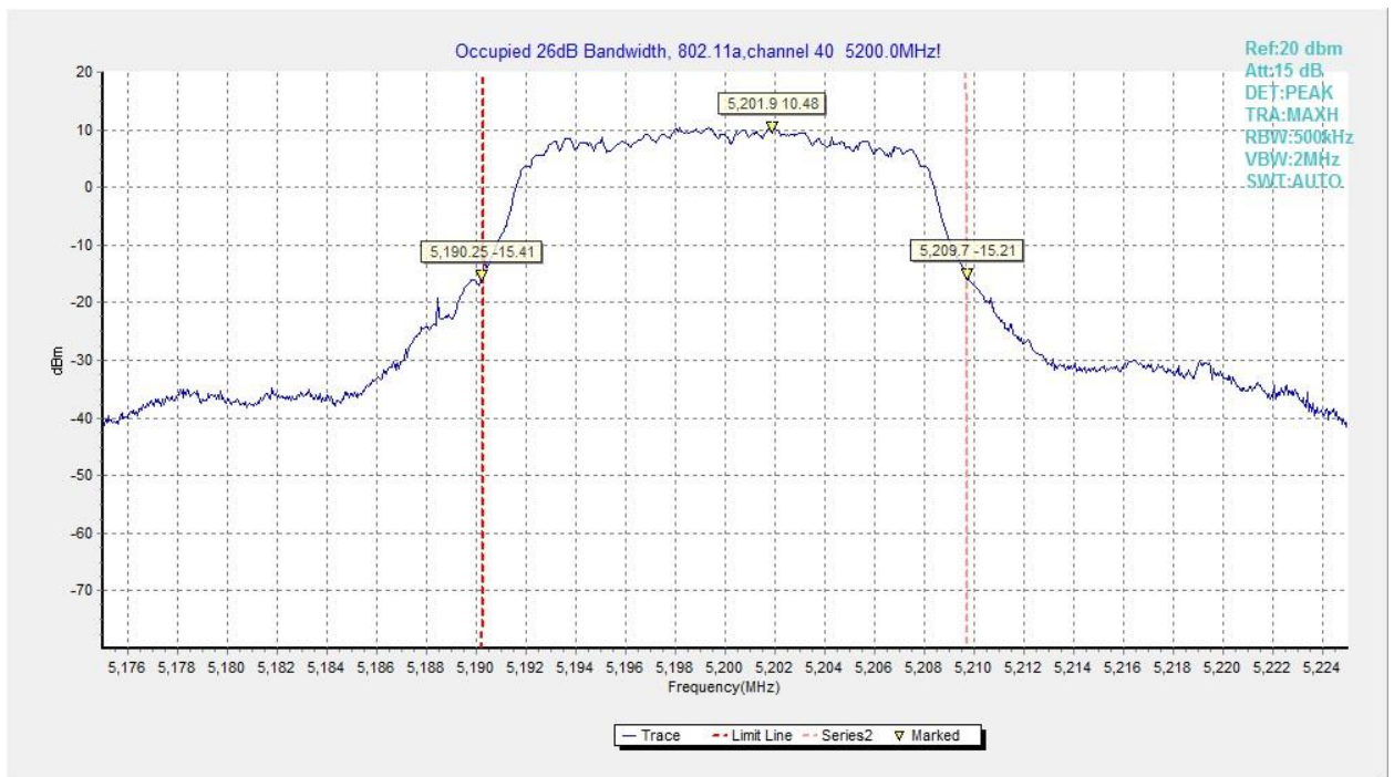
Fig.62 Occupied 26dB Bandwidth (802.11a, 5200MHz)
