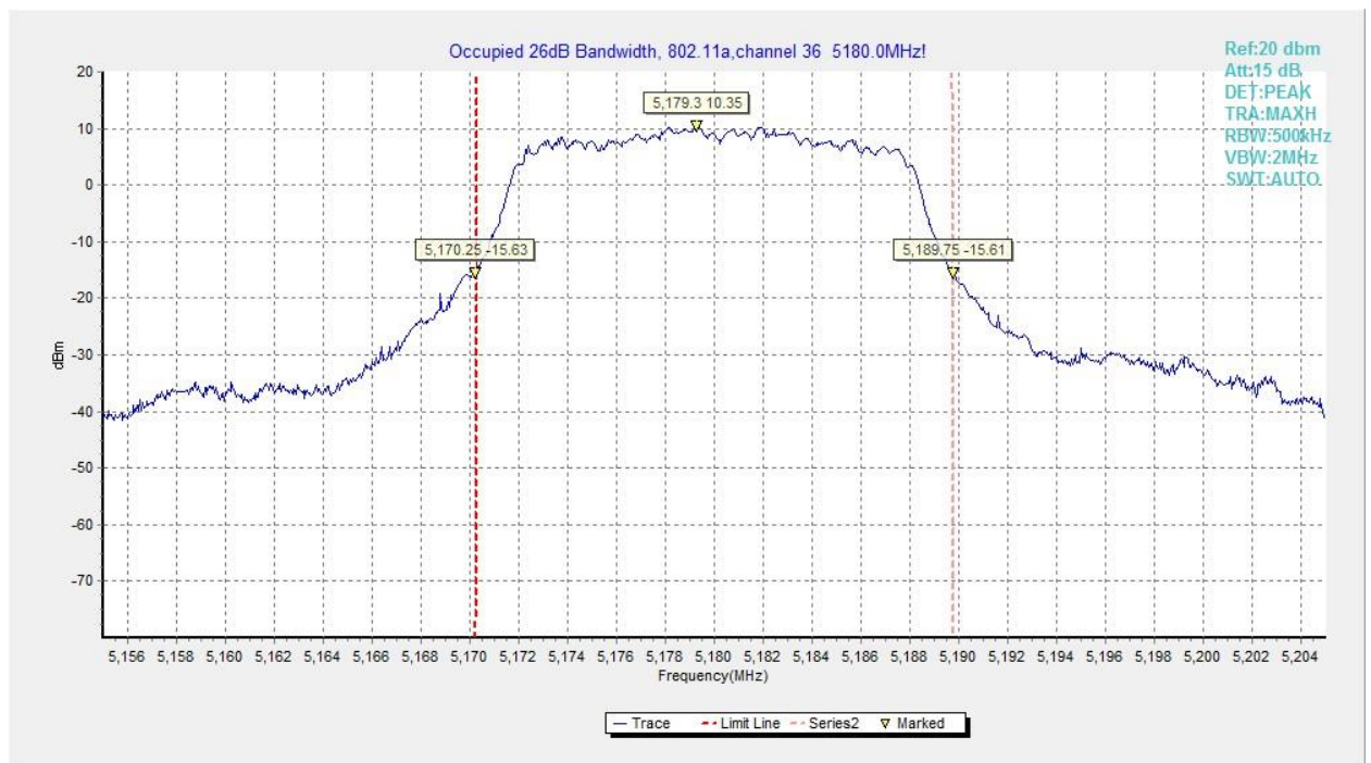
Fig.61 Occupied 26dB Bandwidth (802.11a, 5180MHz)
