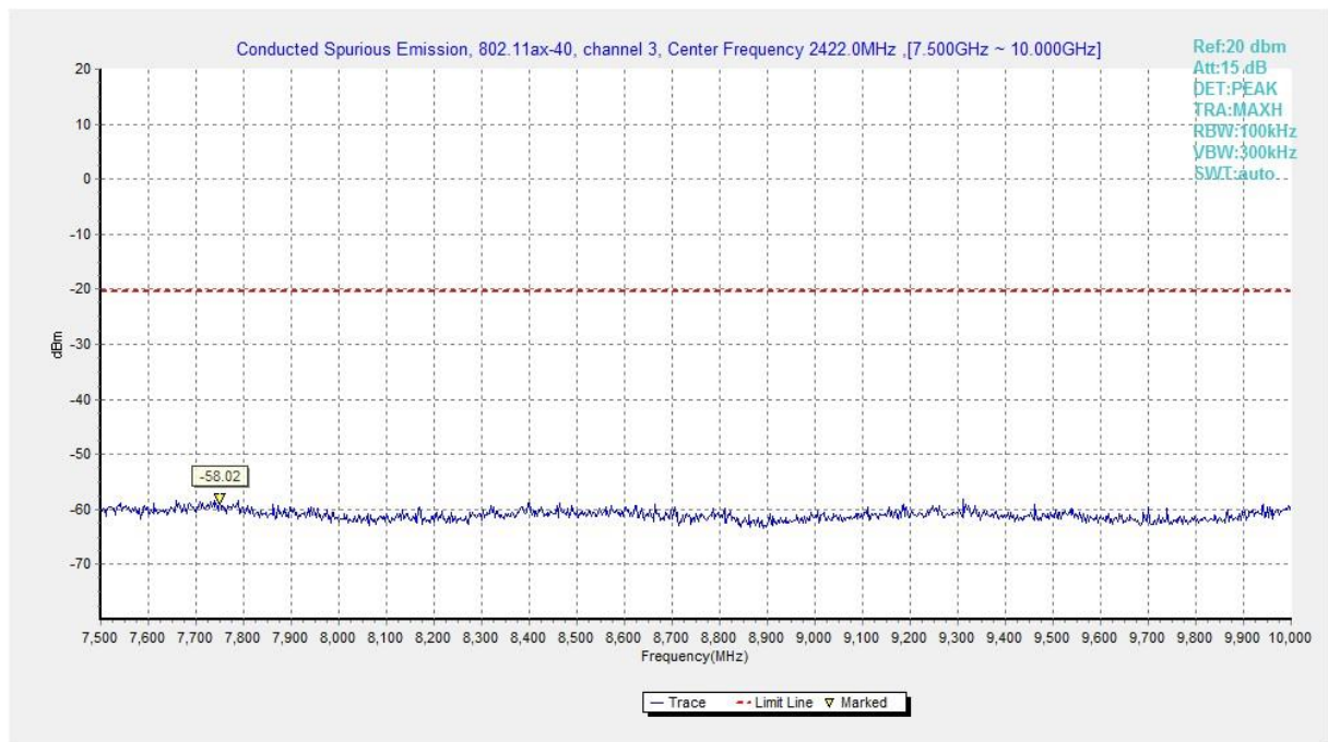
Fig.A.6.1.461 Transmitter Spurious Emission - Conducted (802.11ax-HE40, Ch3, 7.5 GHz-10 GHz)
