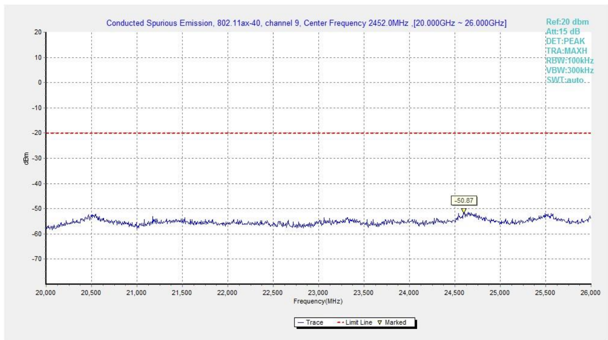
Fig.A.6.1.480 Transmitter Spurious Emission - Conducted (802.11ax-HE40, Ch9, 20 GHz-26 GHz)
