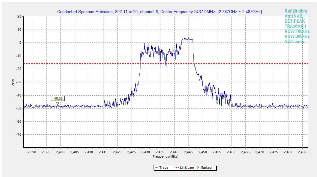
Fig.A.6.1.489 Transmitter Spurious Emission - Conducted (802.11ax-HE20-RU52-right, Ch6, Center Frequency)
