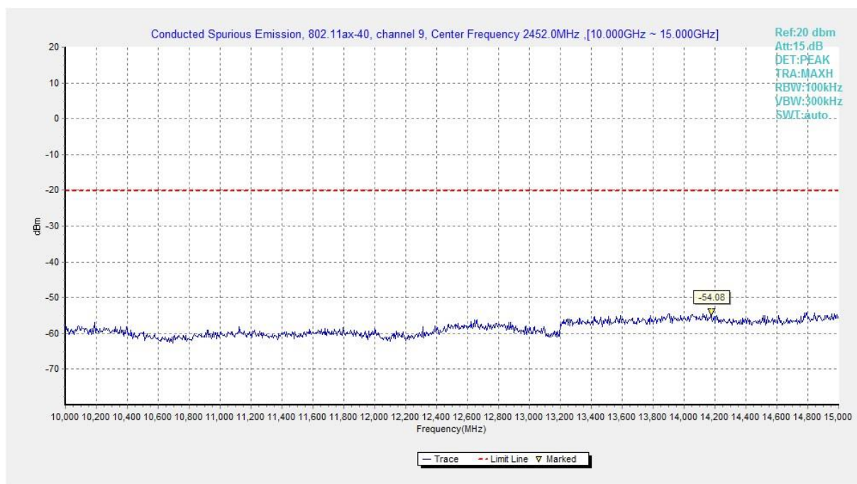
Fig.A.6.1.478 Transmitter Spurious Emission - Conducted (802.11ax-HE40, Ch9, 10 GHz-15 GHz)
