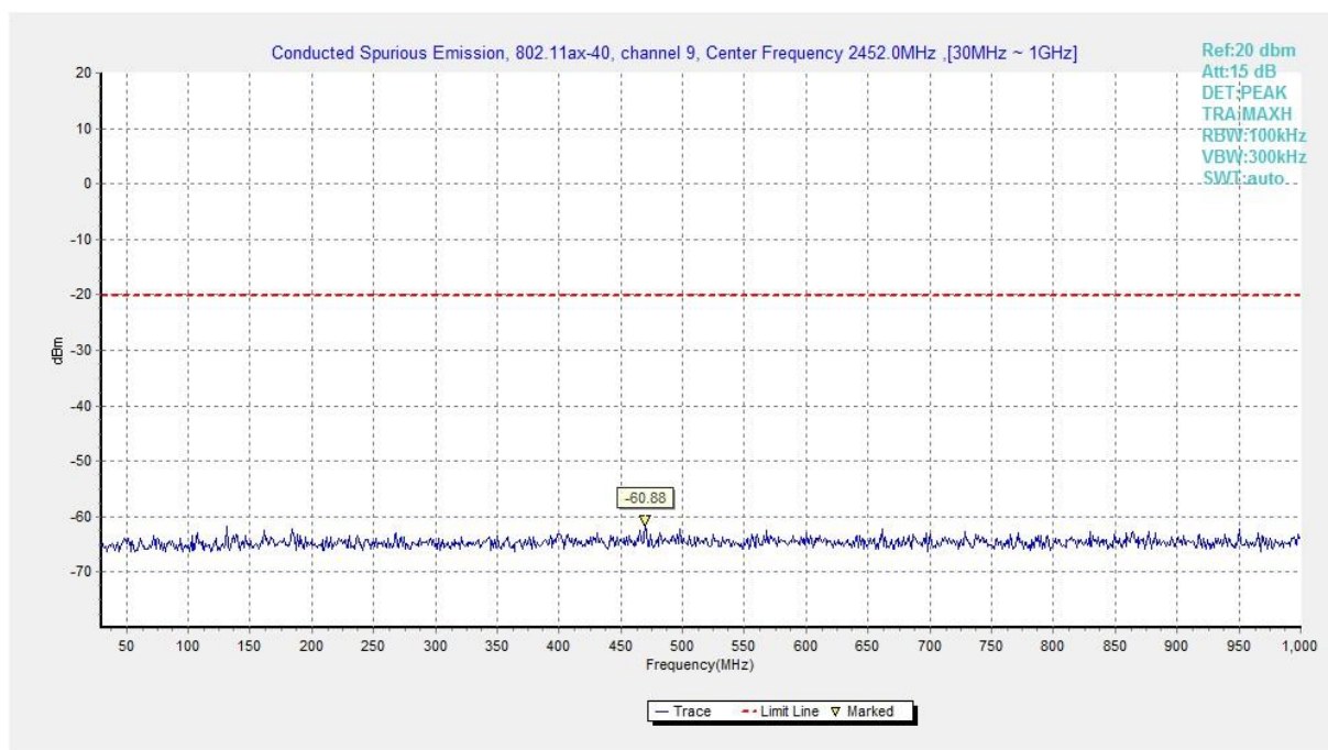
Fig.A.6.1.474 Transmitter Spurious Emission - Conducted (802.11ax-HE40, Ch9, 30 MHz-1 GHz)
