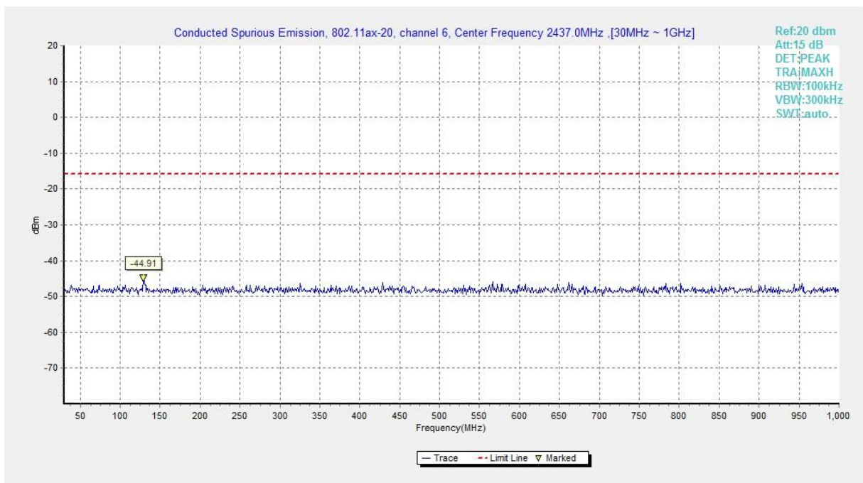
Fig.A.6.1.490 Transmitter Spurious Emission - Conducted (802.11ax-HE20-RU52-right, Ch6, 30 MHz-1 GHz)
