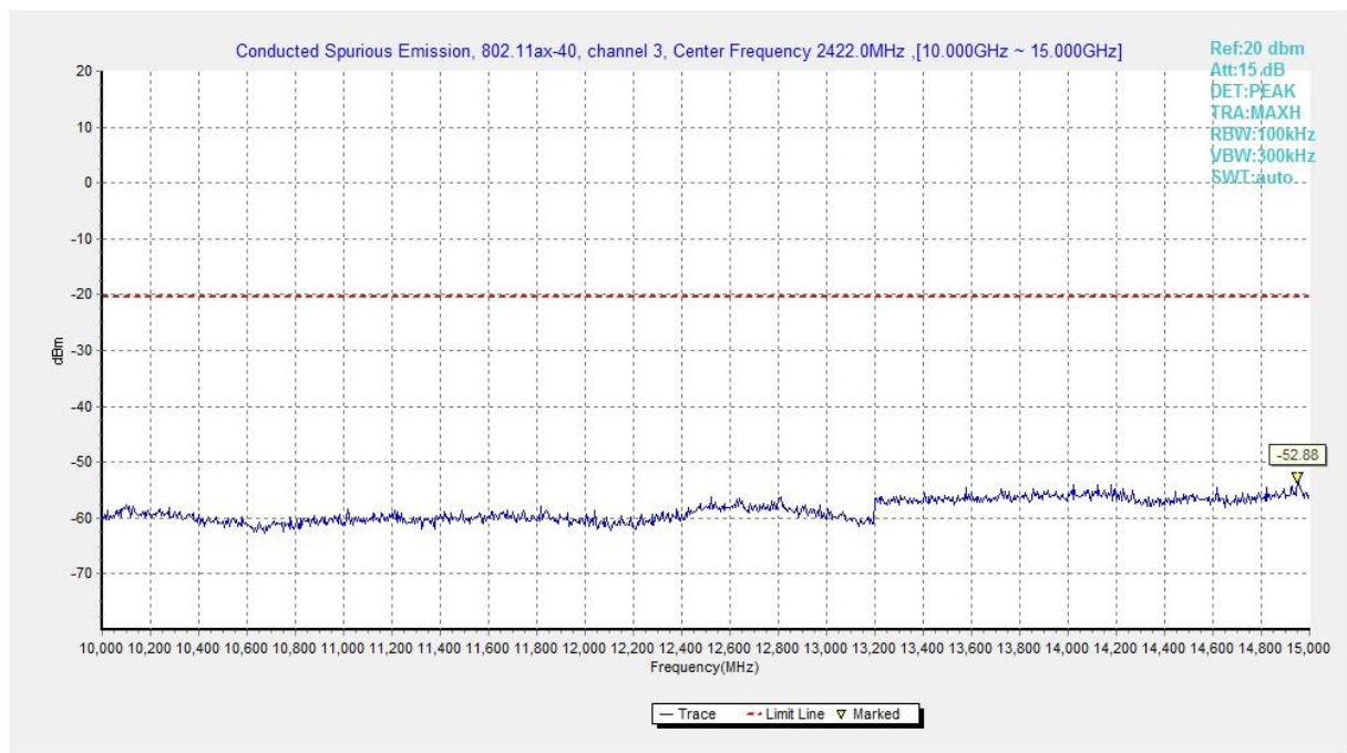
Fig.A.6.1.462 Transmitter Spurious Emission - Conducted (802.11ax-HE40, Ch3, 10 GHz-15 GHz)
