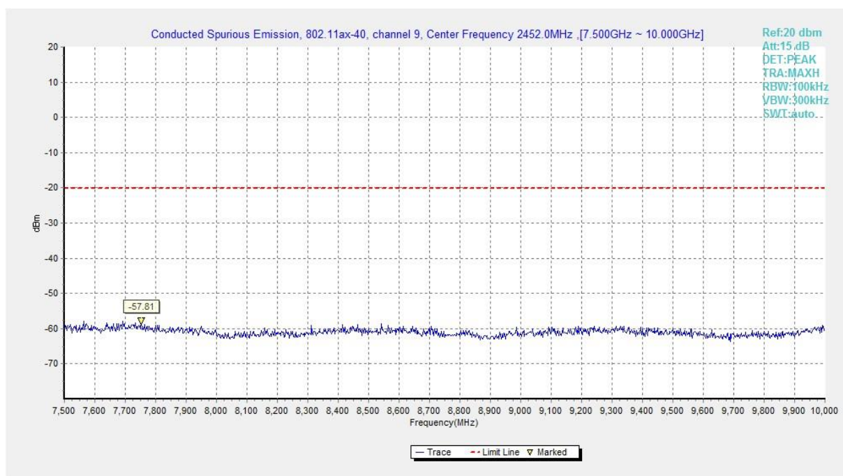
Fig.A.6.1.477 Transmitter Spurious Emission - Conducted (802.11ax-HE40, Ch9, 7.5 GHz-10 GHz)
