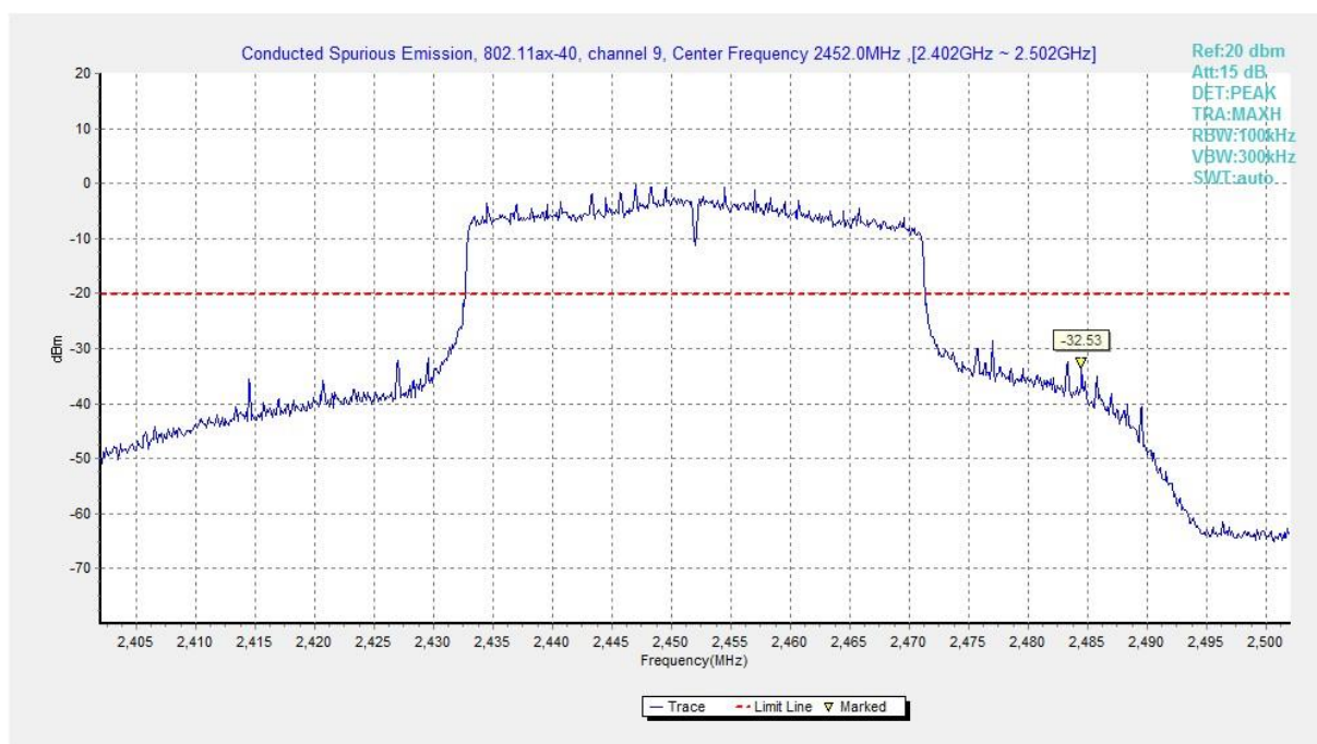
Fig.A.6.1.473 Transmitter Spurious Emission - Conducted (802.11ax-HE40, Ch9, Center Frequency)
