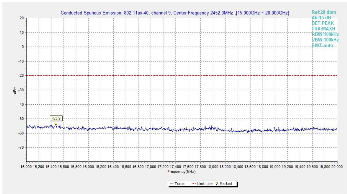
Fig.A.6.1.479 Transmitter Spurious Emission - Conducted (802.11ax-HE40, Ch9, 15 GHz-20 GHz)
