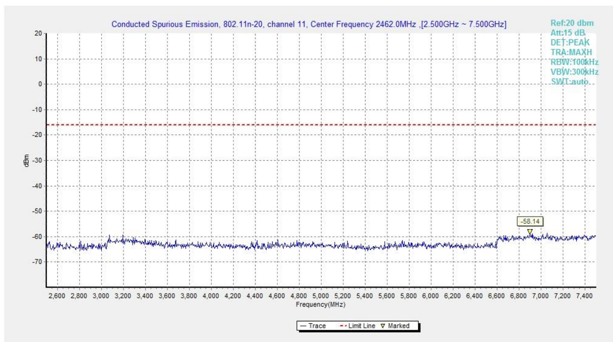
Fig.A.6.1.404 Transmitter Spurious Emission - Conducted (802.11n-HT20, Ch11, 2.5 GHz-7.5 GHz)
