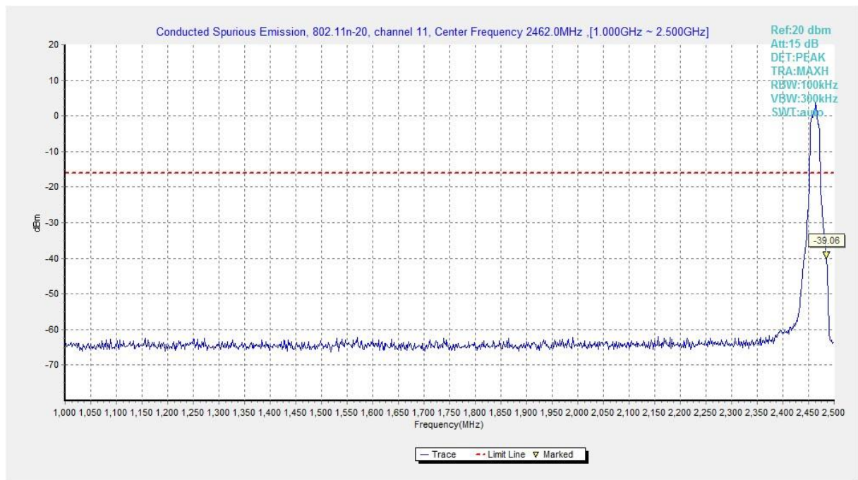
Fig.A.6.1.403 Transmitter Spurious Emission - Conducted (802.11n-HT20, Ch11, 1 GHz-2.5 GHz)
