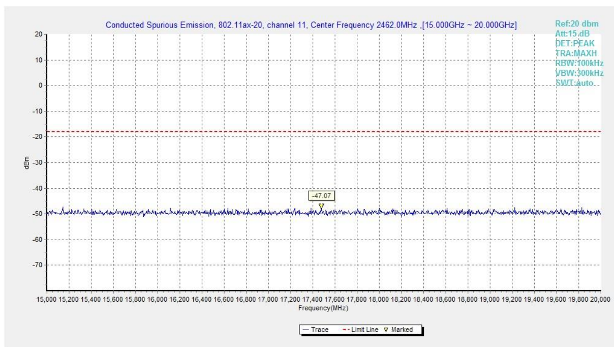
Fig.A.6.1.335 Transmitter Spurious Emission - Conducted (802.11ax-HE20-RU52-right, Ch11, 15 GHz-20 GHz)
