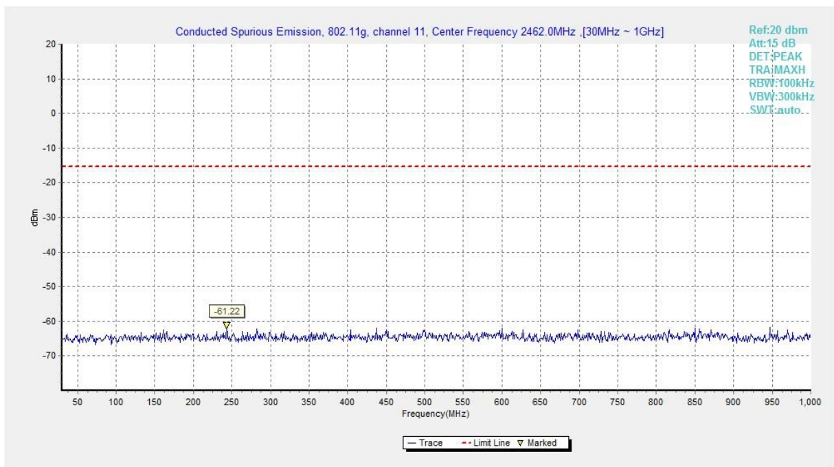
Fig.A.6.1.378 Transmitter Spurious Emission - Conducted (802.11g, Ch11, 30 MHz-1 GHz)
