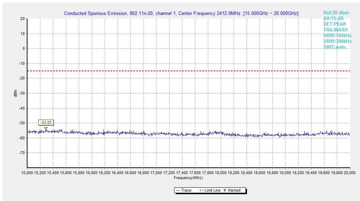
Fig.A.6.1.391 Transmitter Spurious Emission - Conducted (802.11n-HT20, Ch1, 15 GHz-20 GHz)
