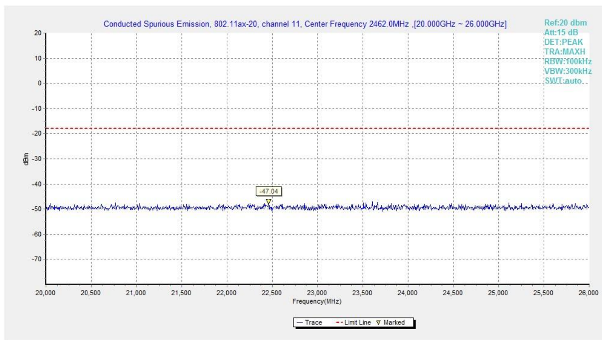
Fig.A.6.1.336 Transmitter Spurious Emission - Conducted (802.11ax-HE20-RU52-right, Ch11, 20 GHz-26 GHz)
