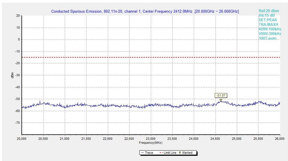
Fig.A.6.1.392 Transmitter Spurious Emission - Conducted (802.11n-HT20, Ch1, 20 GHz-26 GHz)
