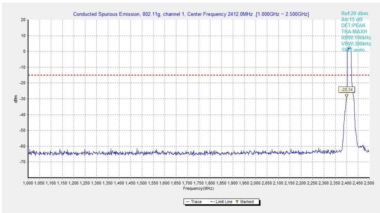
Fig.A.6.1.363 Transmitter Spurious Emission - Conducted (802.11g, Ch1, 1 GHz-2.5 GHz)
