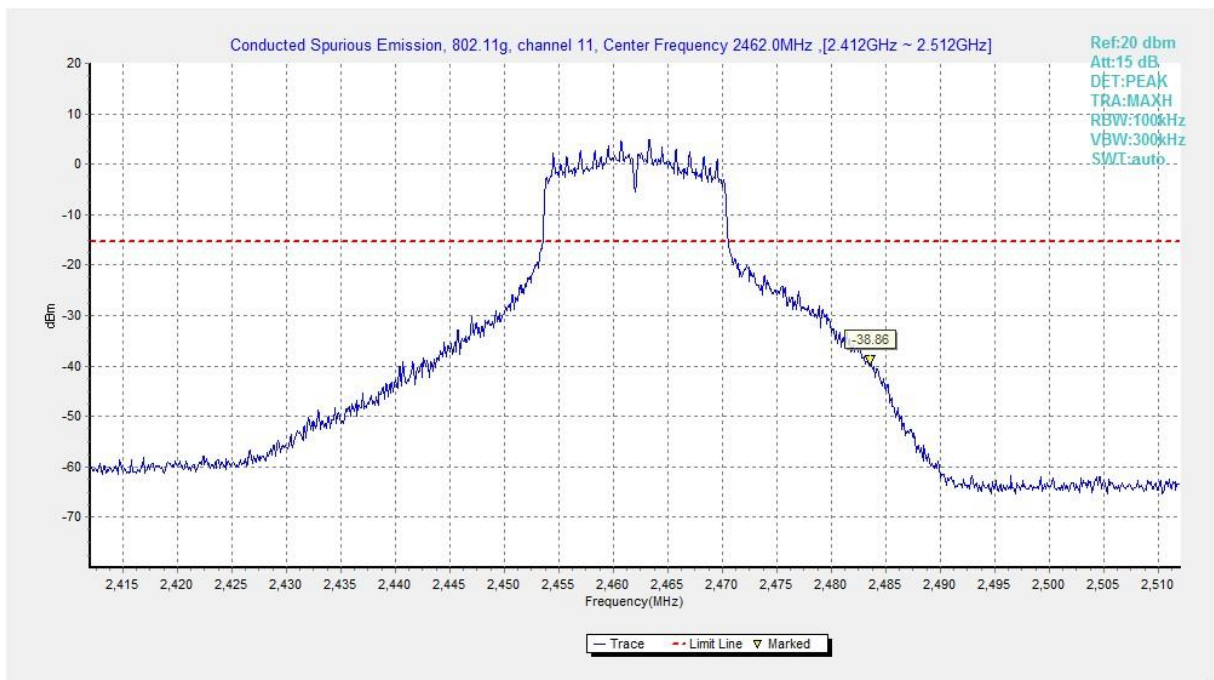
Fig.A.6.1.377 Transmitter Spurious Emission - Conducted (802.11g, Ch11, Center Frequency)
