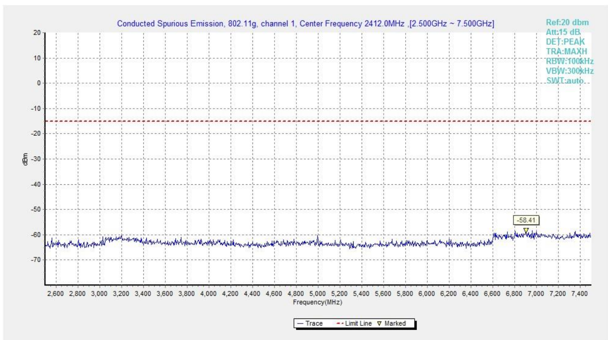
Fig.A.6.1.364 Transmitter Spurious Emission - Conducted (802.11g, Ch1, 2.5 GHz-7.5 GHz)
