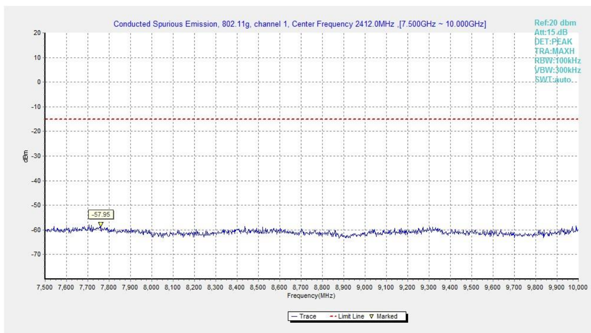
Fig.A.6.1.365 Transmitter Spurious Emission - Conducted (802.11g, Ch1, 7.5 GHz-10 GHz)
