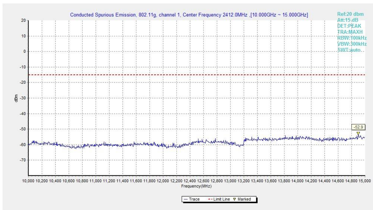
Fig.A.6.1.366 Transmitter Spurious Emission - Conducted (802.11g, Ch1, 10 GHz-15 GHz)
