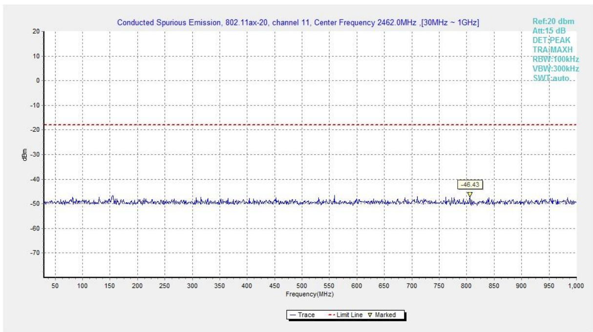
Fig.A.6.1.330 Transmitter Spurious Emission - Conducted (802.11ax-HE20-RU52-right, Ch11, 30 MHz-1 GHz)
