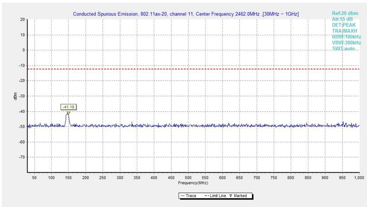
Fig.A.6.1.282 Transmitter Spurious Emission - Conducted (802.11ax-HE20, Ch11, 30 MHz-1 GHz)
