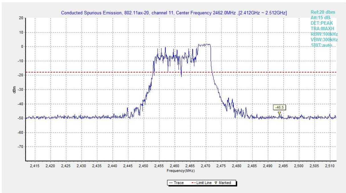
Fig.A.6.1.329 Transmitter Spurious Emission - Conducted (802.11ax-HE20-RU52-right, Ch11, Center Frequency)
