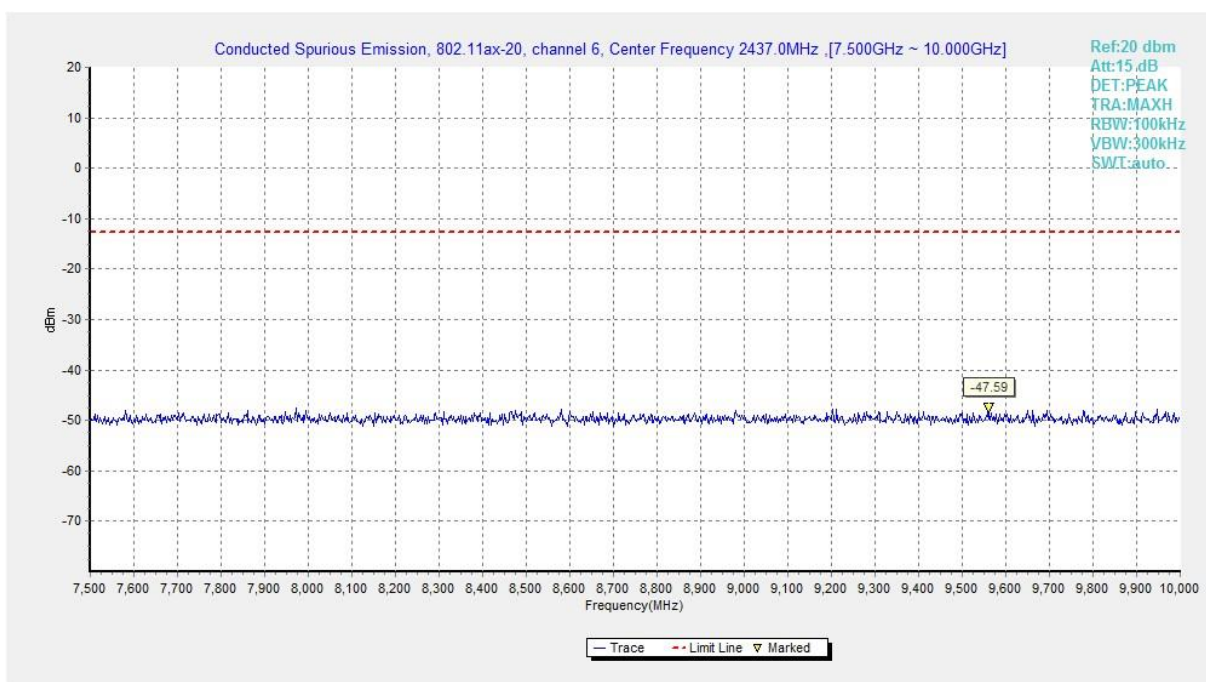
Fig.A.6.1.277 Transmitter Spurious Emission - Conducted (802.11ax-HE20, Ch6, 7.5 GHz-10 GHz)
