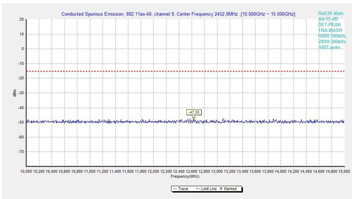
Fig.A.6.1.310 Transmitter Spurious Emission - Conducted (802.11ax-HE40, Ch9, 10 GHz-15 GHz)
