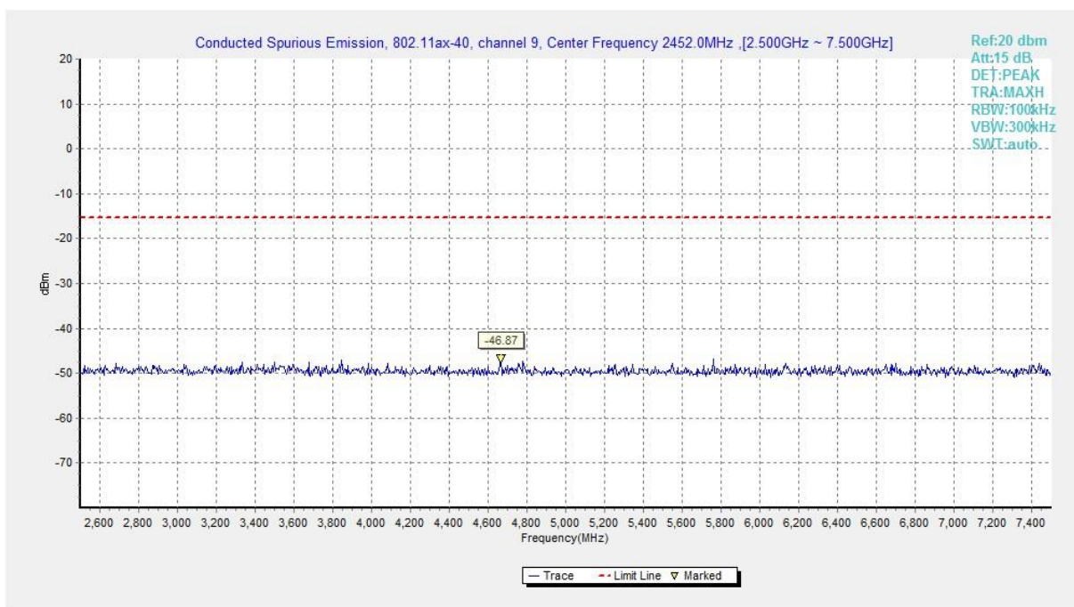
Fig.A.6.1.308 Transmitter Spurious Emission - Conducted (802.11ax-HE40, Ch9, 2.5 GHz-7.5 GHz)
