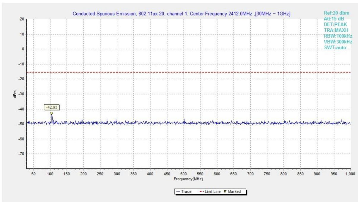
Fig.A.6.1.314 Transmitter Spurious Emission - Conducted (802.11ax-HE20-RU52-right, Ch1, 30 MHz-1 GHz)
