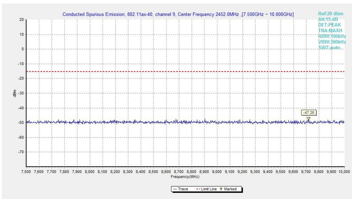
Fig.A.6.1.309 Transmitter Spurious Emission - Conducted (802.11ax-HE40, Ch9, 7.5 GHz-10 GHz)
