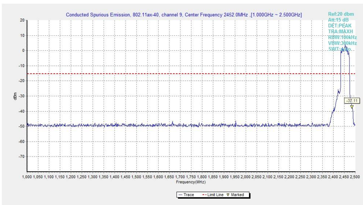
Fig.A.6.1.307 Transmitter Spurious Emission - Conducted (802.11ax-HE40, Ch9, 1 GHz-2.5 GHz)
