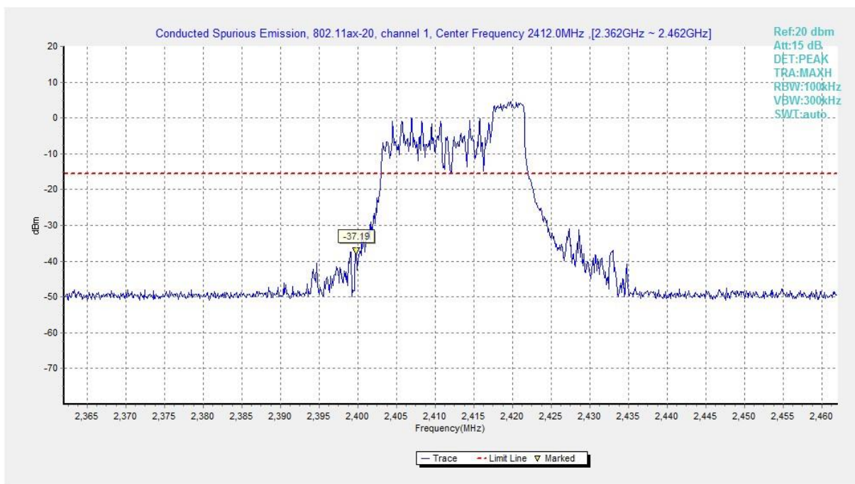
Fig.A.6.1.313 Transmitter Spurious Emission - Conducted (802.11ax-HE20-RU52-right, Ch1, Center Frequency)
