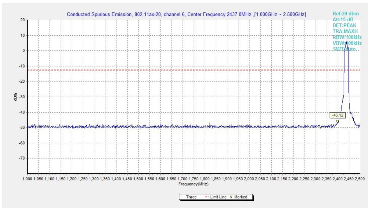
Fig.A.6.1.275 Transmitter Spurious Emission - Conducted (802.11ax-HE20, Ch6, 1 GHz-2.5 GHz)
