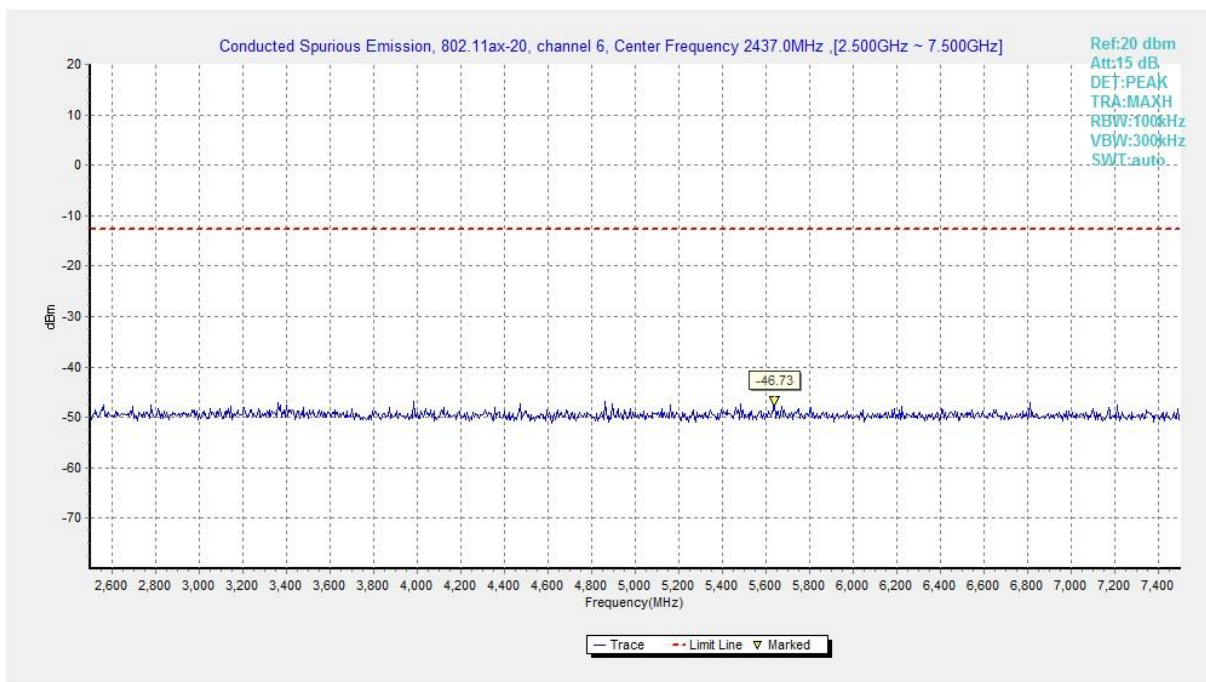
Fig.A.6.1.276 Transmitter Spurious Emission - Conducted (802.11ax-HE20, Ch6, 2.5 GHz-7.5 GHz)
