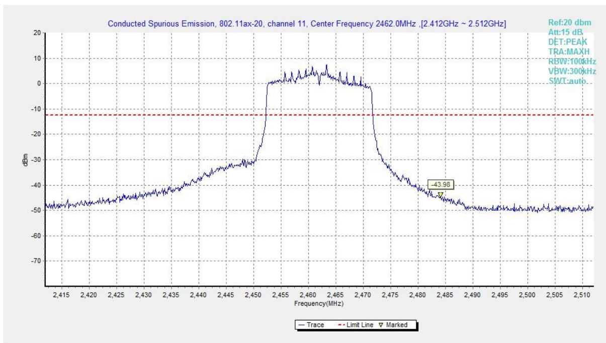
Fig.A.6.1.281 Transmitter Spurious Emission - Conducted (802.11ax-HE20, Ch11, Center Frequency)
