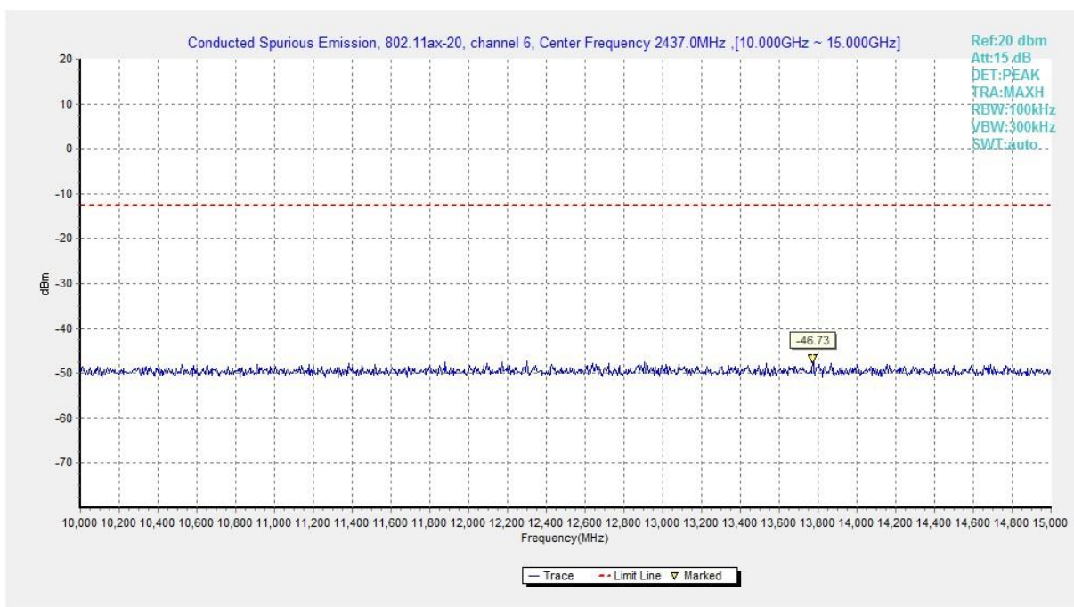
Fig.A.6.1.278 Transmitter Spurious Emission - Conducted (802.11ax-HE20, Ch6, 10 GHz-15 GHz)
