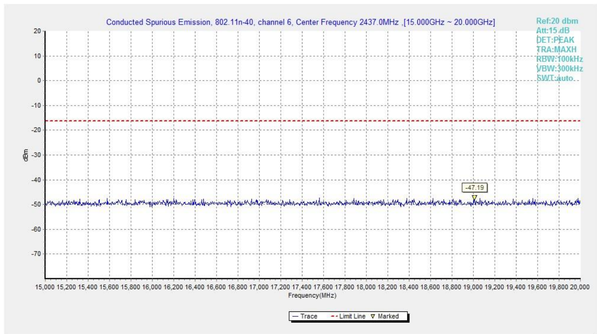
Fig.A.6.1.255 Transmitter Spurious Emission - Conducted (802.11n-HT40, Ch6, 15 GHz-20 GHz)
