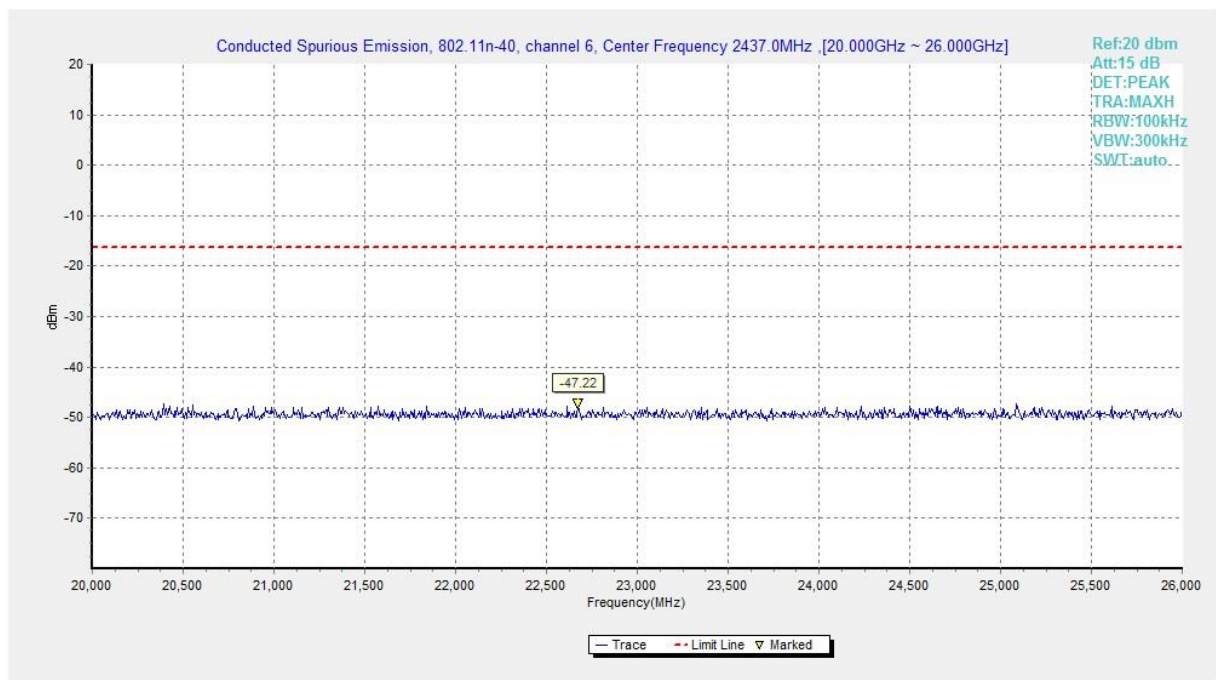
Fig.A.6.1.256 Transmitter Spurious Emission - Conducted (802.11n-HT40, Ch6, 20 GHz-26 GHz)
