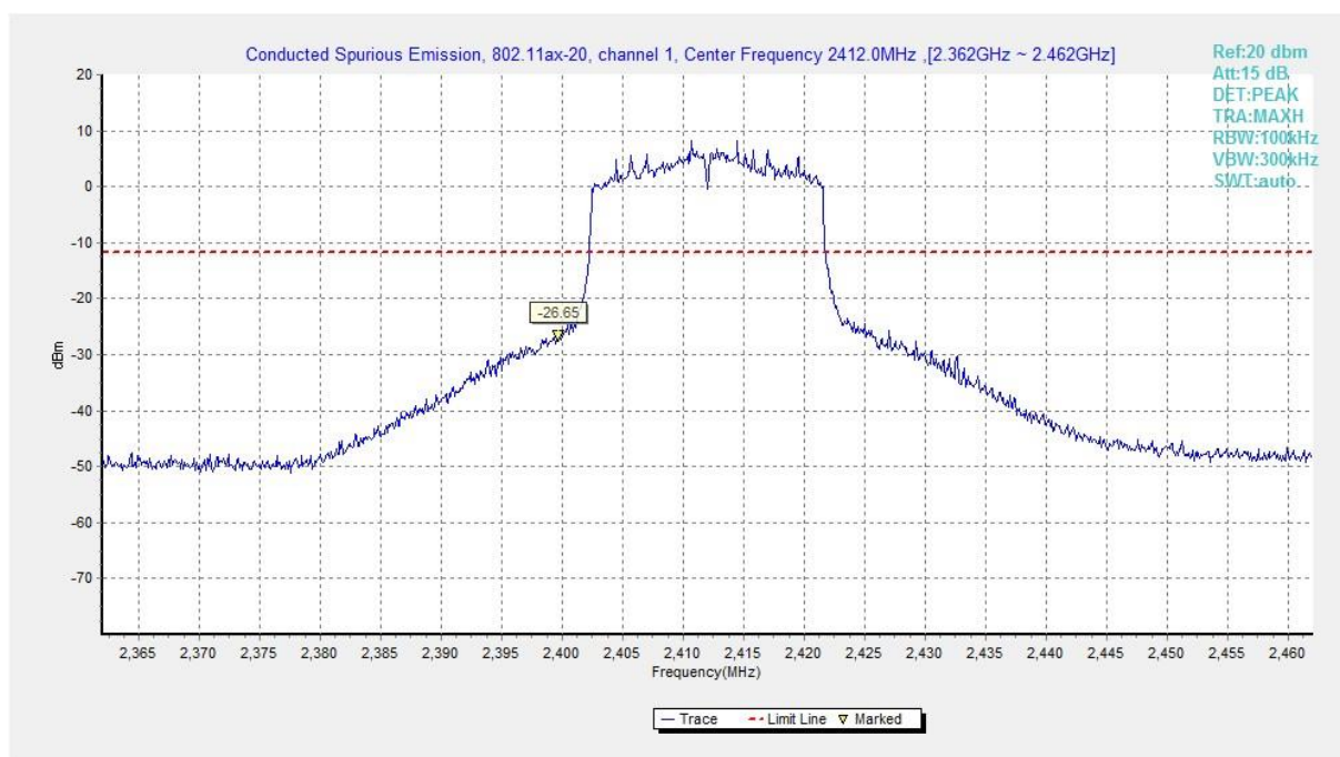
Fig.A.6.1.97 Transmitter Spurious Emission - Conducted (802.11ax-HE20, Ch1, Center Frequency)
