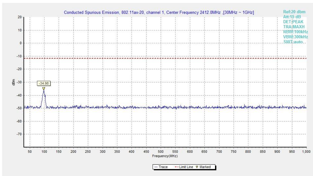
Fig.A.6.1.98 Transmitter Spurious Emission - Conducted (802.11ax-HE20, Ch1, 30 MHz-1 GHz)
