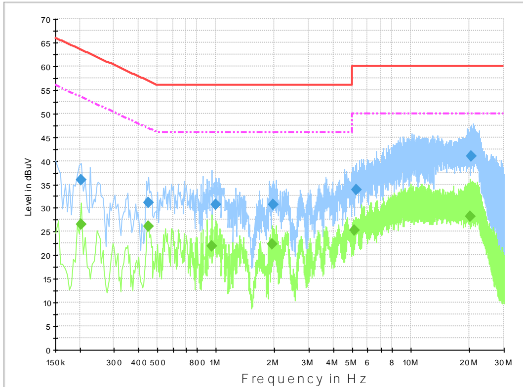
Figure A.18 Conducted Emission
