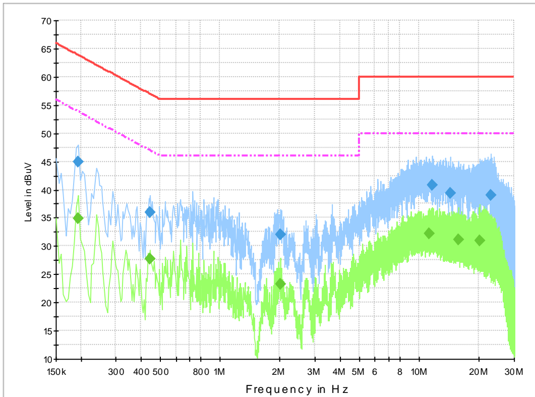
Fig.B.11.2 AC Powerline Conducted Emission-Idle
