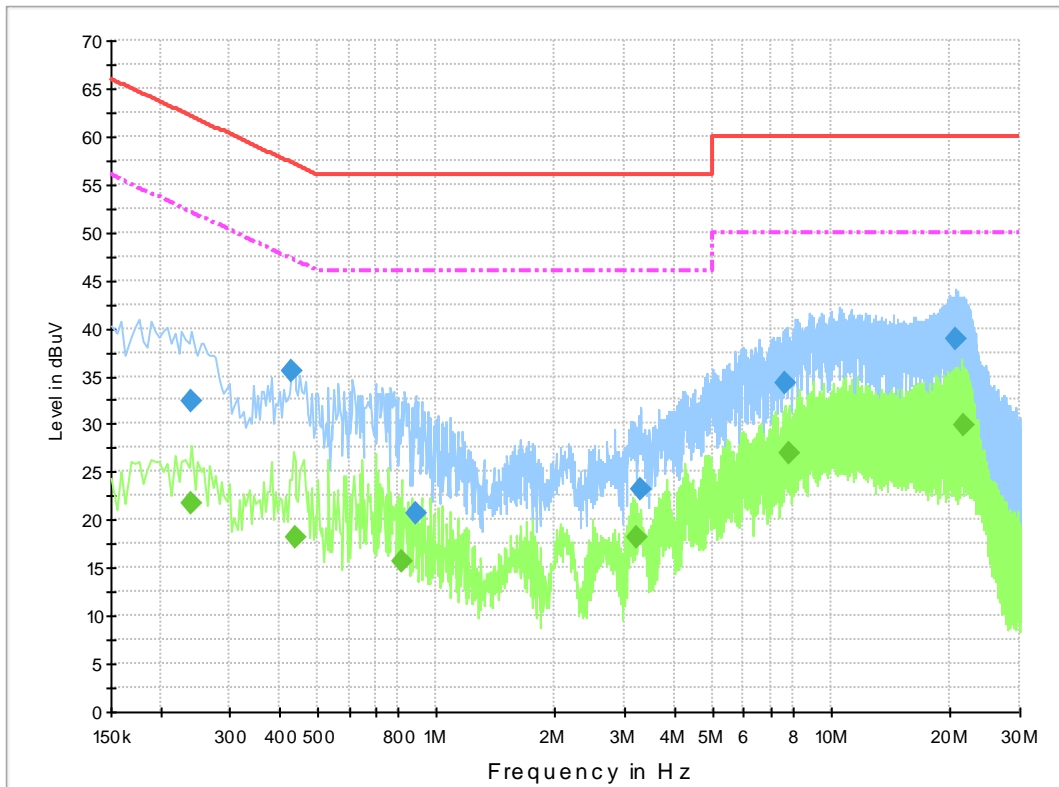
Fig.B.9.2 AC Powerline Conducted Emission-Idle
