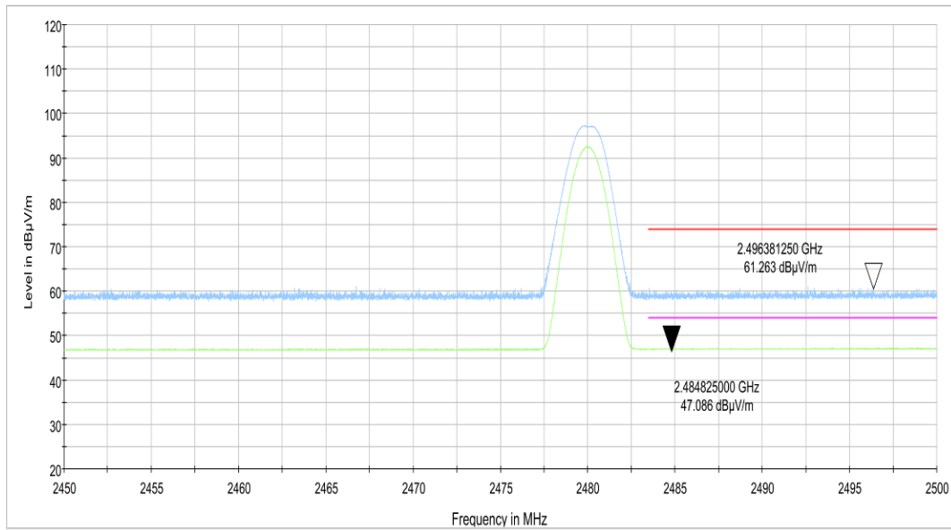
Fig.4. Frequency Band Edges: GFSK, 2480 MHz, 2.45 GHz - 2.50GHz
