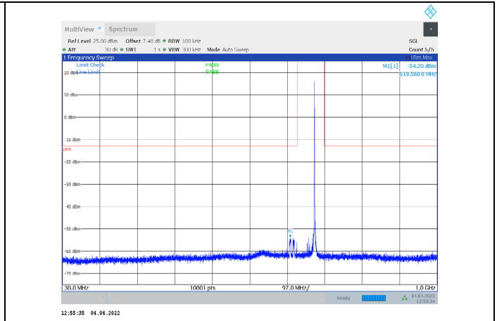
1-N71-PC3-15-20-L-2-CP-QPSK-Edge_1RB_Right-1@ 105-30-1000-Ant1--54.20--13-PASS
