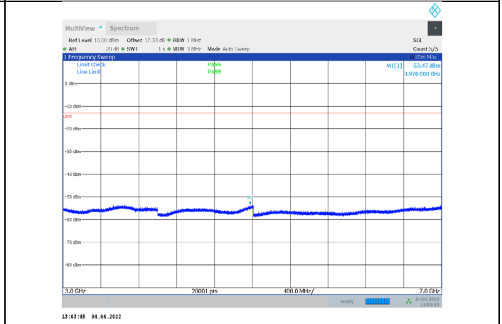
1-N71-PC3-15-20-H-2-CP-QPSK-Edge_1RB_Right-1@ 105-3000-7000-Ant1--53.47--13-PASS
