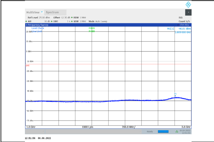
1-N71-PC3-15-15-H-2-CP-QPSK-Edge_1RB_Right-1@ 78-1000-3000-Ant1--46.01--13-PASS
