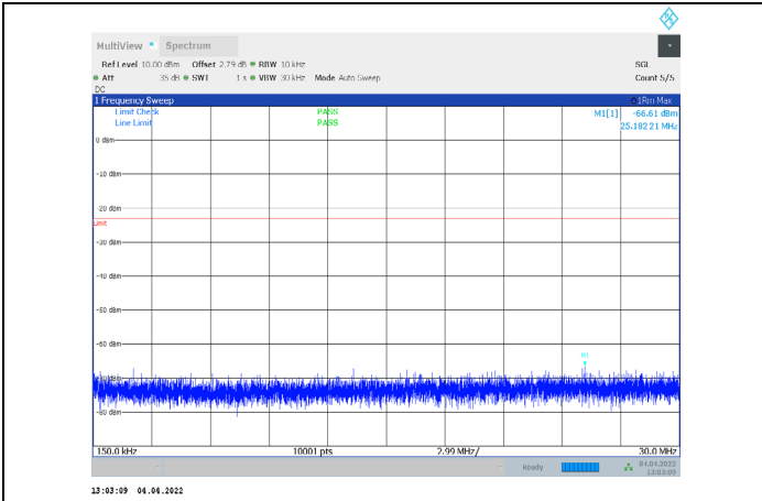
1-N71-PC3-15-20-H-2-CP-QPSK-Edge_1RB_Right-1@ 105-0.15-30-Ant1--66.61--23-PASS
