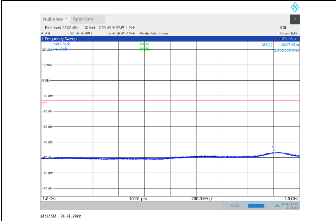
1-N71-PC3-15-20-H-2-CP-QPSK-Edge_1RB_Right-1@ 105-1000-3000-Ant1--46.27--13-PASS
