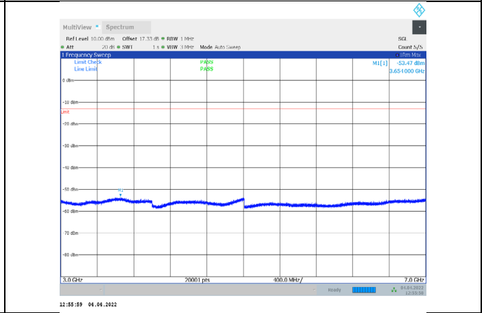
1-N71-PC3-15-20-L-2-CP-QPSK-Edge_1RB_Right-1@ 105-3000-7000-Ant1--53.47--13-PASS
