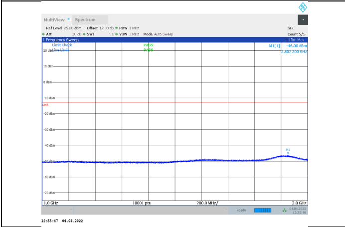
1-N71-PC3-15-20-L-2-CP-QPSK-Edge_1RB_Right-1@ 105-1000-3000-Ant1--46.00--13-PASS
