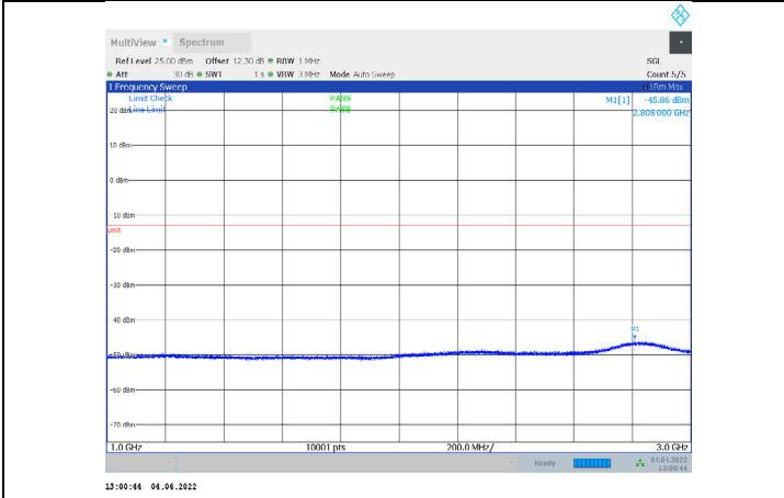
1-N71-PC3-15-20-M-3-CP-QPSK-Outer_Full-106@0-1000 -3000-Ant1--45.86--13-PASS
