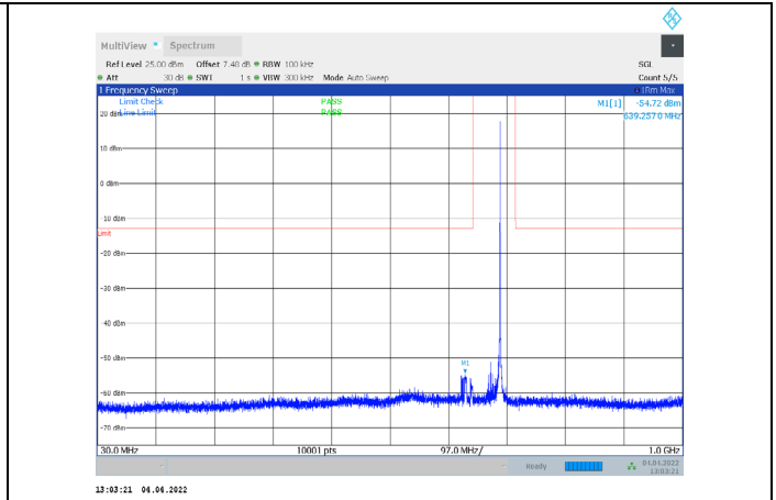
1-N71-PC3-15-20-H-2-CP-QPSK-Edge_1RB_Right-1@ 105-30-1000-Ant1--54.72--13-PASS
