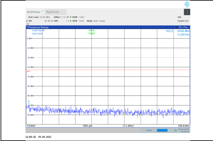
1-N71-PC3-15-20-L-3-CP-QPSK-Outer_Full-106@0-0.0 09-0.15-Ant1--69.06--33-PASS
