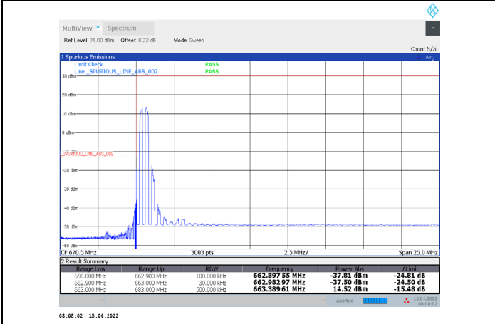
1-N71-PC3-15-20-L-25-CP-16QAM-Edge_1RB_Left-1 @0-Ant1-PASS-see graph
