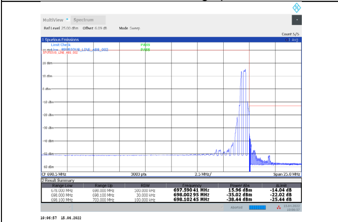
1-N71-PC3-15-20-H-3-DFT-PI/2BPSK-Edge_1RB_Right-1@105-Ant1-PASS-see graph
