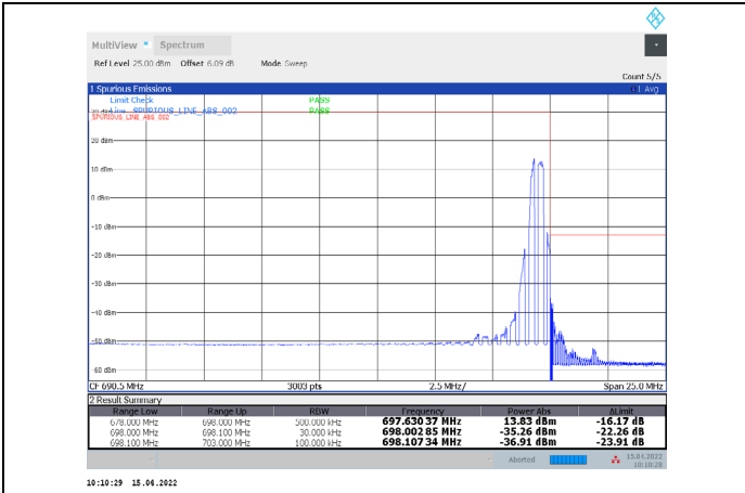
1-N71-PC3-15-20-H-14-DFT-64QAM-Edge_1RB_Right -1@105-Ant1-PASS-see graph
