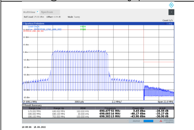
1-N71-PC3-15-20-H-8-DFT-QPSK-Inner_Full-50@25-Ant1-PASS-see graph
