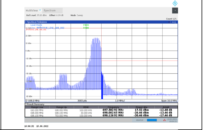
1-N71-PC3-15-5-H-34-CP-256QAM-Edge_1RB_Right-1 @24-Ant1-PASS-see graph
