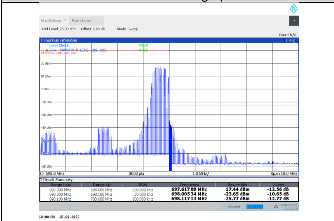
1-N71-PC3-15-5-H-22-CP-QPSK-Edge_1RB_Right-1@24-Ant1-PASS-see graph
