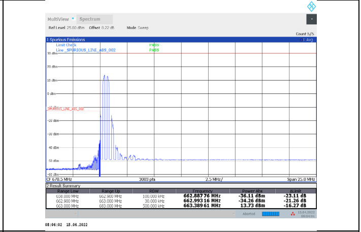
1-N71-PC3-15-20-L-13-DFT-64QAM-Edge_1RB_Left-1 @0-Ant1-PASS-see graph
