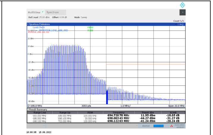
1-N71-PC3-15-5-H-20-DFT-256QAM-Inner_Full-12@6-Ant1-PASS-see graph
