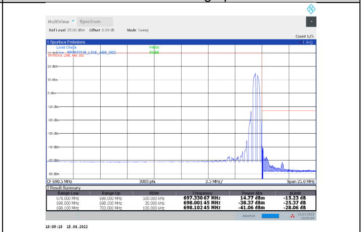
1-N71-PC3-15-20-H-10-DFT-16QAM-Edge_1RB_Right-1 @105-Ant1-PASS-see graph
