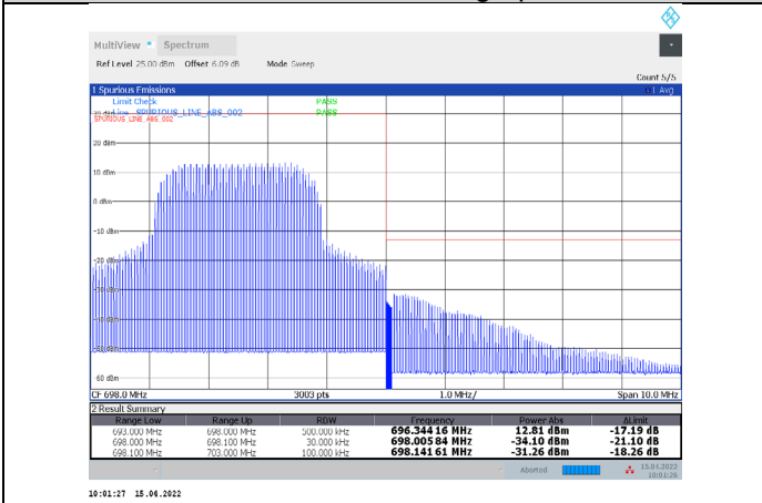
1-N71-PC3-15-5-H-24-CP-QPSK-Inner_Full-13@6-Ant1-PASS-see graph
