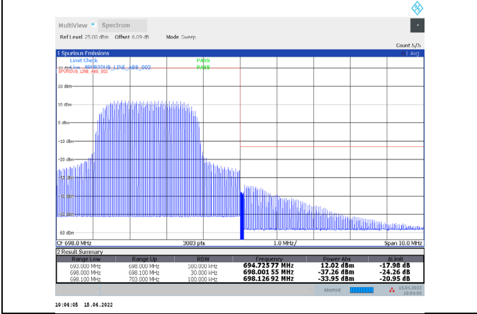
1-N71-PC3-15-5-H-32-CP-64QAM-Inner_Full-13@6-Ant t1-PASS-see graph
