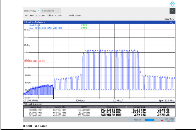
1-N71-PC3-15-20-L-12-DFT-16QAM-Inner_Full-50@25-Ant1-PASS-see graph
