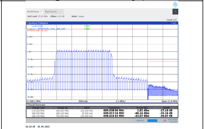
1-N71-PC3-15-20-H-12-DFT-16QAM-Inner_Full-50@25-Ant1-PASS-see graph
