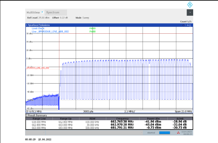
1-N71-PC3-15-20-L-27-CP-16QAM-Outer_Full-106@0-Ant1-PASS-see graph
