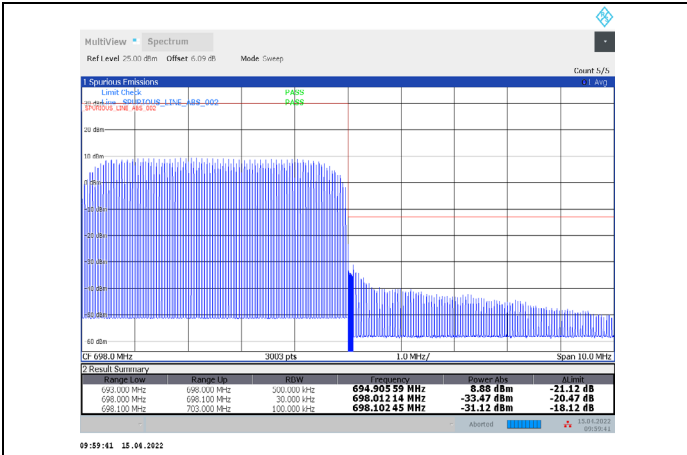
1-N71-PC3-15-5-H-19-DFT-256QAM-Outer_Full-25@0-Ant1-PASS-see graph
