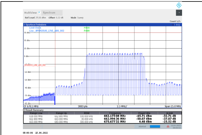
1-N71-PC3-15-20-L-1-DFT-PI/2BPSK-Inner_Full-50@25-Ant1-PASS-see graph
