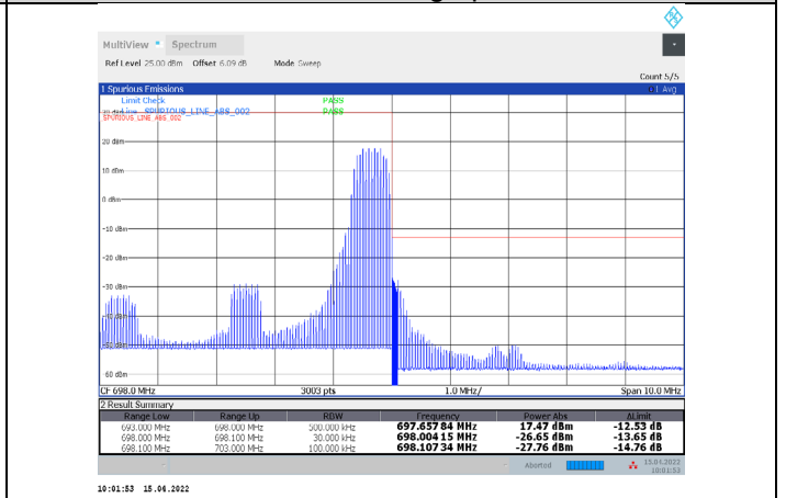
1-N71-PC3-15-5-H-26-CP-16QAM-Edge_1RB_Right-1@24-Ant1-PASS-see graph
