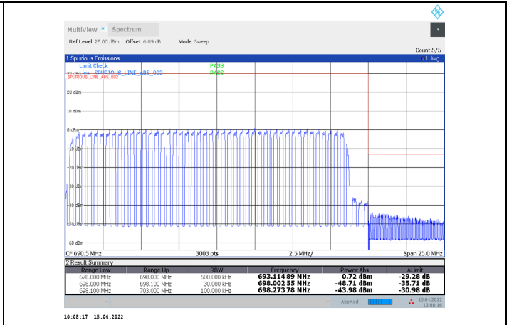
1-N71-PC3-15-20-H-7-DFT-QPSK-Outer_Full-100@0-Ant1-PASS-see graph
