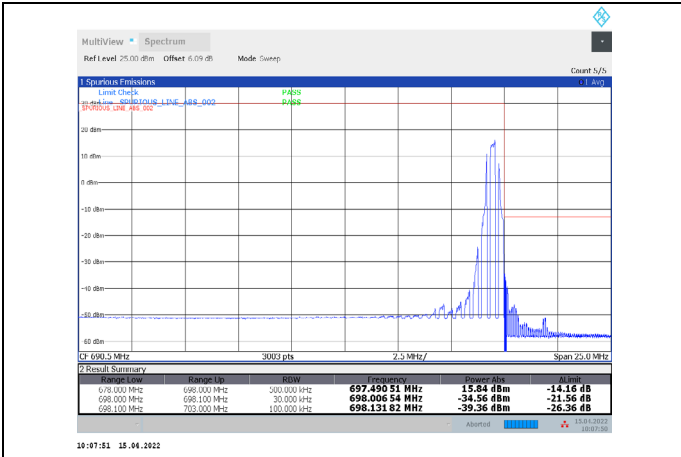
1-N71-PC3-15-20-H-6-DFT-QPSK-Edge_1RB_Right-1 @105-Ant1-PASS-see graph
