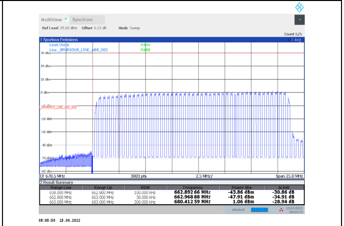
1-N71-PC3-15-20-L-19-DFT-256QAM-Outer_Full-100 @0-Ant1-PASS-see graph
