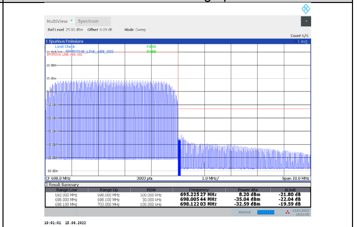
1-N71-PC3-15-5-H-23-CP-QPSK-Outer_Full-25@0-Ant1-PASS-see graph
