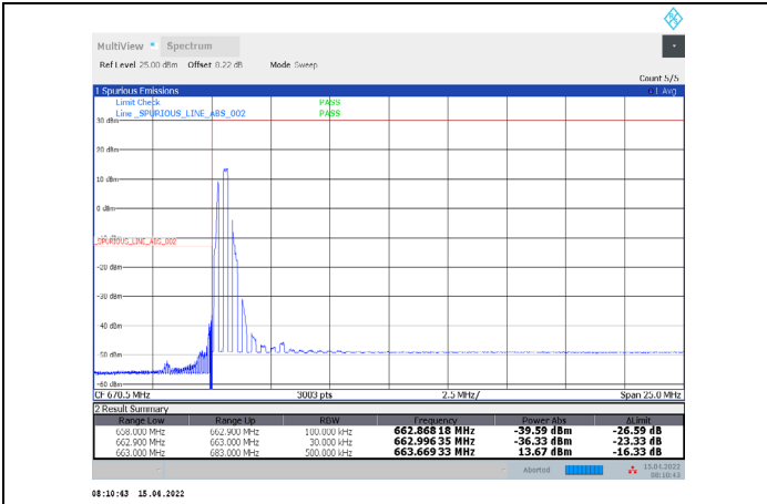
1-N71-PC3-15-20-L-33-CP-256QAM-Edge_1RB_Left-1@0-Ant1-PASS-see graph
