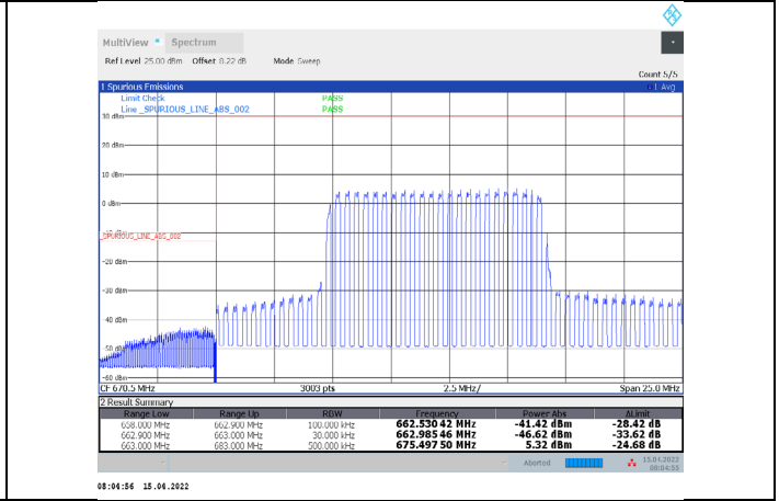
1-N71-PC3-15-20-L-16-DFT-64QAM-Inner_Full-50@25-Ant1-PASS-see graph
