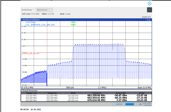
1-N71-PC3-15-20-L-28-CP-16QAM-Inner_Full-53@26-Ant1-PASS-see graph
