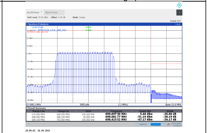
1-N71-PC3-15-20-H-1-DFT-PI/2BPSK-Inner_Full-50@25-Ant1-PASS-see graph
