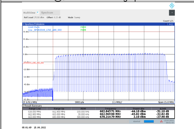
1-N71-PC3-15-20-L-7-DFT-QPSK-Outer_Full-100@0-Ant1-PASS-see graph
