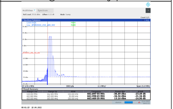
1-N71-PC3-15-20-L-5-DFT-QPSK-Edge_1RB_Left-1@0-Ant1-PASS-see graph
