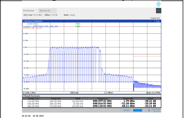
1-N71-PC3-15-20-H-20-DFT-256QAM-Inner_Full-50@25 -Ant1-PASS-see graph
