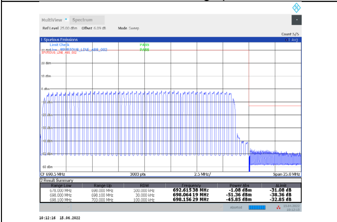
1-N71-PC3-15-20-H-19-DFT-256QAM-Outer_Full-100 @0-Ant1-PASS-see graph
