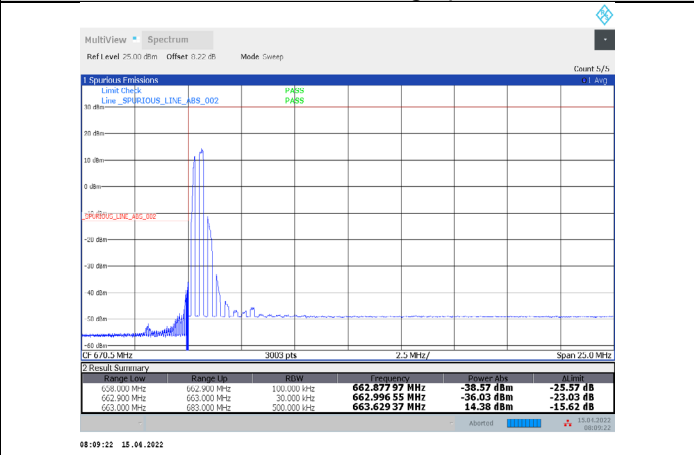
1-N71-PC3-15-20-L-29-CP-64QAM-Edge_1RB_Left-1 @0-Ant1-PASS-see graph
