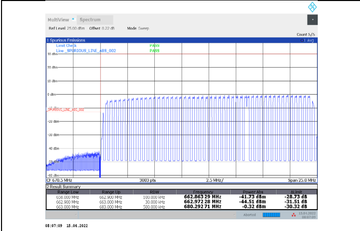
1-N71-PC3-15-20-L-23-CP-QPSK-Outer_Full-106@0-Ant1-PASS-see graph
