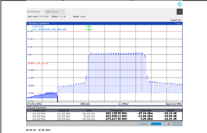
1-N71-PC3-15-20-L-20-DFT-256QAM-Inner_Full-50@25 -Ant1-PASS-see graph
