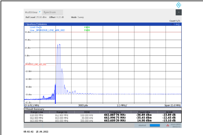
1-N71-PC3-15-20-L-9-DFT-16QAM-Edge_1RB_Left-1 @0-Ant1-PASS-see graph
