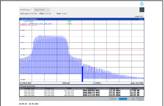
1-N71-PC3-15-5-H-36-CP-256QAM-Inner_Full-13@6-A nt1-PASS-see graph
