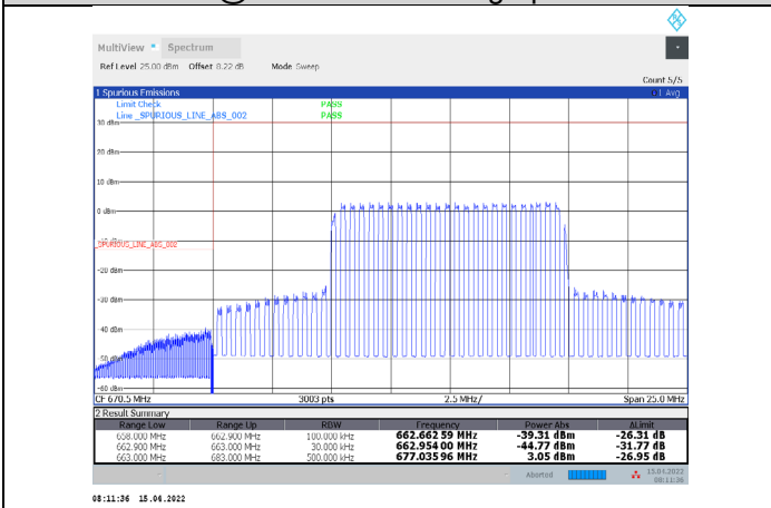
1-N71-PC3-15-20-L-36-CP-256QAM-Inner_Full-53@26-Ant1-PASS-see graph
