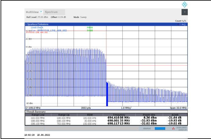
1-N71-PC3-15-5-H-27-CP-16QAM-Outer_Full-25@0-A nt1-PASS-see graph
