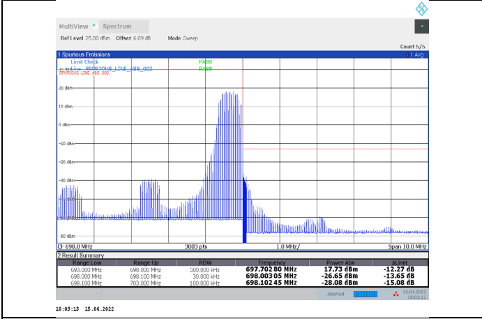
1-N71-PC3-15-5-H-30-CP-64QAM-Edge_1RB_Right-1 @24-Ant1-PASS-see graph
