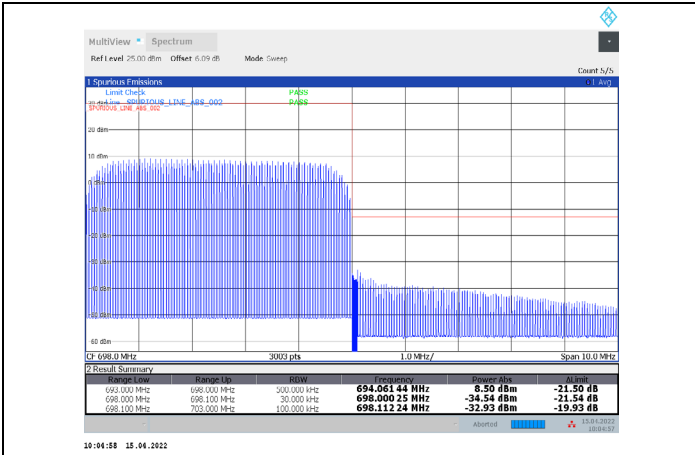
1-N71-PC3-15-5-H-35-CP-256QAM-Outer_Full-25@0-A nt1-PASS-see graph
