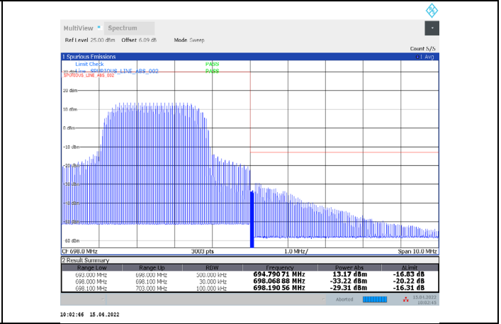
1-N71-PC3-15-5-H-28-CP-16QAM-Inner_Full-13@6-Ant 1-PASS-see graph
