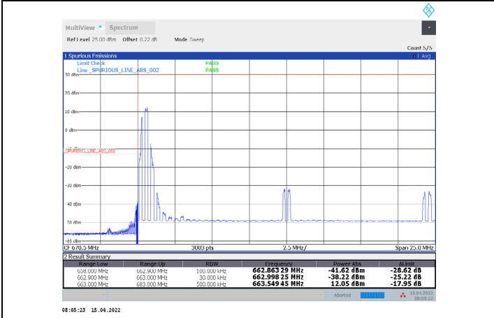
1-N71-PC3-15-20-L-17-DFT-256QAM-Edge_1RB_Left-1 @0-Ant1-PASS-see graph
