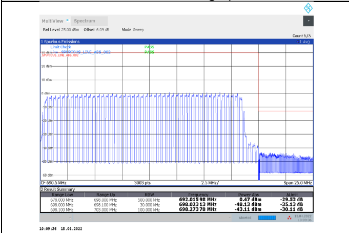
1-N71-PC3-15-20-H-11-DFT-16QAM-Outer_Full-100@0-Ant1-PASS-see graph
