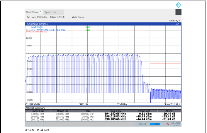
1-N71-PC3-15-20-H-15-DFT-64QAM-Outer_Full-100@0 -Ant1-PASS-see graph
