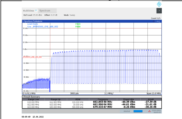
1-N71-PC3-15-20-L-31-CP-64QAM-Outer_Full-106@0-Ant1-PASS-see graph
