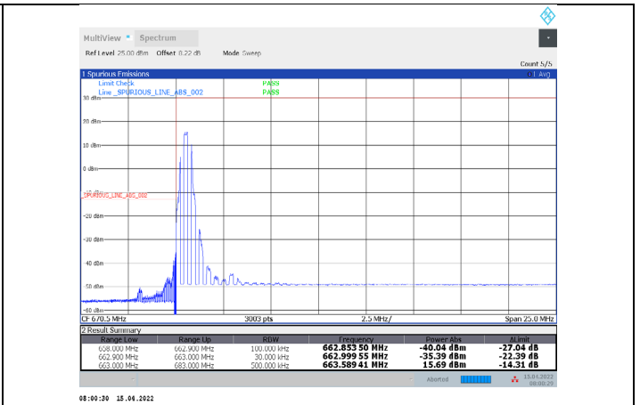
1-N71-PC3-15-20-L-2-DFT-PI/2BPSK-Edge_1RB_Left-1@0-Ant1-PASS-see graph
