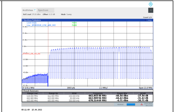
1-N71-PC3-15-20-L-35-CP-256QAM-Outer_Full-106@0-Ant1-PASS-see graph
