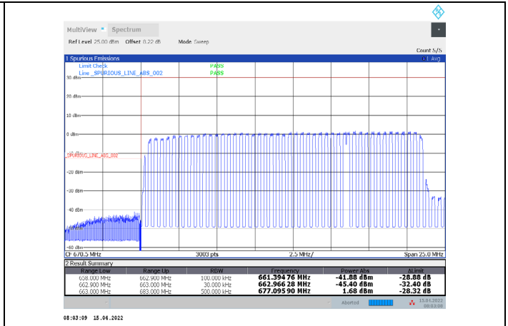
1-N71-PC3-15-20-L-11-DFT-16QAM-Outer_Full-100@0-Ant1-PASS-see graph
