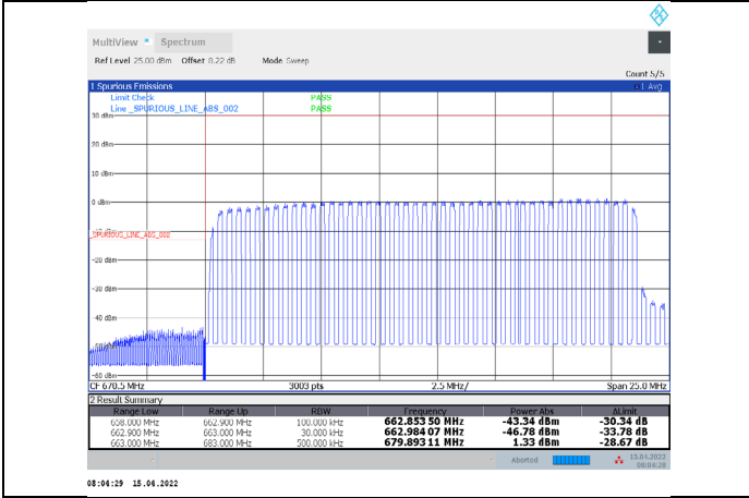
1-N71-PC3-15-20-L-15-DFT-64QAM-Outer_Full-100@0-Ant1-PASS-see graph
