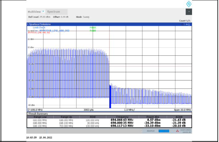
1-N71-PC3-15-5-H-31-CP-64QAM-Outer_Full-25@0-Ant 1-PASS-see graph
