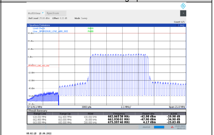
1-N71-PC3-15-20-L-8-DFT-QPSK-Inner_Full-50@25-Ant1-PASS-see graph
