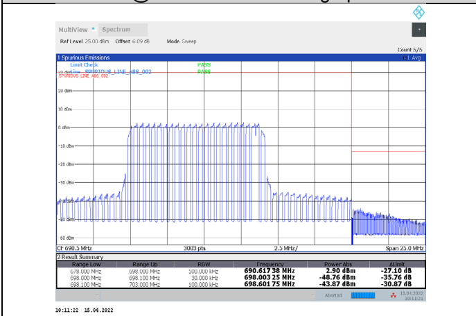
1-N71-PC3-15-20-H-16-DFT-64QAM-Inner_Full-50@25 -Ant1-PASS-see graph
