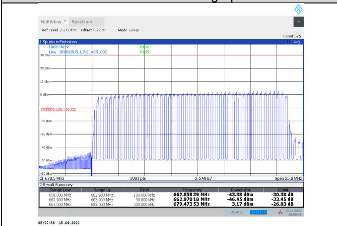
1-N71-PC3-15-20-L-4-DFT-PI/2BPSK-Outer_Full-100@0-Ant1-PASS-see graph
