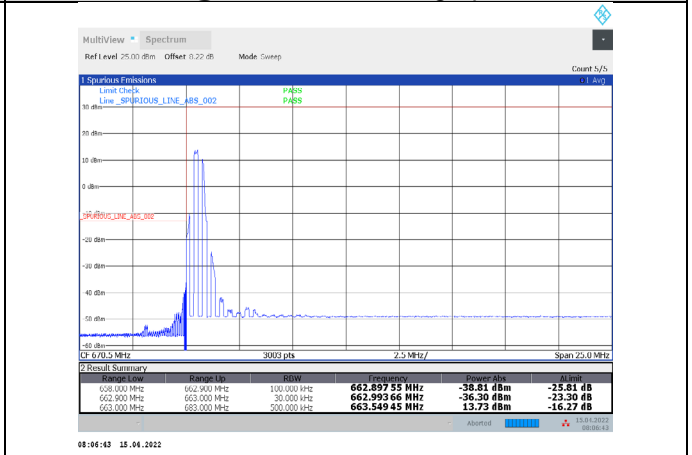
1-N71-PC3-15-20-L-21-CP-QPSK-Edge_1RB_Left-1@ 0-Ant1-PASS-see graph
