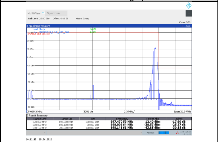
1-N71-PC3-15-20-H-18-DFT-256QAM-Edge_1RB_Right -1@105-Ant1-PASS-see graph
