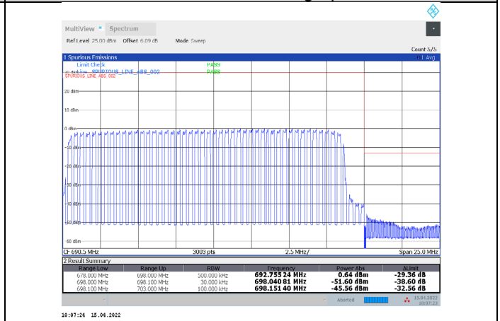
1-N71-PC3-15-20-H-4-DFT-PI/2BPSK-Outer_Full-100@0-Ant1-PASS-see graph
