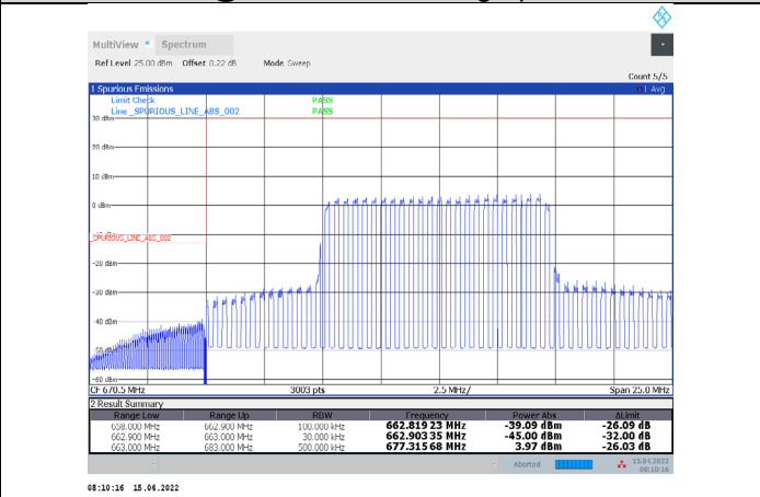
1-N71-PC3-15-20-L-32-CP-64QAM-Inner_Full-53@26-Ant1-PASS-see graph
