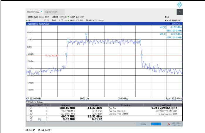
1-N71-PC3-15-10-H-3-CP-64QAM-Outer_Full-52@0-Ant1 1-9.212-9.620-≤10-PASS
