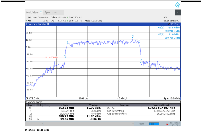
1-N71-PC3-15-20-L-3-CP-64QAM-Outer_Full-106@0-Ant t1-18.611-19.560-≤20-PASS
