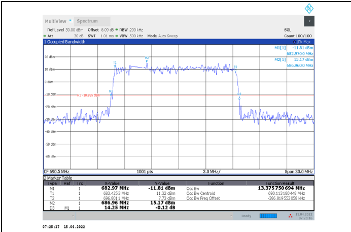
1-N71-PC3-15-15-H-7-DFT-16QAM-Outer_Full-75@0-A Ant1-13.376-14.250-≤15-PASS
