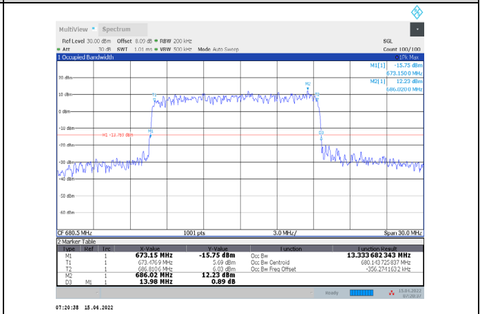
1-N71-PC3-15-15-M-1-CP-QPSK-Outer_Full-75@0-Ant 1-13.334-13.980-≤15-PASS
