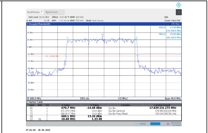
1-N71-PC3-15-20-M-5-DFT-PI/2BPSK-Outer_Full-100@0-Ant1-17.839-18.480-≤20-PASS
