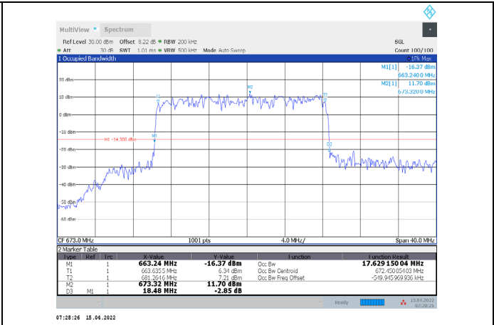
1-N71-PC3-15-20-L-8-DFT-64QAM-Outer_Full-100@0-Ant1-17.629-18.480-≤20-PASS
