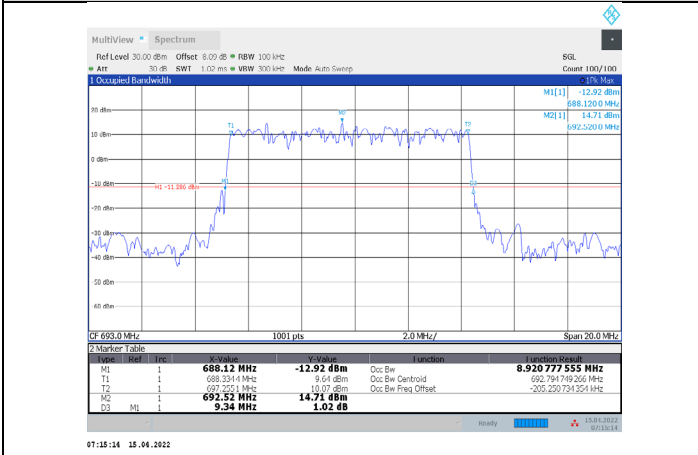
1-N71-PC3-15-10-H-5-DFT-PI/2BPSK-Outer_Full-50@0-Ant1 -8.921-9.340-≤10-PASS
