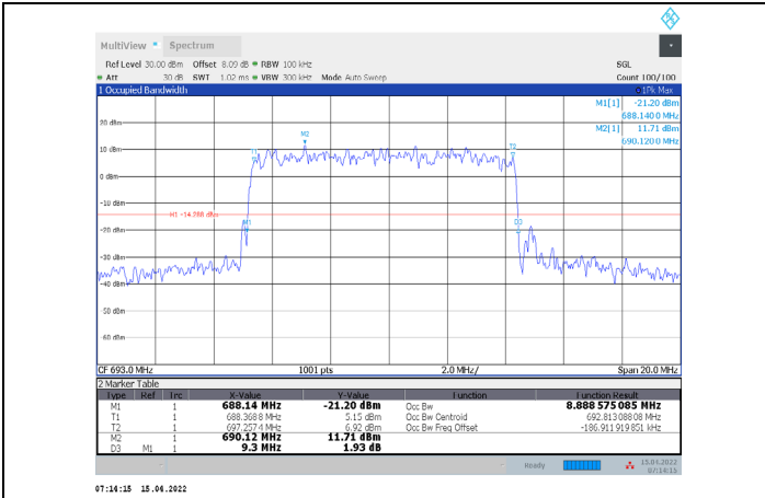
1-N71-PC3-15-10-H-1-CP-QPSK-Outer_Full-50@0-Ant1 -8.889-9.300-≤10-PASS
