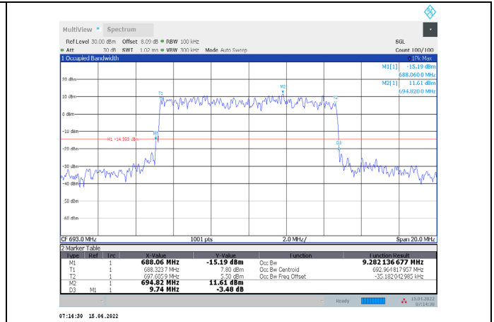
1-N71-PC3-15-10-H-2-CP-16QAM-Outer_Full-52@0-Ant1 -9.282-9.740-≤10-PASS
