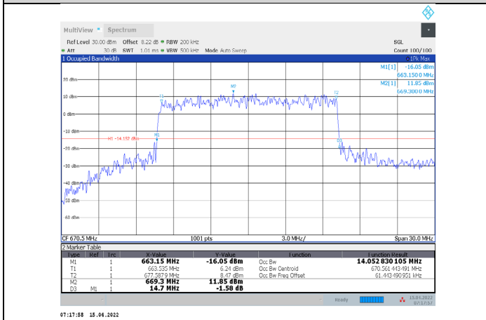
1-N71-PC3-15-15-L-3-CP-64QAM-Outer_Full-79@0-Ant 1-14.053-14.700-≤15-PASS
