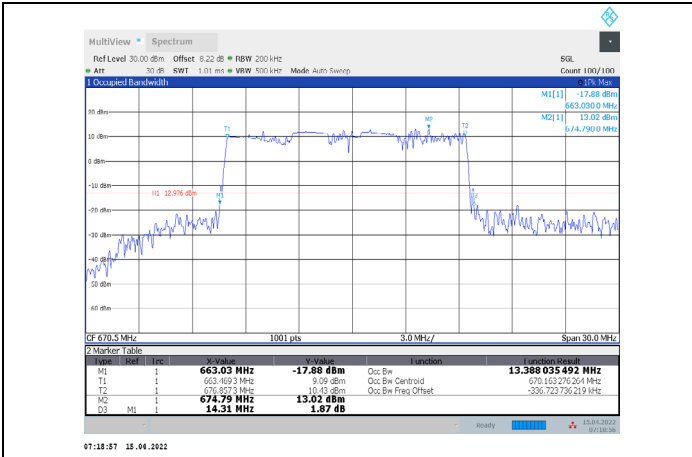
1-N71-PC3-15-15-L-7-DFT-16QAM-Outer_Full-75@0-A nt1-13.388-14.310-≤15-PASS
