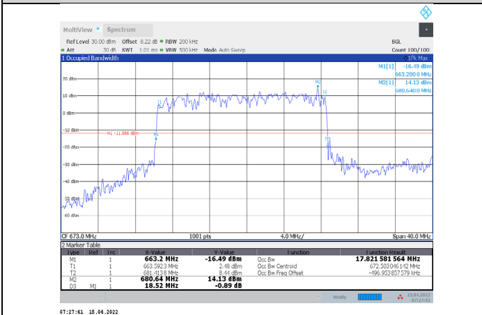
1-N71-PC3-15-20-L-5-DFT-PI/2BPSK-Outer_Full-100@0-Ant1-17.822-18.520-≤20-PASS
