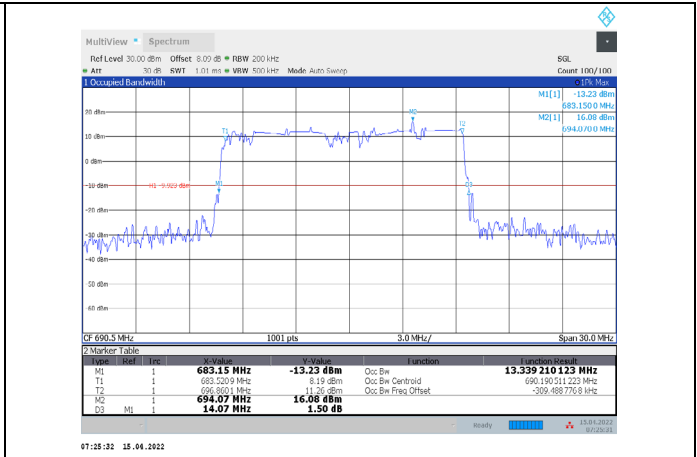
1-N71-PC3-15-15-H-8-DFT-64QAM-Outer_Full-75@0- Ant1-13.339-14.070-≤15-PASS
