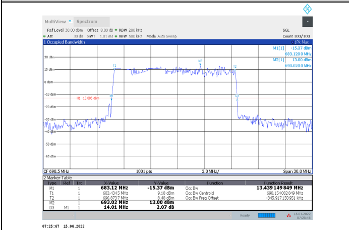
1-N71-PC3-15-15-H-9-DFT-256QAM-Outer_Full-75@0- Ant1-13.439-14.010-≤15-PASS
