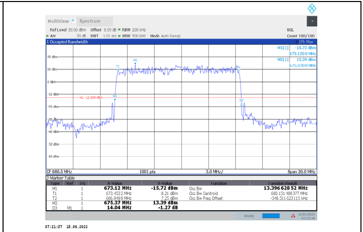
1-N71-PC3-15-15-M-5-DFT-PI/2BPSK-Outer_Full-75@0-Ant1-13.397-14.040≤15-PASS
