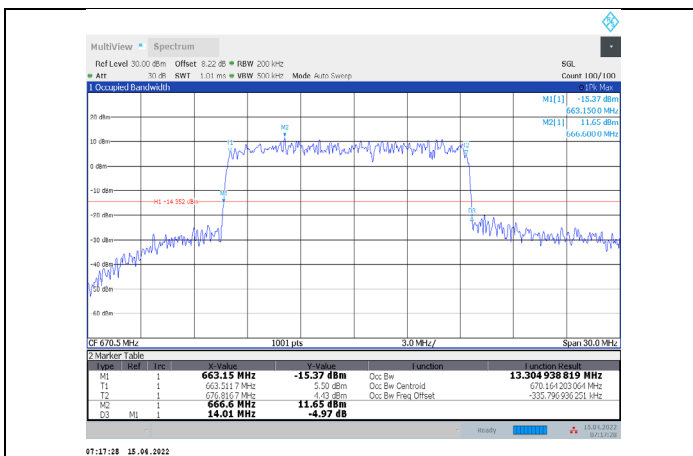
1-N71-PC3-15-15-L-1-CP-QPSK-Outer_Full-75@0-Ant1 -13.305-14.010-≤15-PASS
