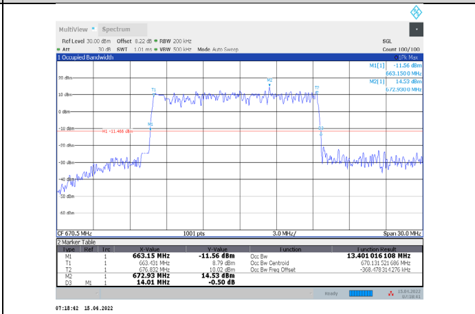
1-N71-PC3-15-15-L-6-DFT-QPSK-Outer_Full-75@0-An t1-13.401-14.010-≤15-PASS
