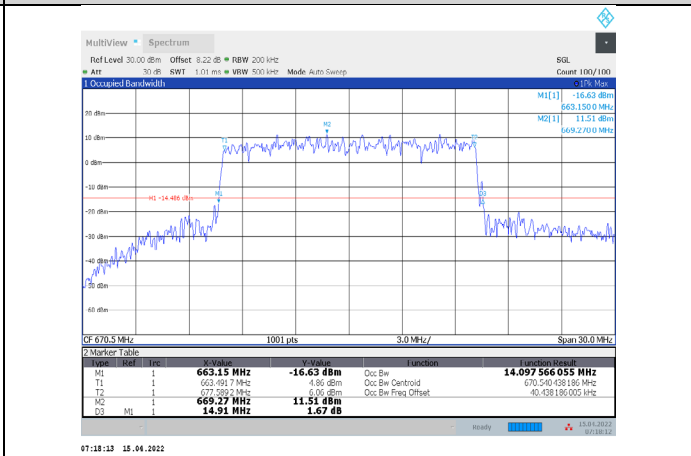
1-N71-PC3-15-15-L-4-CP-256QAM-Outer_Full-79@0-A nt1-14.098-14.910-≤15-PASS
