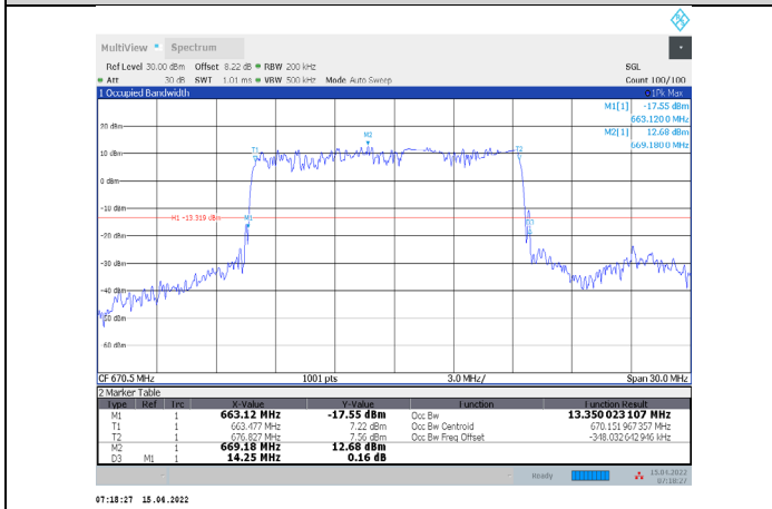
1-N71-PC3-15-15-L-5-DFT-PI/2BPSK-Outer_Full-75@0- Ant1-13.35-14.250-≤15-PASS
