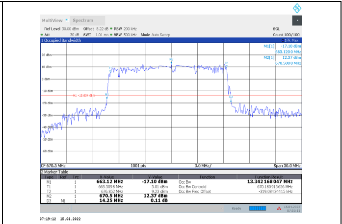
1-N71-PC3-15-15-L-8-DFT-64QAM-Outer_Full-75@0-A nt1-13.342-14.250-≤15-PASS
