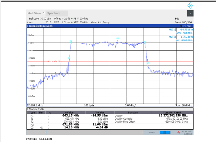
1-N71-PC3-15-15-L-9-DFT-256QAM-Outer_Full-75@0-A Ant1-13.372-14.160-≤15-PASS
