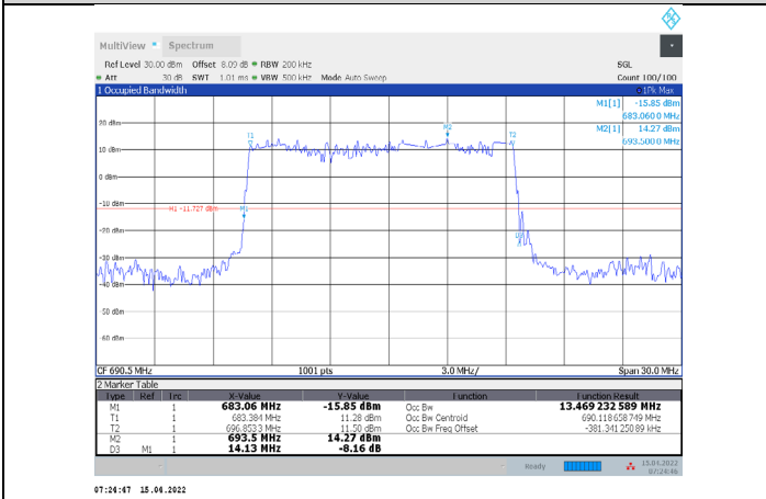
1-N71-PC3-15-15-H-5-DFT-PI/2BPSK-Outer_Full-75@0-Ant1 -13.469-14.130≤15-PASS
