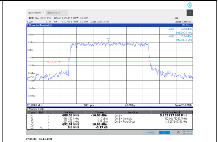
1-N71-PC3-15-10-H-4-CP-256QAM-Outer_Full-52@0-Ant1 -9.253-9.800-≤10-PASS
