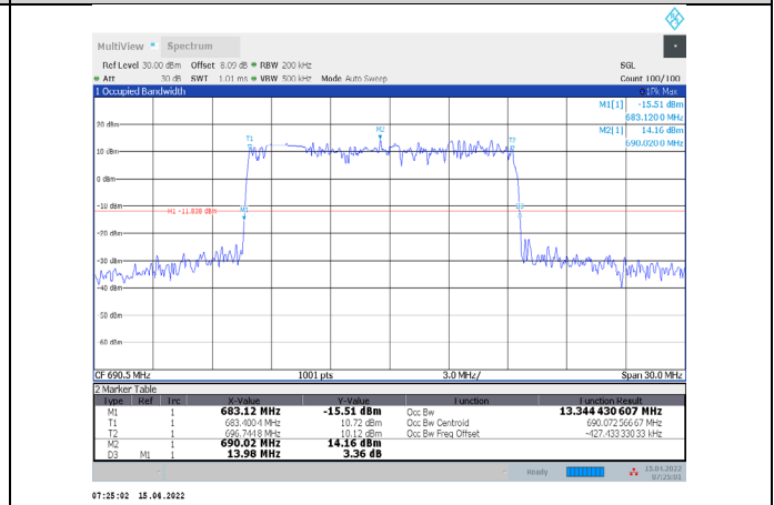
1-N71-PC3-15-15-H-6-DFT-QPSK-Outer_Full-75@0-Ant1 -13.344-13.980≤15-PASS
