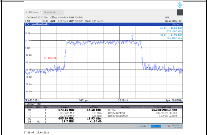
1-N71-PC3-15-15-M-3-CP-64QAM-Outer_Full-79@0-A nt1-14.059-14.700-≤15-PASS
