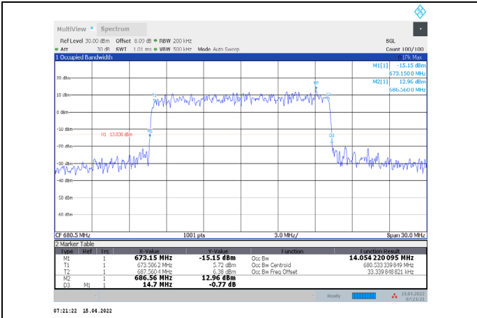
1-N71-PC3-15-15-M-4-CP-256QAM-Outer_Full-79@0-Ant1-14.054-14.700≤15-PASS
