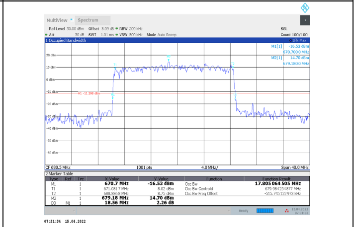
1-N71-PC3-15-20-M-7-DFT-16QAM-Outer_Full-100@0-Ant1-17.805-18.560-≤20-PASS
