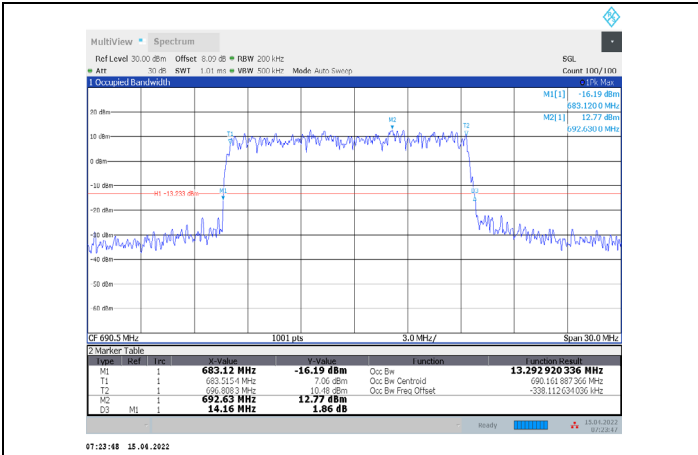
1-N71-PC3-15-15-H-1-CP-QPSK-Outer_Full-75@0-Ant1 -13.293-14.160≤15-PASS
