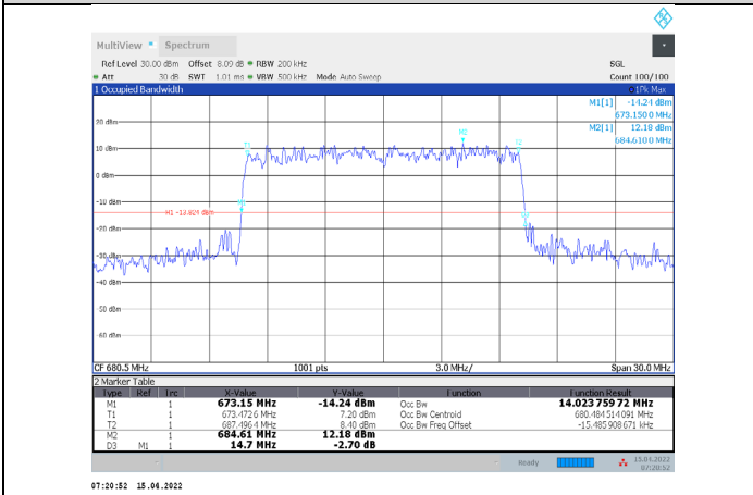
1-N71-PC3-15-15-M-2-CP-16QAM-Outer_Full-79@0-Ant t1-14.024-14.700-≤15-PASS
