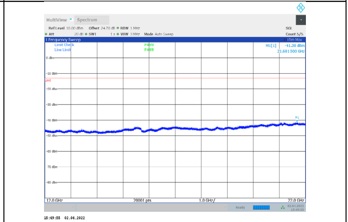
1-N66-PC3-15-5-H-2-CP-QPSK-Edge_1RB_Right-1@2 4-12000-22000-Ant1--41.38--13-PASS
