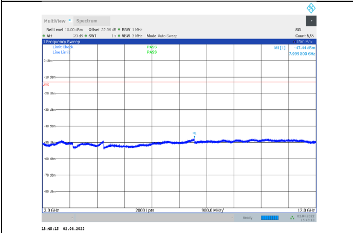
1-N66-PC3-15-5-M-2-CP-QPSK-Edge_1RB_Right-1@2 4-3000-12000-Ant1--47.44--13-PASS
