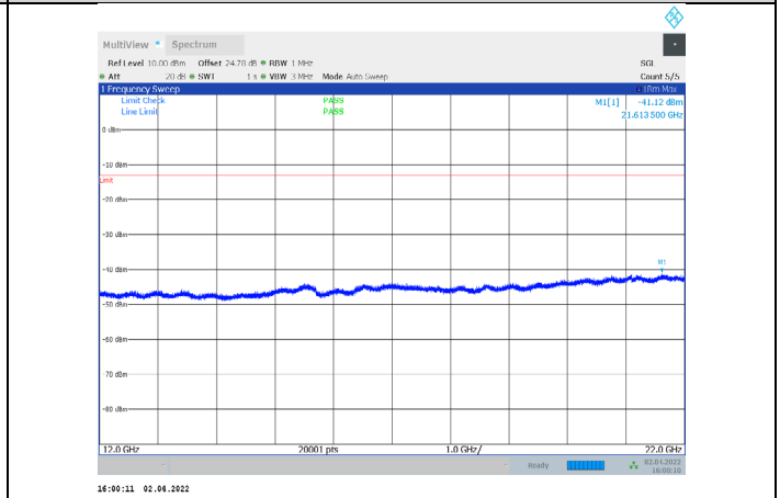
1-N66-PC3-15-15-M-3-CP-QPSK-Outer_Full-79@0-120 00-22000-Ant1--41.12--13-PASS
