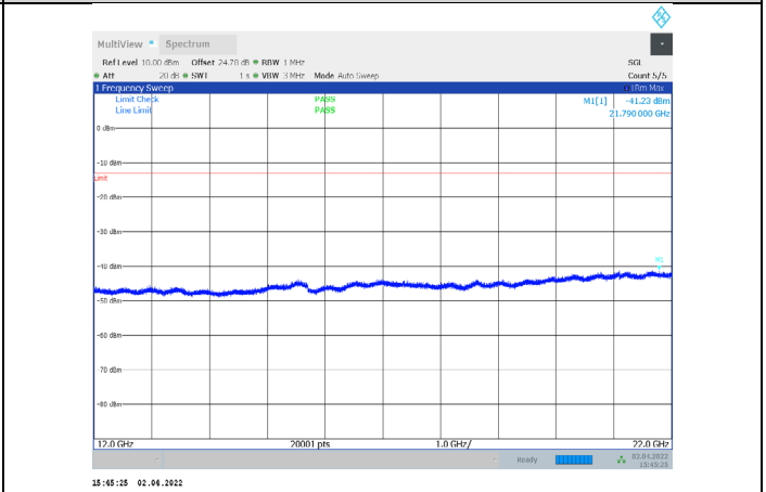
1-N66-PC3-15-5-M-2-CP-QPSK-Edge_1RB_Right-1@2 4-12000-22000-Ant1--41.23--13-PASS
