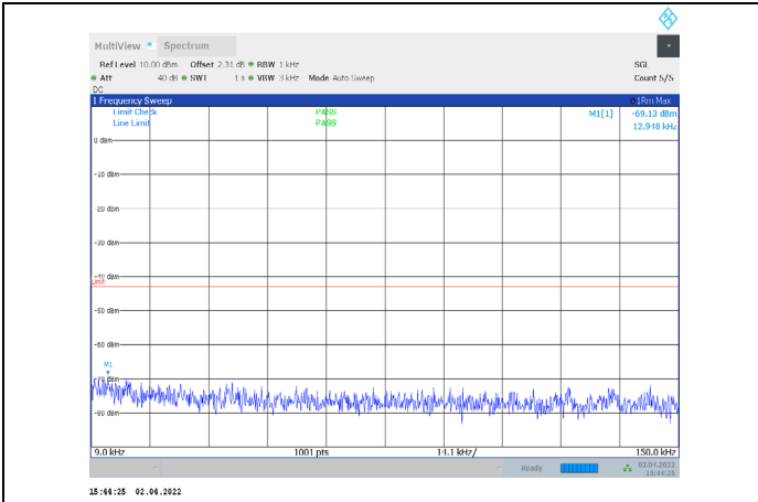
1-N66-PC3-15-5-M-2-CP-QPSK-Edge_1RB_Right-1@2 4-0.009-0.15-Ant1--69.13--43-PASS
