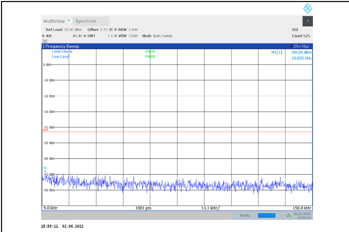
1-N66-PC3-15-15-M-3-CP-QPSK-Outer_Full-79@0-0.0 09-0.15-Ant1--69.26--43-PASS
