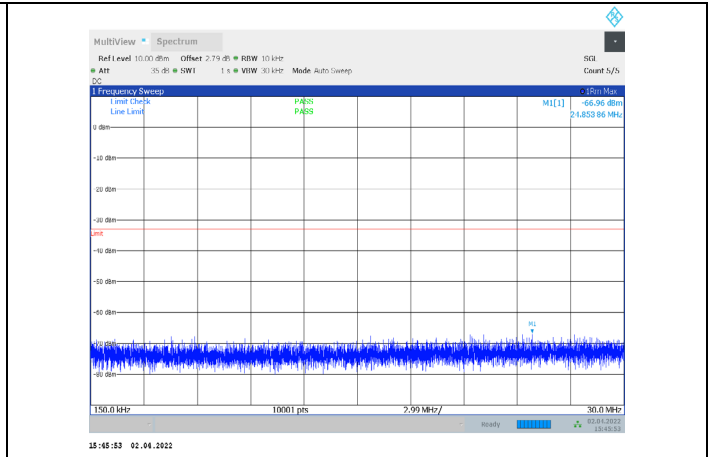
1-N66-PC3-15-5-M-3-CP-QPSK-Outer_Full-25@0-0.15- 30-Ant1--66.96--33-PASS
