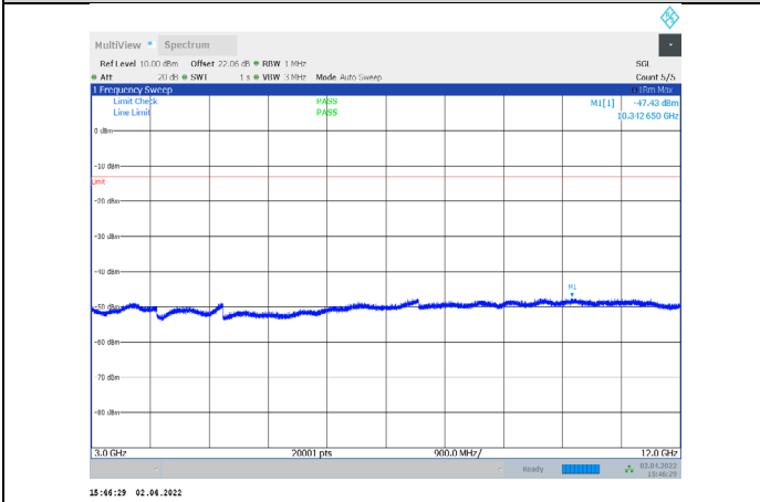
1-N66-PC3-15-5-M-3-CP-QPSK-Outer_Full-25@0-300 0-12000-Ant1--47.43--13-PASS
