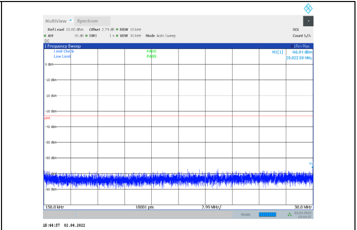
1-N66-PC3-15-5-M-2-CP-QPSK-Edge_1RB_Right-1@2 4-0.15-30-Ant1--66.94--33-PASS
