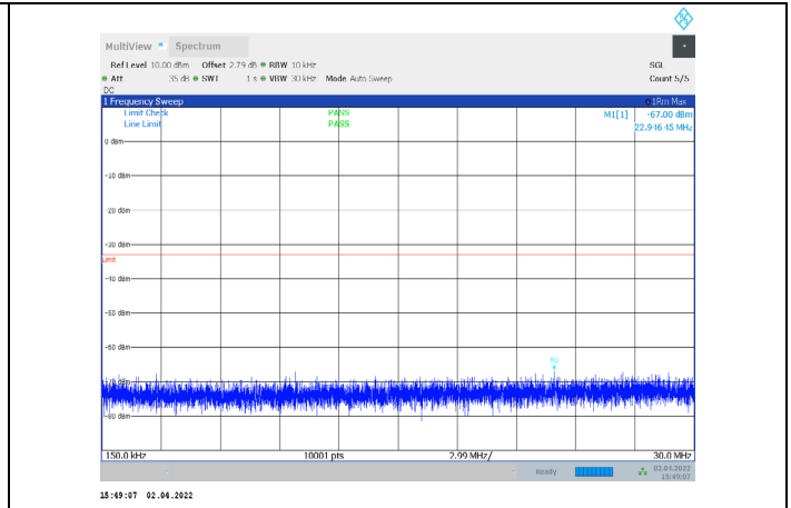
1-N66-PC3-15-5-H-2-CP-QPSK-Edge_1RB_Right-1@2 4-0.15-30-Ant1--67.00--33-PASS
