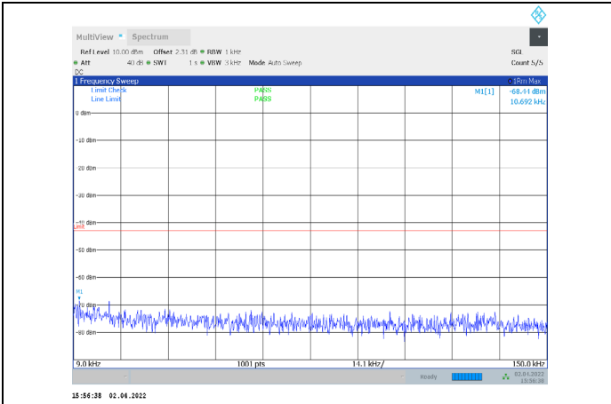
1-N66-PC3-15-15-M-1-CP-QPSK-Edge_1RB_Left-1@0 -0.009-0.15-Ant1--68.44--43-PASS
