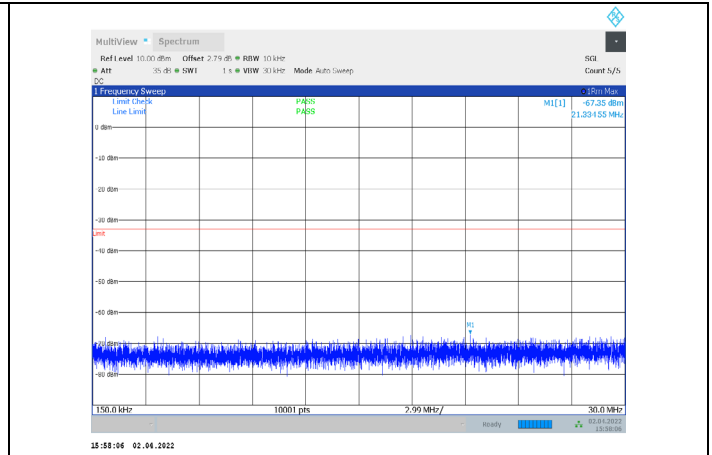
1-N66-PC3-15-15-M-2-CP-QPSK-Edge_1RB_Right-1@ 78-0.15-30-Ant1--67.35--33-PASS
