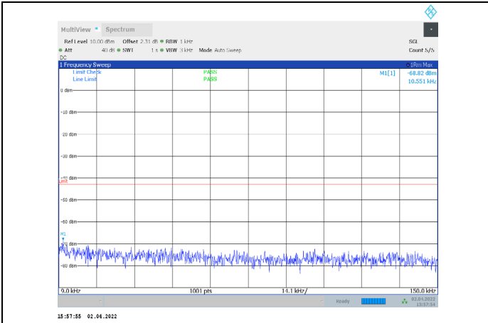
1-N66-PC3-15-15-M-2-CP-QPSK-Edge_1RB_Right-1@ 78-0.009-0.15-Ant1--68.82--43-PASS
