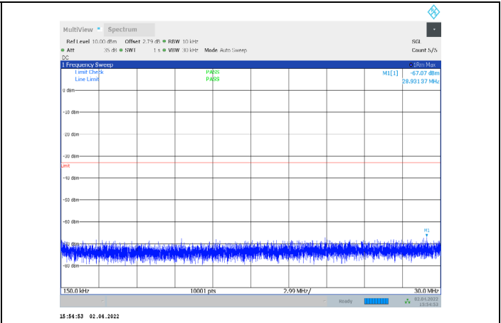
1-N66-PC3-15-15-L-3-CP-QPSK-Outer_Full-79@0-0.15- 30-Ant1--67.07--33-PASS
