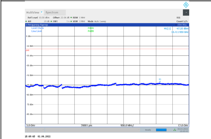
1-N66-PC3-15-5-H-2-CP-QPSK-Edge_1RB_Right-1@2 4-3000-12000-Ant1--47.35--13-PASS
