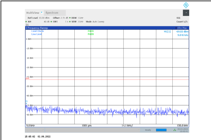
1-N66-PC3-15-5-M-3-CP-QPSK-Outer_Full-25@0-0.00 9-0.15-Ant1--69.03--43-PASS
