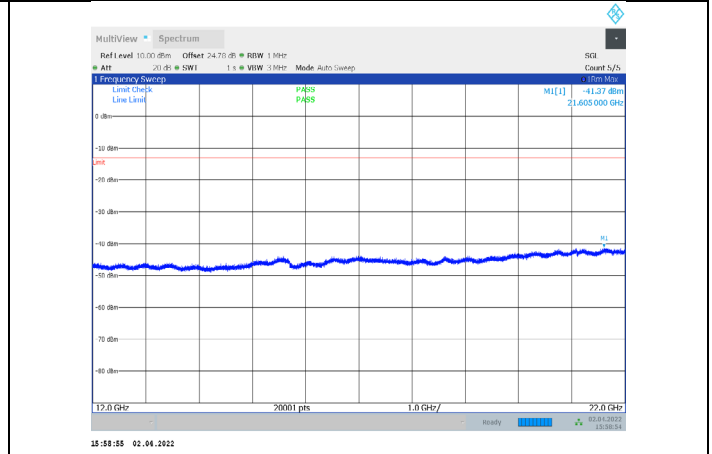
1-N66-PC3-15-15-M-2-CP-QPSK-Edge_1RB_Right-1@ 78-12000-22000-Ant1--41.37--13-PASS
