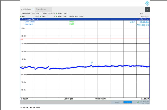
1-N66-PC3-15-15-L-3-CP-QPSK-Outer_Full-79@0-300- 0-12000-Ant1--47.36--13-PASS
