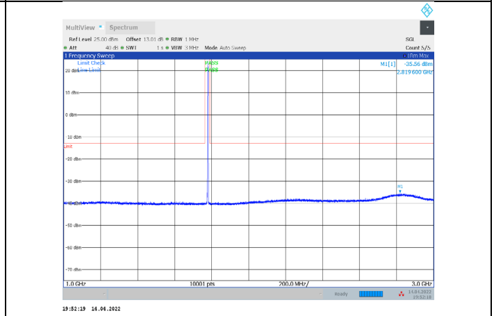
1-N66-PC3-15-5-H-2-CP-QPSK-Edge_1RB_Right-1@2 4-1000-3000-Ant1--35.56--13-PASS
