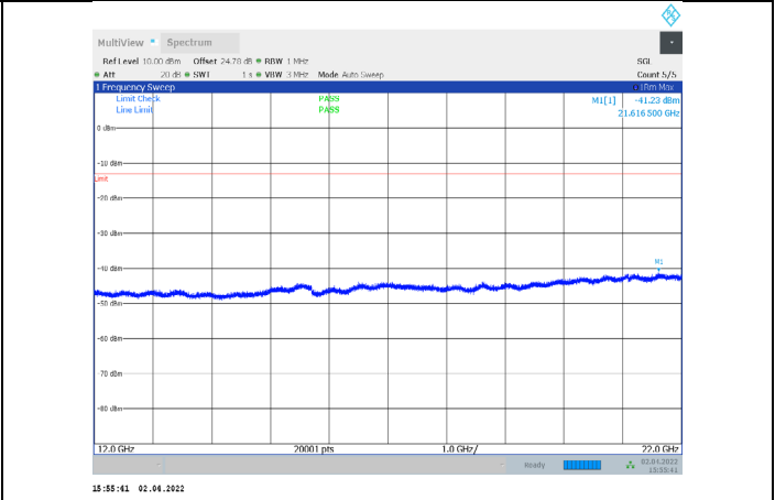
1-N66-PC3-15-15-L-3-CP-QPSK-Outer_Full-79@0-1200- 0-22000-Ant1--41.23--13-PASS
