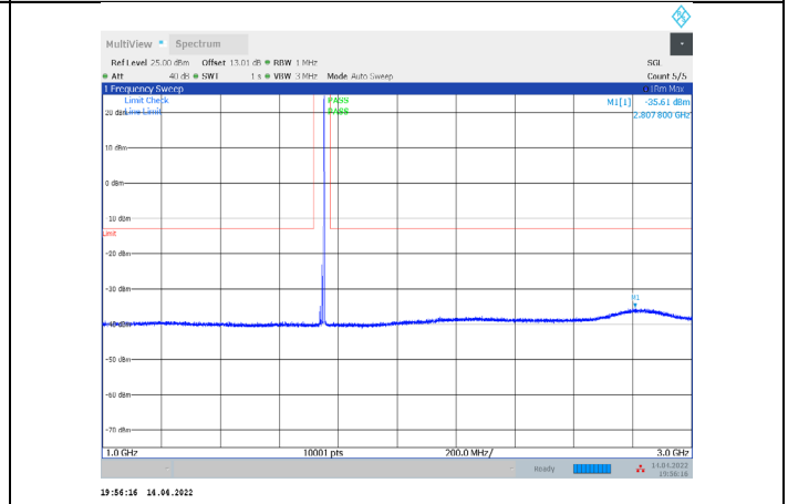
1-N66-PC3-15-15-M-2-CP-QPSK-Edge_1RB_Right-1@ 78-1000-3000-Ant1--35.61--13-PASS
