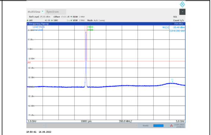
1-N66-PC3-15-5-M-3-CP-QPSK-Outer_Full-25@0-1000- 3000-Ant1--35.40--13-PASS
