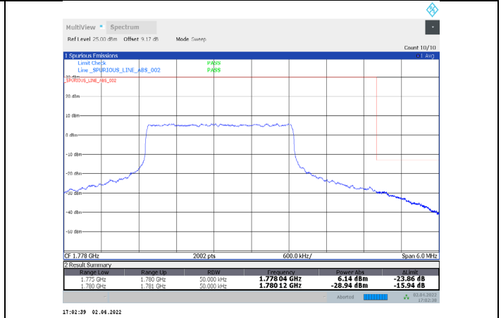
1-N66-PC3-15-5-H-28-CP-16QAM-Inner_Full-13@6-Ant1-seegraph-PASS-see graph
