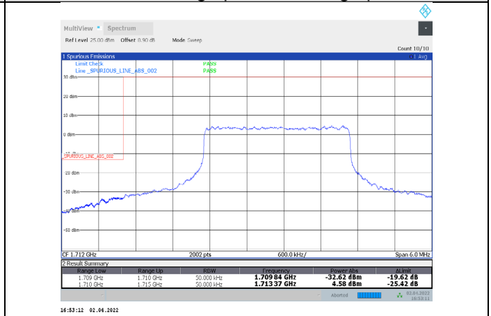
1-N66-PC3-15-5-L-32-CP-64QAM-Inner_Full-13@6-Ant1-seegraph-PASS-see graph
