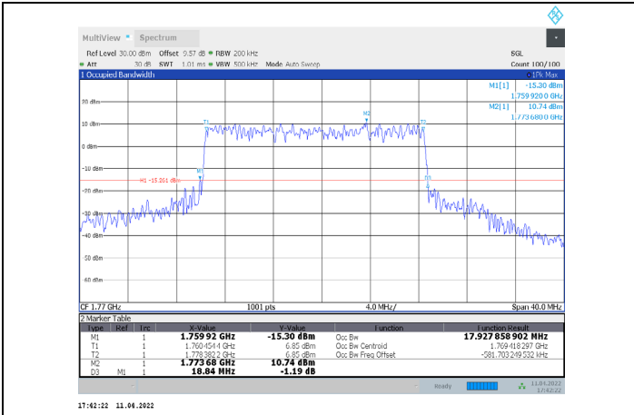
1-N66-PC3-15-20-H-1-CP-QPSK-Outer_Full-100@0-Ant 1-17.928-18.840-≤20-PASS
