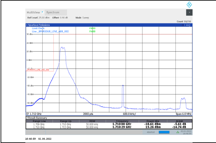
1-N66-PC3-15-5-L-9-DFT-16QAM-Edge_1RB_Left-1@0-Ant1-seegraph-PASS-see graph
