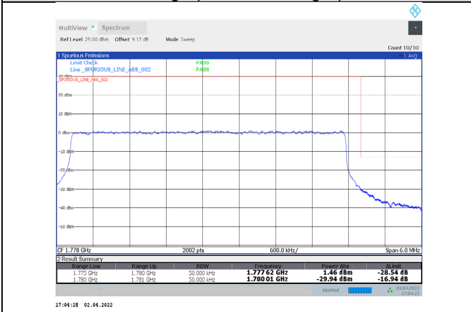
1-N66-PC3-15-5-H-35-CP-256QAM-Outer_Full-25@0-Ant1-seegraph-PASS-see graph
