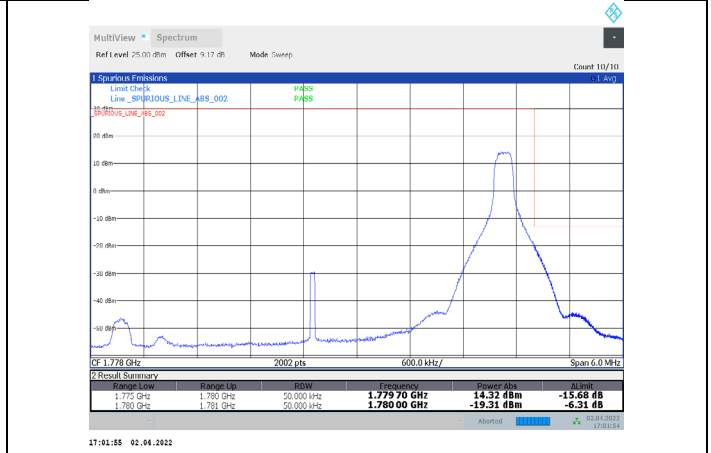
1-N66-PC3-15-5-H-26-CP-16QAM-Edge_1RB_Right-1@24-Ant1-seegraph-PASS-see graph
