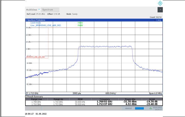
1-N66-PC3-15-5-L-36-CP-256QAM-Inner_Full-13@6-Ant1-seegraph-PASS-see graph
