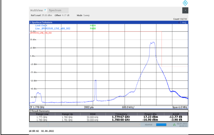
1-N66-PC3-15-5-H-3-DFT-PI/2BPSK-Edge_1RB_Right-1@24-Ant1-seegraph-PASS-see graph
