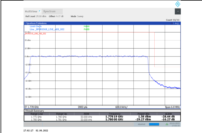
1-N66-PC3-15-5-H-27-CP-16QAM-Outer_Full-25@0-Ant1-seegraph-PASS-see graph
