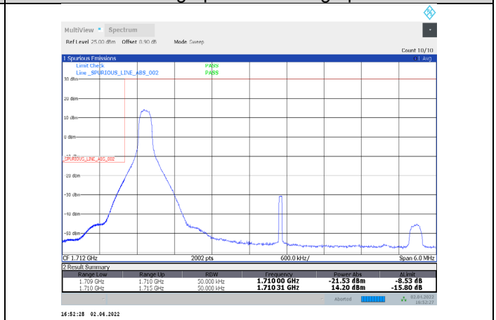
1-N66-PC3-15-5-L-29-CP-64QAM-Edge_1RB_Left-1@0-Ant1-seegraph-PASS-see graph
