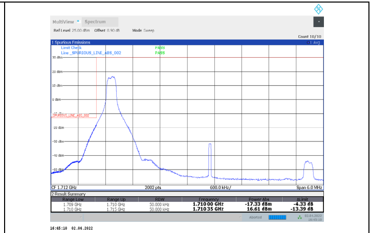
1-N66-PC3-15-5-L-2-DFT-PI/2BPSK-Edge_1RB_Left-1@0-Ant1-seegraph-PASS-see graph
