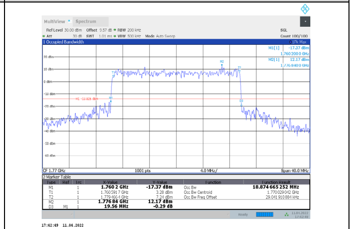
1-N66-PC3-15-20-H-4-CP-256QAM-Outer_Full-106@0-Ant 1-18.875-19.560-≤20-PASS
