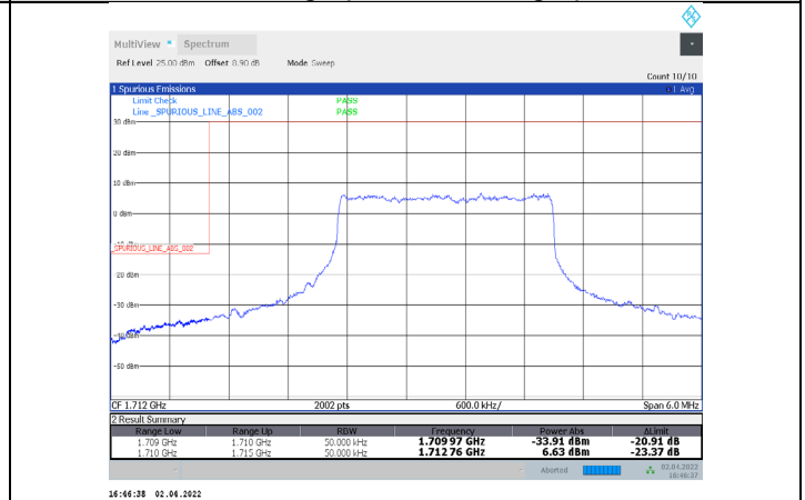
1-N66-PC3-15-5-L-8-DFT-QPSK-Inner_Full-12@6-Ant1-seegraph-PASS-see graph
