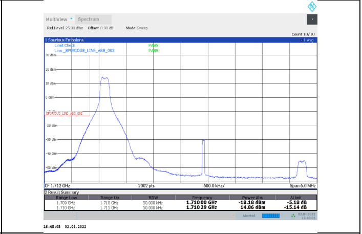
1-N66-PC3-15-5-L-13-DFT-64QAM-Edge_1RB_Left-1@0-Ant1-seegraph-PASS-see graph
