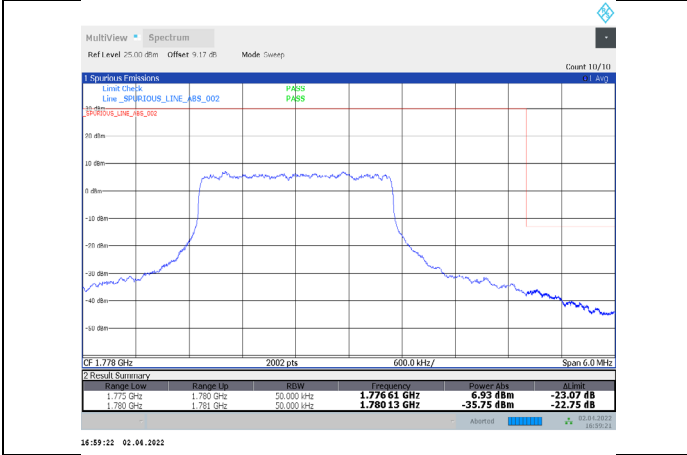
1-N66-PC3-15-5-H-16-DFT-64QAM-Inner_Full-12@6-Ant1-seegraph-PASS-see graph
