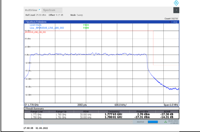
1-N66-PC3-15-5-H-19-DFT-256QAM-Outer_Full-25@0-Ant1-seegraph-PASS-see graph
