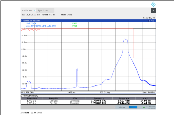
1-N66-PC3-15-5-H-14-DFT-64QAM-Edge_1RB_Right-1 @24-Ant1-seegraph-PASS-see graph
