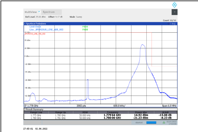
1-N66-PC3-15-5-H-30-CP-64QAM-Edge_1RB_Right-1 @24-Ant1-seegraph-PASS-see graph
