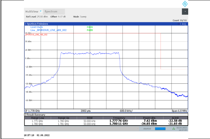
1-N66-PC3-15-5-H-8-DFT-QPSK-Inner_Full-12@6-Ant1-seegraph-PASS-see graph
