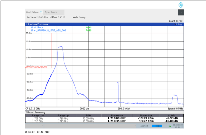
1-N66-PC3-15-5-L-25-CP-16QAM-Edge_1RB_Left-1@0-Ant1-seegraph-PASS-see graph
