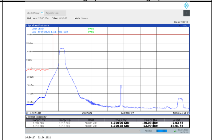
1-N66-PC3-15-5-L-21-CP-QPSK-Edge_1RB_Left-1@0-Ant1-seegraph-PASS-see graph
