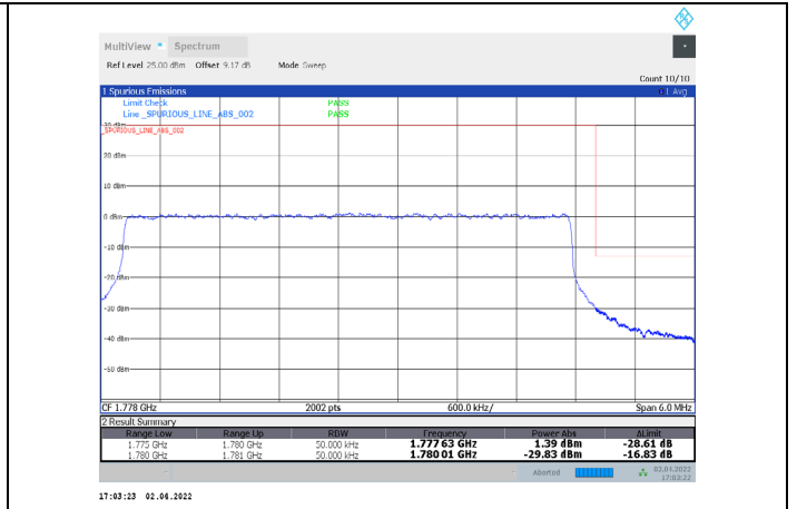
1-N66-PC3-15-5-H-31-CP-64QAM-Outer_Full-25@0-Ant 1-seegraph-PASS-see graph
