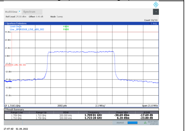
1-N66-PC3-15-20-L-8-DFT-QPSK-Inner_Full-50@25-Ant 1-seegraph-PASS-see graph
