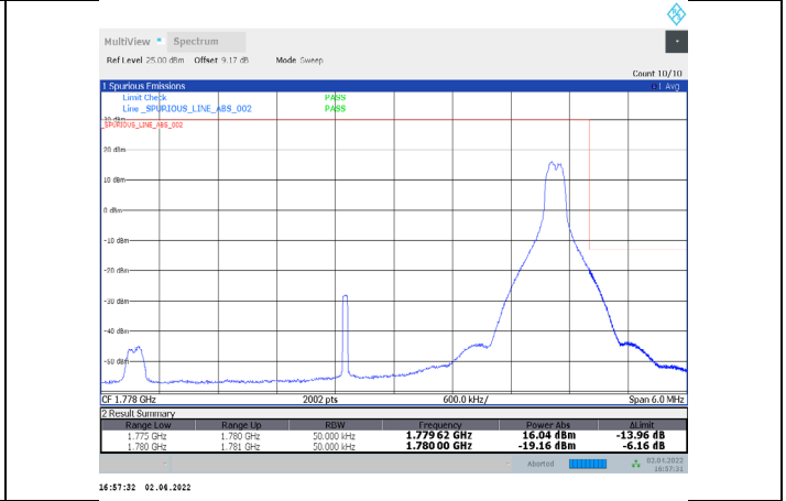
1-N66-PC3-15-5-H-10-DFT-16QAM-Edge_1RB_Right-1 @24-Ant1-seegraph-PASS-see graph
