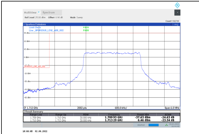
1-N66-PC3-15-5-L-1-DFT-PI/2BPSK-Inner_Full-12@6-Ant1-seegraph-PASS-see graph
