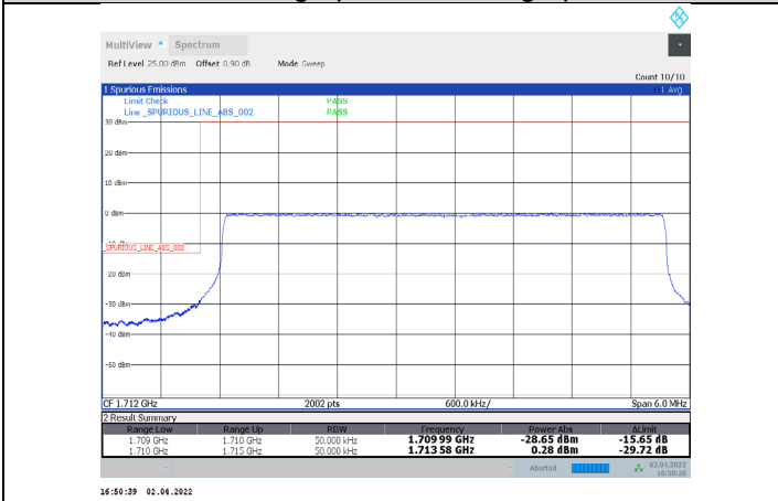
1-N66-PC3-15-5-L-23-CP-QPSK-Outer_Full-25@0-Ant1-seegraph-PASS-see graph
