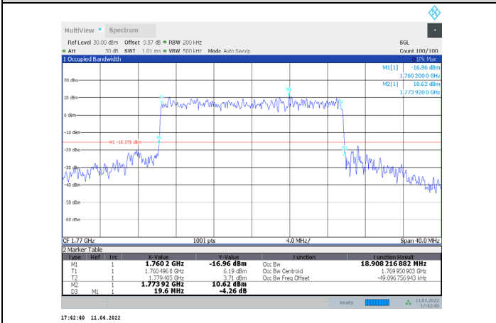
1-N66-PC3-15-20-H-3-CP-64QAM-Outer_Full-106@0-Ant 1-18.908-19.600-≤20-PASS
