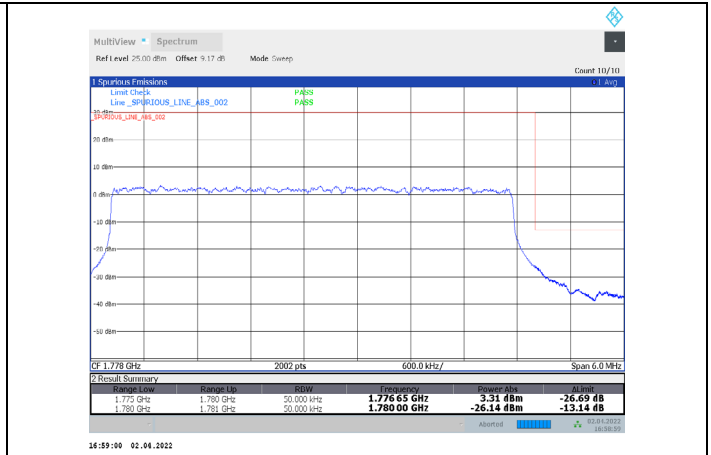
1-N66-PC3-15-5-H-15-DFT-64QAM-Outer_Full-25@0-Ant1-seegraph-PASS-see graph
