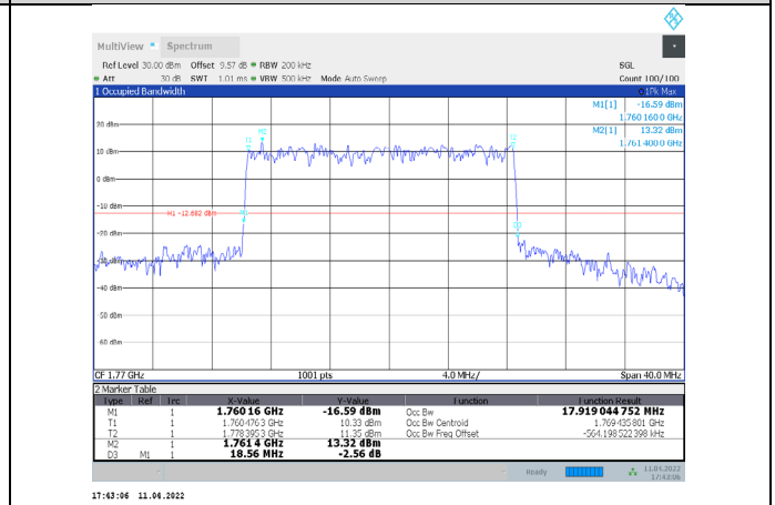
1-N66-PC3-15-20-H-6-DFT-QPSK-Outer_Full-100@0-Ant 1-17.919-18.560-≤20-PASS
