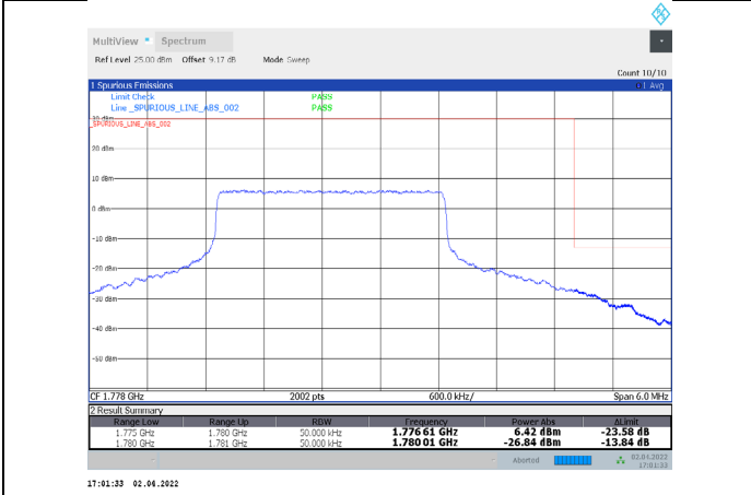
1-N66-PC3-15-5-H-24-CP-QPSK-Inner_Full-13@6-Ant1-seegraph-PASS-see graph
