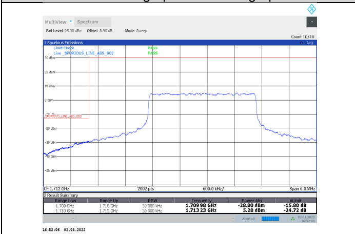
1-N66-PC3-15-5-L-28-CP-16QAM-Inner_Full-13@6-Ant1-seegraph-PASS-see graph
