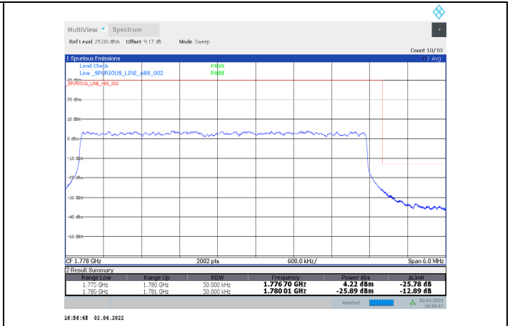
1-N66-PC3-15-5-H-7-DFT-QPSK-Outer_Full-25@0-Ant1-seegraph-PASS-see graph
