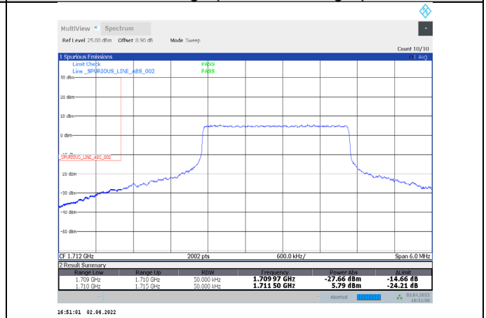
1-N66-PC3-15-5-L-24-CP-QPSK-Inner_Full-13@6-Ant1-seegraph-PASS-see graph
