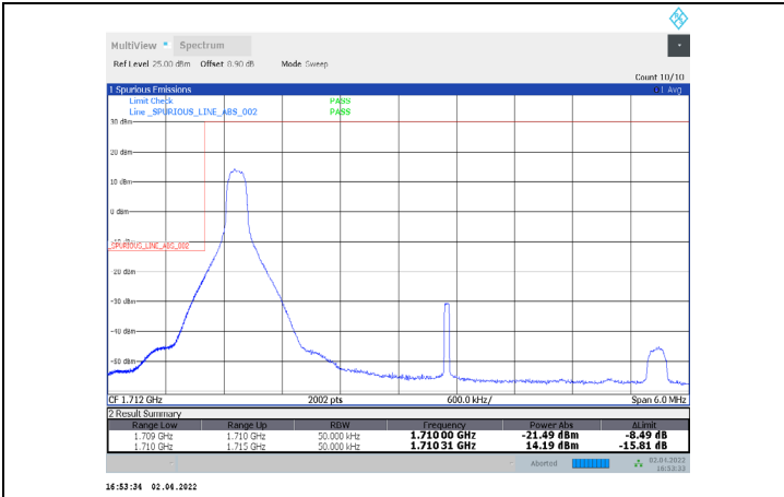
1-N66-PC3-15-5-L-33-CP-256QAM-Edge_1RB_Left-1@0-Ant1-seegraph-PASS-see graph
