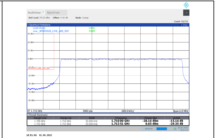
1-N66-PC3-15-5-L-27-CP-16QAM-Outer_Full-25@0-Ant1-seegraph-PASS-see graph
