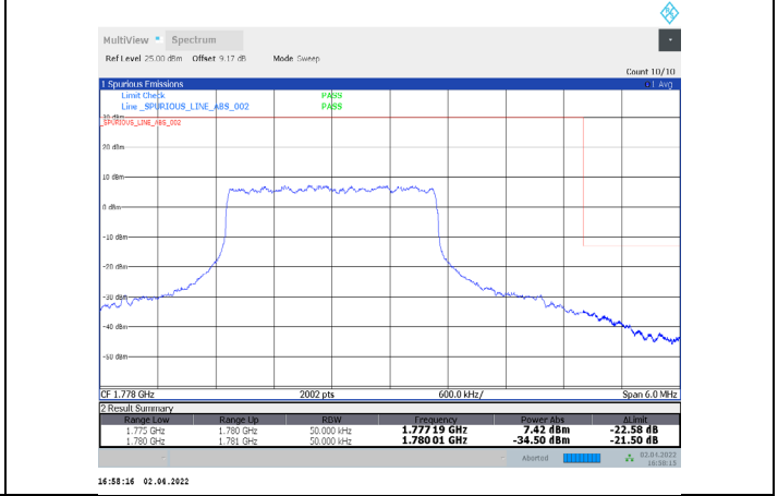
1-N66-PC3-15-5-H-12-DFT-16QAM-Inner_Full-12@6-Ant1-seegraph-PASS-see graph
