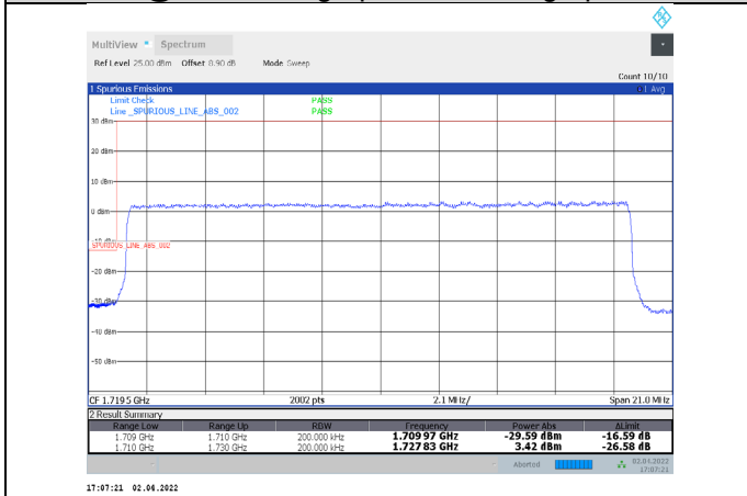
1-N66-PC3-15-20-L-7-DFT-QPSK-Outer_Full-100@0 -Ant1-seegraph-PASS-see graph
