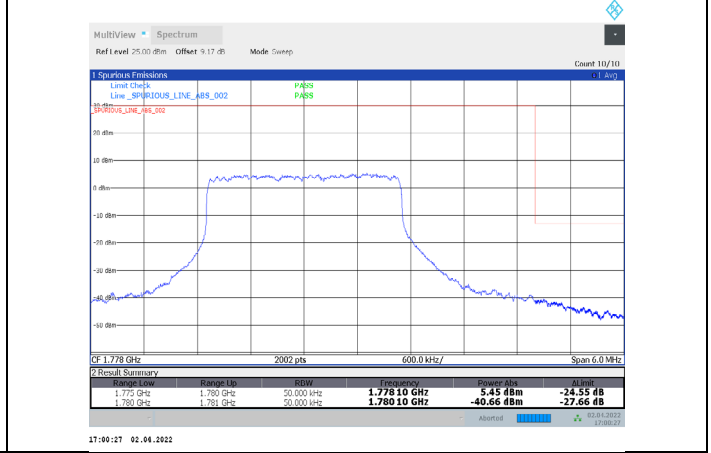
1-N66-PC3-15-5-H-20-DFT-256QAM-Inner_Full-12@6-Ant1-seegraph-PASS-see graph
