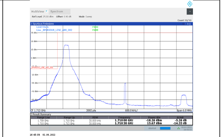
1-N66-PC3-15-5-L-5-DFT-QPSK-Edge_1RB_Left-1@0-Ant1-seegraph-PASS-see graph
