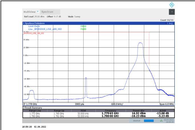
1-N66-PC3-15-5-H-6-DFT-QPSK-Edge_1RB_Right-1 @24-Ant1-seegraph-PASS-see graph
