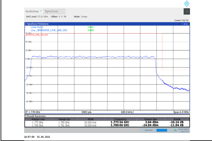
1-N66-PC3-15-5-H-11-DFT-16QAM-Outer_Full-25@0-Ant1-seegraph-PASS-see graph
