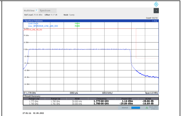
1-N66-PC3-15-5-H-23-CP-QPSK-Outer_Full-25@0-Ant1-seegraph-PASS-see graph
