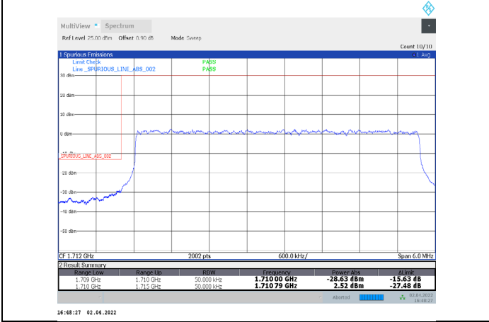
1-N66-PC3-15-5-L-15-DFT-64QAM-Outer_Full-25@0-Ant1-seegraph-PASS-see graph
