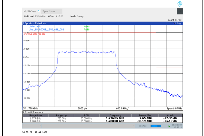
1-N66-PC3-15-5-H-1-DFT-PI/2BPSK-Inner_Full-12@6-Ant1-seegraph-PASS-see graph
