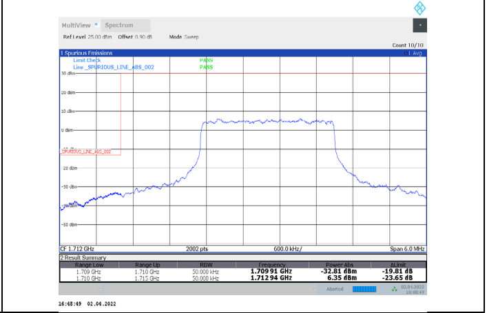
1-N66-PC3-15-5-L-16-DFT-64QAM-Inner_Full-12@6-Ant1-seegraph-PASS-see graph
