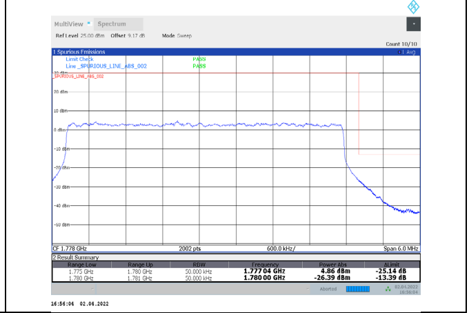
1-N66-PC3-15-5-H-4-DFT-PI/2BPSK-Outer_Full-25@0-Ant1-seegraph-PASS-see graph
