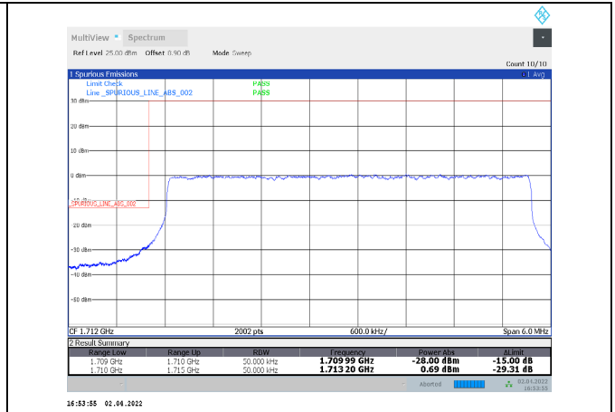
1-N66-PC3-15-5-L-35-CP-256QAM-Outer_Full-25@0-Ant1-seegraph-PASS-see graph
