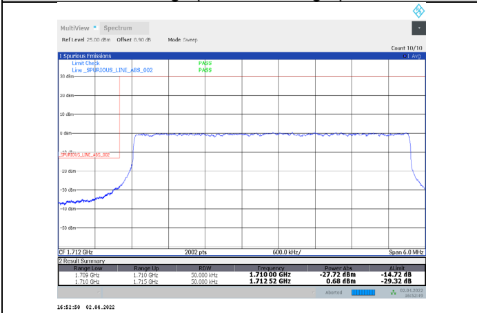
1-N66-PC3-15-5-L-31-CP-64QAM-Outer_Full-25@0-Ant1-seegraph-PASS-see graph
