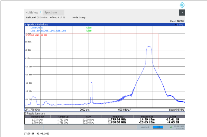
1-N66-PC3-15-5-H-22-CP-QPSK-Edge_1RB_Right-1@24-Ant1-seegraph-PASS-see graph
