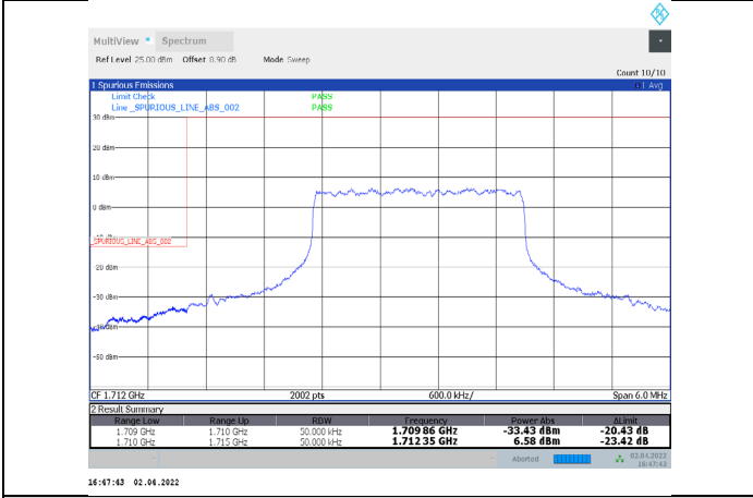
1-N66-PC3-15-5-L-12-DFT-16QAM-Inner_Full-12@6-Ant1-seegraph-PASS-see graph
