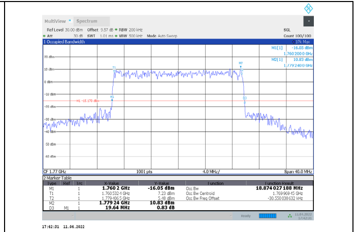
1-N66-PC3-15-20-H-2-CP-16QAM-Outer_Full-106@0-Ant 1-18.874-19.640-≤20-PASS
