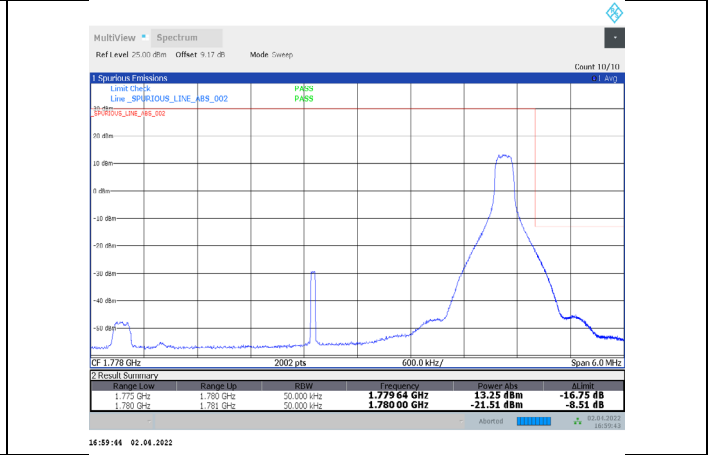
1-N66-PC3-15-5-H-18-DFT-256QAM-Edge_1RB_Right-1@24-Ant1-seegraph-PASS-see graph
