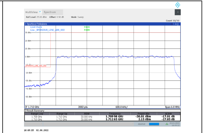
1-N66-PC3-15-5-L-19-DFT-256QAM-Outer_Full-25@0-Ant1-seegraph-PASS-see graph
