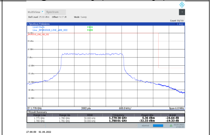
1-N66-PC3-15-5-H-36-CP-256QAM-Inner_Full-13@6-Ant1-seegraph-PASS-see graph
