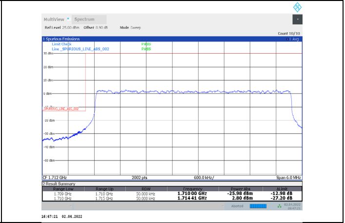
1-N66-PC3-15-5-L-11-DFT-16QAM-Outer_Full-25@0-Ant1-seegraph-PASS-see graph
