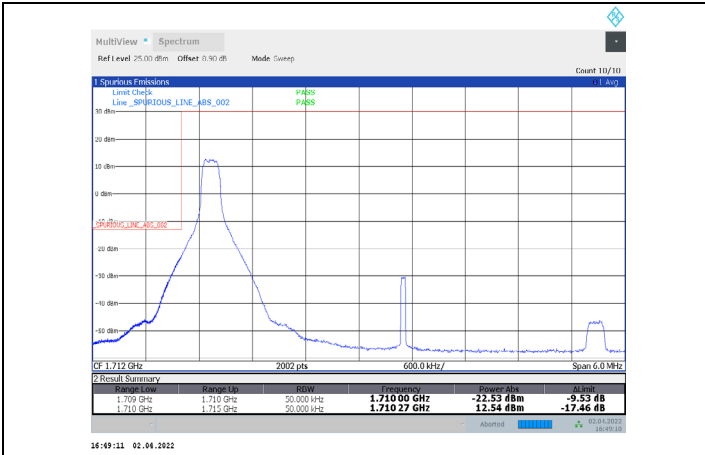
1-N66-PC3-15-5-L-17-DFT-256QAM-Edge_1RB_Left-1@0-Ant1-seegraph-PASS-see graph
