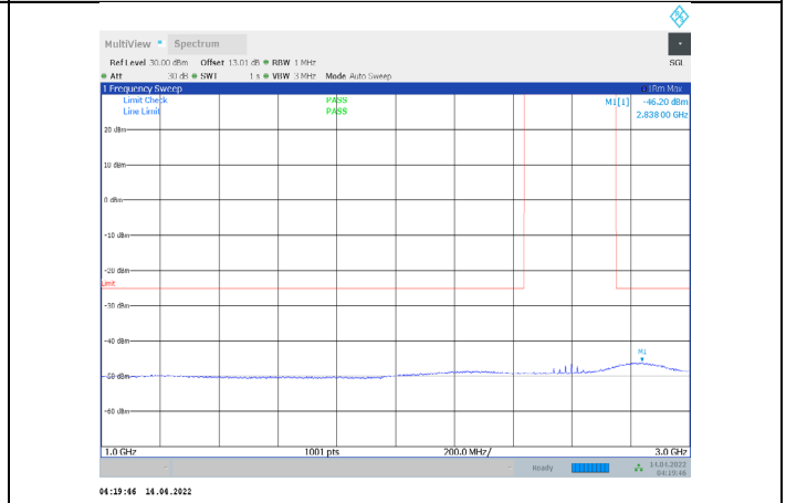
1-N41-PC3-30-100-M-1-CP-QPSK-Edge_1RB_Left-1@ 0-1000-3000-Ant1--46.20--25-PASS
