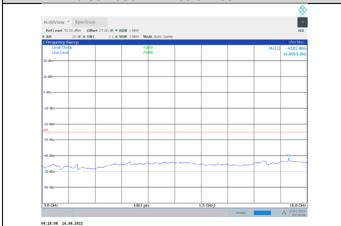
1-N41-PC3-30-100-L-1-CP-QPSK-Edge_1RB_Left-1@ 0-3000-18000-Ant1--43.02--25-PASS
