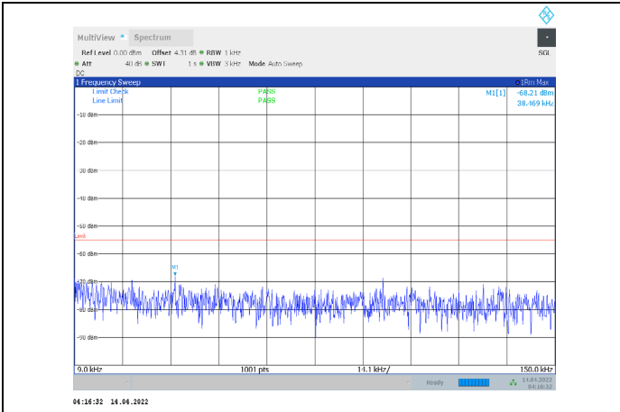
1-N41-PC3-30-100-L-2-CP-QPSK-Edge_1RB_Right-1 @272-0.009-0.15-Ant1--68.21--55-PASS
