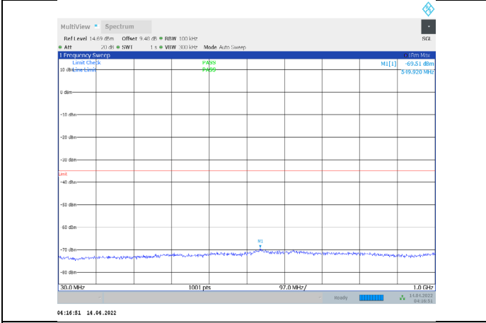
1-N41-PC3-30-100-L-2-CP-QPSK-Edge_1RB_Right-1 @272-30-1000-Ant1--69.51--35-PASS
