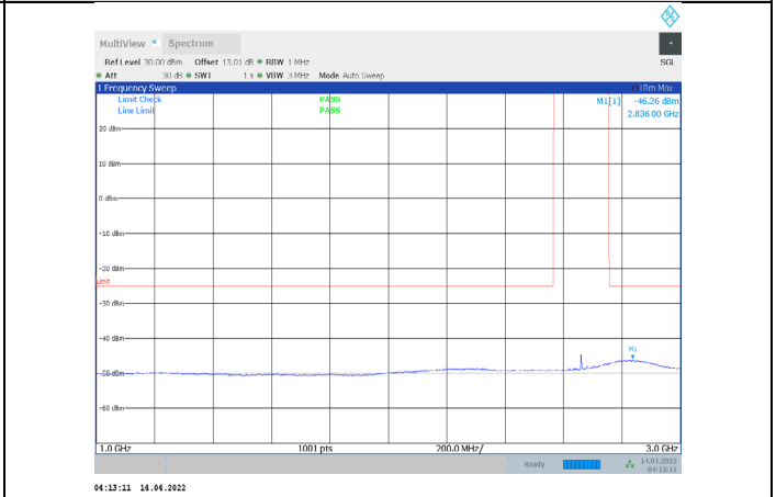
1-N41-PC3-30-60-H-2-CP-QPSK-Edge_1RB_Right-1@ 161-1000-3000-Ant1--46.26--25-PASS
