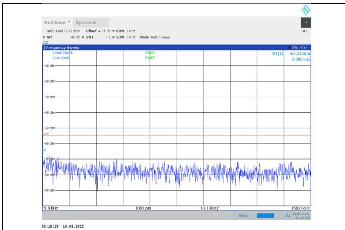
1-N41-PC3-30-100-L-1-CP-QPSK-Edge_1RB_Left-1@ 0-0.009-0.15-Ant1--67.24--55-PASS
