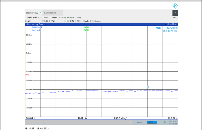
1-N41-PC3-30-100-L-1-CP-QPSK-Edge_1RB_Left-1@ -18000-26900-Ant1--40.42--25-PASS
