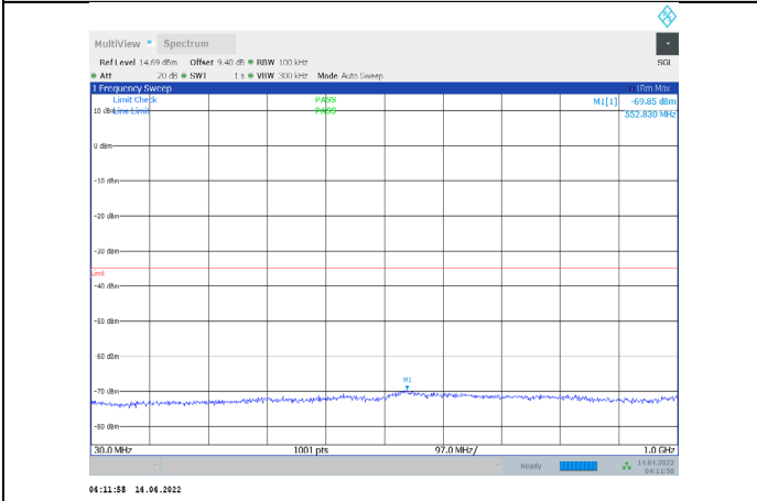
1-N41-PC3-30-60-H-1-CP-QPSK-Edge_1RB_Left-1@ -30-1000-Ant1--69.85--35-PASS
