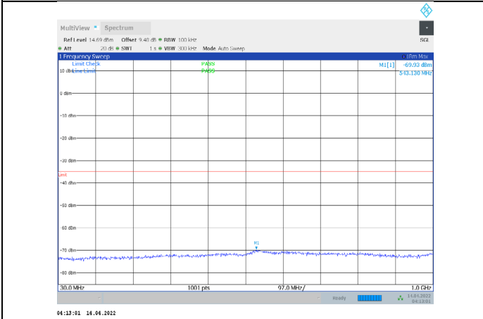
1-N41-PC3-30-60-H-2-CP-QPSK-Edge_1RB_Right-1@ 161-30-1000-Ant1--69.93--35-PASS
