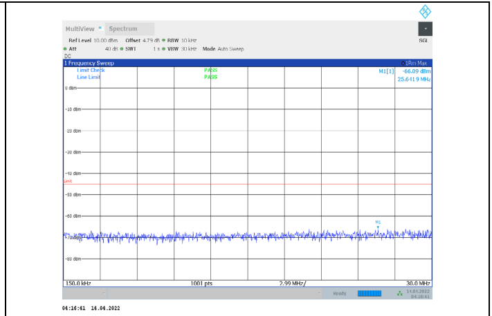
1-N41-PC3-30-100-L-2-CP-QPSK-Edge_1RB_Right-1@ 272-0.15-30-Ant1--66.09--45-PASS
