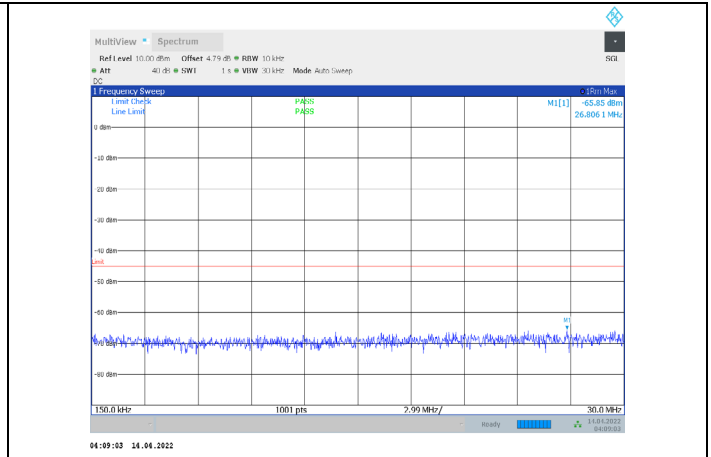
1-N41-PC3-30-60-M-2-CP-QPSK-Edge_1RB_Right-1@ 161-0.15-30-Ant1--65.85--45-PASS
