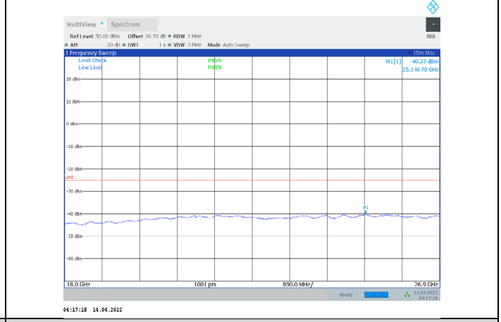
1-N41-PC3-30-100-L-2-CP-QPSK-Edge_1RB_Right-1@ 272-18000-26900-Ant1--40.37--25-PASS
