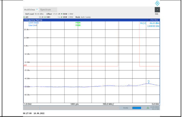
1-N41-PC3-30-100-L-2-CP-QPSK-Edge_1RB_Right-1@ 272-1000-3000-Ant1--46.33--25-PASS
