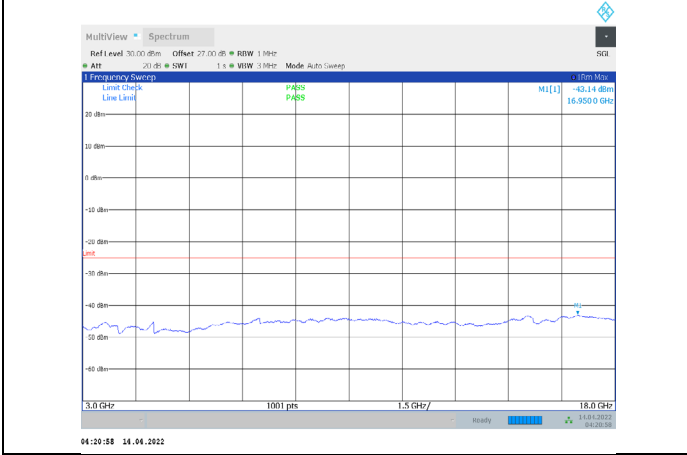
1-N41-PC3-30-100-M-2-CP-QPSK-Edge_1RB_Right-1 @272-3000-18000-Ant1--43.14--25-PASS
