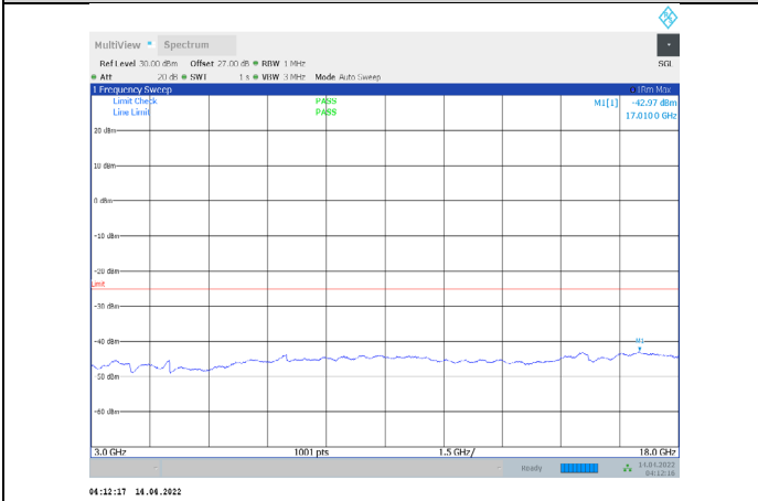
1-N41-PC3-30-60-H-1-CP-QPSK-Edge_1RB_Left-1@ -3000-18000-Ant1--42.97--25-PASS
