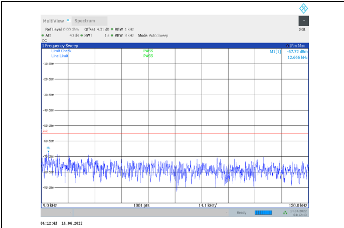
1-N41-PC3-30-60-H-2-CP-QPSK-Edge_1RB_Right-1@ 161-0.009-0.15-Ant1--67.72--55-PASS
