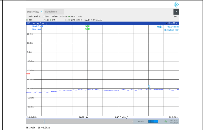
1-N41-PC3-30-100-M-1-CP-QPSK-Edge_1RB_Left-1@ 0-18000-26900-Ant1--40.34--25-PASS
