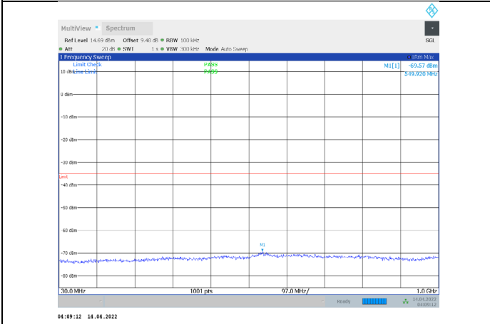
1-N41-PC3-30-60-M-2-CP-QPSK-Edge_1RB_Right-1@ 161-30-1000-Ant1--69.57--35-PASS
