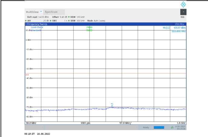
1-N41-PC3-30-100-M-1-CP-QPSK-Edge_1RB_Left-1@ 0-30-1000-Ant1--69.97--35-PASS
