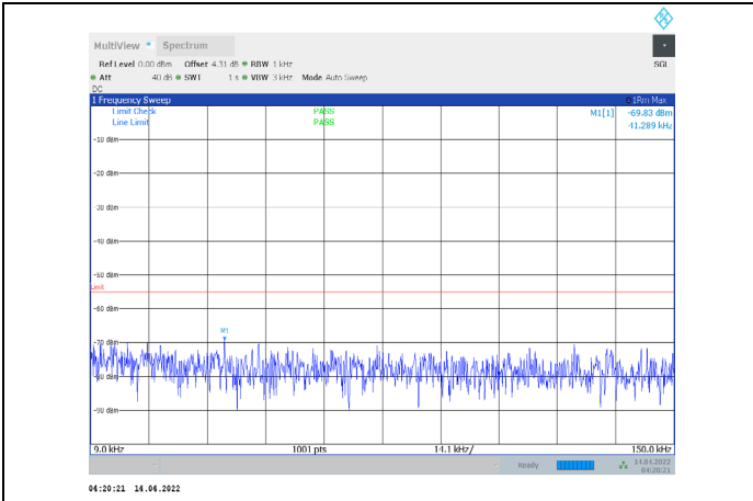
1-N41-PC3-30-100-M-2-CP-QPSK-Edge_1RB_Right-1 @272-0.009-0.15-Ant1--69.83--55-PASS
