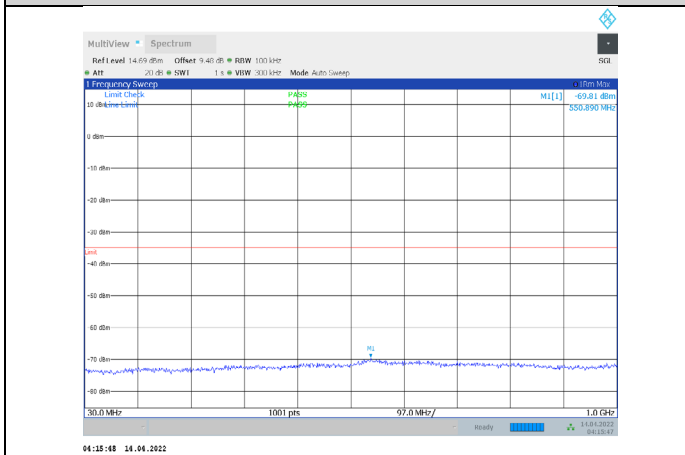
1-N41-PC3-30-100-L-1-CP-QPSK-Edge_1RB_Left-1@ 0-30-1000-Ant1--69.81--35-PASS
