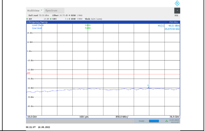
1-N41-PC3-30-100-M-2-CP-QPSK-Edge_1RB_Right-1 @272-18000-26900-Ant1--40.31--25-PASS
