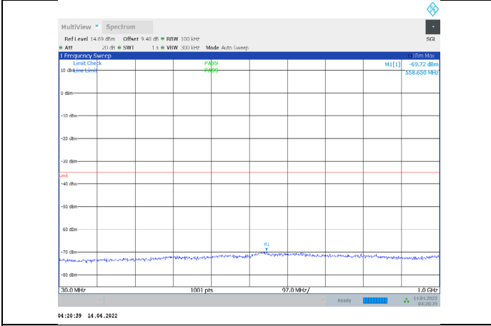
1-N41-PC3-30-100-M-2-CP-QPSK-Edge_1RB_Right-1 @272-30-1000-Ant1--69.72--35-PASS
