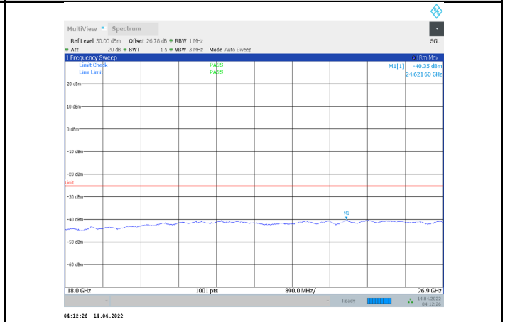
1-N41-PC3-30-60-H-1-CP-QPSK-Edge_1RB_Left-1@ 18000-26900-Ant1--40.35--25-PASS
