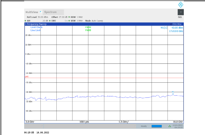
1-N41-PC3-30-100-M-1-CP-QPSK-Edge_1RB_Left-1@ 0-3000-18000-Ant1--43.05--25-PASS
