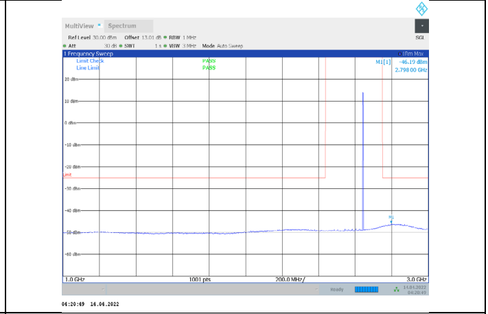
1-N41-PC3-30-100-M-2-CP-QPSK-Edge_1RB_Right-1 @272-1000-3000-Ant1--46.19--25-PASS
