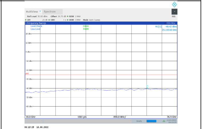
1-N41-PC3-30-60-H-2-CP-QPSK-Edge_1RB_Right-1@ 161-18000-26900-Ant1--40.42--25-PASS
