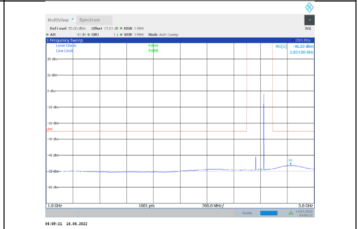
1-N41-PC3-30-60-M-2-CP-QPSK-Edge_1RB_Right-1@ 161-1000-3000-Ant1--46.33--25-PASS
