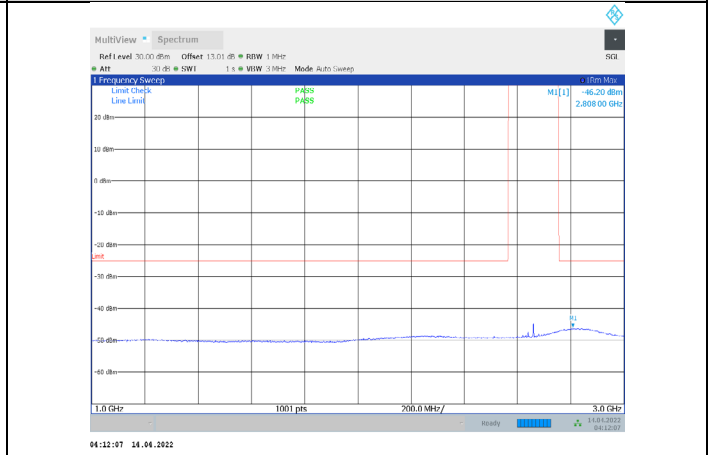
1-N41-PC3-30-60-H-1-CP-QPSK-Edge_1RB_Left-1@ 1000-3000-Ant1--46.20--25-PASS
