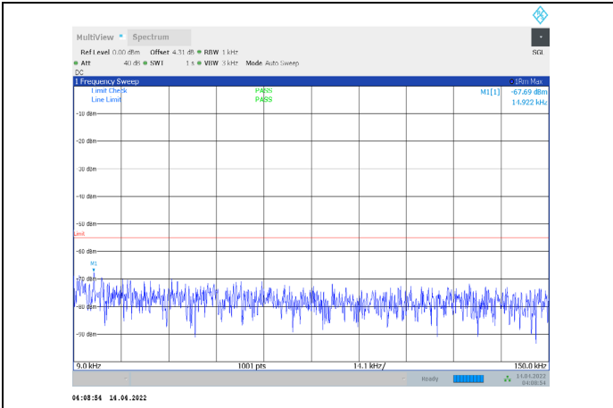
1-N41-PC3-30-60-M-2-CP-QPSK-Edge_1RB_Right-1@ 161-0.009-0.15-Ant1--67.69--55-PASS
