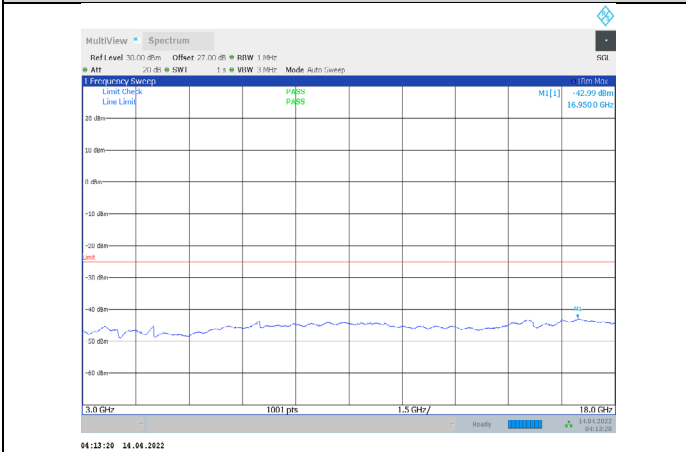
1-N41-PC3-30-60-H-2-CP-QPSK-Edge_1RB_Right-1@ 161-3000-18000-Ant1--42.99--25-PASS
