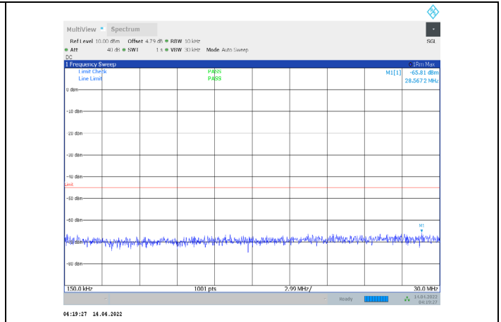
1-N41-PC3-30-100-M-1-CP-QPSK-Edge_1RB_Left-1@ 0-0.15-30-Ant1--65.81--45-PASS
