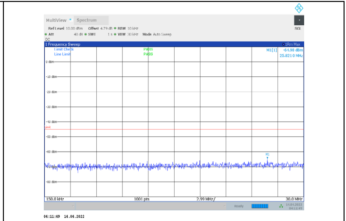
1-N41-PC3-30-60-H-1-CP-QPSK-Edge_1RB_Left-1@ 0.15-30-Ant1--64.98--45-PASS
