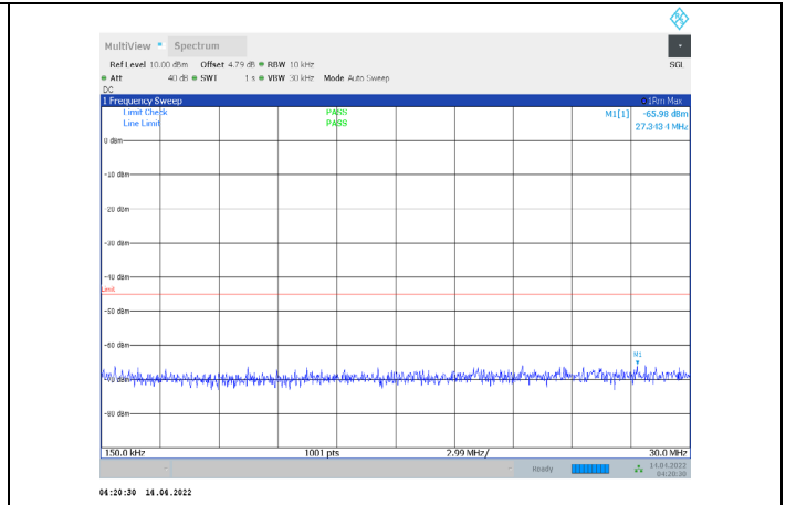
1-N41-PC3-30-100-M-2-CP-QPSK-Edge_1RB_Right-1 @272-0.15-30-Ant1--65.98--45-PASS
