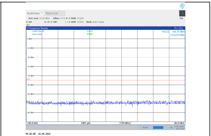
1-N41-PC3-30-100-L-1-CP-QPSK-Edge_1RB_Left-1@ -0.15-30-Ant1--65.75--45-PASS
