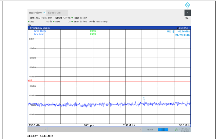
1-N41-PC3-30-100-H-1-CP-QPSK-Edge_1RB_Left-1@ -0.15-30-Ant1--65.76--45-PASS
