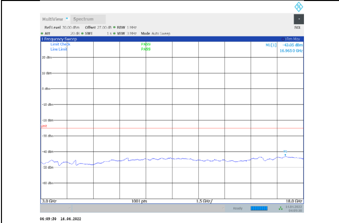
1-N41-PC3-30-60-M-2-CP-QPSK-Edge_1RB_Right-1@ 161-3000-18000-Ant1--43.05--25-PASS
