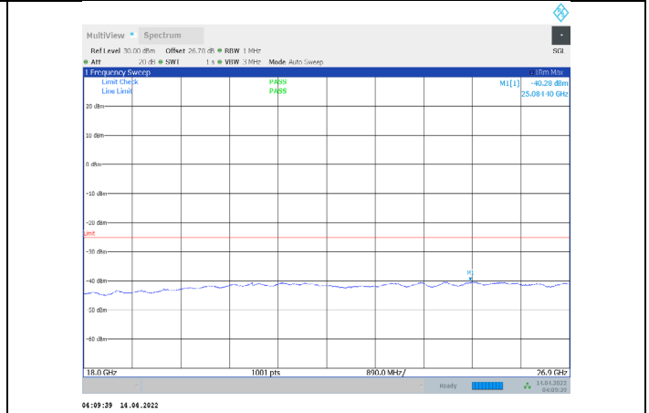
1-N41-PC3-30-60-M-2-CP-QPSK-Edge_1RB_Right-1@ 161-18000-26900-Ant1--40.28--25-PASS
