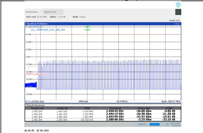
1-N41-PC3-30-100-L-31-CP-64QAM-Outer_Full-273@0 -Ant1-PASS-see graph
