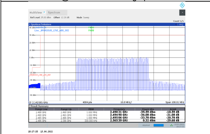
1-N41-PC3-30-100-L-36-CP-256QAM-Inner_Full-137@68 -Ant1-PASS-see graph
