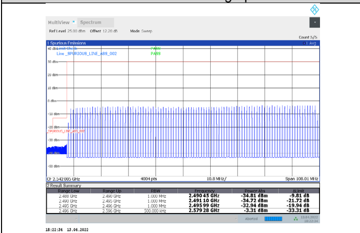
1-N41-PC3-30-100-L-23-CP-QPSK-Outer_Full-273@0-Ant1-PASS-see graph
