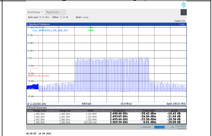
1-N41-PC3-30-100-L-32-CP-64QAM-Inner_Full-137@6 8-Ant1-PASS-see graph
