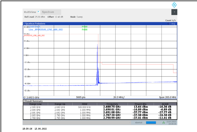
1-N41-PC3-30-100-H-6-DFT-QPSK-Edge_1RB_Right-1@272-Ant1-PASS-see graph
