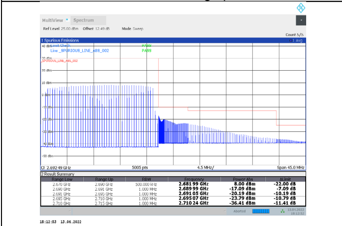
1-N41-PC3-30-20-H-35-CP-256QAM-Outer_Full-51@0-Ant1-PASS-see graph
