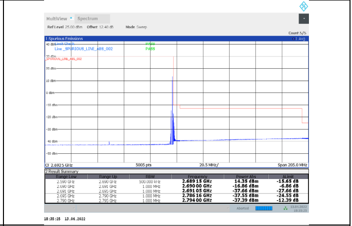
1-N41-PC3-30-100-H-18-DFT-256QAM-Edge_1RB_Right-1@272-Ant1-PASS-see graph
