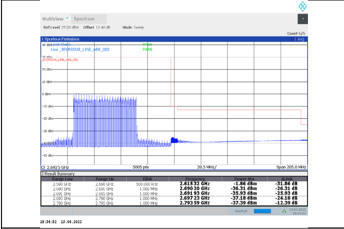
1-N41-PC3-30-100-H-16-DFT-64QAM-Inner_Full-135@67-Ant1-PASS-see graph
