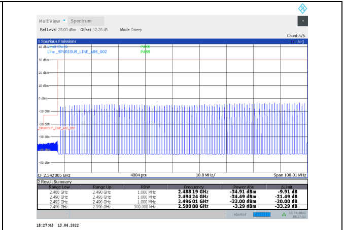
1-N41-PC3-30-100-L-35-CP-256QAM-Outer_Full-273 @0-Ant1-PASS-see graph
