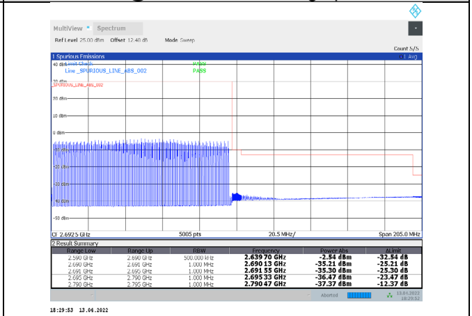
1-N41-PC3-30-100-H-4-DFT-PI/2BPSK-Outer_Full-27 0@0-Ant1-PASS-see graph
