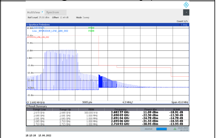
1-N41-PC3-30-20-H-36-CP-256QAM-Inner_Full-25@12-Ant1-PASS-see graph
