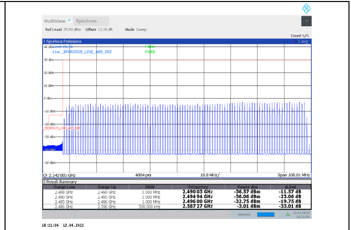
1-N41-PC3-30-100-L-19-DFT-256QAM-Outer_Full-270@0-Ant1-PASS-see graph
