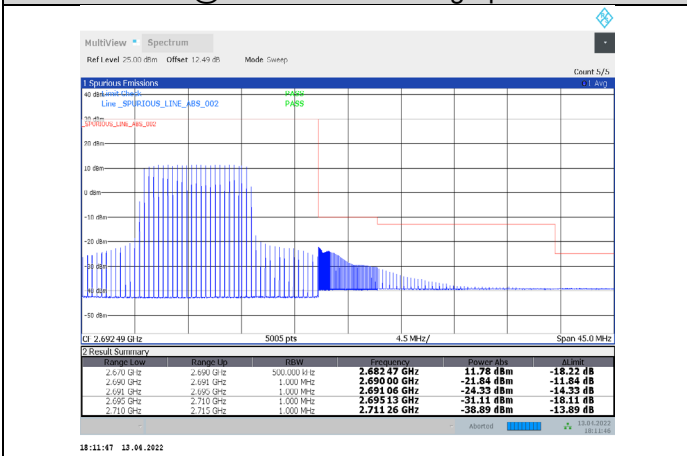
1-N41-PC3-30-20-H-32-CP-64QAM-Inner_Full-25@12-Ant1-PASS-see graph
