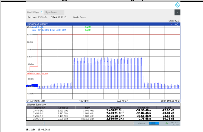
1-N41-PC3-30-100-L-20-DFT-256QAM-Inner_Full-135@67-Ant1-PASS-see graph
