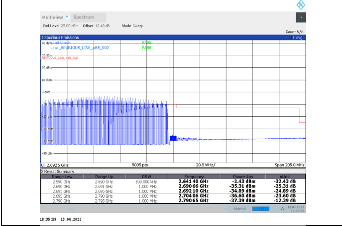
1-N41-PC3-30-100-H-19-DFT-256QAM-Outer_Full-270@0-Ant1-PASS-see graph
