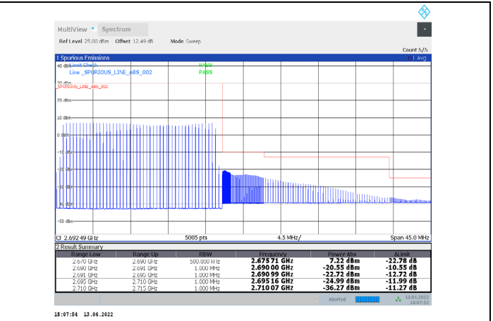
1-N41-PC3-30-20-H-23-CP-QPSK-Outer_Full-51@0-Ant 1-PASS-see graph
