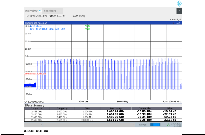
1-N41-PC3-30-100-L-15-DFT-64QAM-Outer_Full-270 @0-Ant1-PASS-see graph
