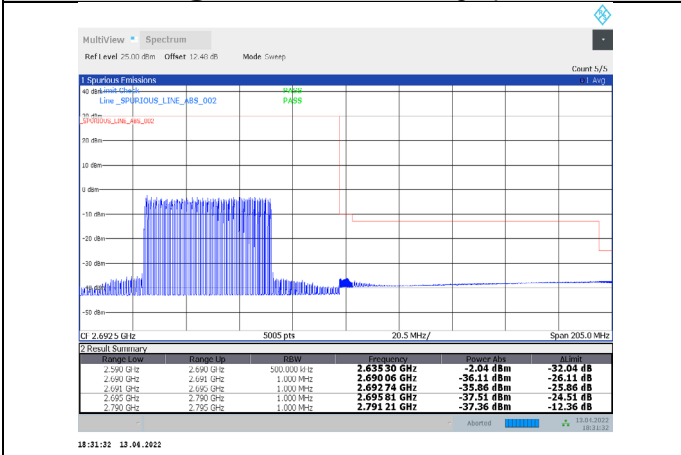
1-N41-PC3-30-100-H-8-DFT-QPSK-Inner_Full-135@67-Ant1-PASS-see graph
