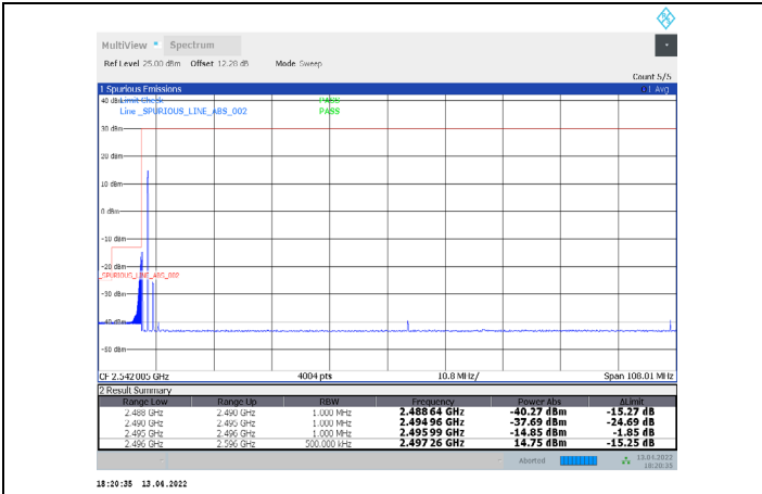
1-N41-PC3-30-100-L-17-DFT-256QAM-Edge_1RB_Left-1@0-Ant1-PASS-see graph
