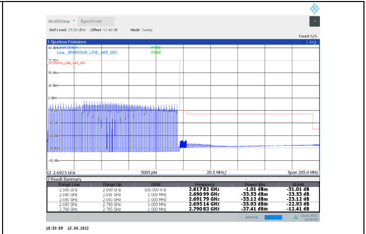
1-N41-PC3-30-100-H-7-DFT-QPSK-Outer_Full-270@0-Ant1-PASS-see graph
