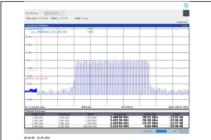
1-N41-PC3-30-100-L-1-DFT-PI/2BPSK-Inner_Full-135 @67-Ant1-PASS-see graph
