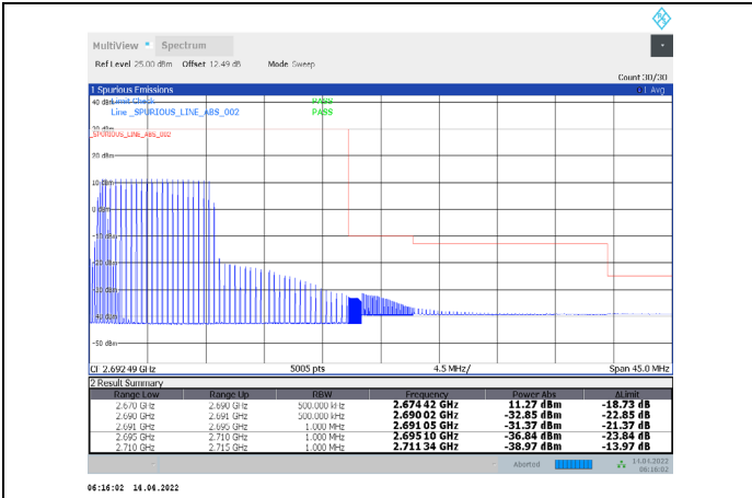
1-N41-PC3-30-20-H-22-CP-QPSK-Edge_1RB_Right-1 @50-Ant1-PASS-see graph
