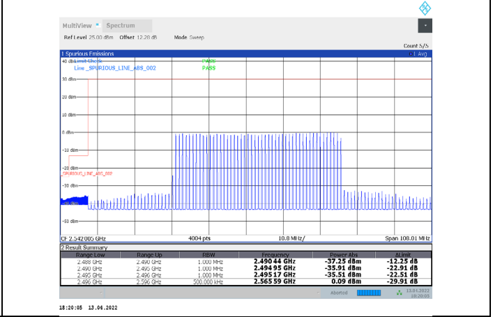
1-N41-PC3-30-100-L-16-DFT-64QAM-Inner_Full-135@6 7-Ant1-PASS-see graph
