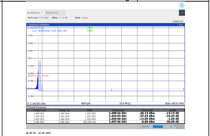
1-N41-PC3-30-100-L-29-CP-64QAM-Edge_1RB_Left-1 @0-Ant1-PASS-see graph
