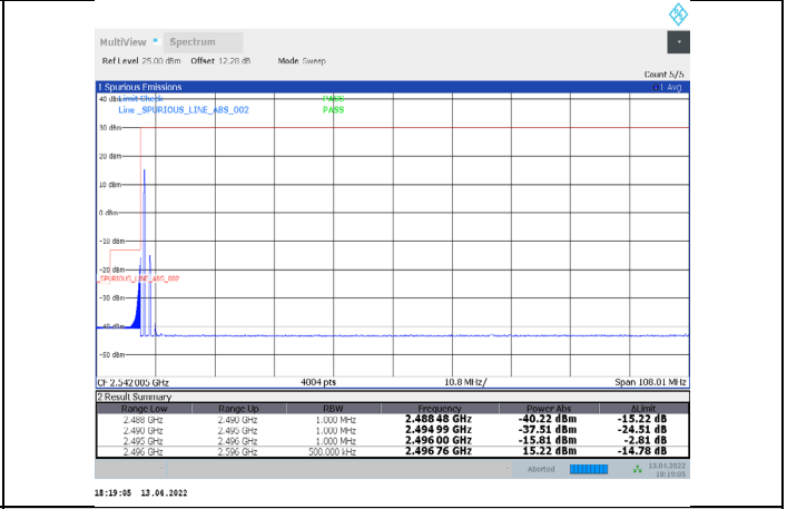
1-N41-PC3-30-100-L-13-DFT-64QAM-Edge_1RB_Left-1 @0-Ant1-PASS-see graph
