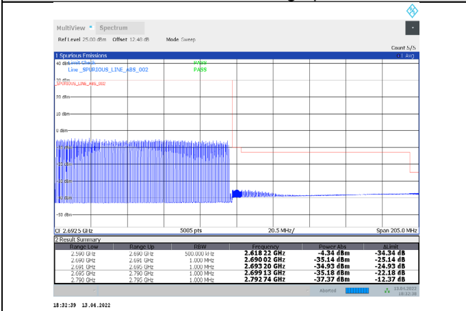
1-N41-PC3-30-100-H-11-DFT-16QAM-Outer_Full-270@0-Ant1-PASS-see graph
