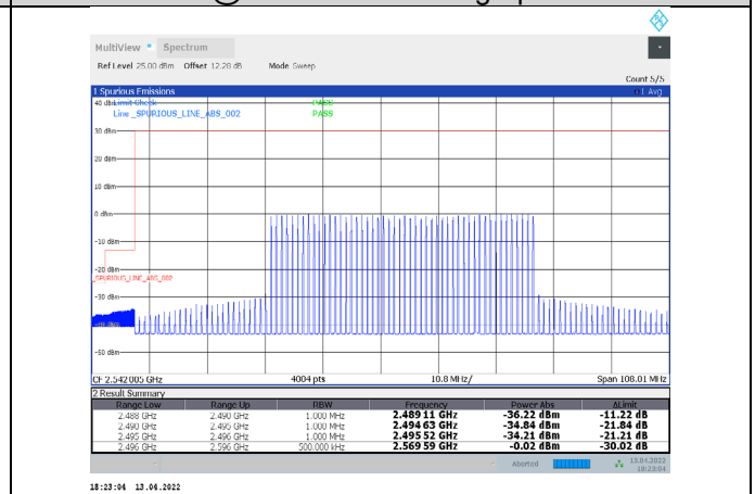
1-N41-PC3-30-100-L-24-CP-QPSK-Inner_Full-137@8-Ant1-PASS-see graph
