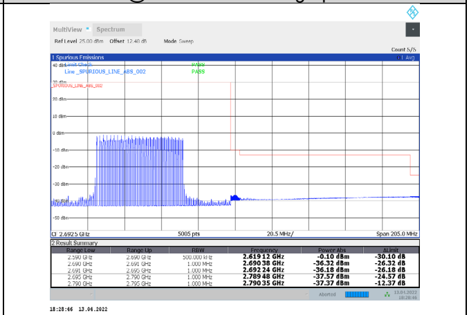
1-N41-PC3-30-100-H-1-DFT-PI/2BPSK-Inner_Full-13 5@67-Ant1-PASS-see graph
