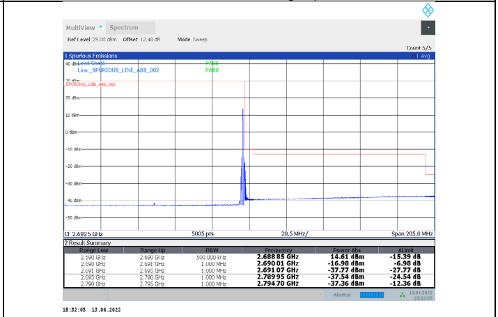
1-N41-PC3-30-100-H-10-DFT-16QAM-Edge_1RB_Right-1@272-Ant1-PASS-see graph
