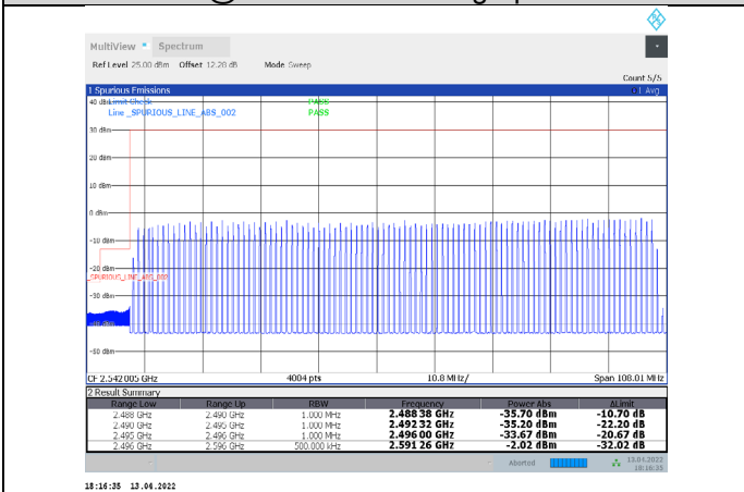
1-N41-PC3-30-100-L-7-DFT-QPSK-Outer_Full-270@0-Ant1-PASS-see graph
