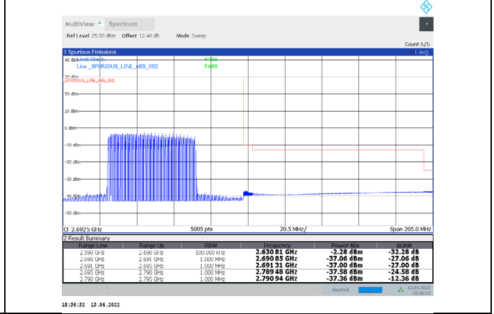
1-N41-PC3-30-100-H-20-DFT-256QAM-Inner_Full-135@67-Ant1-PASS-see graph
