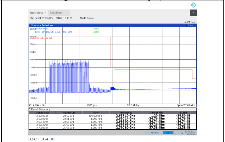
1-N41-PC3-30-100-H-12-DFT-16QAM-Inner_Full-135@67-Ant1-PASS-see graph
