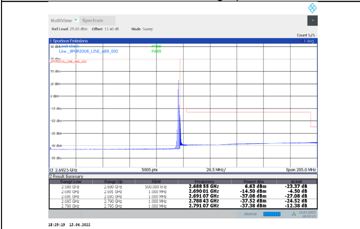
1-N41-PC3-30-100-H-3-DFT-PI/2BPSK-Edge_1RB_Right-1@272-Ant1-PASS-see graph
