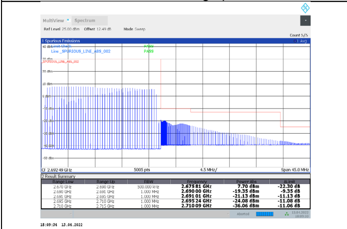
1-N41-PC3-30-20-H-27-CP-16QAM-Outer_Full-51@0-Ant1-PASS-see graph
