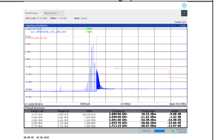
1-N41-PC3-30-20-H-26-CP-16QAM-Edge_1RB_Right-1 @50-Ant1-PASS-see graph
