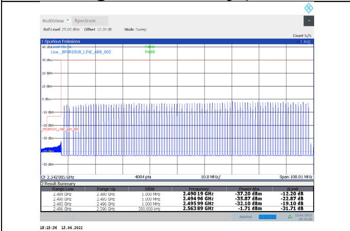
1-N41-PC3-30-100-L-4-DFT-PI/2BPSK-Outer_Full-270 @0-Ant1-PASS-see graph
