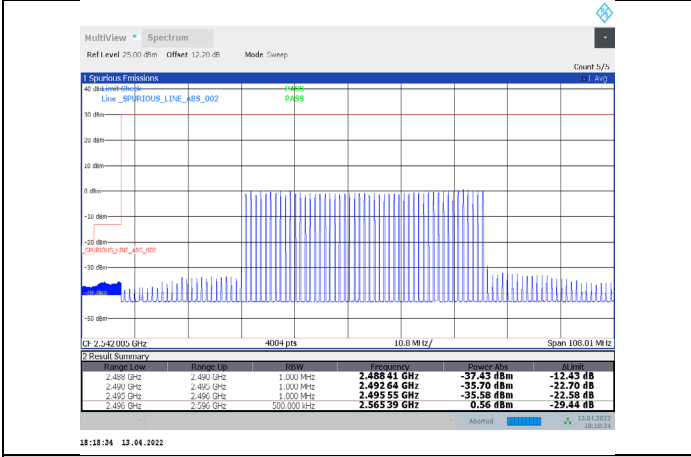
1-N41-PC3-30-100-L-12-DFT-16QAM-Inner_Full-135@ 67-Ant1-PASS-see graph
