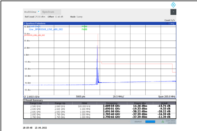
1-N41-PC3-30-100-H-14-DFT-64QAM-Edge_1RB_Right-1@272-Ant1-PASS-see graph
