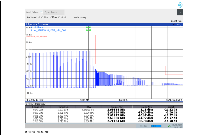
1-N41-PC3-30-20-H-31-CP-64QAM-Outer_Full-51@0-Ant1-PASS-see graph
