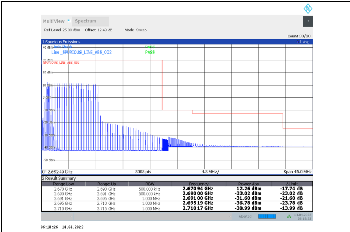
1-N41-PC3-30-20-H-30-CP-64QAM-Edge_1RB_Right-1@50-Ant1-PASS-see graph
