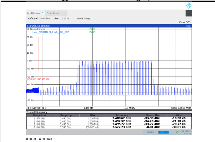
1-N41-PC3-30-100-L-28-CP-16QAM-Inner_Full-137@6 8-Ant1-PASS-see graph
