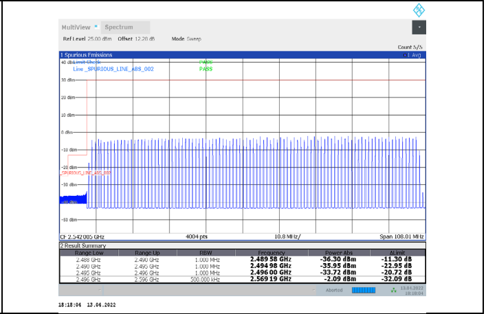
1-N41-PC3-30-100-L-11-DFT-16QAM-Outer_Full-270@ 0-Ant1-PASS-see graph
