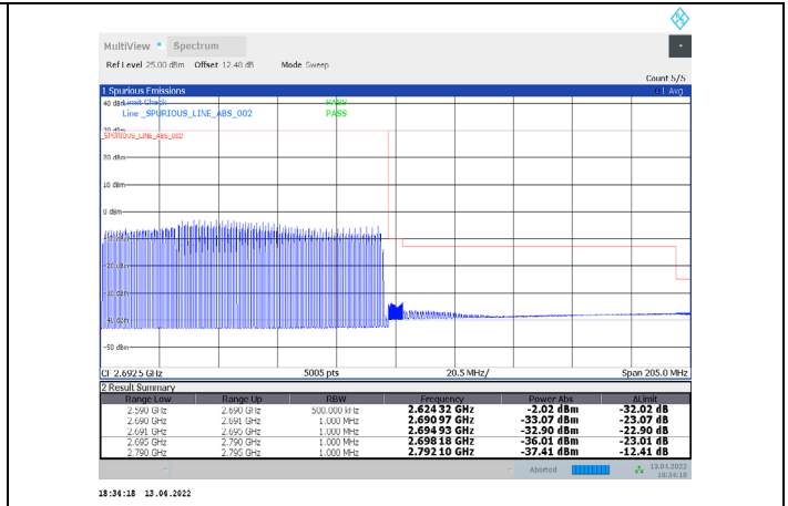
1-N41-PC3-30-100-H-15-DFT-64QAM-Outer_Full-270@0-Ant1-PASS-see graph
