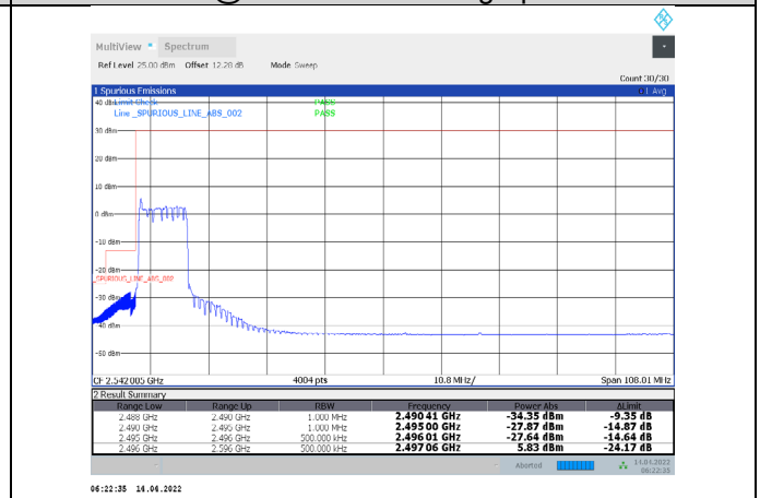
1-N41-PC3-30-100-L-21-CP-QPSK-Edge_1RB_Left-1@0-Ant1-PASS-see graph
