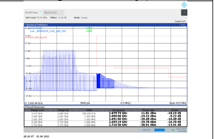
1-N41-PC3-30-20-H-28-CP-16QAM-Inner_Full-25@12-A nt1-PASS-see graph
