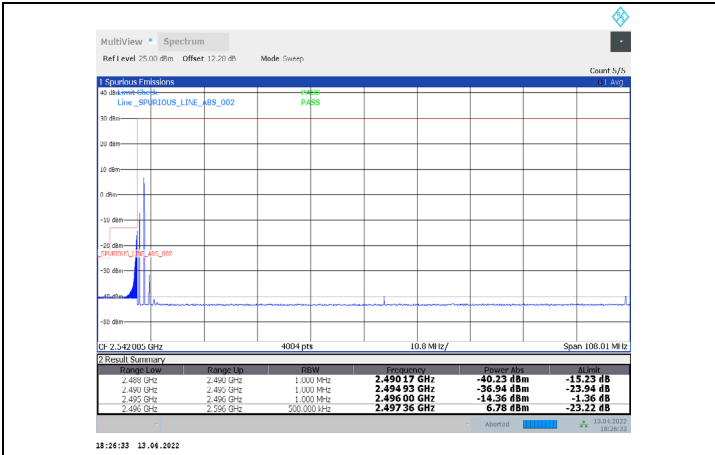
1-N41-PC3-30-100-L-33-CP-256QAM-Edge_1RB_Left-1 @0-Ant1-PASS-see graph
