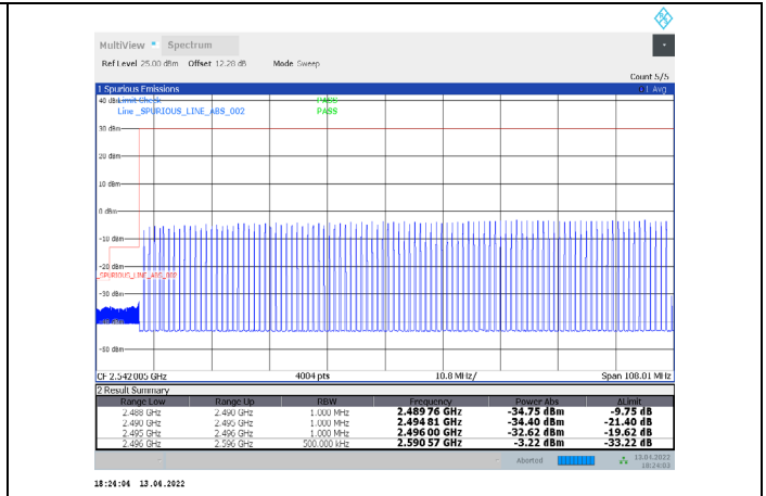
1-N41-PC3-30-100-L-27-CP-16QAM-Outer_Full-273@0 -Ant1-PASS-see graph
