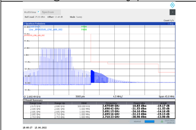
1-N41-PC3-30-20-H-24-CP-QPSK-Inner_Full-25@12-A nt1-PASS-see graph
