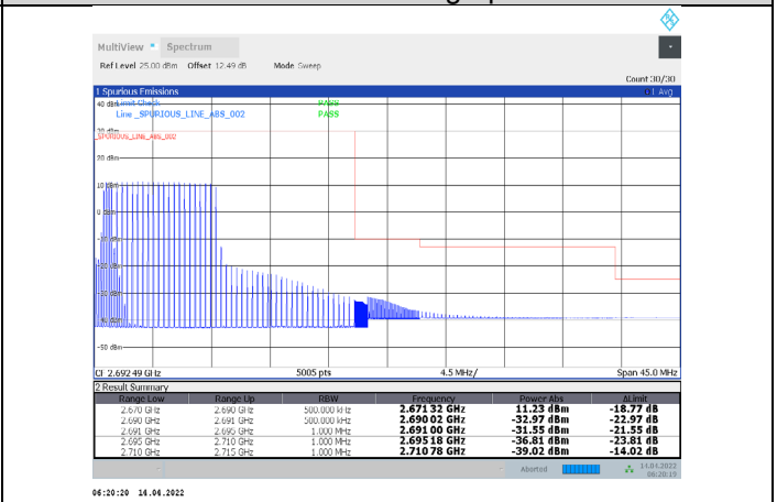
1-N41-PC3-30-20-H-34-CP-256QAM-Edge_1RB_Right-1@50-Ant1-PASS-see graph
