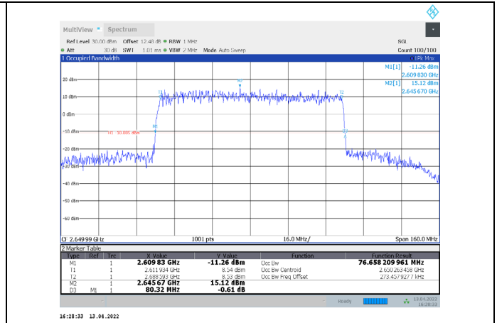
1-N41-PC3-30-80-H-2-CP-16QAM-Outer_Full-217@0-Ant1-76.658-80.320-≤80-PASS
