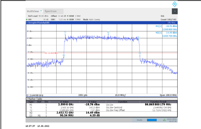
1-N41-PC3-30-90-H-3-CP-64QAM-Outer_Full-245@0-Ant 1-86.866-90.540-<=90-PASS
