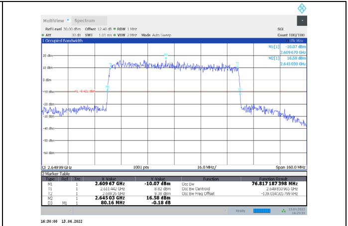
1-N41-PC3-30-80-H-8-DFT-64QAM-Outer_Full-216@0-Ant1-76.817-80.160-≤80-PASS
