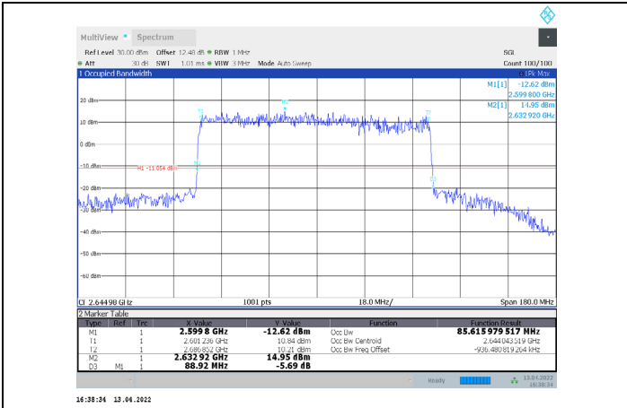
1-N41-PC3-30-90-H-7-DFT-16QAM-Outer_Full-240@0-Ant1-85.616-88.920-<=90-PASS
