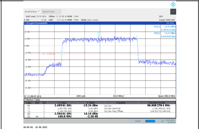
1-N41-PC3-30-100-L-4-CP-256QAM-Outer_Full-273@0-A Ant1-96.908-100.800-≤100-PASS
