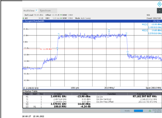
1-N41-PC3-30-100-L-3-CP-64QAM-Outer_Full-273@0-A Ant1-97.182-100.800-≤100-PASS
