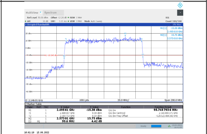
1-N41-PC3-30-100-L-6-DFT-QPSK-Outer_Full-270@0-A Ant1-95.746-99.600-≤100-PASS
