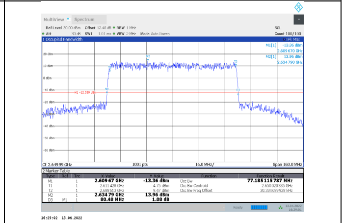
1-N41-PC3-30-80-H-4-CP-256QAM-Outer_Full-217@0-Ant1-77.185-80.480-≤80-PASS
