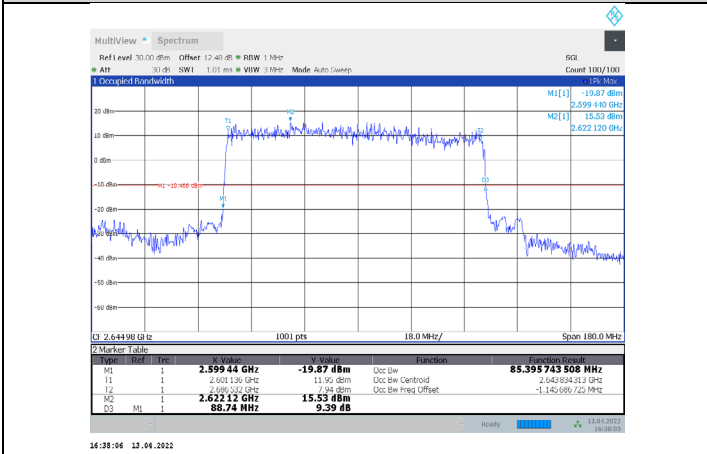
1-N41-PC3-30-90-H-5-DFT-PI/2BPSK-Outer_Full-240@0-Ant1-85.396-88.740-<=90-PASS
