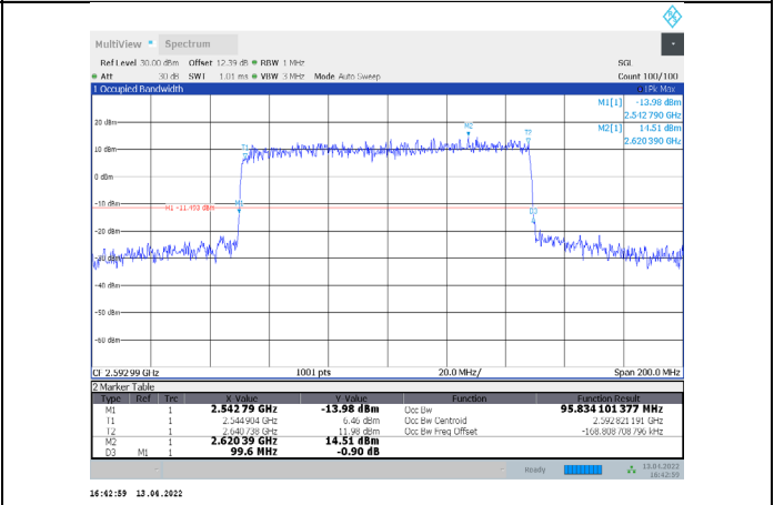
1-N41-PC3-30-100-M-1-CP-QPSK-Outer_Full-273@0-Ant1-95.834-99.600-≤100-PASS
