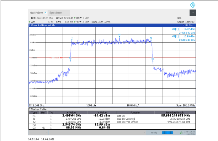
1-N41-PC3-30-90-L-5-DFT-PI/2BPSK-Outer_Full-240@0- -Ant1-85.694-88.920-≤90-PASS
