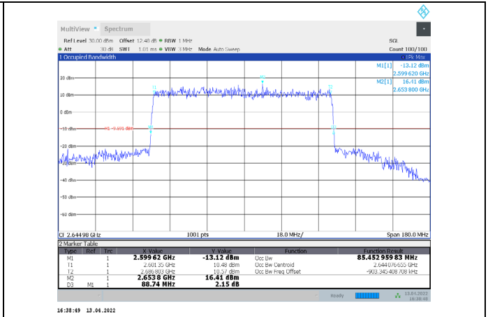
1-N41-PC3-30-90-H-8-DFT-64QAM-Outer_Full-240@0-Ant1-85.453-88.740-<=90-PASS
