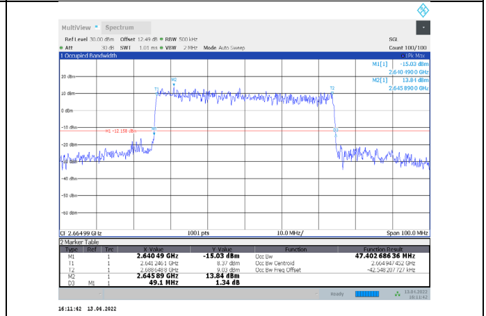
1-N41-PC3-30-50-H-4-CP-256QAM-Outer_Full-133@0-Ant1 -Ant1-47.403-49.100-≤50-PASS
