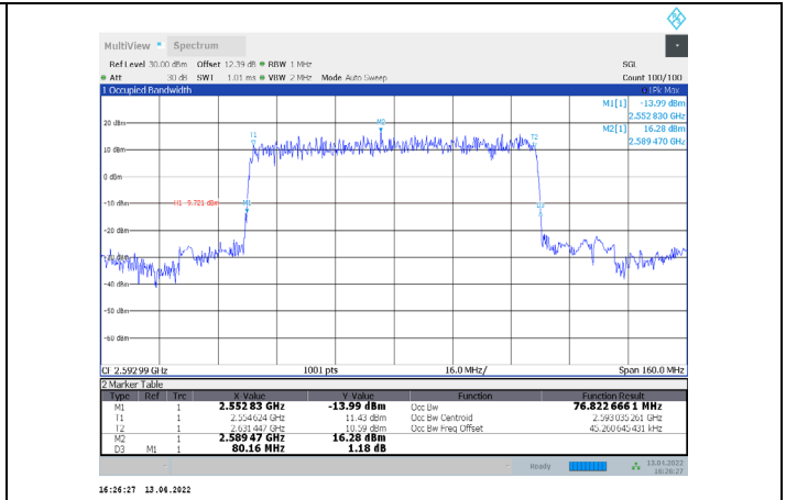
1-N41-PC3-30-80-M-5-DFT-PI/2BPSK-Outer_Full-216@0-Ant1-76.823-80.160-≤80-PASS
