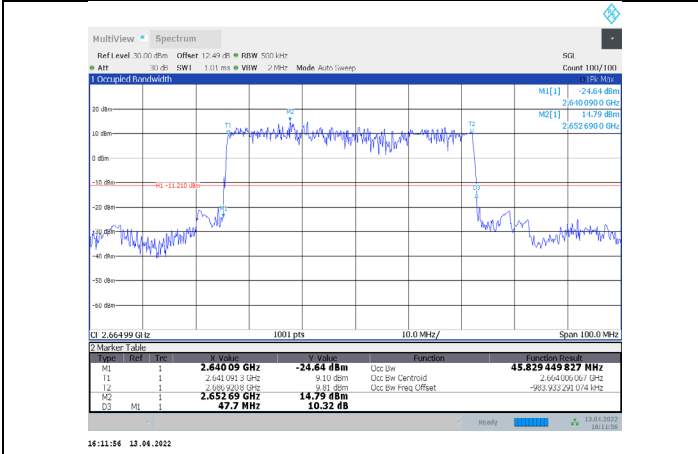
1-N41-PC3-30-50-H-5-DFT-PI/2BPSK-Outer_Full-128@0-Ant1 -Ant1-45.829-47.700-≤50-PASS
