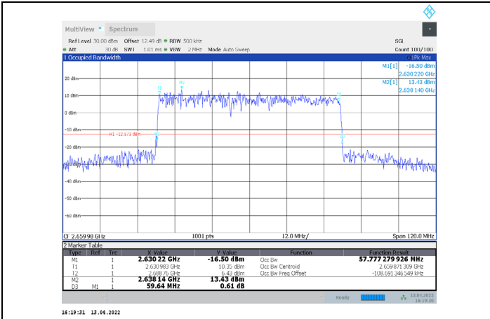
1-N41-PC3-30-60-H-1-CP-QPSK-Outer_Full-162@0-Ant 1-57.777-59.640-≤60-PASS
