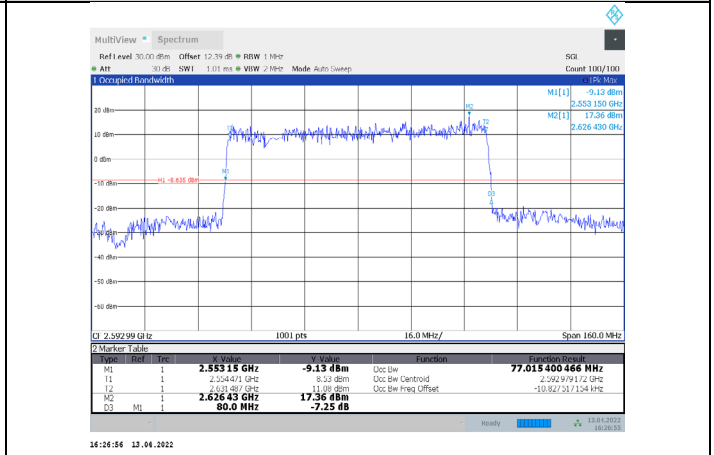
1-N41-PC3-30-80-M-7-DFT-16QAM-Outer_Full-216@0-Ant1-77.015-80.000-≤80-PASS
