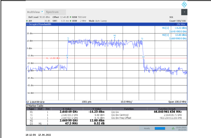
1-N41-PC3-30-50-H-9-DFT-256QAM-Outer_Full-128@0-Ant1-46.041-47.300-≤50-PASS
