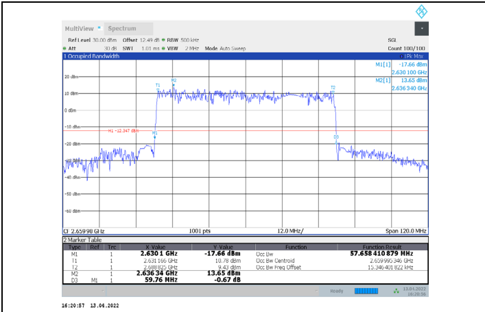
1-N41-PC3-30-60-H-7-DFT-16QAM-Outer_Full-162@0-A nt1-57.658-59.760-≤60-PASS
