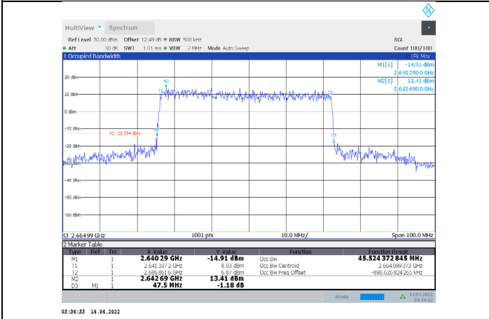
1-N41-PC3-30-50-H-3-CP-64QAM-Outer_Full-133@0-Ant1 -Ant1-45.524-47.500-≤50-PASS
