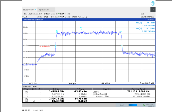
1-N41-PC3-30-80-L-3-CP-64QAM-Outer_Full-217@0-Ant 1-77.113-80.320-<80-PASS
