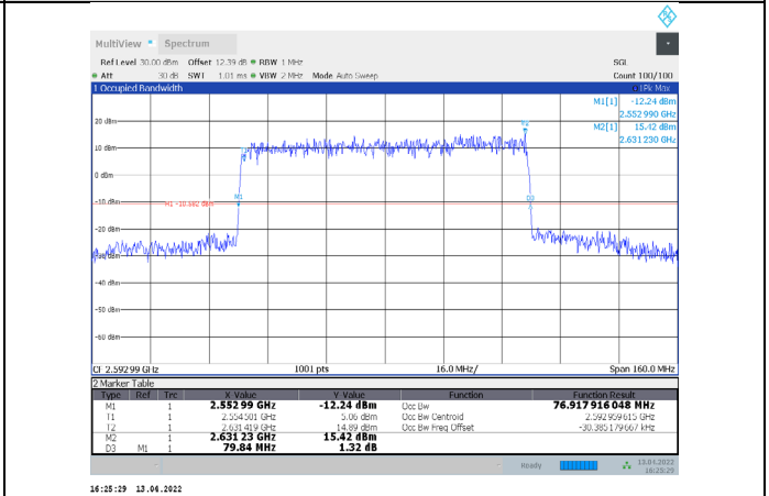
1-N41-PC3-30-80-M-1-CP-QPSK-Outer_Full-217@0-Ant1-76.918-79.840-≤80-PASS
