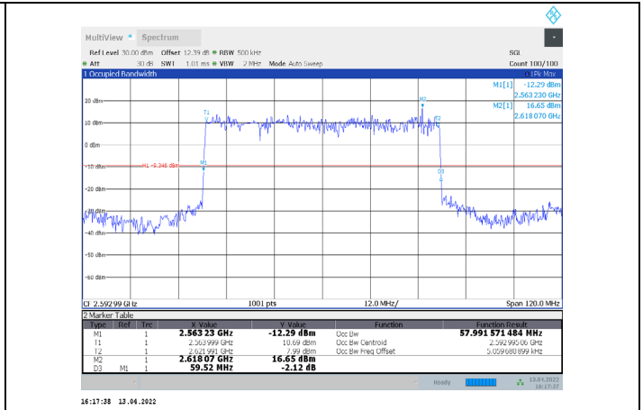
1-N41-PC3-30-60-M-5-DFT-PI/2BPSK-Outer_Full-162@0-Ant1-57.992-59.520-≤60-PASS
