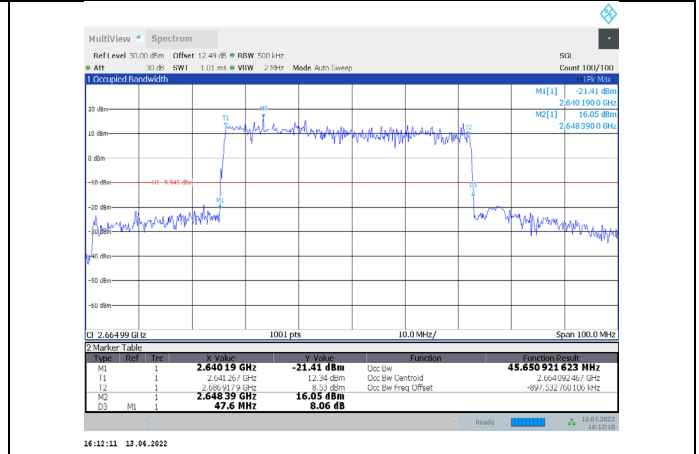
1-N41-PC3-30-50-H-6-DFT-QPSK-Outer_Full-128@0-Ant1 -Ant1-45.651-47.600-≤50-PASS
