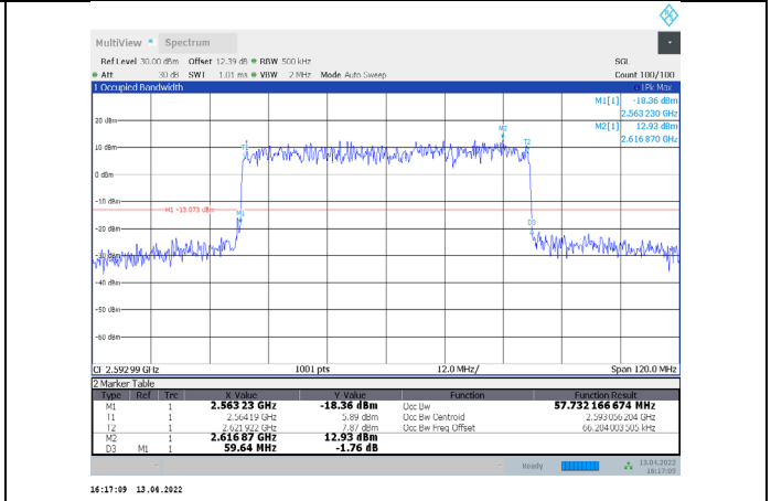
1-N41-PC3-30-60-M-3-CP-64QAM-Outer_Full-162@0-Ant1-57.732-59.640-≤60-PASS
