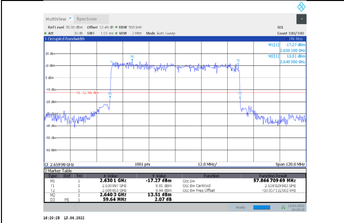
1-N41-PC3-30-60-H-5-DFT-PI/2BPSK-Outer_Full-162@0-Ant1-57.867-59.640-≤60-PASS
