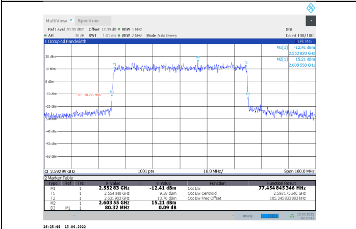
1-N41-PC3-30-80-M-2-CP-16QAM-Outer_Full-217@0-Ant1-77.455-80.320-≤80-PASS
