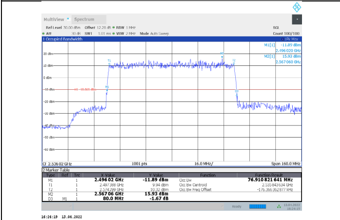
1-N41-PC3-30-80-L-9-DFT-256QAM-Outer_Full-216@0-Ant1-76.911-80.000-≤80-PASS
