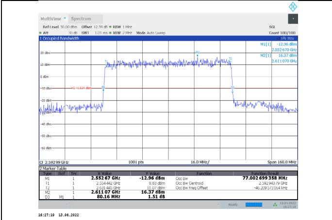
1-N41-PC3-30-80-M-8-DFT-64QAM-Outer_Full-216@0-Ant1-77.003-80.160-≤80-PASS
