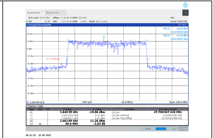
1-N41-PC3-30-50-H-2-CP-16QAM-Outer_Full-133@0-Ant1 -Ant1-47.701-49.400-≤50-PASS
