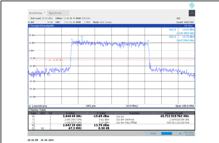
1-N41-PC3-30-50-H-1-CP-QPSK-Outer_Full-133@0-Ant 1-45.723-47.300-≤50-PASS
