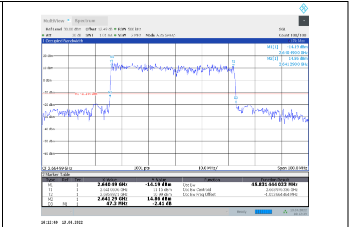
1-N41-PC3-30-50-H-8-DFT-64QAM-Outer_Full-128@0-Ant1-45.831-47.300-≤50-PASS
