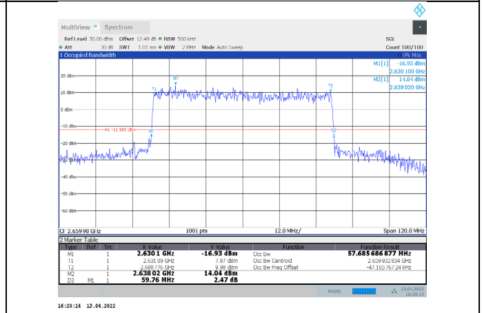
1-N41-PC3-30-60-H-4-CP-256QAM-Outer_Full-162@0-Ant1-57.686-59.760-≤60-PASS
