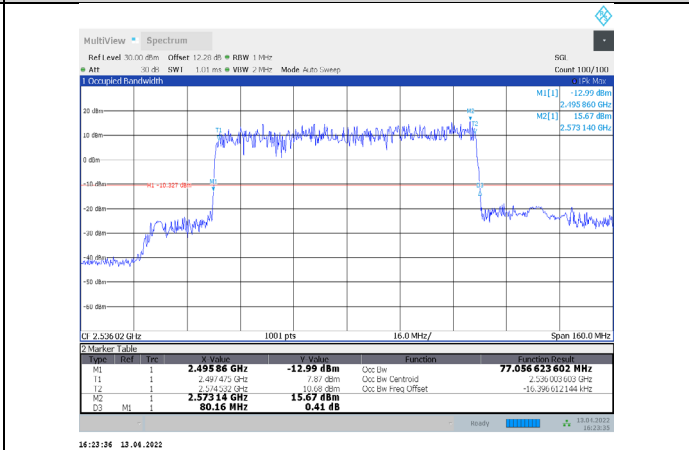
1-N41-PC3-30-80-L-6-DFT-QPSK-Outer_Full-216@0-Ant 1-77.057-80.160-<80-PASS
