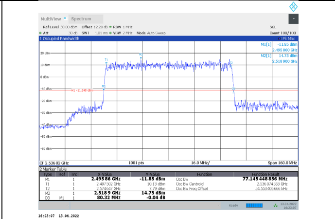
1-N41-PC3-30-80-L-4-CP-256QAM-Outer_Full-217@0-Ant 1-77.145-80.320-<80-PASS
