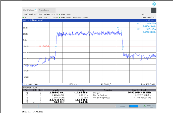
1-N41-PC3-30-80-L-5-DFT-PI/2BPSK-Outer_Full-216@0-Ant 1-76.973-80.000-<80-PASS
