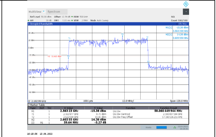
1-N41-PC3-30-60-M-9-DFT-256QAM-Outer_Full-162@0-Ant1-58.06-59.640-≤60-PASS
