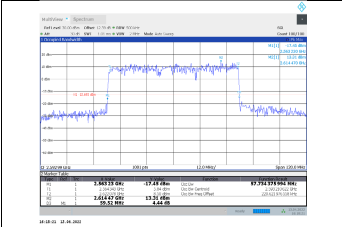
1-N41-PC3-30-60-M-8-DFT-64QAM-Outer_Full-162@0-Ant1-57.734-59.520-≤60-PASS
