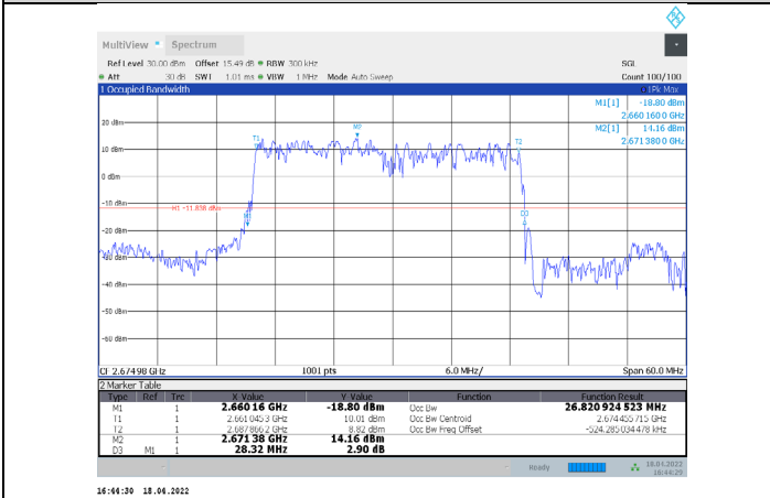
1-N41-PC3-30-30-H-5-DFT-PI/2BPSK-Outer_Full-75@0-Ant1 -26.821-28.320-≤30-PASS
