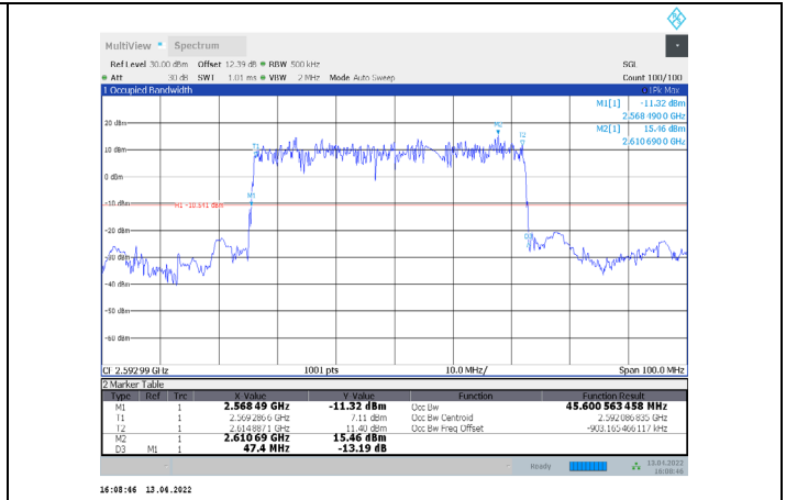
1-N41-PC3-30-50-M-5-DFT-PI/2BPSK-Outer_Full-128@0-Ant1-45.601-47.400-≤50-PASS
