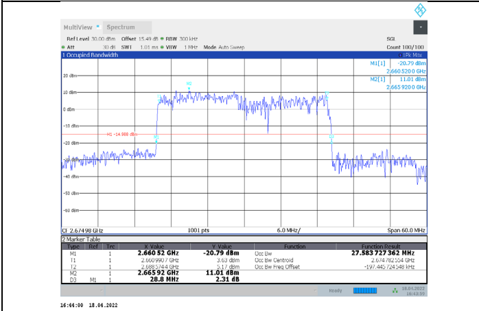
1-N41-PC3-30-30-H-3-CP-64QAM-Outer_Full-78@0-Ant1 1-27.584-28.800-≤30-PASS
