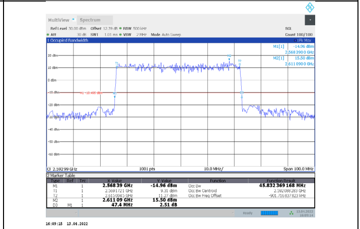
1-N41-PC3-30-50-M-7-DFT-16QAM-Outer_Full-128@0-Ant1-45.832-47.400-≤50-PASS
