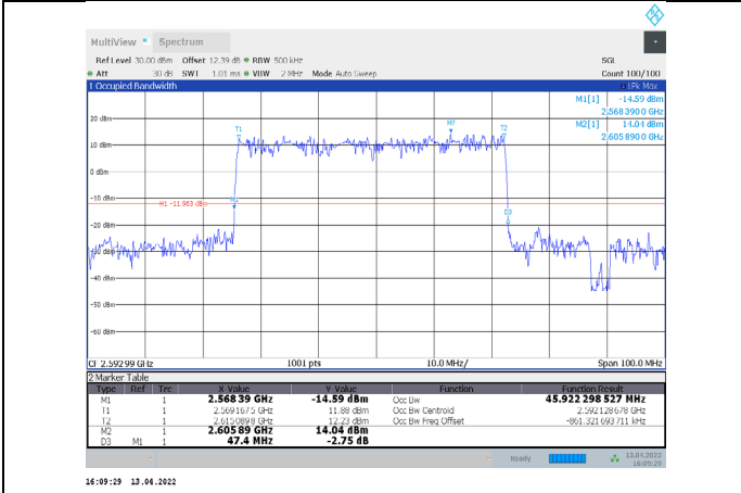
1-N41-PC3-30-50-M-8-DFT-64QAM-Outer_Full-128@0-Ant1-45.922-47.400-≤50-PASS
