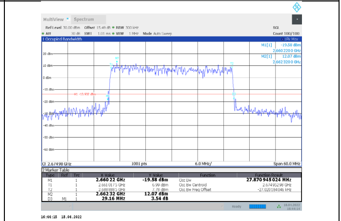
1-N41-PC3-30-30-H-4-CP-256QAM-Outer_Full-78@0-Ant1 -27.871-29.160-≤30-PASS
