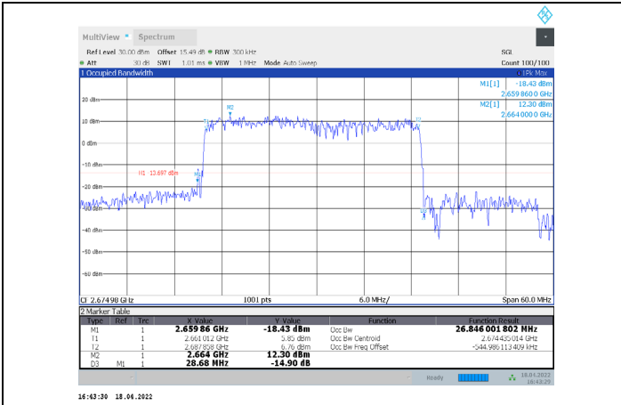
1-N41-PC3-30-30-H-1-CP-QPSK-Outer_Full-78@0-Ant1 -26.846-28.680-≤30-PASS
