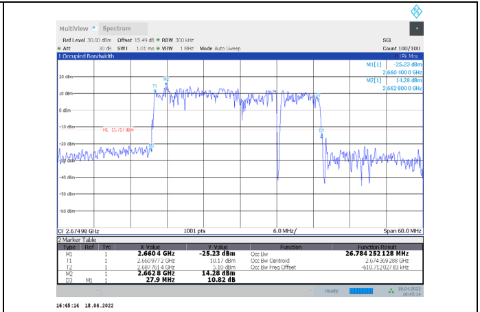
1-N41-PC3-30-30-H-8-DFT-64QAM-Outer_Full-75@0-A nt1-26.784-27.900-≤30-PASS
