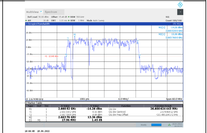
1-N41-PC3-30-30-H-6-DFT-QPSK-Outer_Full-75@0-Ant1 -26.601-27.960-≤30-PASS
