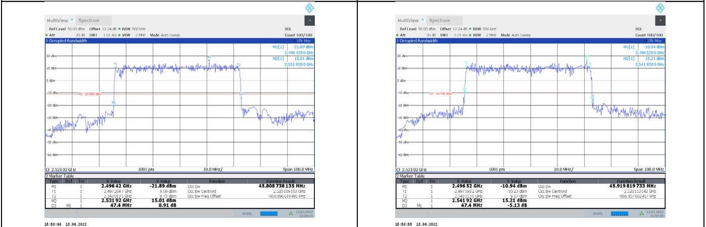
1-N41-PC3-30-50-L-5-DFT-PI/2BPSK-Outer_Full-128@0-Ant1-45.809-47.400-≤50-PASS
