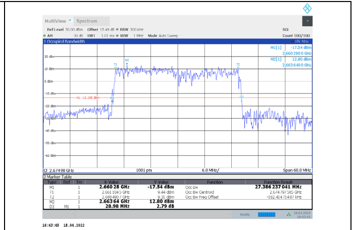
1-N41-PC3-30-30-H-2-CP-16QAM-Outer_Full-78@0-Ant1 -27.386-28.980-≤30-PASS
