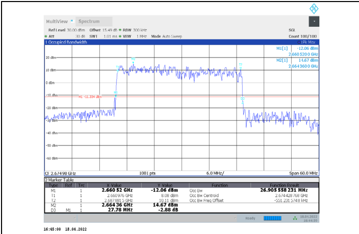
1-N41-PC3-30-30-H-7-DFT-16QAM-Outer_Full-75@0-A nt1-26.905-27.780-≤30-PASS
