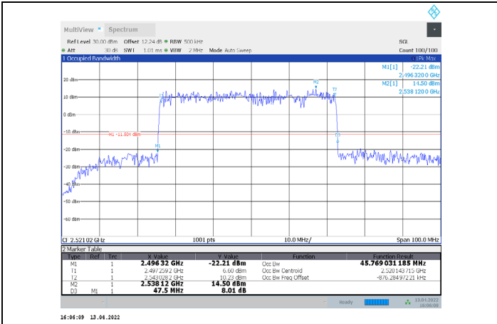
1-N41-PC3-30-50-L-7-DFT-16QAM-Outer_Full-128@0-Ant1-45.769-47.500-≤50-PASS
