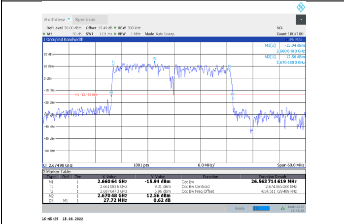
1-N41-PC3-30-30-H-9-DFT-256QAM-Outer_Full-75@0-A nt1-26.563-27.720-≤30-PASS
