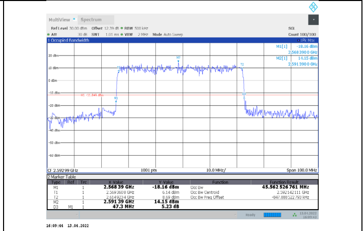
1-N41-PC3-30-50-M-9-DFT-256QAM-Outer_Full-128@0-Ant1-45.563-47.300-≤50-PASS
