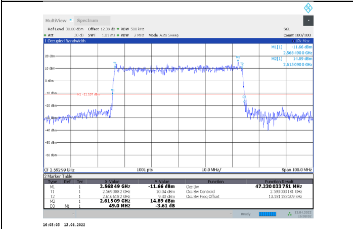
1-N41-PC3-30-50-M-2-CP-16QAM-Outer_Full-133@0-Ant1-47.23-49.000-≤50-PASS
