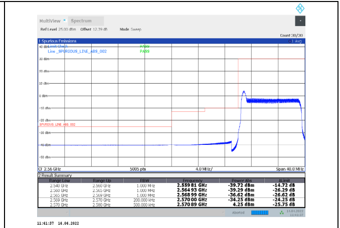
1-N38-PC3-30-10-L-35-CP-256QAM-Outer_Full-24@0-Ant1-PASS-see graph
