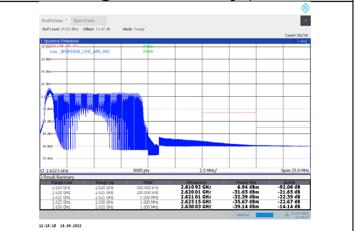
1-N38-PC3-30-10-H-20-DFT-256QAM-Inner_Full-12@6-Ant1-PASS-see graph
