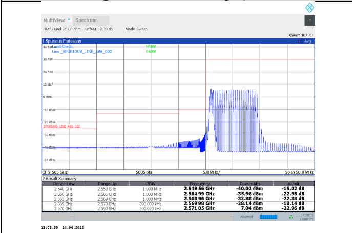
1-N38-PC3-30-20-L-12-DFT-16QAM-Inner_Full-25@12-Ant1-PASS-see graph
