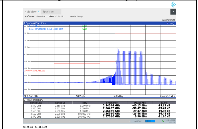
1-N38-PC3-30-20-L-24-CP-QPSK-Inner_Full-25@12-Ant1-PASS-see graph
