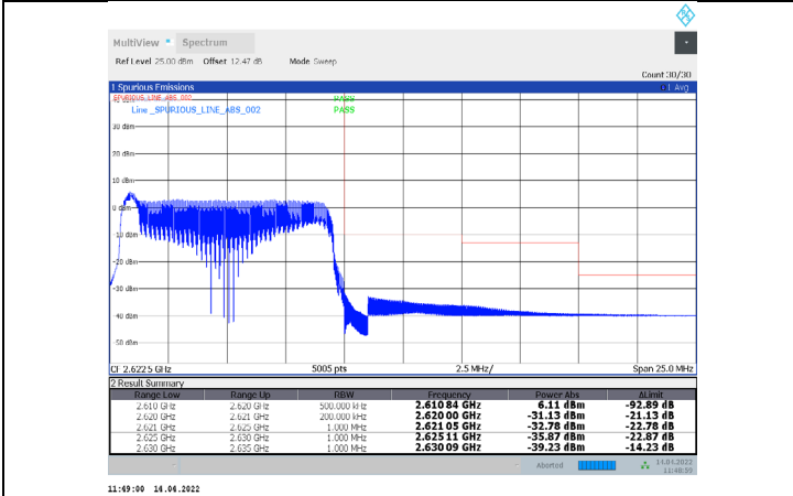
1-N38-PC3-30-10-H-3-DFT-PI/2BPSK-Edge_1RB_Right-1@23-Ant1-PASS-see graph
