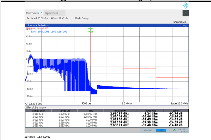
1-N38-PC3-30-10-H-32-CP-64QAM-Inner_Full-12@6-Ant1-PASS-see graph
