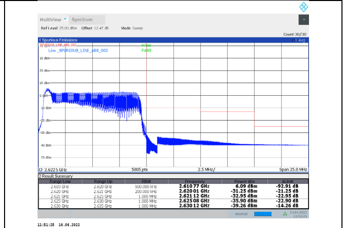
1-N38-PC3-30-10-H-4-DFT-PI/2BPSK-Outer_Full-24@0-Ant1-PASS-see graph
