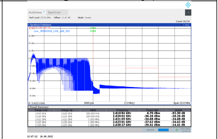
1-N38-PC3-30-10-H-36-CP-256QAM-Inner_Full-12@6-Ant1-PASS-see graph
