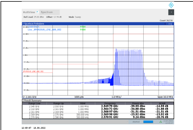
1-N38-PC3-30-20-L-1-DFT-PI/2BPSK-Inner_Full-25@12-Ant1-PASS-see graph
