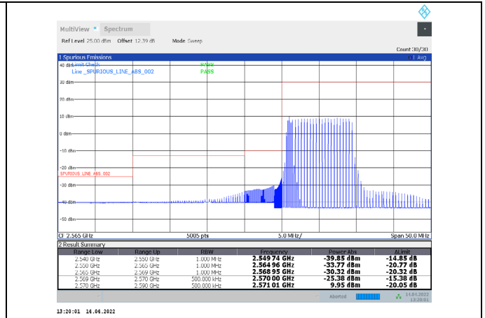
1-N38-PC3-30-20-L-19-DFT-256QAM-Outer_Full-50@0-Ant1-PASS-see graph
