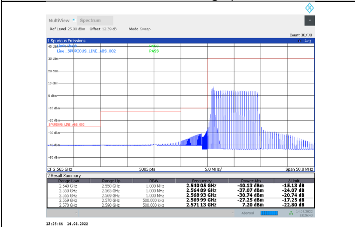
1-N38-PC3-30-20-L-23-CP-QPSK-Outer_Full-51@0-Ant1-PASS-see graph
