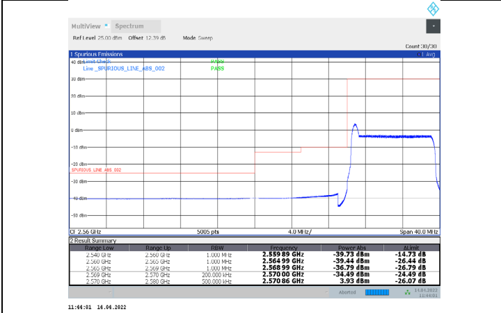
1-N38-PC3-30-10-L-36-CP-256QAM-Inner_Full-12@6-Ant1-PASS-see graph
