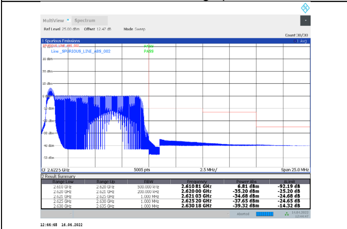
1-N38-PC3-30-10-H-35-CP-256QAM-Outer_Full-24@0-Ant1-PASS-see graph
