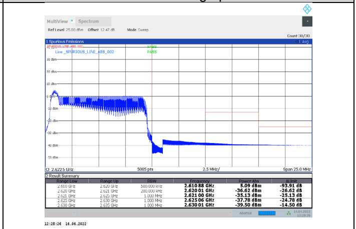
1-N38-PC3-30-10-H-26-CP-16QAM-Edge_1RB_Right-1 @23-Ant1-PASS-see graph
