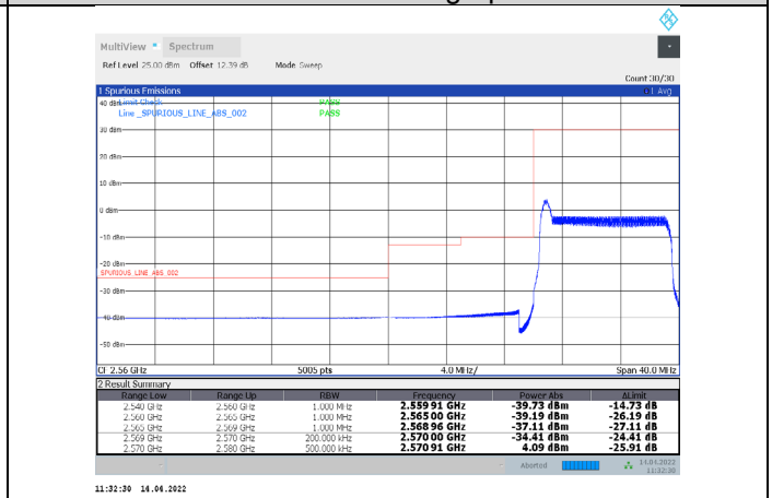
1-N38-PC3-30-10-L-29-CP-64QAM-Edge_1RB_Left-1 @0-Ant1-PASS-see graph
