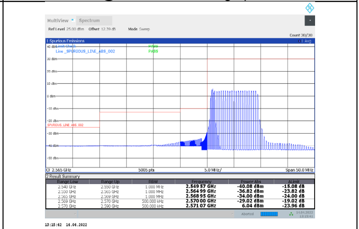
1-N38-PC3-30-20-L-16-DFT-64QAM-Inner_Full-25@12-Ant1-PASS-see graph
