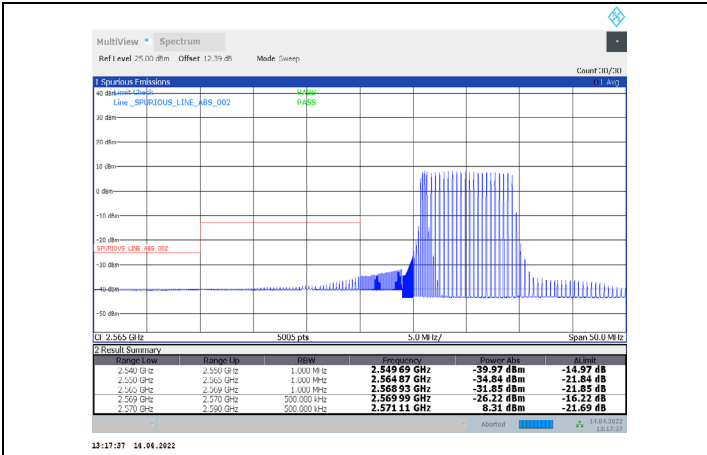
1-N38-PC3-30-20-L-17-DFT-256QAM-Edge_1RB_Left-1@0-Ant1-PASS-see graph
