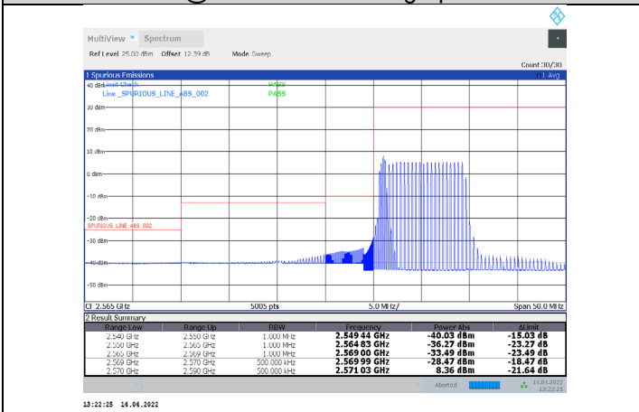
1-N38-PC3-30-20-L-20-DFT-256QAM-Inner_Full-25@12-Ant1-PASS-see graph
