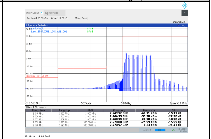
1-N38-PC3-30-20-L-21-CP-QPSK-Edge_1RB_Left-1@0-Ant1-PASS-see graph
