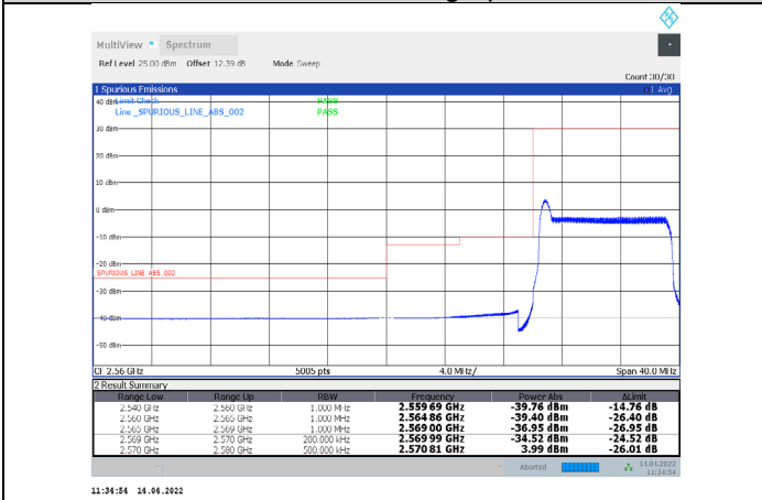
1-N38-PC3-30-10-L-31-CP-64QAM-Outer_Full-24@0-Ant1-PASS-see graph
