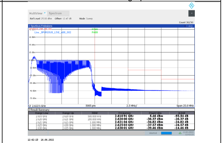
1-N38-PC3-30-10-H-34-CP-256QAM-Edge_1RB_Right-1@23-Ant1-PASS-see graph
