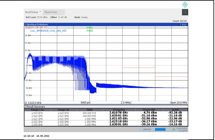
1-N38-PC3-30-10-H-15-DFT-64QAM-Outer_Full-24@0-Ant1-PASS-see graph
