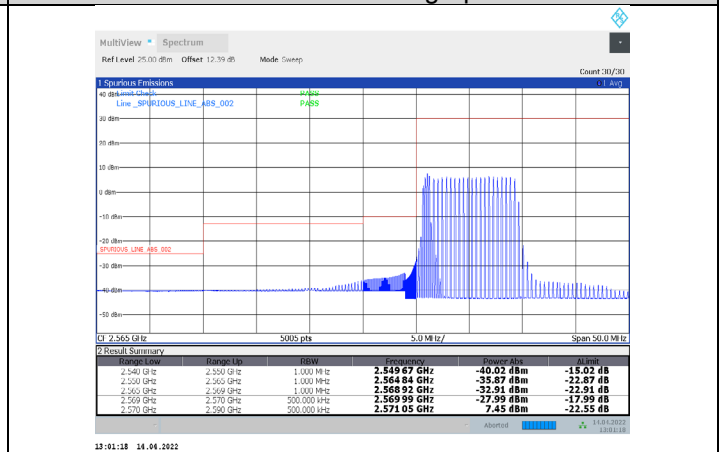
1-N38-PC3-30-20-L-8-DFT-QPSK-Inner_Full-25@12-Ant1-PASS-see graph
