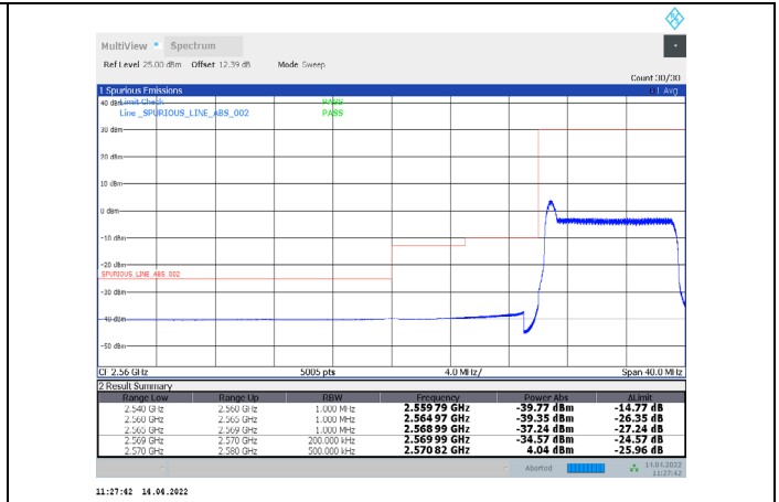
1-N38-PC3-30-10-L-27-CP-16QAM-Outer_Full-24@0-Ant1-PASS-see graph
