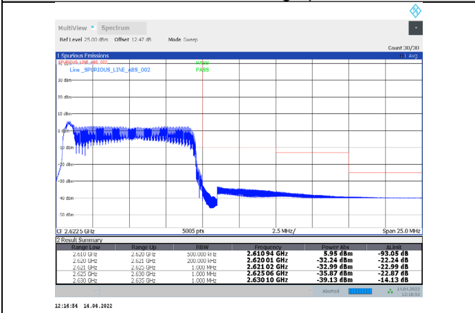
1-N38-PC3-30-10-H-19-DFT-256QAM-Outer_Full-24@0-Ant1-PASS-see graph
