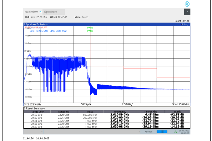
1-N38-PC3-30-10-H-1-DFT-PI/2BPSK-Inner_Full-12@6-Ant1-PASS-see graph
