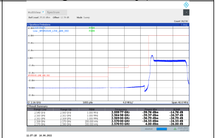
1-N38-PC3-30-10-L-32-CP-64QAM-Inner_Full-12@6-Ant1-PASS-see graph
