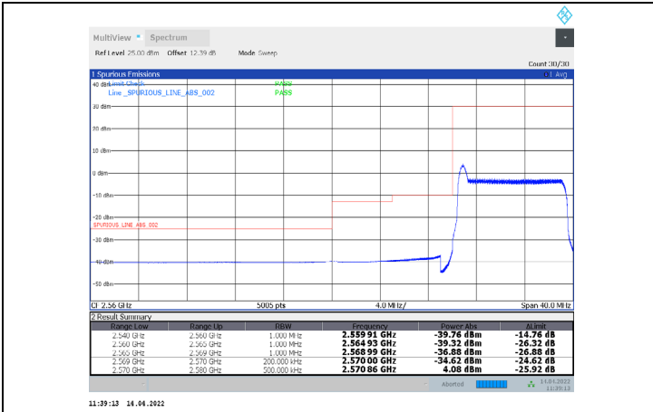
1-N38-PC3-30-10-L-33-CP-256QAM-Edge_1RB_Left-1@0-Ant1-PASS-see graph
