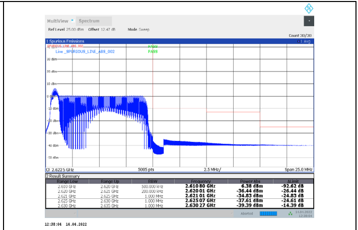
1-N38-PC3-30-10-H-31-CP-64QAM-Outer_Full-24@0-Ant1-PASS-see graph
