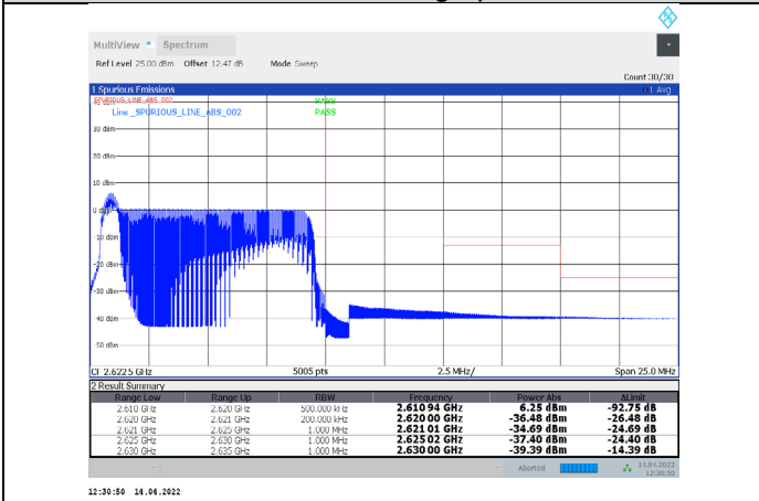
1-N38-PC3-30-10-H-27-CP-16QAM-Outer_Full-24@0-Ant1-PASS-see graph
