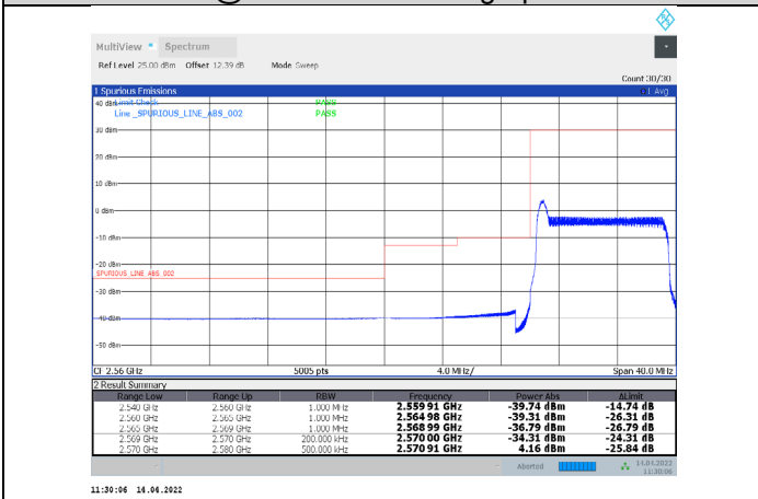
1-N38-PC3-30-10-L-28-CP-16QAM-Inner_Full-12@6-Ant1-PASS-see graph
