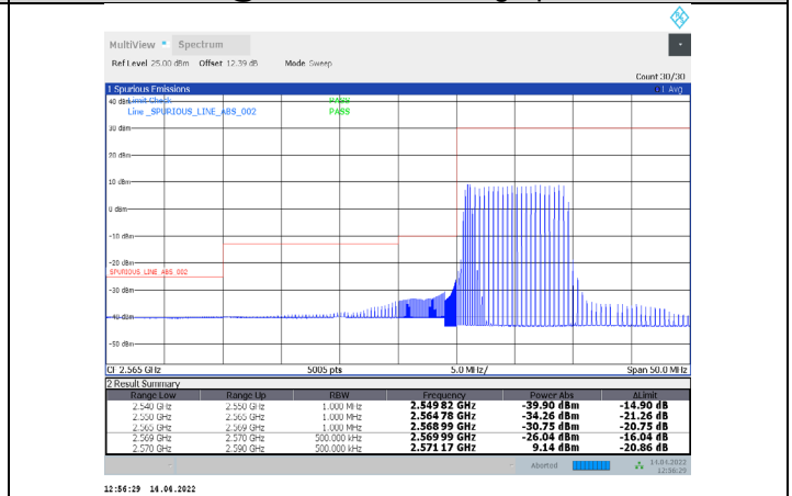
1-N38-PC3-30-20-L-5-DFT-QPSK-Edge_1RB_Left-1@0-Ant1-PASS-see graph
