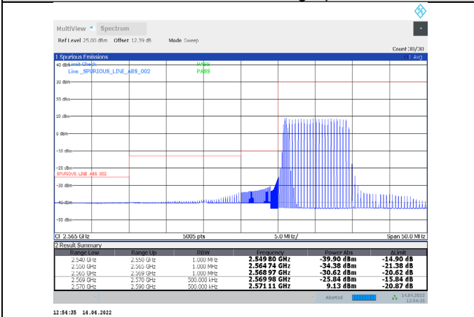
1-N38-PC3-30-20-L-4-DFT-PI/2BPSK-Outer_Full-50@0-Ant1-PASS-see graph
