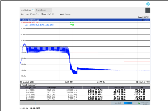
1-N38-PC3-30-10-H-30-CP-64QAM-Edge_1RB_Right-1@23-Ant1-PASS-see graph
