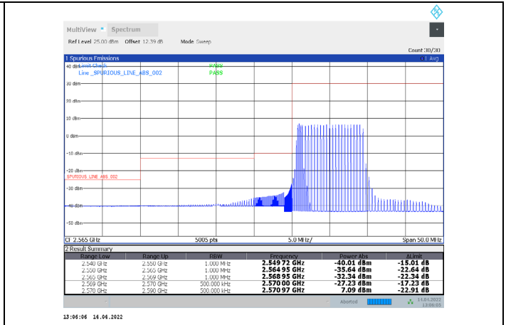
1-N38-PC3-30-20-L-11-DFT-16QAM-Outer_Full-50@0-Ant1-PASS-see graph
