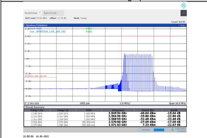
1-N38-PC3-30-20-L-7-DFT-QPSK-Outer_Full-50@0-Ant1-PASS-see graph
