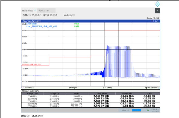
1-N38-PC3-30-20-L-15-DFT-64QAM-Outer_Full-50@0-Ant1-PASS-see graph
