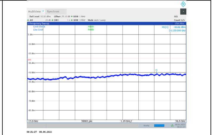
1-N7-PC3-15-15-H-2-CP-QPSK-Edge_1RB_Right-1@7 8-12000-26900-Ant1--40.66--25-PASS
