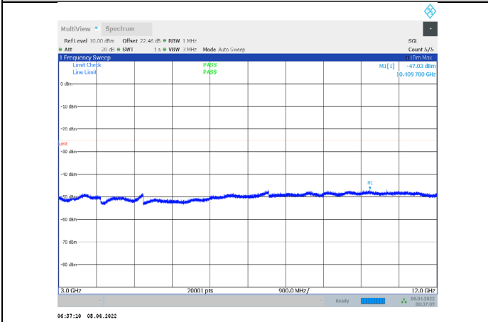
1-N7-PC3-15-20-L-3-CP-QPSK-Outter_Full-106@0-300- 0-12000-Ant1--47.03--25-PASS
