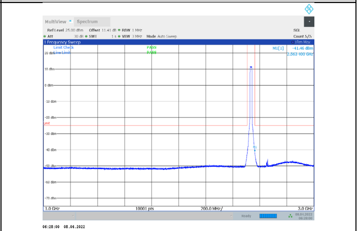
1-N7-PC3-15-15-M-3-CP-QPSK-Outter_Full-79@0-1000- 3000-Ant1--41.46--25-PASS
