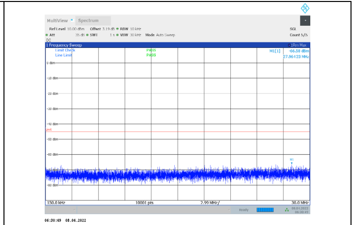
1-N7-PC3-15-15-H-2-CP-QPSK-Edge_1RB_Right-1@7 8-0.15-30-Ant1--66.58--45-PASS
