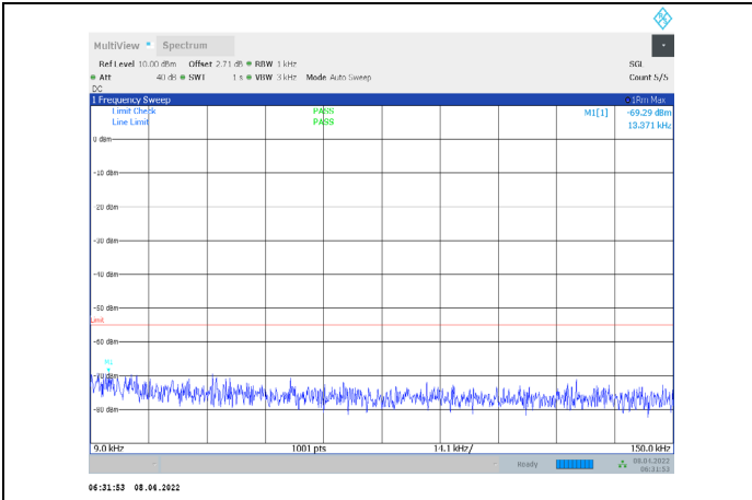
1-N7-PC3-15-15-H-3-CP-QPSK-Outter_Full-79@0-0.00 9-0.15-Ant1--69.29--55-PASS
