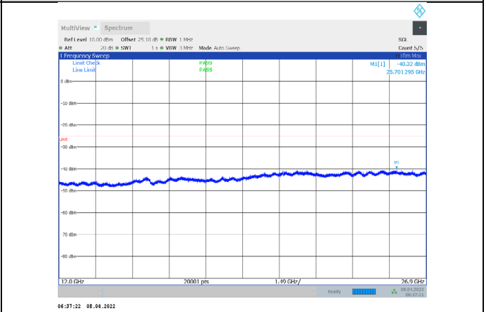
1-N7-PC3-15-20-L-3-CP-QPSK-Outter_Full-106@0-1200- 0-26900-Ant1--40.32--25-PASS
