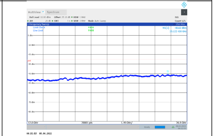
1-N7-PC3-15-15-H-3-CP-QPSK-Outter_Full-79@0-1200 0-26900-Ant1--40.63--25-PASS
