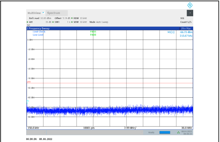
1-N7-PC3-15-20-L-3-CP-QPSK-Outter_Full-106@0-0.15- 30-Ant1--66.73--45-PASS
