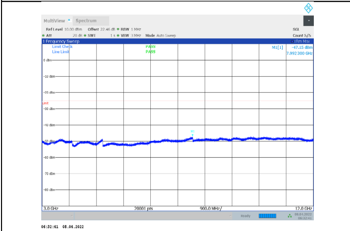
1-N7-PC3-15-15-H-3-CP-QPSK-Outter_Full-79@0-3000 -12000-Ant1--47.15--25-PASS
