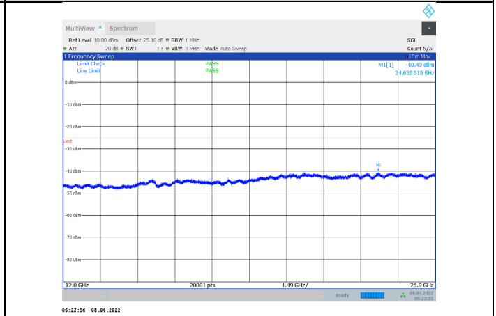
1-N7-PC3-15-15-L-3-CP-QPSK-Outer_Full-79@0-12000 -26900-Ant1--40.49--25-PASS
