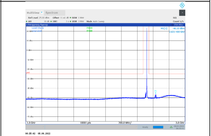
1-N7-PC3-15-20-L-2-CP-QPSK-Edge_1RB_Right-1@1 5-1000-3000-Ant1--46.10--25-PASS
