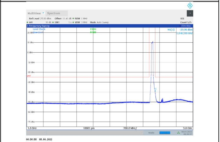
1-N7-PC3-15-20-L-3-CP-QPSK-Outter_Full-106@0-1000- 3000-Ant1--39.96--25-PASS
