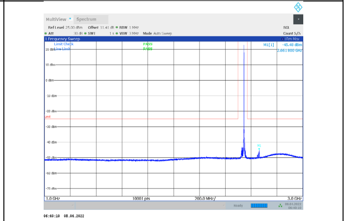
1-N7-PC3-15-20-M-2-CP-QPSK-Edge_1RB_Right-1@1 05-1000-3000-Ant1--45.48--25-PASS
