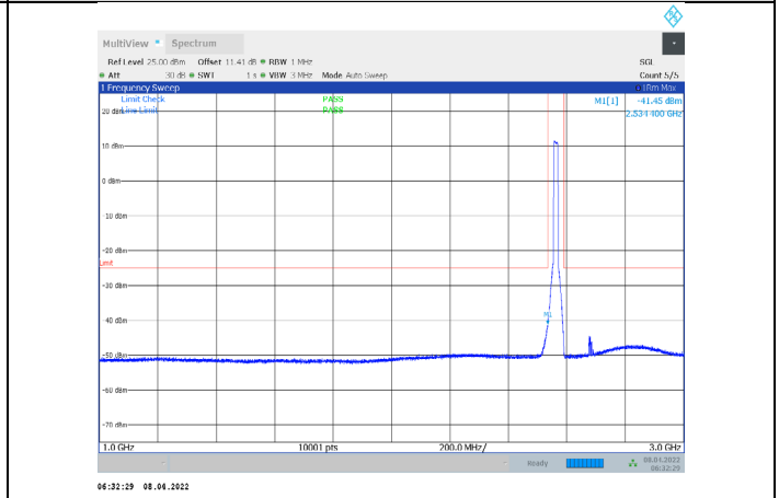
1-N7-PC3-15-15-H-3-CP-QPSK-Outter_Full-79@0-1000- 3000-Ant1--41.45--25-PASS
