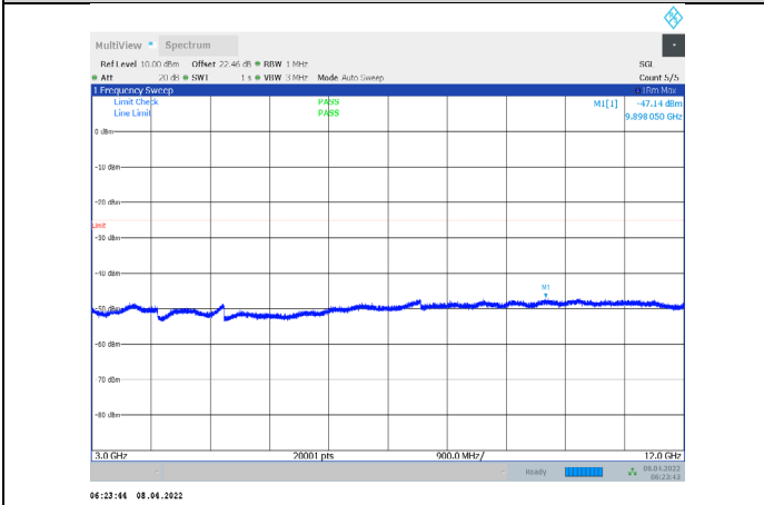
1-N7-PC3-15-15-L-3-CP-QPSK-Outer_Full-79@0-3000 -12000-Ant1--47.14--25-PASS
