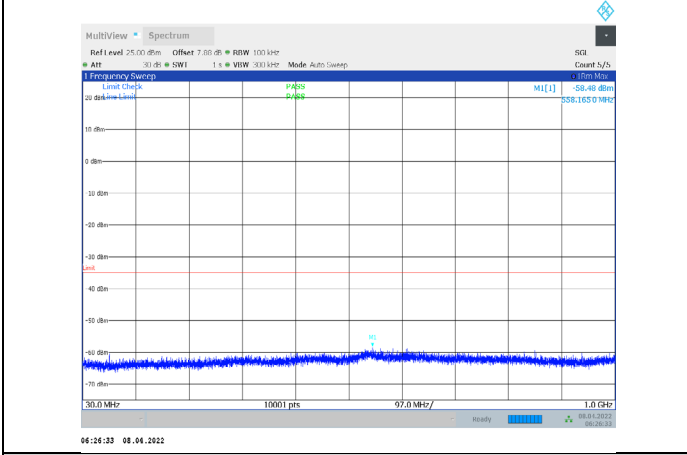
1-N7-PC3-15-15-M-2-CP-QPSK-Edge_1RB_Right-1@7 8-30-1000-Ant1--58.48--35-PASS
