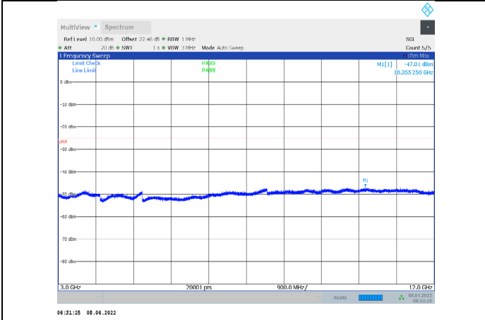
1-N7-PC3-15-15-H-2-CP-QPSK-Edge_1RB_Right-1@7 8-3000-12000-Ant1--47.01--25-PASS
