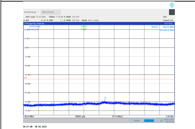
1-N7-PC3-15-15-M-3-CP-QPSK-Outter_Full-79@0-30-1 000-Ant1--58.75--35-PASS
