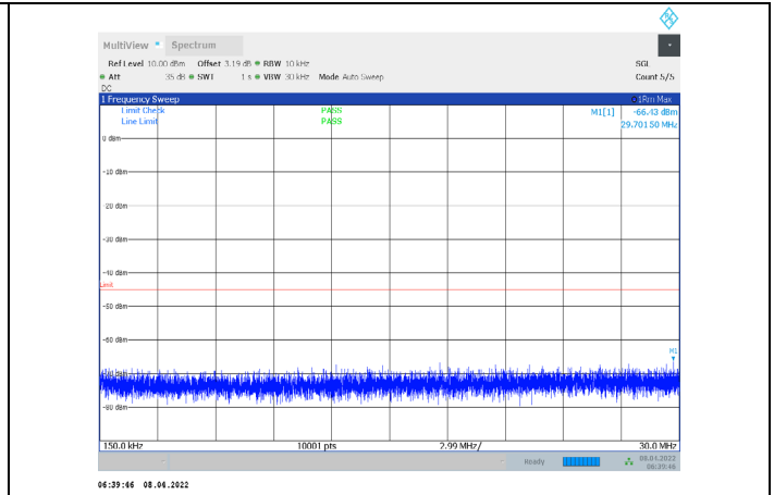
1-N7-PC3-15-20-M-2-CP-QPSK-Edge_1RB_Right-1@1 05-0.15-30-Ant1--66.43--45-PASS
