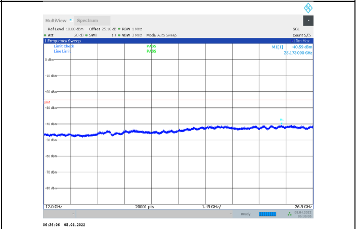
1-N7-PC3-15-20-L-2-CP-QPSK-Edge_1RB_Right-1@1 5-12000-26900-Ant1--40.59--25-PASS
