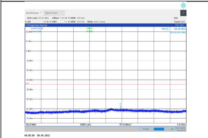
1-N7-PC3-15-20-L-2-CP-QPSK-Edge_1RB_Right-1@1 05-30-1000-Ant1--58.38--35-PASS
