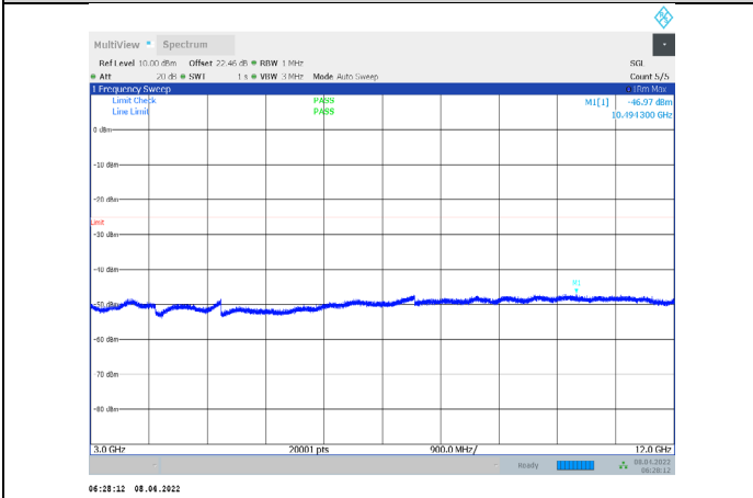
1-N7-PC3-15-15-M-3-CP-QPSK-Outter_Full-79@0-300 0-12000-Ant1--46.97--25-PASS
