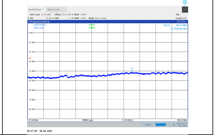
1-N7-PC3-15-15-M-2-CP-QPSK-Edge_1RB_Right-1@7 8-12000-26900-Ant1--40.47--25-PASS
