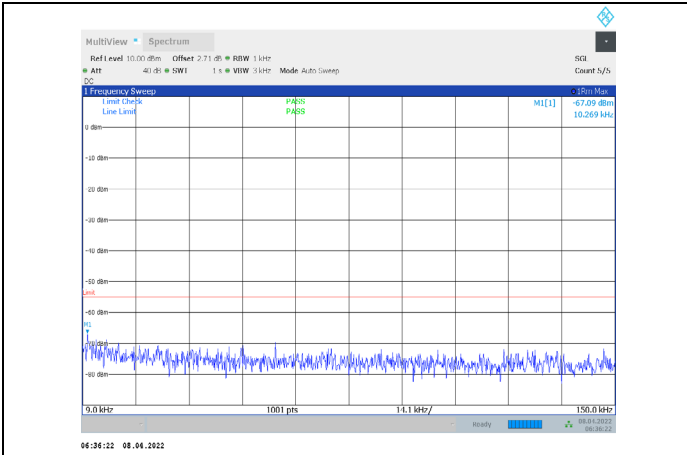
1-N7-PC3-15-20-L-3-CP-QPSK-Outter_Full-106@0-0.0 09-0.15-Ant1--67.09--55-PASS
