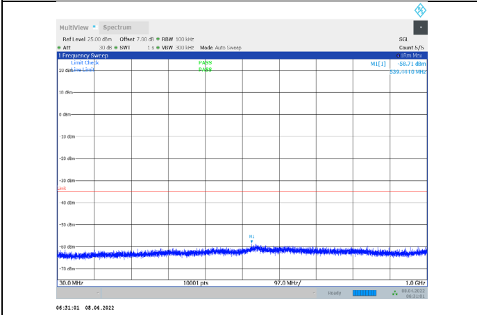
1-N7-PC3-15-15-H-2-CP-QPSK-Edge_1RB_Right-1@7 8-30-1000-Ant1--58.71--35-PASS
