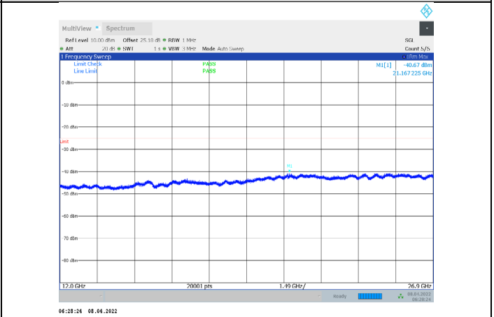
1-N7-PC3-15-15-M-3-CP-QPSK-Outter_Full-79@0-1200 0-26900-Ant1--40.67--25-PASS
