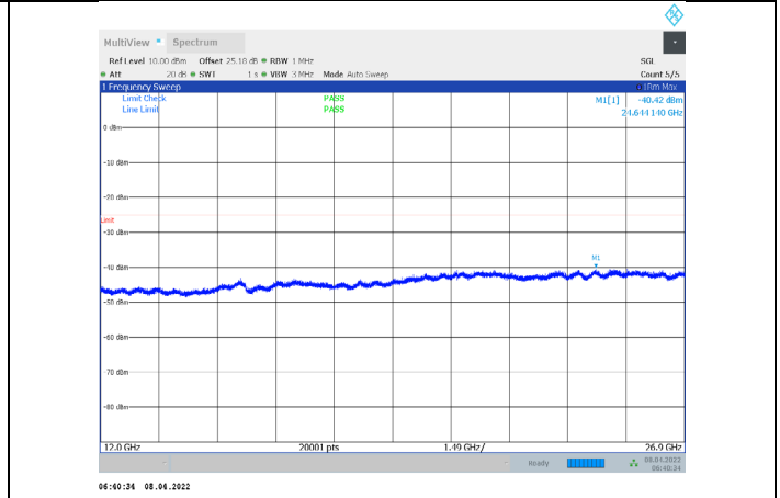
1-N7-PC3-15-20-M-2-CP-QPSK-Edge_1RB_Right-1@1 05-12000-26900-Ant1--40.42--25-PASS
