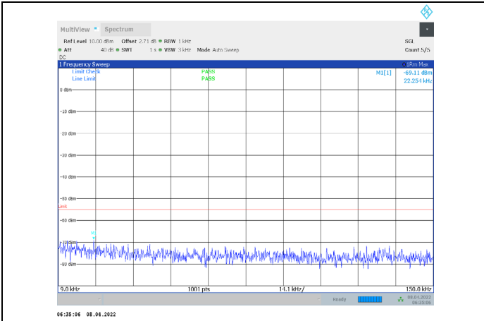
1-N7-PC3-15-20-L-2-CP-QPSK-Edge_1RB_Right-1@1 05-0-009-0.15-Ant1--69.11--55-PASS
