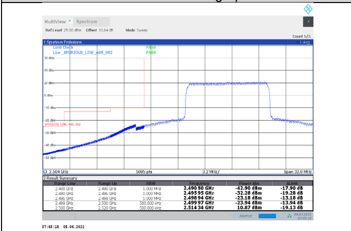
1-N7-PC3-15-20-L-28-CP-16QAM-Inner_Full-53@26-Ant1-PASS-see graph
