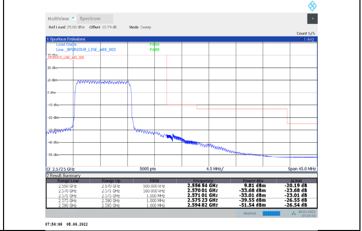
1-N7-PC3-15-20-H-20-DFT-256QAM-Inner_Full-50@25-Ant1-PASS-see graph
