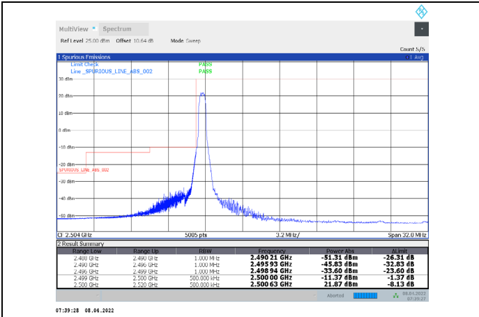
1-N7-PC3-15-20-L-9-DFT-16QAM-Edge_1RB_Left-1@0-Ant1-PASS-see graph
