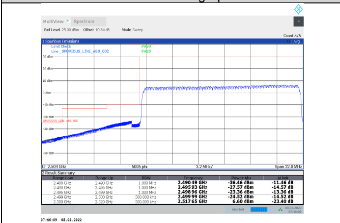
1-N7-PC3-15-20-L-31-CP-64QAM-Outer_Full-106@0-Ant1-PASS-see graph
