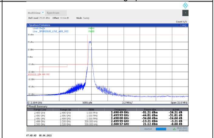
1-N7-PC3-15-20-L-29-CP-64QAM-Edge_1RB_Left-1@0-Ant1-PASS-see graph
