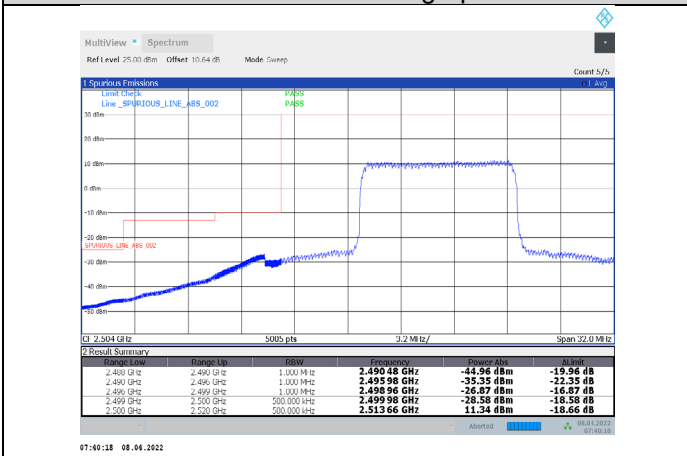
1-N7-PC3-15-20-L-12-DFT-16QAM-Inner_Full-50@25-Ant1-PASS-see graph
