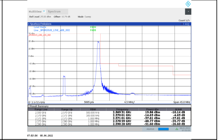
1-N7-PC3-15-20-H-18-DFT-256QAM-Edge_1RB_Right-1@105-Ant1-PASS-see graph
