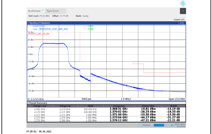
1-N7-PC3-15-5-H-36-CP-256QAM-Inner_Full-13@6-Ant1-PASS-see graph
