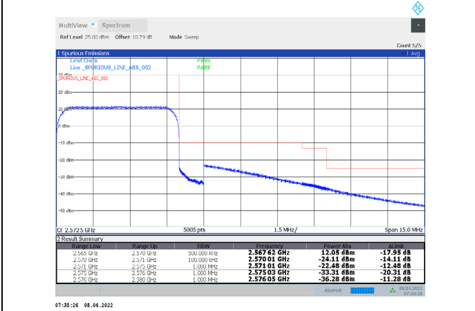
1-N7-PC3-15-5-H-35-CP-256QAM-Outer_Full-25@0-Ant1-PASS-see graph
