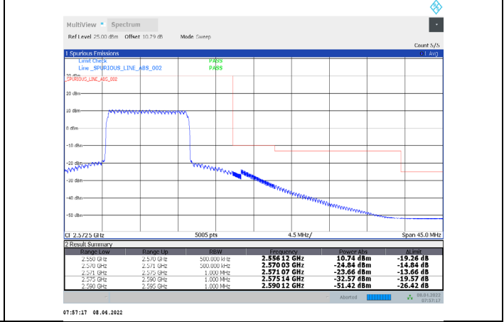
1-N7-PC3-15-20-H-28-CP-16QAM-Inner_Full-53@26-Ant1-PASS-see graph
