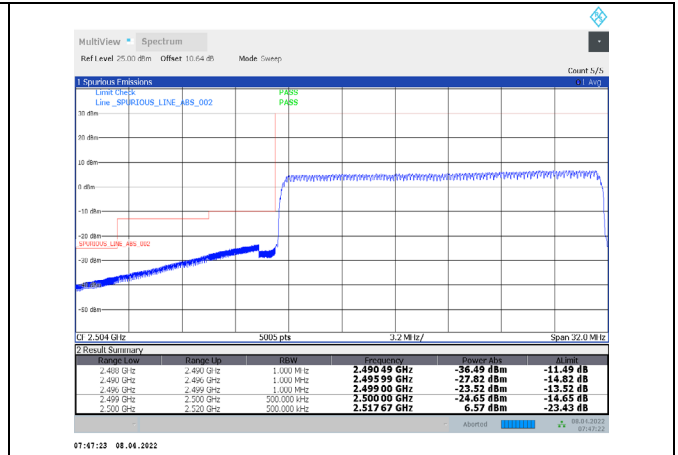
1-N7-PC3-15-20-L-35-CP-256QAM-Outer_Full-106@0-Ant1-PASS-see graph
