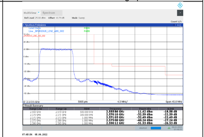
1-N7-PC3-15-20-H-1-DFT-PI/2BPSK-Inner_Full-50@25-Ant1-PASS-see graph
