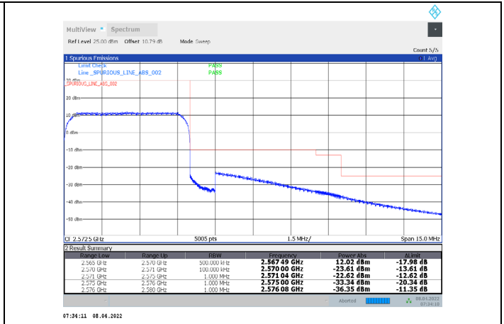
1-N7-PC3-15-5-H-31-CP-64QAM-Outer_Full-25@0-Ant1-PASS-see graph
