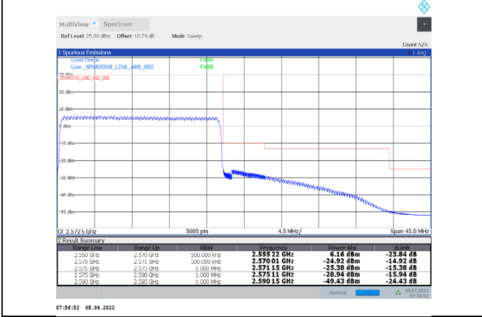
1-N7-PC3-15-20-H-27-CP-16QAM-Outer_Full-106@0-Ant1-PASS-see graph
