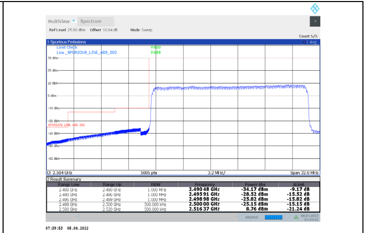
1-N7-PC3-15-20-L-11-DFT-16QAM-Outer_Full-100@0-Ant1-PASS-see graph
