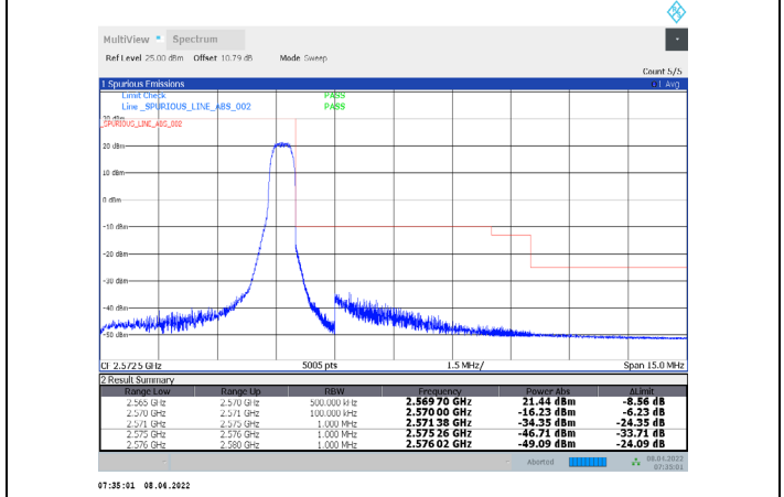
1-N7-PC3-15-5-H-34-CP-256QAM-Edge_1RB_Right-1@24-Ant1-PASS-see graph
