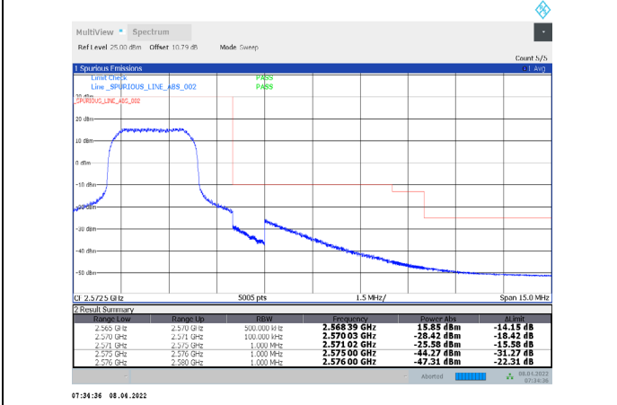
1-N7-PC3-15-5-H-32-CP-64QAM-Inner_Full-13@6-Ant1-PASS-see graph
