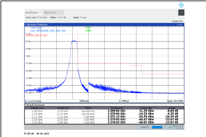
1-N7-PC3-15-5-H-30-CP-64QAM-Edge_1RB_Right-1@24-Ant1-PASS-see graph
