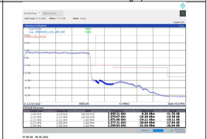
1-N7-PC3-15-20-H-4-DFT-PI/2BPSK-Outer_Full-100@0-Ant1-PASS-see graph
