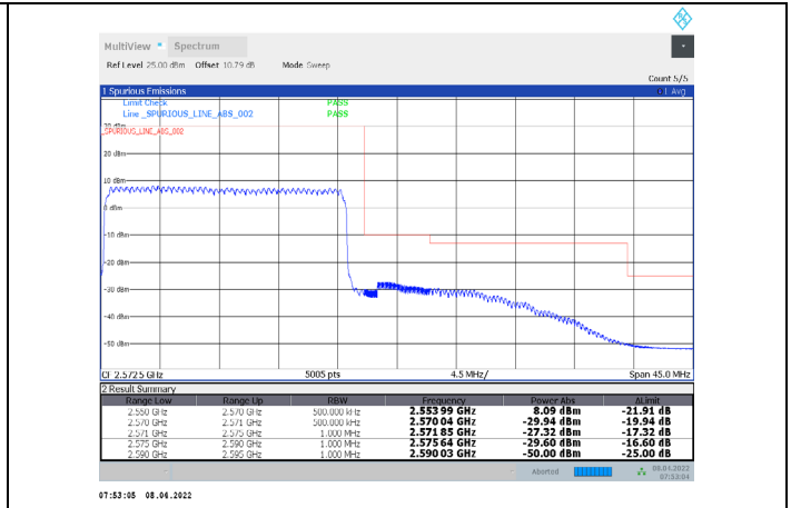
1-N7-PC3-15-20-H-15-DFT-64QAM-Outer_Full-100@0-Ant1-PASS-see graph
