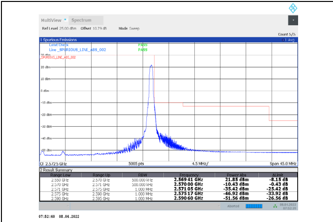
1-N7-PC3-15-20-H-14-DFT-64QAM-Edge_1RB_Right-1@105-Ant1-PASS-see graph
