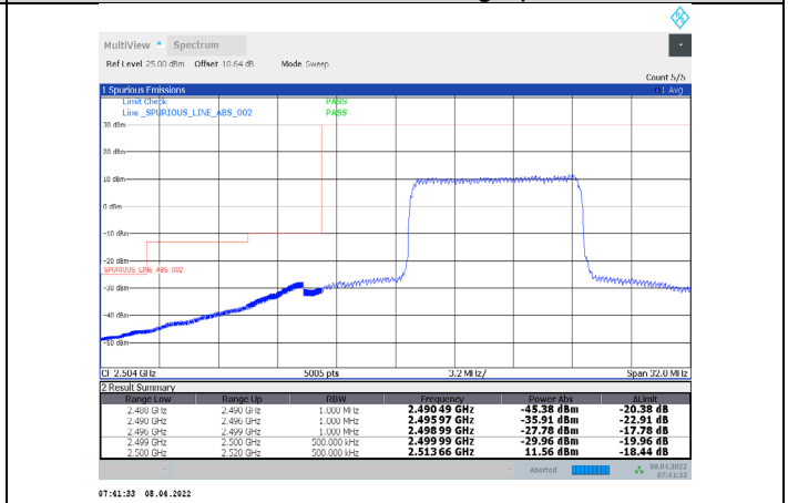
1-N7-PC3-15-20-L-16-DFT-64QAM-Inner_Full-50@25-Ant1-PASS-see graph
