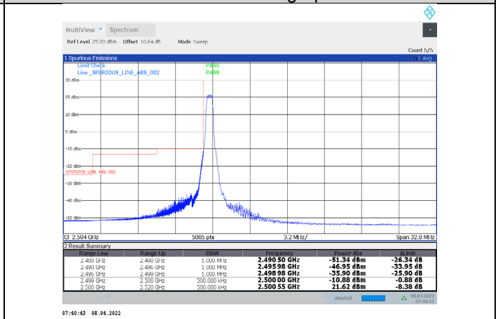
1-N7-PC3-15-20-L-13-DFT-64QAM-Edge_1RB_Left-1@0-Ant1-PASS-see graph
