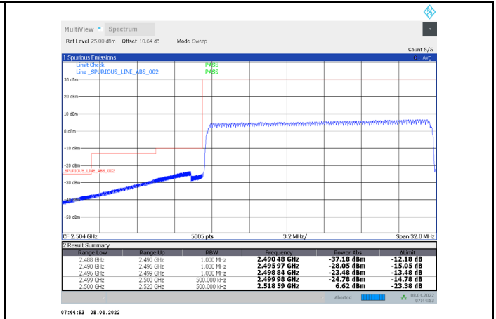
1-N7-PC3-15-20-L-27-CP-16QAM-Outer_Full-106@0-Ant1-PASS-see graph
