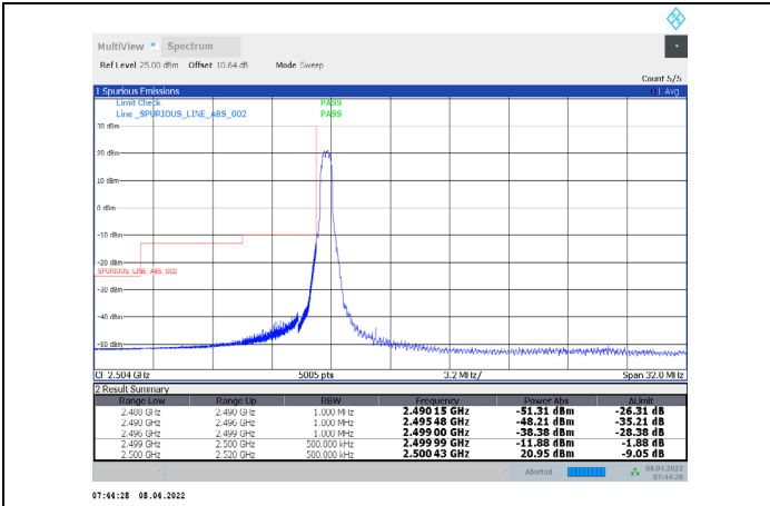
1-N7-PC3-15-20-L-25-CP-16QAM-Edge_1RB_Left-1@0-Ant1-PASS-see graph
