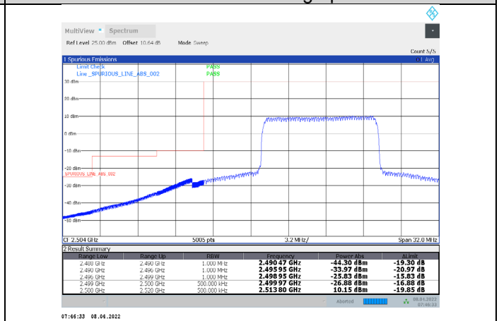
1-N7-PC3-15-20-L-32-CP-64QAM-Inner_Full-53@26-Ant1-PASS-see graph
