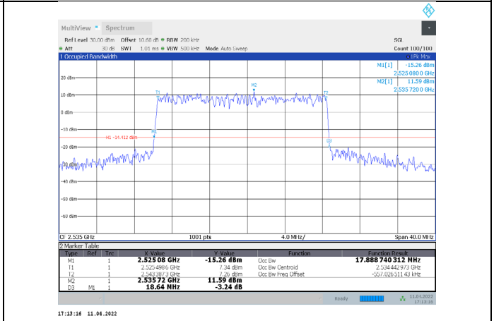
1-N7-PC3-15-20-M-1-CP-QPSK-Outer_Full-100@0-Ant 1-17.889-18.640-≤20-PASS
