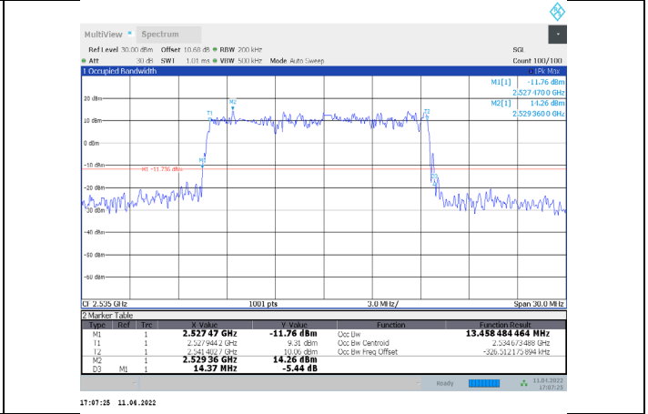
1-N7-PC3-15-15-M-7-DFT-16QAM-Outer_Full-75@0-Ant 1-13.458-14.370≤15-PASS
