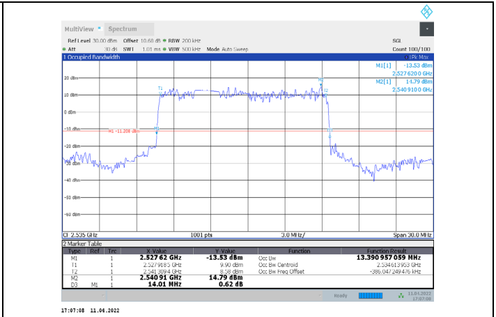
1-N7-PC3-15-15-M-5-DFT-PI/2BPSK-Outer_Full-75@0-A Ant1-13.391-14.010≤15-PASS
