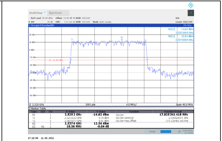
1-N7-PC3-15-20-M-5-DFT-PI/2BPSK-Outer_Full-100@0-Ant1-17.825-18.560-≤20-PASS
