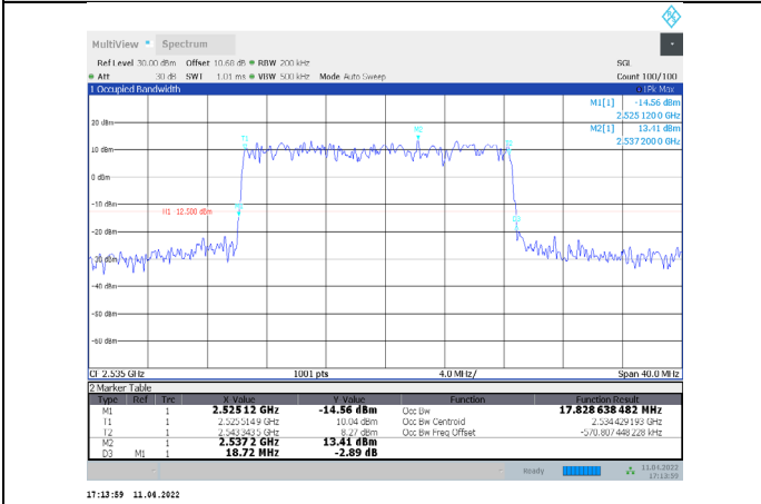
1-N7-PC3-15-20-M-6-DFT-QPSK-Outer_Full-100@0-Ant1-17.829-18.720-≤20-PASS
