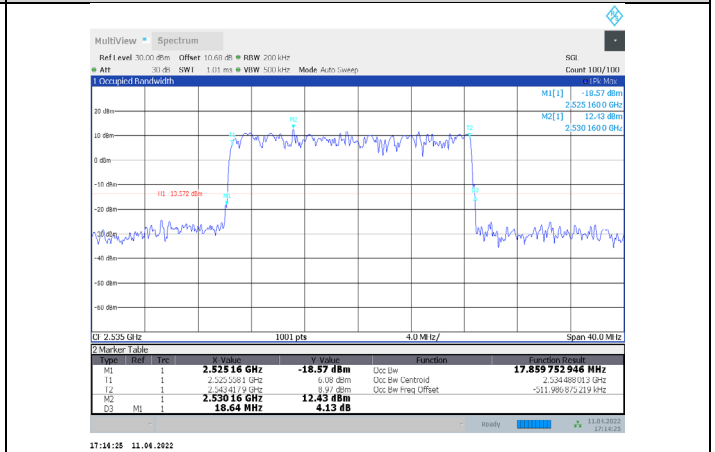
1-N7-PC3-15-20-M-9-DFT-256QAM-Outer_Full-100@0-Ant1-17.86-18.640-≤20-PASS
