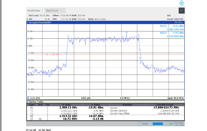
1-N7-PC3-15-20-L-5-DFT-PI/2BPSK-Outer_Full-100@0-Ant1-17.896-18.720-≤20-PASS
