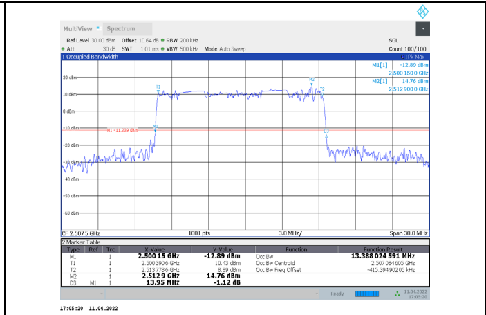
1-N7-PC3-15-15-L-8-DFT-64QAM-Outer_Full-75@0-Ant 1-13.388-13.950-≤15-PASS
