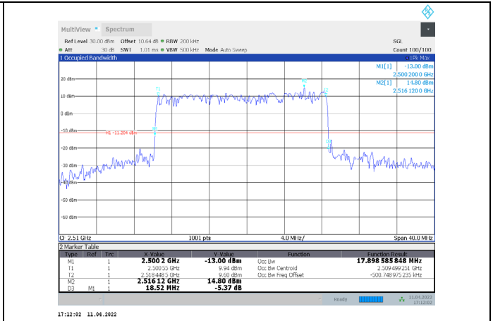
1-N7-PC3-15-20-L-8-DFT-64QAM-Outer_Full-100@0-A nt1-17.899-18.520-≤20-PASS
