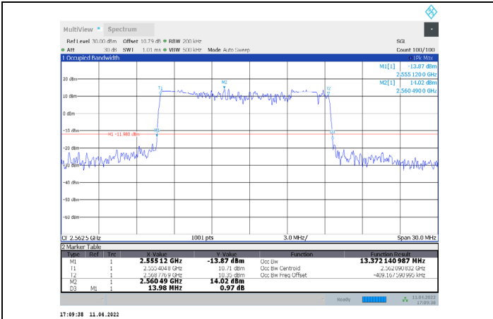
1-N7-PC3-15-15-H-7-DFT-16QAM-Outer_Full-75@0-Ant 1-13.372-13.980-≤15-PASS
