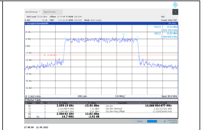
1-N7-PC3-15-15-H-2-CP-16QAM-Outer_Full-79@0-Ant1-14.067-14.700-≤15-PASS
