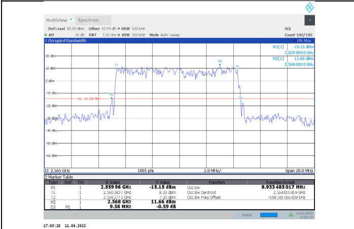
1-N7-PC3-15-10-H-9-DFT-256QAM-Outer_Full-50@0-Ant 1-8.933-9.580-≤10-PASS
