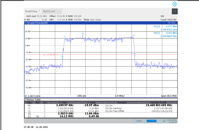
1-N7-PC3-15-15-L-9-DFT-256QAM-Outer_Full-75@0-A nt1-13.47-14.130-≤15-PASS
