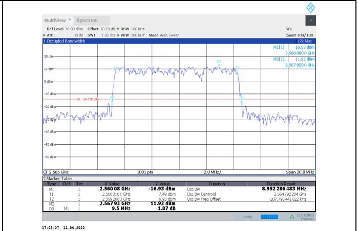
1-N7-PC3-15-10-H-8-DFT-64QAM-Outer_Full-50@0-Ant 1-8.952-9.500-≤10-PASS
