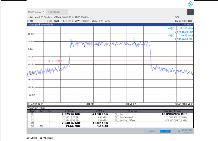
1-N7-PC3-15-20-M-2-CP-16QAM-Outer_Full-106@0-A nt1-18.899-19.640-≤20-PASS
