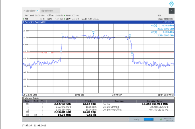
1-N7-PC3-15-15-M-6-DFT-QPSK-Outer_Full-75@0-Ant t1-13.358-14.040≤15-PASS
