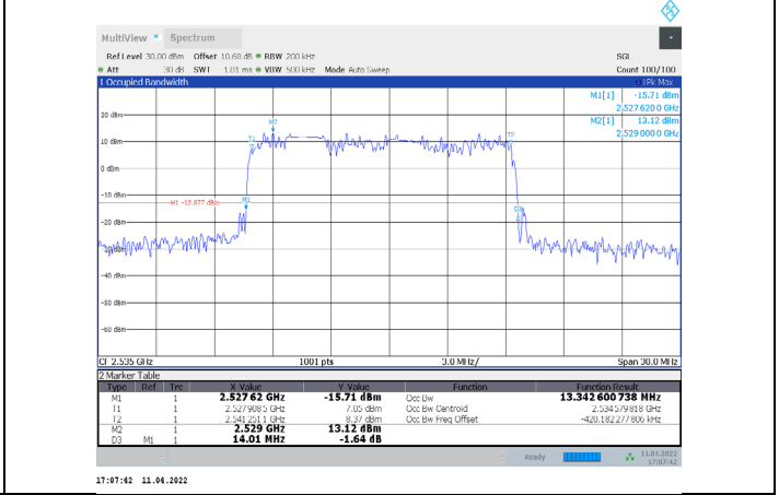
1-N7-PC3-15-15-M-9-DFT-256QAM-Outer_Full-75@0-A nt1-13.343-14.010≤15-PASS
