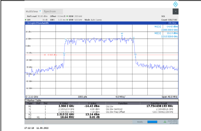
1-N7-PC3-15-20-L-9-DFT-256QAM-Outer_Full-100@0-A Ant1-17.735-18.640-≤20-PASS
