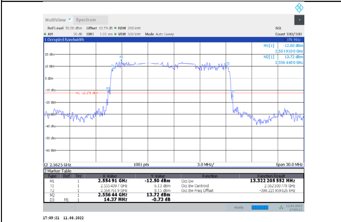
1-N7-PC3-15-15-H-5-DFT-PI/2BPSK-Outer_Full-75@0-Ant1-13.322-14.370-≤15-PASS
