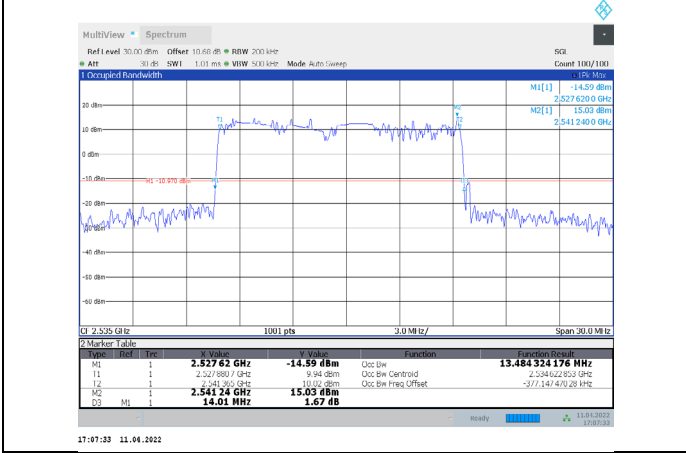
1-N7-PC3-15-15-M-8-DFT-64QAM-Outer_Full-75@0-A nt1-13.484-14.010≤15-PASS
