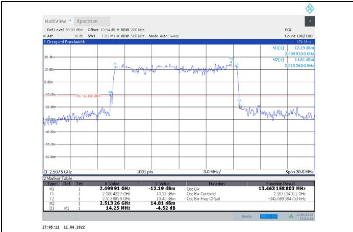
1-N7-PC3-15-15-L-7-DFT-16QAM-Outer_Full-75@0-Ant 1-13.463-14.250-≤15-PASS
