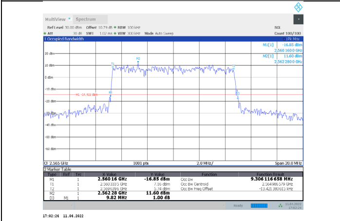
1-N7-PC3-15-10-H-3-CP-64QAM-Outer_Full-52@0-Ant1-9.306-9.820-≤10-PASS
