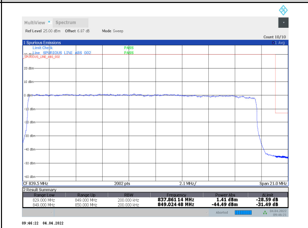
1-N5-PC3-15-20-H-4-DFT-PI/2BPSK-Outer_Full-100@0-Ant1-seegraph-PASS-see graph
