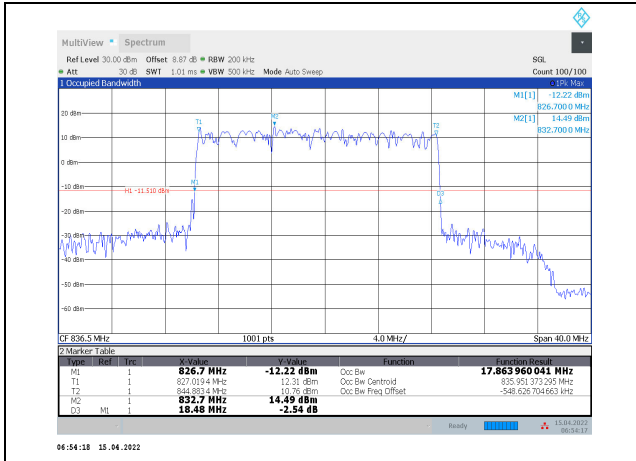
1-N5-PC3-15-20-M-9-DFT-256QAM-Outer_Full-10@0-Ant1-17.864-18.480-≤20-PASS
