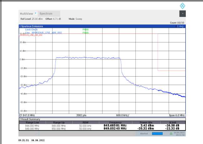
1-N5-PC3-15-5-H-28-CP-16QAM-Inner_Full-13@6-Ant1-seegraph-PASS-see graph
