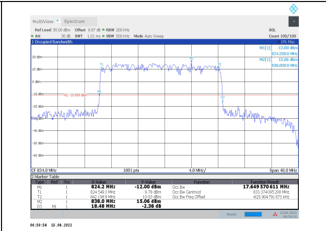
1-N5-PC3-15-20-L-7-DFT-16QAM-Outer_Full-100@ 0-Ant1-17.65-18.480-≤20-PASS
