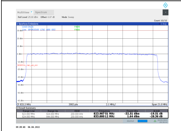
1-N5-PC3-15-20-L-15-DFT-64QAM-Outer_Full-100@0-Ant1-seegraph-PASS-see graph
