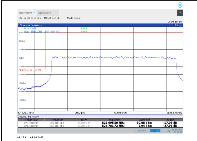
1-N5-PC3-15-5-L-15-DFT-64QAM-Outer_Full-25@ 0-Ant1-seegraph-PASS-see graph
