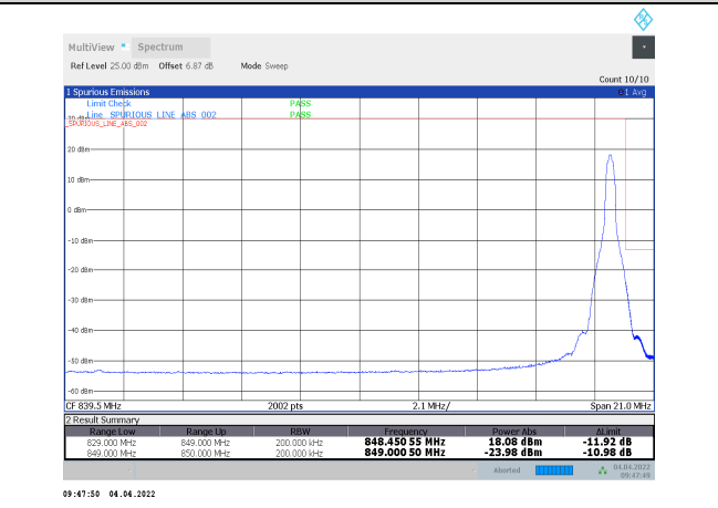
1-N5-PC3-15-20-H-10-DFT-16QAM-Edge_1RB_Right@105-Ant1-seegraph-PASS-see graph
