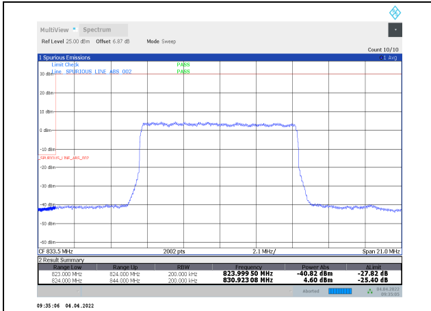
1-N5-PC3-15-20-L-1-DFT-PI/2BPSK-Inner_Full-50 @25-Ant1-seegraph-PASS-see graph
