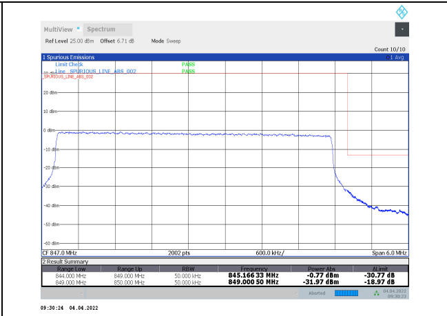
1-N5-PC3-15-5-H-23-CP-QPSK-Outer_Full-25@0-Ant1-seegraph-PASS-see graph
