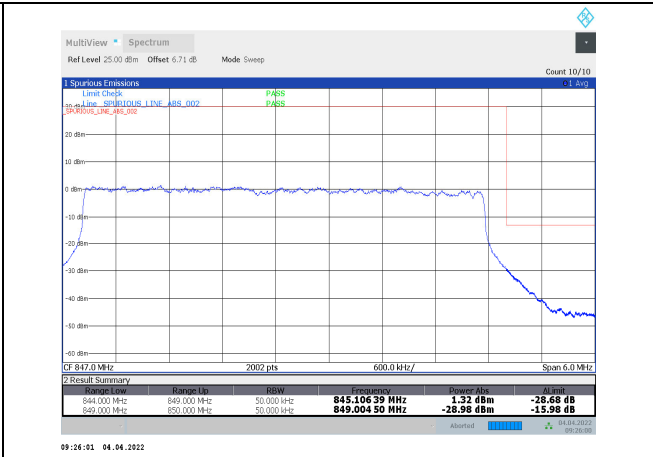
1-N5-PC3-15-5-H-7-DFT-QPSK-Outer_Full-25@0-Ant1-seegraph-PASS-see graph
