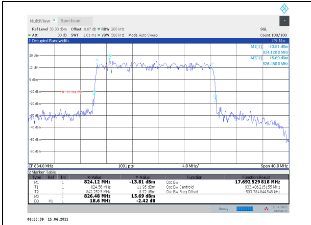
1-N5-PC3-15-20-L-6-DFT-QPSK-Outer_Full-100@ 0-Ant1-17.693-18.600-≤20-PASS
