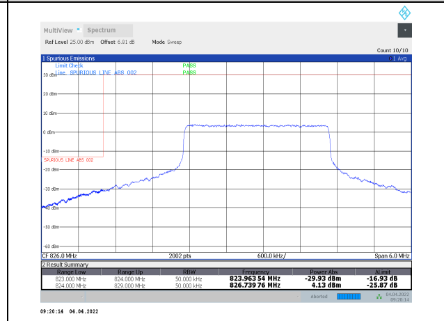
1-N5-PC3-15-5-L-24-CP-QPSK-Inner_Full-13@6-Ant1-seegraph-PASS-see graph
