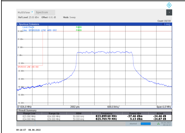
1-N5-PC3-15-5-L-12-DFT-16QAM-Inner_Full-12@ 6-Ant1-seegraph-PASS-see graph
