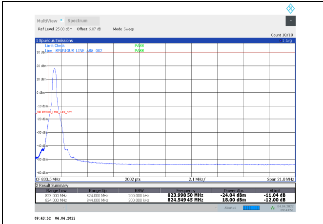
1-N5-PC3-15-20-L-33-CP-256QAM-Edge_1RB_Left_1@0-Ant1-seegraph-PASS-see graph
