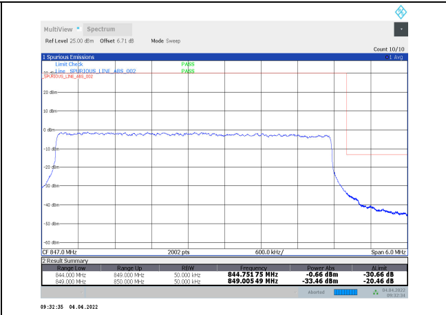
1-N5-PC3-15-5-H-31-CP-64QAM-Outer_Full-25@0- Ant1-seegraph-PASS-see graph
