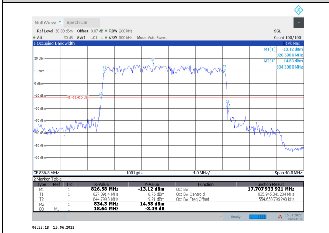
1-N5-PC3-15-20-M-5-DFT-PI/2BPSK-Outer_Full-100 @0-Ant1-17.708-18.640-≤20-PASS
