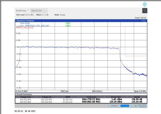
1-N5-PC3-15-5-H-15-DFT-64QAM-Outer_Full-25@ 0-Ant1-seegraph-PASS-see graph
