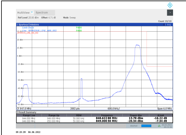
1-N5-PC3-15-5-H-6-DFT-QPSK-Edge_1RB_Right_1@24-Ant1-seegraph-PASS-see graph
