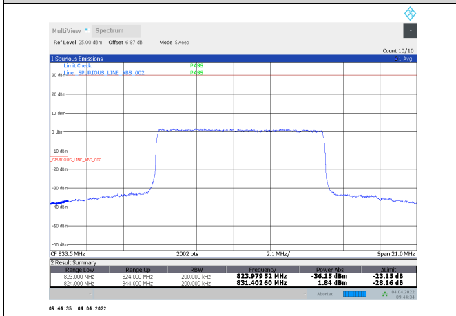
1-N5-PC3-15-20-L-36-CP-256QAM-Inner_Full-53@26-Ant1-seegraph-PASS-see graph
