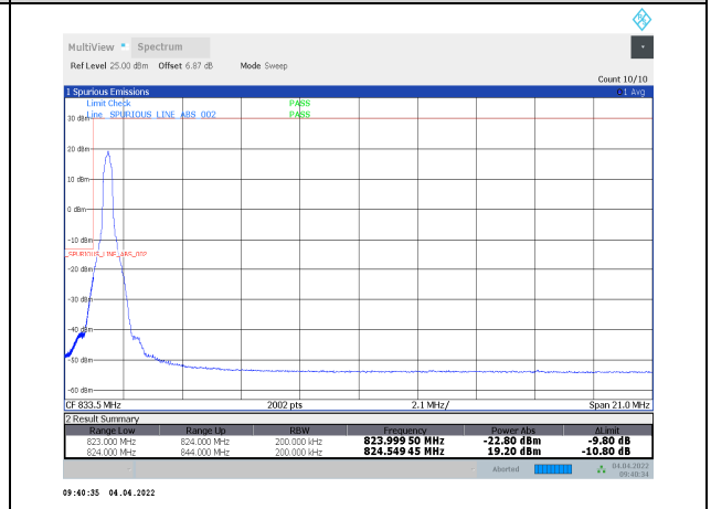
1-N5-PC3-15-20-L-21-CP-QPSK-Edge_1RB_Left- 1@0-Ant1-seegraph-PASS-see graph
