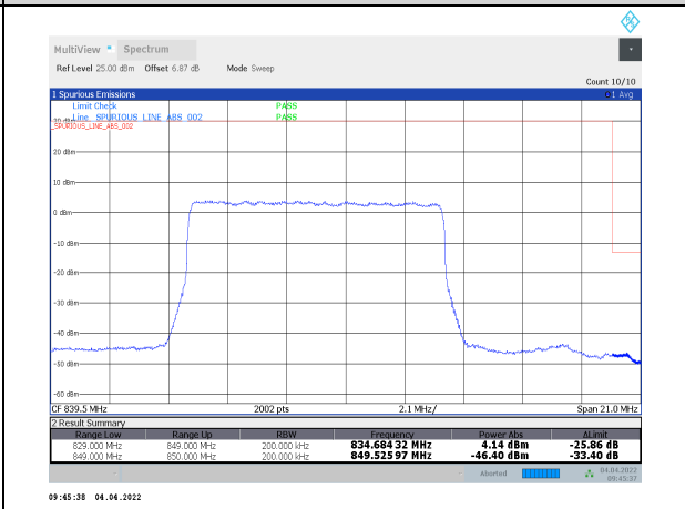
1-N5-PC3-15-20-H-1-DFT-PI/2BPSK-Inner_Full-50@25-Ant1-seegraph-PASS-see graph
