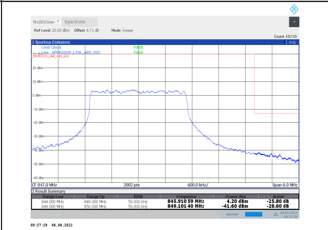
1-N5-PC3-15-5-H-12-DFT-16QAM-Inner_Full-12@6-Ant1-seegraph-PASS-see graph
