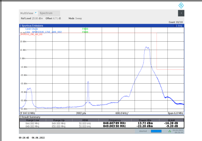
1-N5-PC3-15-5-H-10-DFT-16QAM-Edge_1RB_Right_1@24-Ant1-seegraph-PASS-see graph
