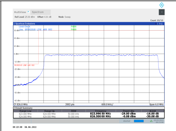
1-N5-PC3-15-5-L-35-CP-256QAM-Outer_Full-25 @0-Ant1-seegraph-PASS-see graph
