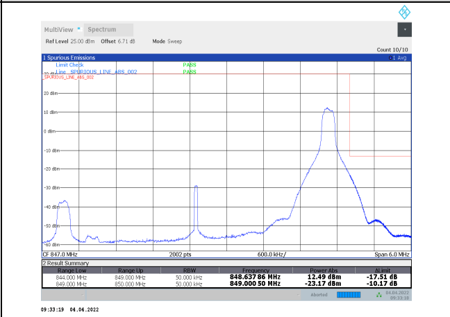
1-N5-PC3-15-5-H-34-CP-256QAM-Edge_1RB_Right t-1@24-Ant1-seegraph-PASS-see graph
