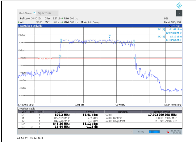
1-N5-PC3-15-20-H-6-DFT-QPSK-Outer_Full-100@ 0-Ant1-17.703-18.440-≤20-PASS
