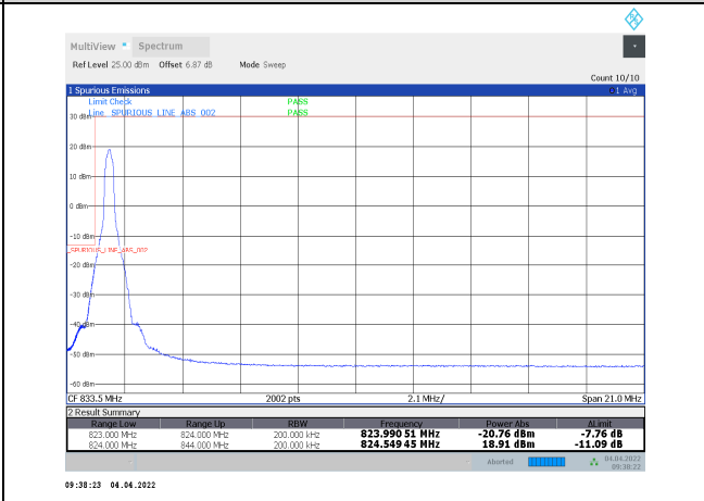
1-N5-PC3-15-20-L-13-DFT-64QAM-Edge_1RB_Left_1@0-Ant1-seegraph-PASS-see graph
