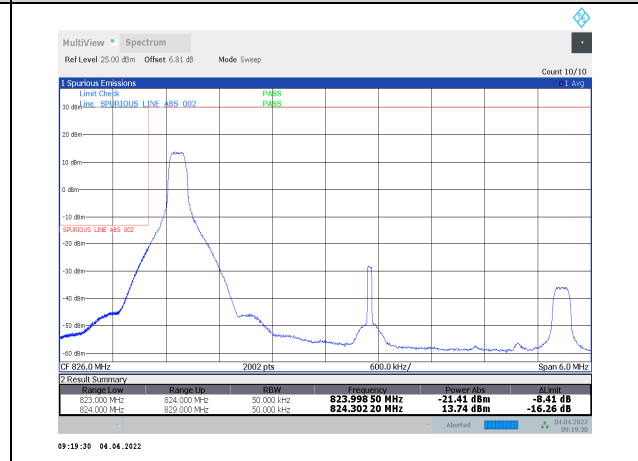
1-N5-PC3-15-5-L-21-CP-QPSK-Edge_1RB_Left-1@0-Ant1-seegraph-PASS-see graph
