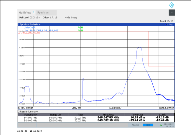
1-N5-PC3-15-5-H-18-DFT-256QAM-Edge_1RB_Rig ht-1@24-Ant1-seegraph-PASS-see graph
