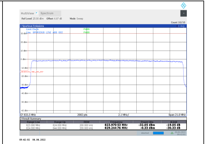
1-N5-PC3-15-20-L-27-CP-16QAM-Outer_Full-106@0-Ant1-seegraph-PASS-see graph
