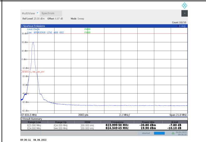
1-N5-PC3-15-20-L-5-DFT-QPSK-Edge_1RB_Left-1 @0-Ant1-seegraph-PASS-see graph
