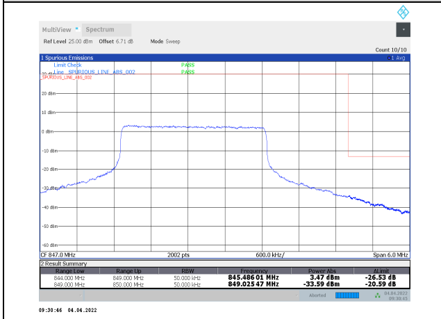
1-N5-PC3-15-5-H-24-CP-QPSK-Inner_Full-13@6-Ant1-seegraph-PASS-see graph
