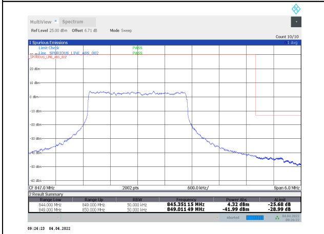
1-N5-PC3-15-5-H-8-DFT-QPSK-Inner_Full-12@6-Ant1-seegraph-PASS-see graph
