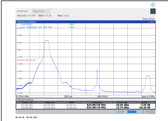
1-N5-PC3-15-5-L-25-CP-16QAM-Edge_1RB_Left-1 @0-Ant1-seegraph-PASS-see graph
