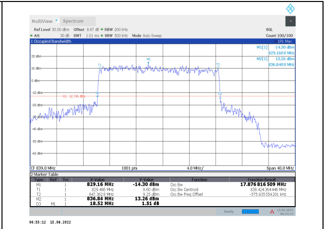
1-N5-PC3-15-20-H-1-CP-QPSK-Outer_Full-100@0-Ant1-17.877-18.520-≤20-PASS
