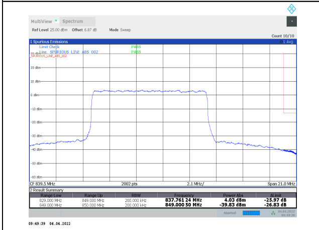
1-N5-PC3-15-20-H-16-DFT-64QAM-Inner_Full-50 @25-Ant1-seegraph-PASS-see graph
