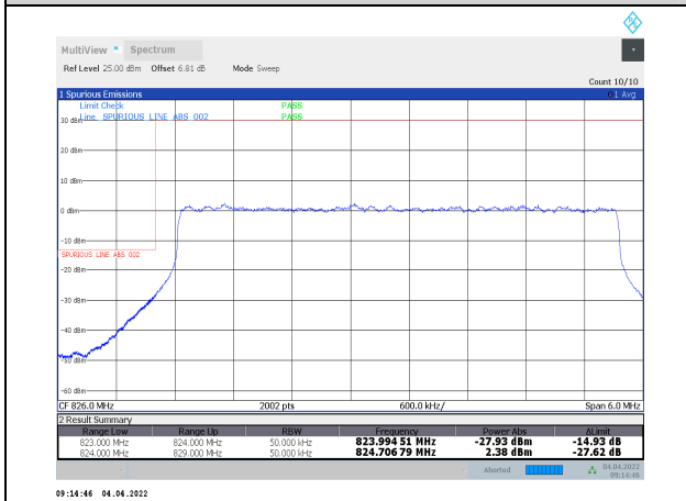
1-N5-PC3-15-5-L-4-DFT-PI/2BPSK-Outer_Full-25 @0-Ant1-seegraph-PASS-see graph
