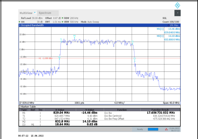
1-N5-PC3-15-20-H-9-DFT-256QAM-Outer_Full-100 @0-Ant1-17.657-18.640-≤20-PASS
