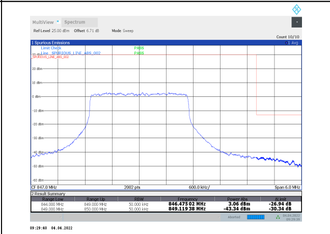
1-N5-PC3-15-5-H-20-DFT-256QAM-Inner_Full-12@ 6-Ant1-seegraph-PASS-see graph
