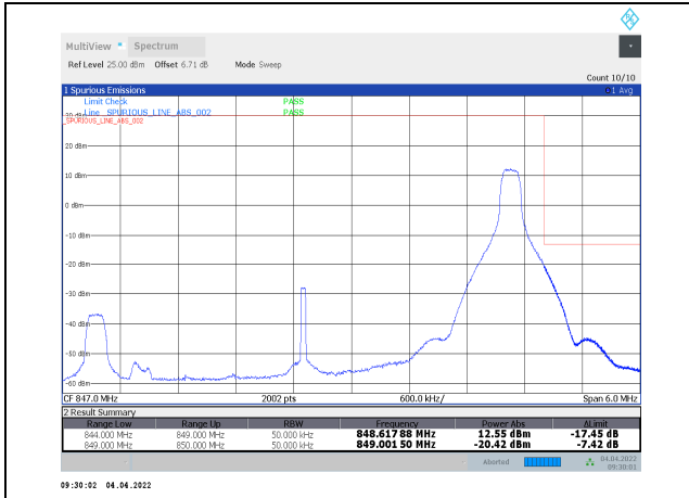
1-N5-PC3-15-5-H-22-CP-QPSK-Edge_1RB_Right-1@24-Ant1-seegraph-PASS-see graph
