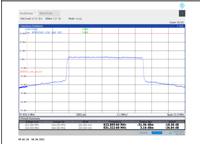
1-N5-PC3-15-20-L-28-CP-16QAM-Inner_Full-53@26-Ant1-seegraph-PASS-see graph
