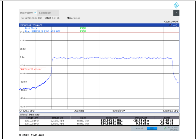
1-N5-PC3-15-5-L-27-CP-16QAM-Outer_Full-25@0- Ant1-seegraph-PASS-see graph
