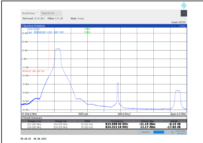
1-N5-PC3-15-5-L-17-DFT-256QAM-Edge_1RB_Left_1@0-Ant1-seegraph-PASS-see graph
