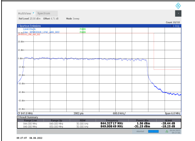
1-N5-PC3-15-5-H-11-DFT-16QAM-Outer_Full-25@0-Ant1-seegraph-PASS-see graph
