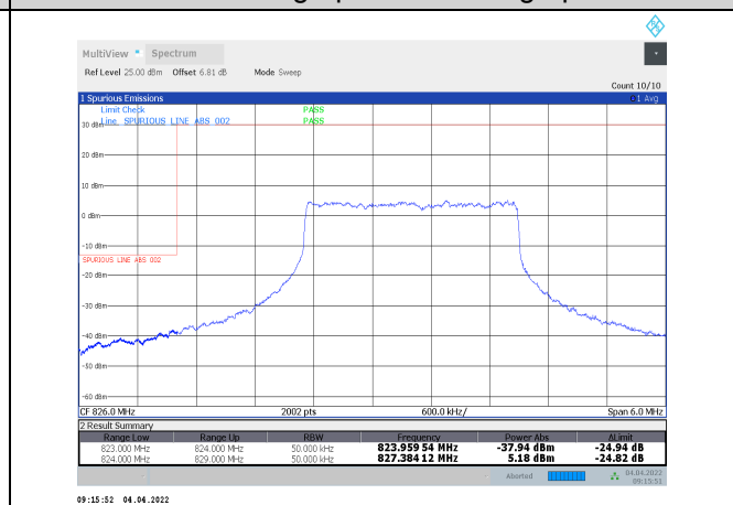
1-N5-PC3-15-5-L-8-DFT-QPSK-Inner_Full-12@6-Ant1-seegraph-PASS-see graph
