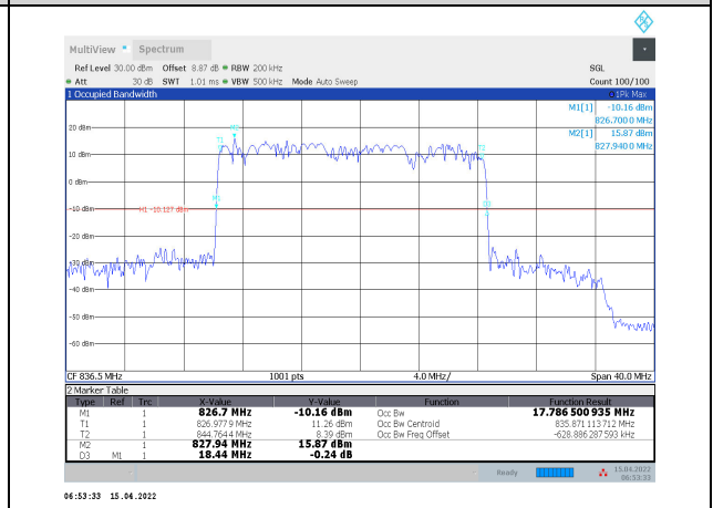
1-N5-PC3-15-20-M-6-DFT-QPSK-Outer_Full-100 @0-Ant1-17.787-18.440-≤20-PASS
