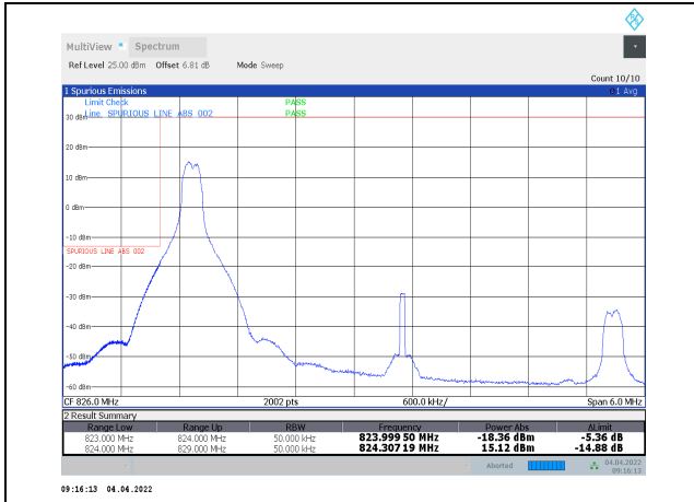
1-N5-PC3-15-5-L-9-DFT-16QAM-Edge_1RB_Left-1 @0-Ant1-seegraph-PASS-see graph
