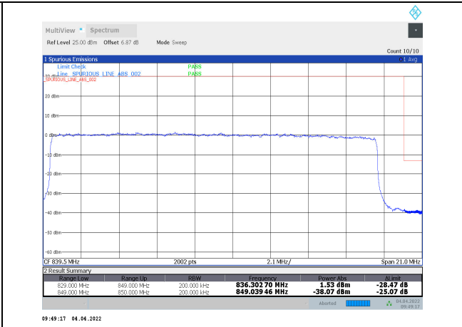
1-N5-PC3-15-20-H-15-DFT-64QAM-Outer_Full-100 @0-Ant1-seegraph-PASS-see graph
