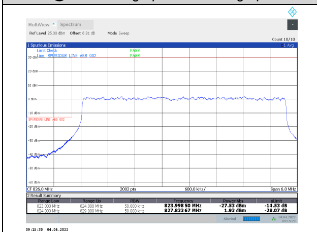
1-N5-PC3-15-5-L-7-DFT-QPSK-Outer_Full-25@0-Ant1-seegraph-PASS-see graph
