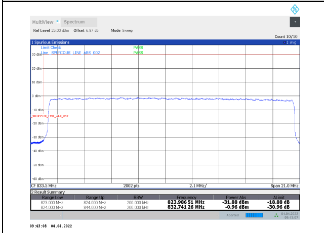
1-N5-PC3-15-20-L-31-CP-64QAM-Outer_Full-106@0-Ant1-seegraph-PASS-see graph
