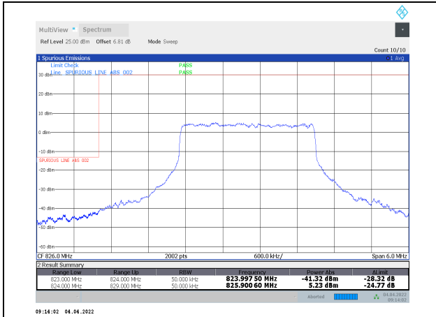
1-N5-PC3-15-5-L-1-DFT-PI/2BPSK-Inner_Full-12 @6-Ant1-seegraph-PASS-see graph
