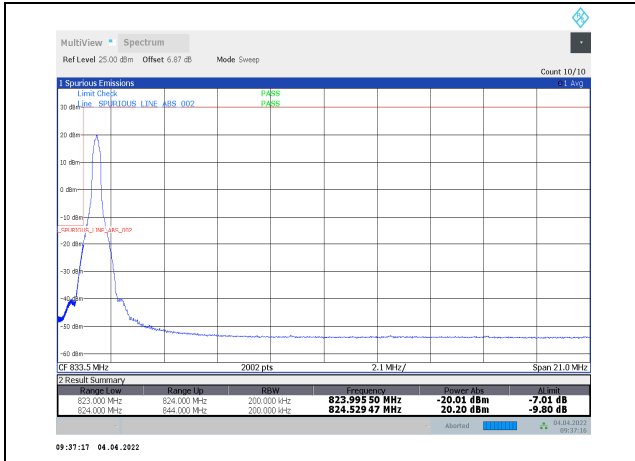
1-N5-PC3-15-20-L-9-DFT-16QAM-Edge_1RB_Left_1@0-Ant1-seegraph-PASS-see graph
