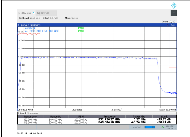
1-N5-PC3-15-20-H-19-DFT-256QAM-Outer_Full-10 @0-Ant1-seegraph-PASS-see graph
