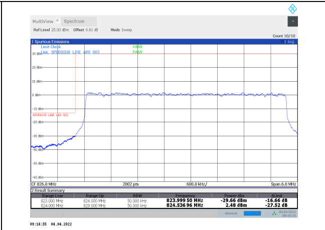
1-N5-PC3-15-5-L-11-DFT-16QAM-Outer_Full-25@0 -Ant1-seegraph-PASS-see graph
