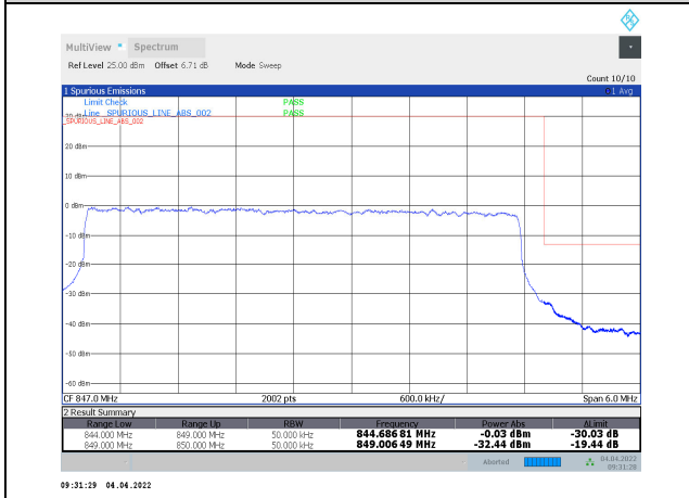
1-N5-PC3-15-5-H-27-CP-16QAM-Outer_Full-25@0-Ant1-seegraph-PASS-see graph
