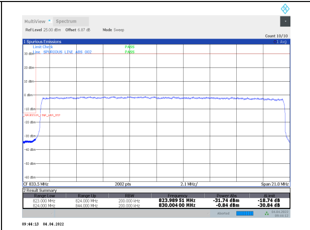
1-N5-PC3-15-20-L-35-CP-256QAM-Outer_Full-106@0-Ant1-seegraph-PASS-see graph
