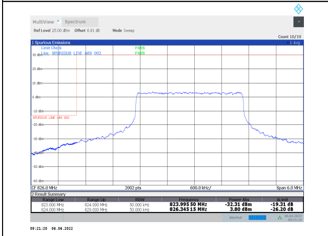
1-N5-PC3-15-5-L-28-CP-16QAM-Inner_Full-13@6- Ant1-seegraph-PASS-see graph
