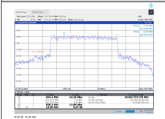
1-N5-PC3-15-20-L-4-CP-256QAM-Outer_Full-106@0-Ant1-18.942-19.560-≤20-PASS
