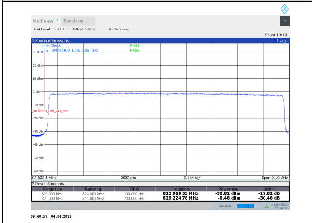
1-N5-PC3-15-20-L-23-CP-QPSK-Outer_Full-106@0 -Ant1-seegraph-PASS-see graph
