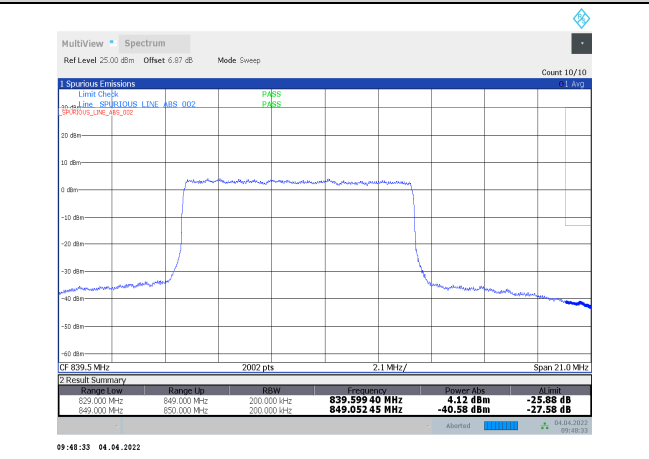
1-N5-PC3-15-20-H-12-DFT-16QAM-Inner_Full-50@25-Ant1-seegraph-PASS-see graph
