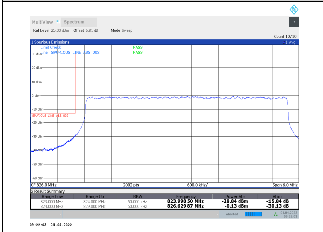
1-N5-PC3-15-5-L-31-CP-64QAM-Outer_Full-25@0- Ant1-seegraph-PASS-see graph
