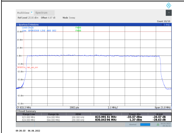
1-N5-PC3-15-20-L-7-DFT-QPSK-Outer_Full-100@ 0-Ant1-seegraph-PASS-see graph
