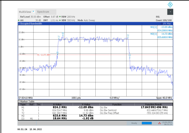
1-N5-PC3-15-20-L-9-DFT-256QAM-Outer_Full-100 @0-Ant1-17.844-18.640-≤20-PASS
