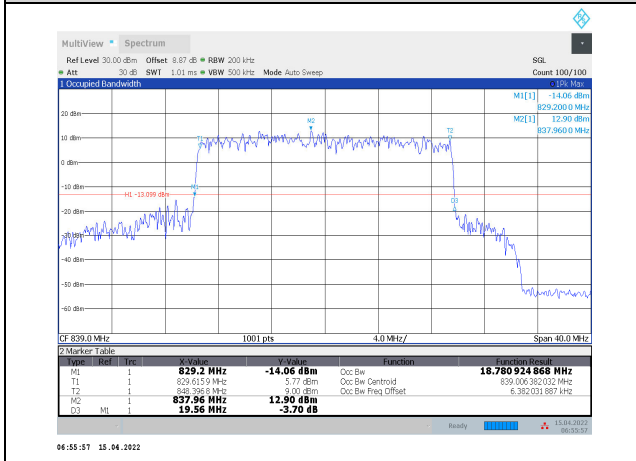
1-N5-PC3-15-20-H-4-CP-256QAM-Outer_Full-106@0-Ant1-18.781-19.560-≤20-PASS
