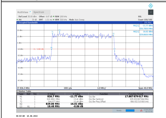
1-N5-PC3-15-20-M-7-DFT-16QAM-Outer_Full-100 @0-Ant1-17.888-18.480-≤20-PASS
