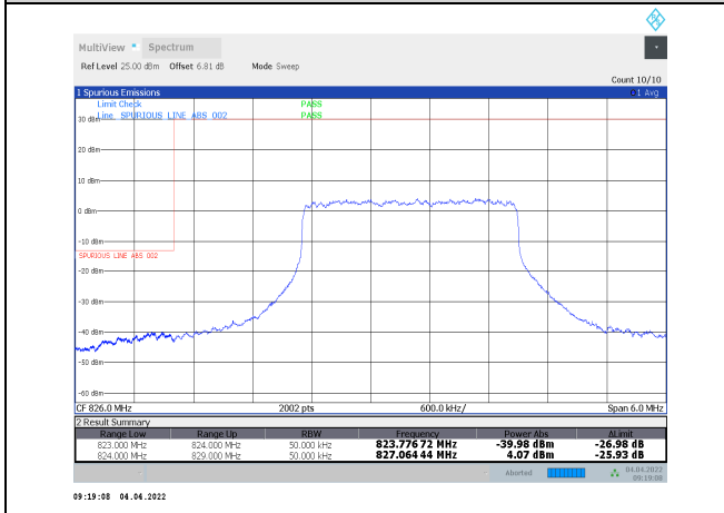
1-N5-PC3-15-5-L-20-DFT-256QAM-Inner_Full-12@6-Ant1-seegraph-PASS-see graph
