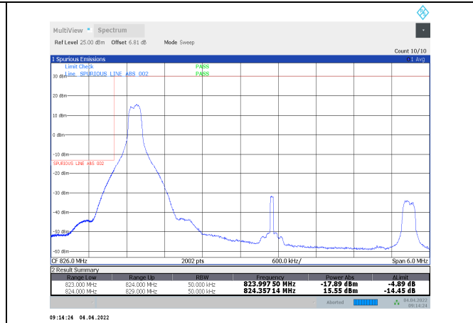
1-N5-PC3-15-5-L-2-DFT-PI/2BPSK-Edge_1RB_Left-1@0-Ant1-seegraph-PASS-see graph
