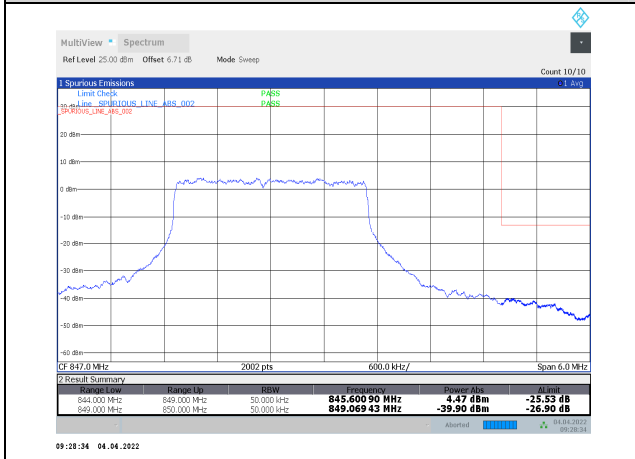
1-N5-PC3-15-5-H-16-DFT-64QAM-Inner_Full-12@ 6-Ant1-seegraph-PASS-see graph
