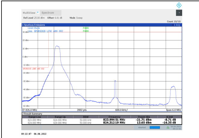
1-N5-PC3-15-5-L-33-CP-256QAM-Edge_1RB_Left-1 @0-Ant1-seegraph-PASS-see graph
