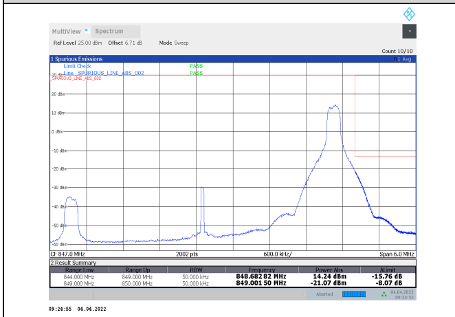
1-N5-PC3-15-5-H-3-DFT-PI/2BPSK-Edge_1RB_Right -1@24-Ant1-seegraph-PASS-see graph
