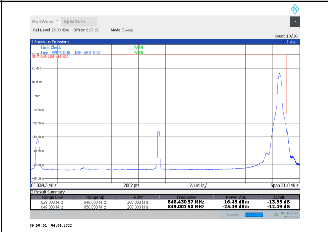
1-N5-PC3-15-20-H-18-DFT-256QAM-Edge_1RB_Ri ght-1@105-Ant1-seegraph-PASS-see graph
