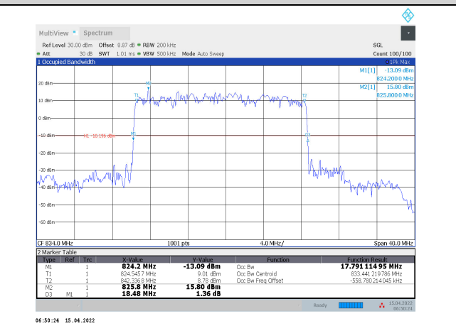
1-N5-PC3-15-20-L-5-DFT-PI/2BPSK-Outer_Full-100@0-Ant1-17.791-18.480-≤20-PASS
