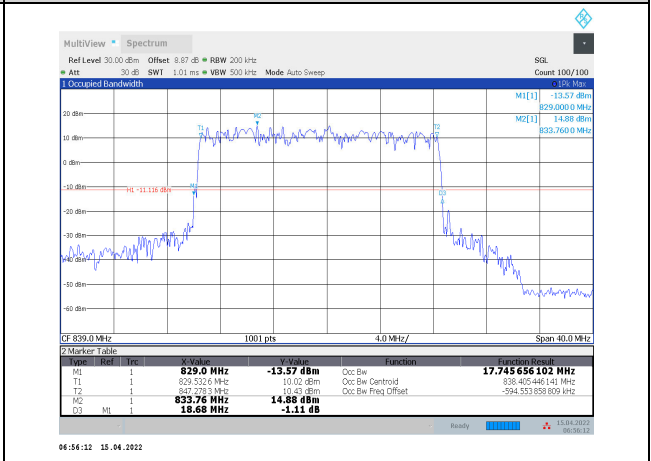
1-N5-PC3-15-20-H-5-DFT-PI/2BPSK-Outer_Full-10@0-Ant1-17.746-18.680-≤20-PASS
