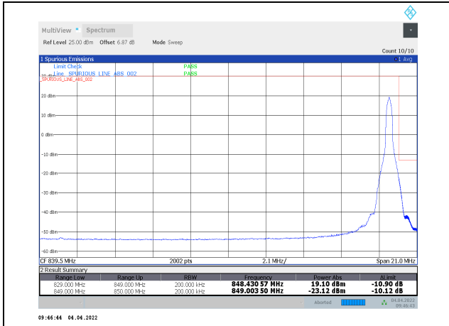
1-N5-PC3-15-20-H-6-DFT-QPSK-Edge_1RB_Right@105-Ant1-seegraph-PASS-see graph
