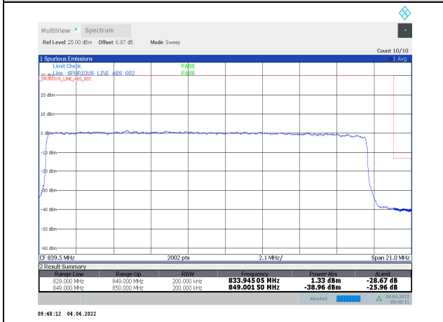
1-N5-PC3-15-20-H-11-DFT-16QAM-Outer_Full-100@0-Ant1-seegraph-PASS-see graph
