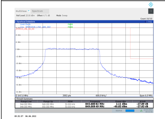
1-N5-PC3-15-5-H-32-CP-64QAM-Inner_Full-13@6 -Ant1-seegraph-PASS-see graph
