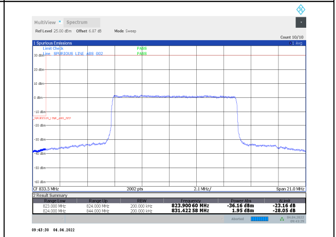
1-N5-PC3-15-20-L-32-CP-64QAM-Inner_Full-53@26-Ant1-seegraph-PASS-see graph
