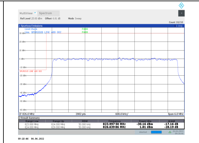
1-N5-PC3-15-5-L-19-DFT-256QAM-Outer_Full-25@0-Ant1-seegraph-PASS-see graph
