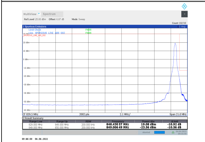
1-N5-PC3-15-20-H-3-DFT-PI/2BPSK-Edge_1RB_Rig ht-1@105-Ant1-seegraph-PASS-see graph
