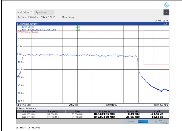
1-N5-PC3-15-5-H-19-DFT-256QAM-Outer_Full-25 @0-Ant1-seegraph-PASS-see graph
