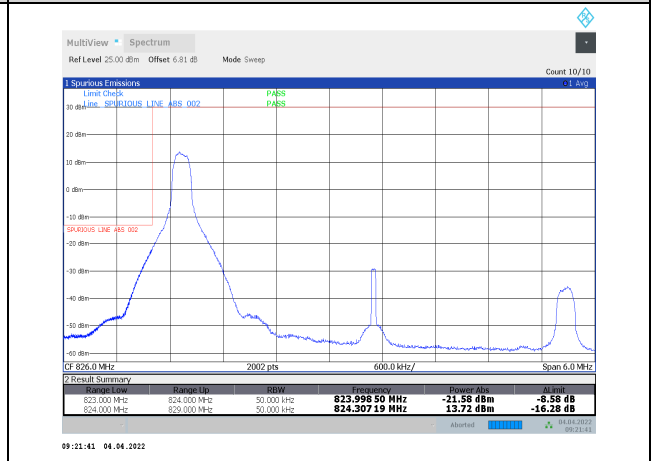
1-N5-PC3-15-5-L-29-CP-64QAM-Edge_1RB_Left-1 @0-Ant1-seegraph-PASS-see graph
