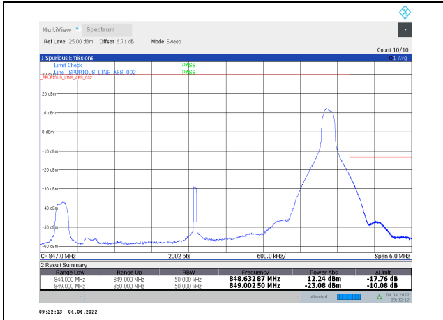
1-N5-PC3-15-5-H-30-CP-64QAM-Edge_1RB_Right -1@24-Ant1-seegraph-PASS-see graph
