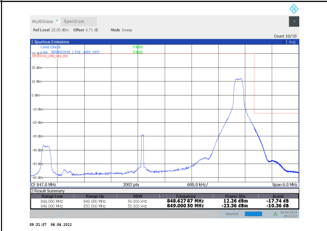
1-N5-PC3-15-5-H-26-CP-16QAM-Edge_1RB_Right-1@24-Ant1-seegraph-PASS-see graph
