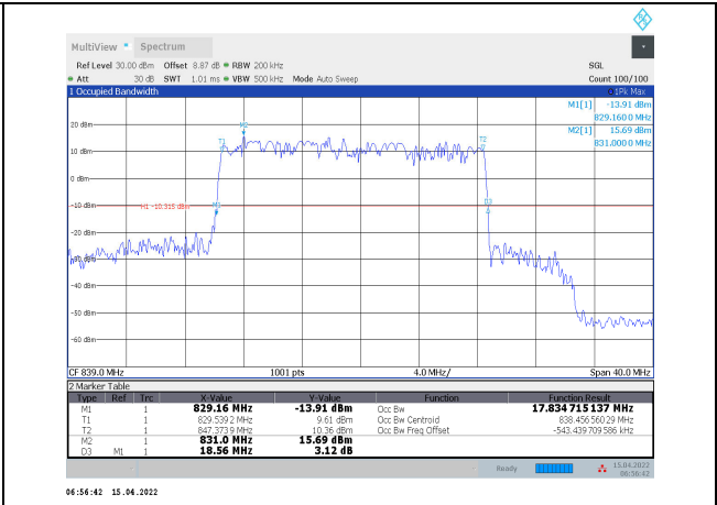
1-N5-PC3-15-20-H-7-DFT-16QAM-Outer_Full-100 @0-Ant1-17.835-18.560-≤20-PASS
