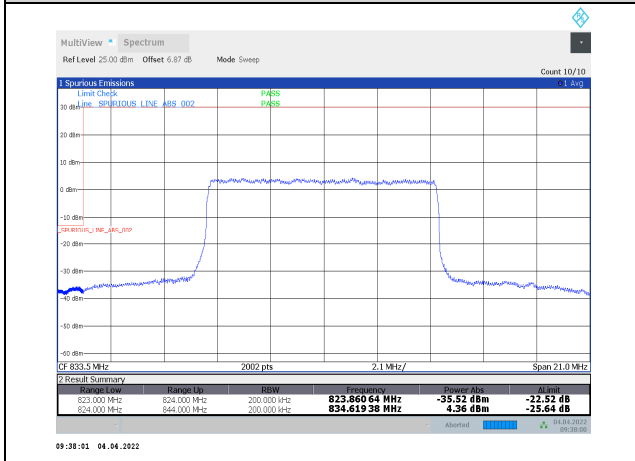
1-N5-PC3-15-20-L-12-DFT-16QAM-Inner_Full-50@25-Ant1-seegraph-PASS-see graph
