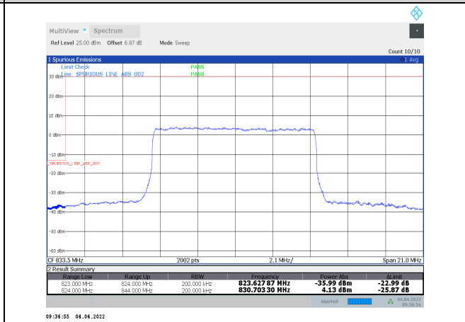
1-N5-PC3-15-20-L-8-DFT-QPSK-Inner_Full-50@25- Ant1-seegraph-PASS-see graph
