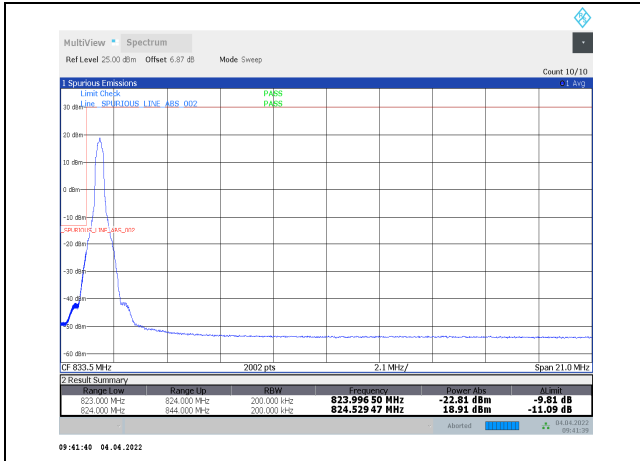
1-N5-PC3-15-20-L-25-CP-16QAM-Edge_1RB_Left_1@0-Ant1-seegraph-PASS-see graph
