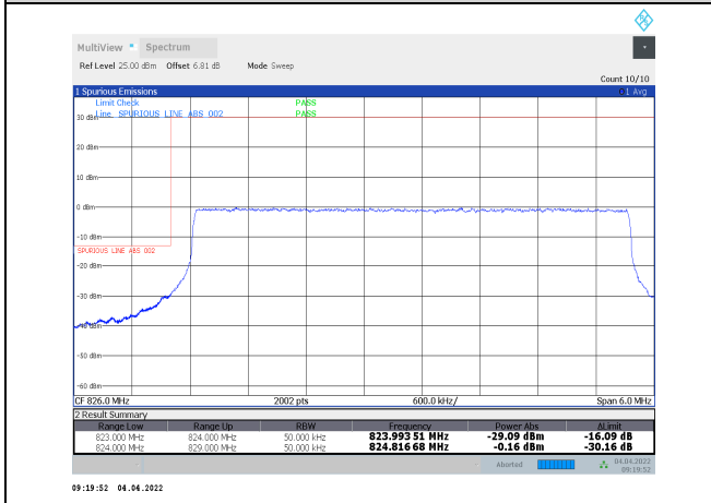
1-N5-PC3-15-5-L-23-CP-QPSK-Outer_Full-25@0-Ant1-seegraph-PASS-see graph
