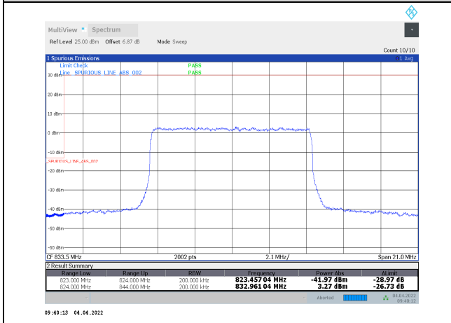
1-N5-PC3-15-20-L-20-DFT-256QAM-Inner_Full-50 @25-Ant1-seegraph-PASS-see graph
