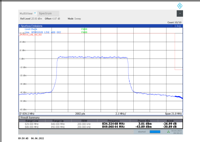
1-N5-PC3-15-20-H-20-DFT-256QAM-Inner_Full-50 @25-Ant1-seegraph-PASS-see graph
