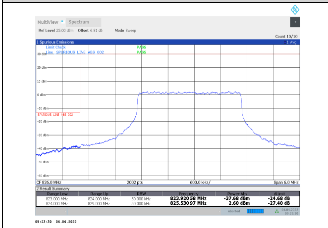
1-N5-PC3-15-5-L-36-CP-256QAM-Inner_Full-13@6-Ant1-seegraph-PASS-see graph
