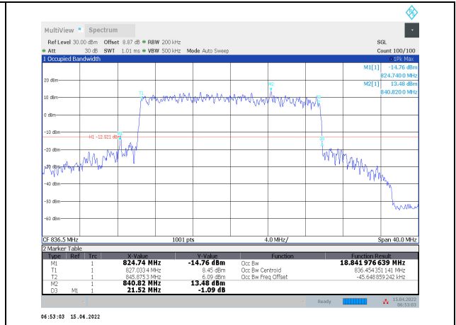
1-N5-PC3-15-20-M-4-CP-256QAM-Outer_Full-106 @0-Ant1-18.842-21.520-≤20-PASS
