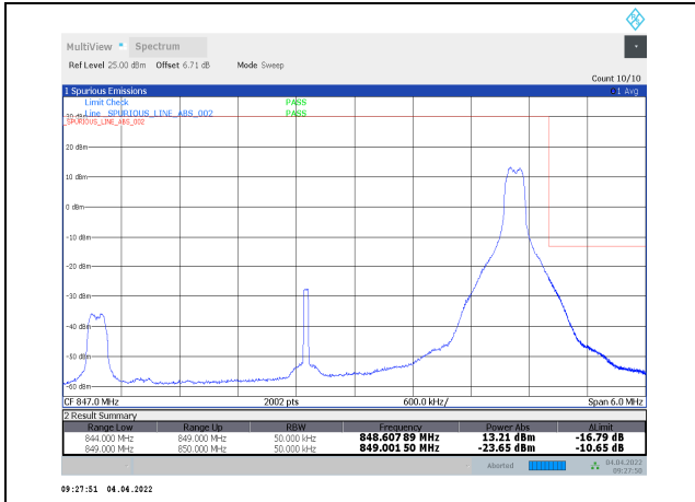
1-N5-PC3-15-5-H-14-DFT-64QAM-Edge_1RB_Rig ht-1@24-Ant1-seegraph-PASS-see graph
