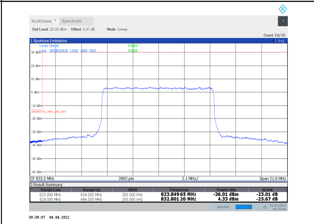
1-N5-PC3-15-20-L-16-DFT-64QAM-Inner_Full-50@25-Ant1-seegraph-PASS-see graph
