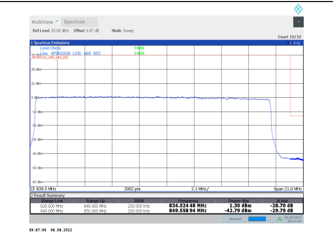
1-N5-PC3-15-20-H-7-DFT-QPSK-Outer_Full-100@0-Ant1-seegraph-PASS-see graph
