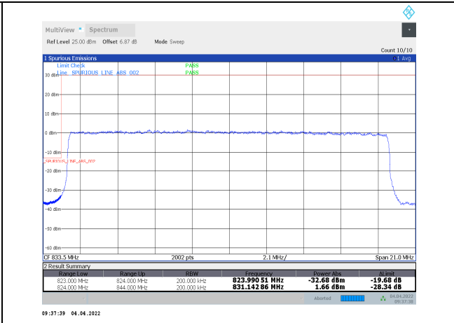
1-N5-PC3-15-20-L-11-DFT-16QAM-Outer_Full-100@0-Ant1-seegraph-PASS-see graph
