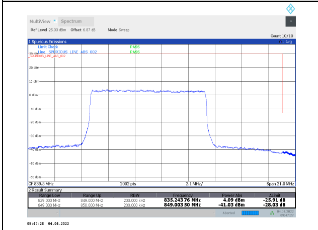
1-N5-PC3-15-20-H-8-DFT-QPSK-Inner_Full-50@25-Ant1-seegraph-PASS-see graph
