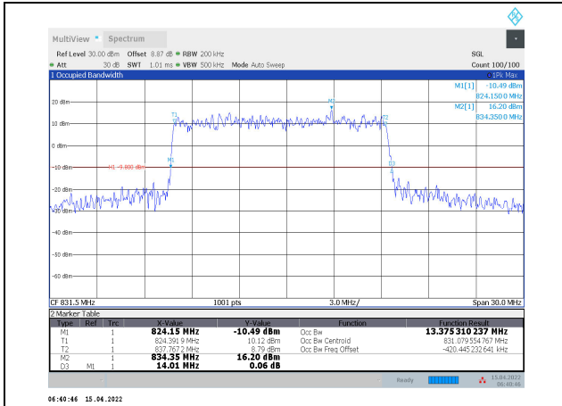
1-N5-PC3-15-15-L-1-CP-QPSK-Outer_Full-75@0- Ant1-13.375-14.010-≤15-PASS
