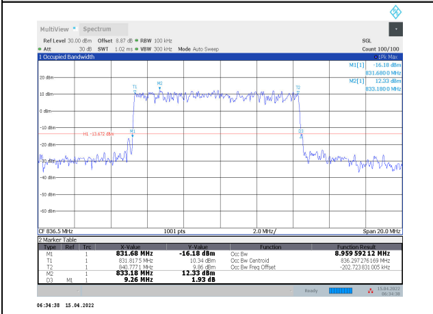
1-N5-PC3-15-10-M-1-CP-QPSK-Outer_Full-50@0- Ant1-8.96-9.260-≤10-PASS
