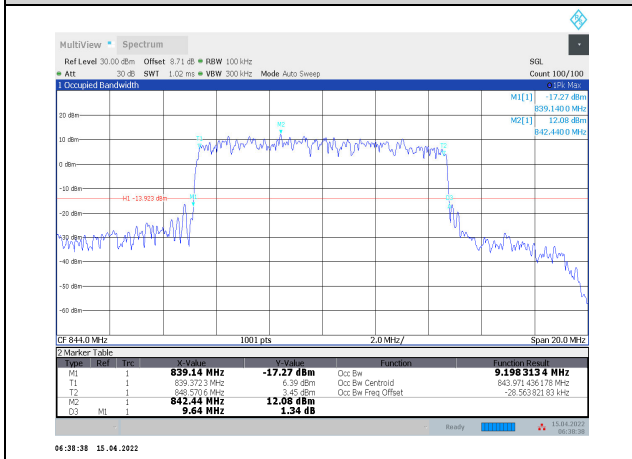
1-N5-PC3-15-10-H-4-CP-256QAM-Outer_Full-52 @0-Ant1-9.198-9.640-≤10-PASS
