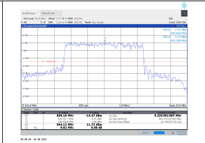
1-N5-PC3-15-10-H-3-CP-64QAM-Outer_Full-52@0- Ant1-9.255-9.620-≤10-PASS
