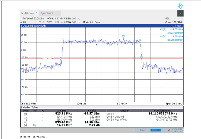
1-N5-PC3-15-15-L-2-CP-16QAM-Outer_Full-79@0- Ant1-14.111-14.910-≤15-PASS
