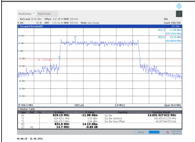
1-N5-PC3-15-15-M-4-CP-256QAM-Outer_Full-79 @0-Ant1-14.052-14.700-≤15-PASS
