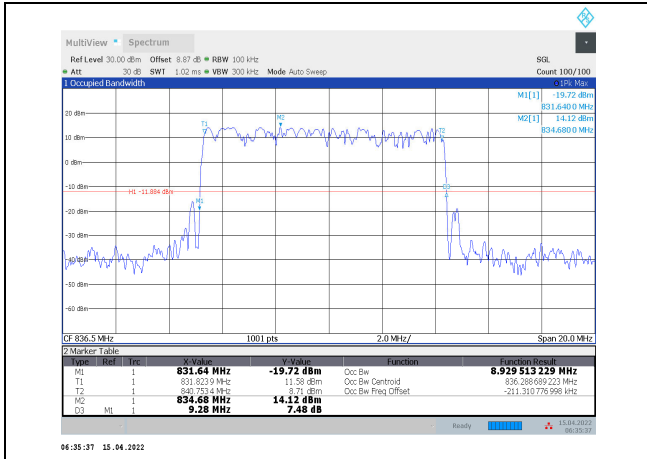
1-N5-PC3-15-10-M-5-DFT-PI/2BPSK-Outter_Full-50 @0-Ant1-8.93-9.280-≤10-PASS
