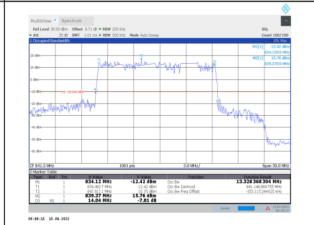
1-N5-PC3-15-15-H-8-DFT-64QAM-Outter_Full-75 @0-Ant1-13.328-14.040-≤15-PASS
