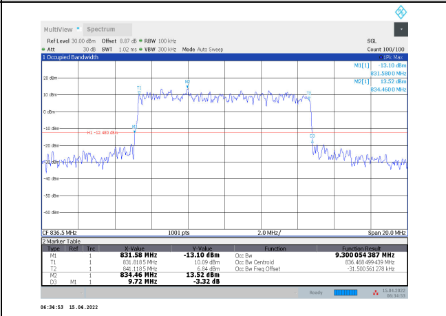
1-N5-PC3-15-10-M-2-CP-16QAM-Outer_Full-52@0 -Ant1-9.3-9.720-≤10-PASS
