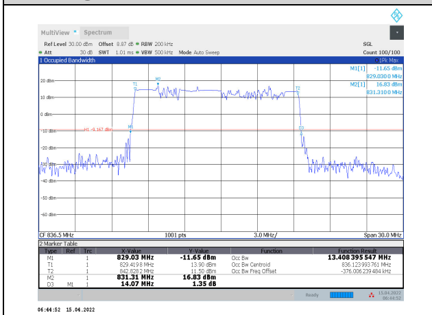
1-N5-PC3-15-15-M-6-DFT-QPSK-Outer_Full-75@ 0-Ant1-13.408-14.070-≤15-PASS
