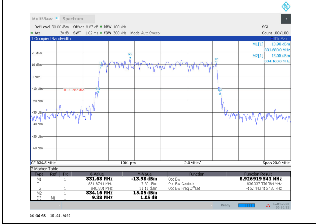
1-N5-PC3-15-10-M-9-DFT-256QAM-Outter_Full-50 @0-Ant1-8.927-9.380-≤10-PASS
