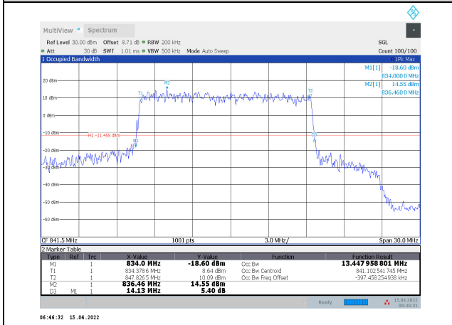
1-N5-PC3-15-15-H-1-CP-QPSK-Outer_Full-75@0- Ant1-13.448-14.130-≤15-PASS
