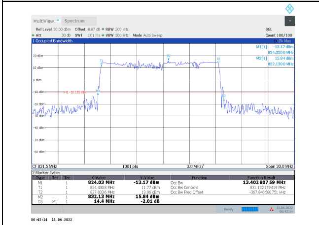
1-N5-PC3-15-15-L-7-DFT-16QAM-Outer_Full-75@0-Ant1-13.403-14.400-≤15-PASS
