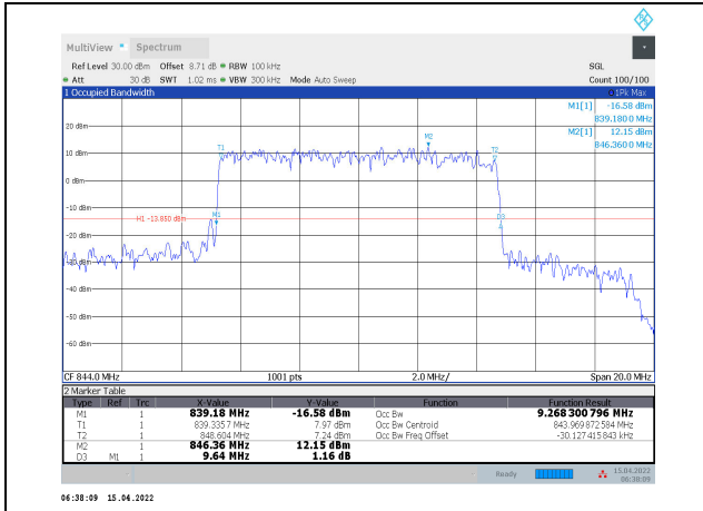
1-N5-PC3-15-10-H-2-CP-16QAM-Outer_Full-52@ 0-Ant1-9.268-9.640-≤10-PASS
