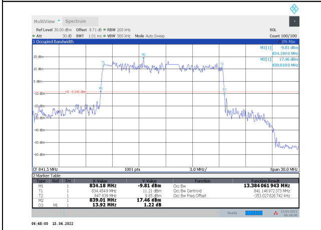
1-N5-PC3-15-15-H-7-DFT-16QAM-Outter_Full-75@0 -Ant1-13.384-13.920-≤15-PASS
