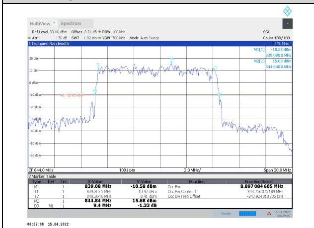
1-N5-PC3-15-10-H-6-DFT-QPSK-Outer_Full-50@0- -Ant1-8.897-9.400-≤10-PASS
