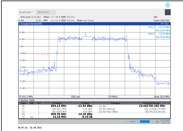
1-N5-PC3-15-15-H-5-DFT-PI/2BPSK-Outter_Full-75 @0-Ant1-13.444-14.160-≤15-PASS
