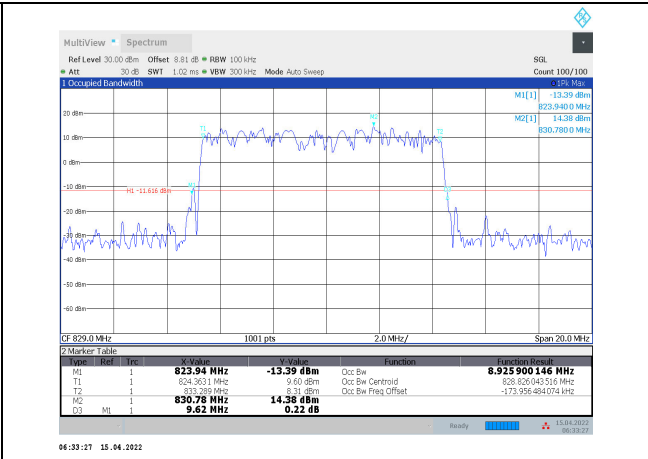
1-N5-PC3-15-10-L-9-DFT-256QAM-Outer_Full-50@ 0-Ant1-8.926-9.620-≤10-PASS
