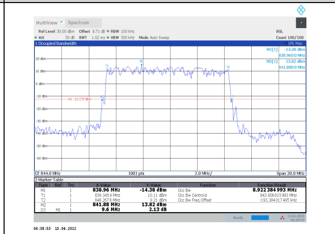
1-N5-PC3-15-10-H-5-DFT-PI/2BPSK-Outer_Full-50 @0-Ant1-8.922-9.600-≤10-PASS
