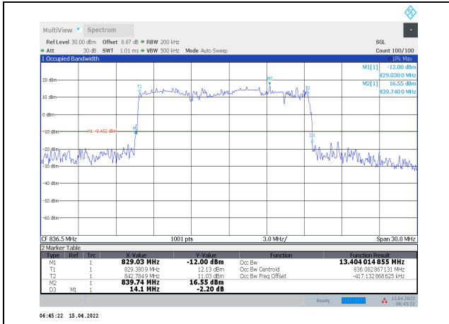
1-N5-PC3-15-15-M-8-DFT-64QAM-Outer_Full-75@ 0-Ant1-13.404-14.100-≤15-PASS
