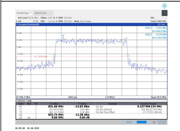
1-N5-PC3-15-10-M-3-CP-64QAM-Outer_Full-52@ 0-Ant1-9.258-9.660-≤10-PASS
