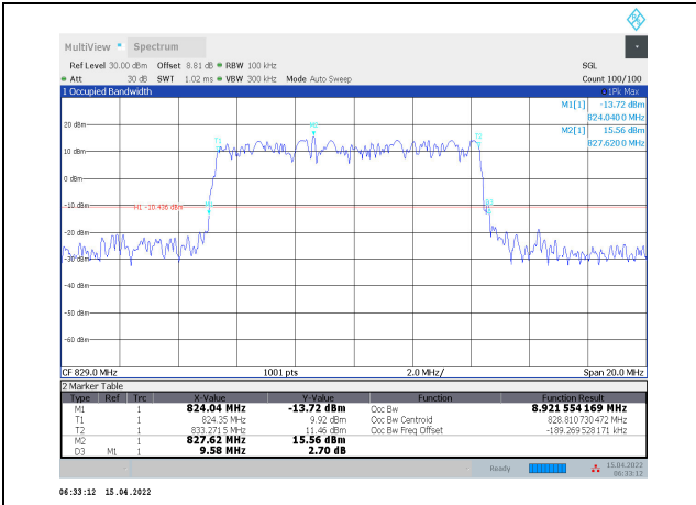
1-N5-PC3-15-10-L-8-DFT-64QAM-Outer_Full-50@ 0-Ant1-8.922-9.580-≤10-PASS
