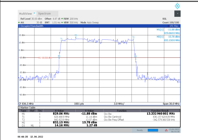
1-N5-PC3-15-15-M-5-DFT-PI/2BPSK-Outer_Full-75 @0-Ant1-13.333-14.160-≤15-PASS
