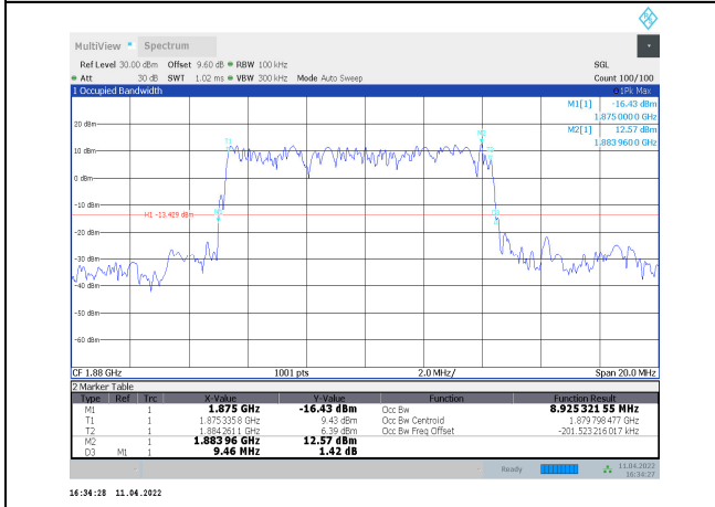
1-N2-PC3-15-10-M-5-DFT-PI/2BPSK-Outer_Full-50@0-Ant1-8.925-9.460-≤10-PASS
