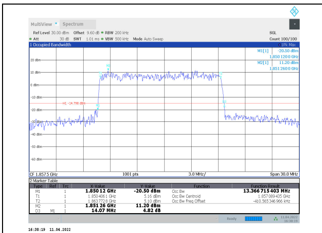
1-N2-PC3-15-15-L-1-CP-QPSK-Outer_Full-75@0-Ant1-13.367-14.070-≤15-PASS
