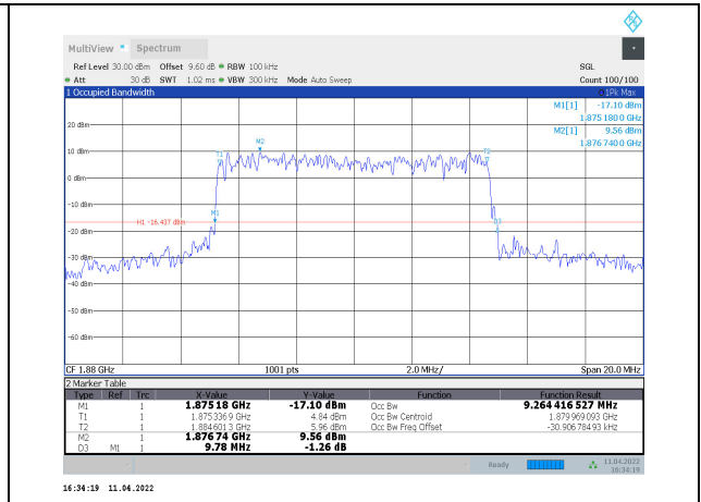
1-N2-PC3-15-10-M-4-CP-256QAM-Outer_Full-52@0-Ant1-9.264-9.780-≤10-PASS
