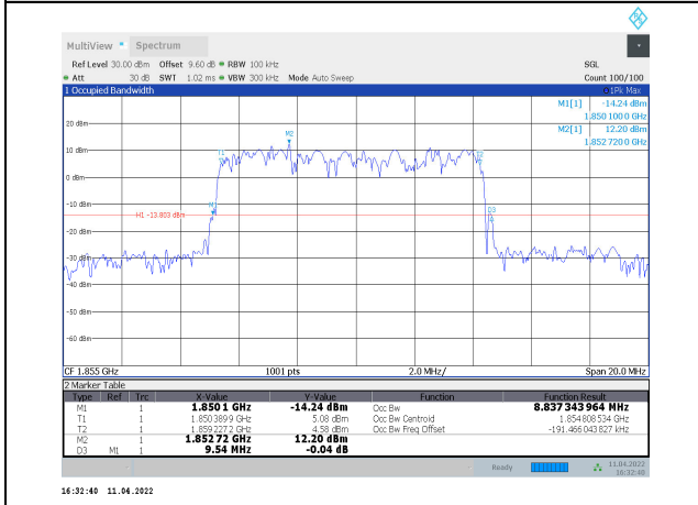
1-N2-PC3-15-10-L-8-DFT-64QAM-Outer_Full-50@0-Ant1-8.837-9.540-≤10-PASS
