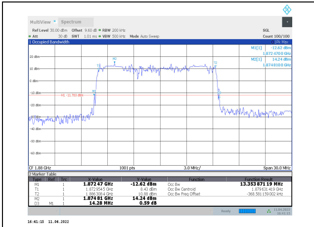
1-N2-PC3-15-15-M-6-DFT-QPSK-Outter_Full-75@0 -Ant1-13.354-14.280-≤15-PASS
