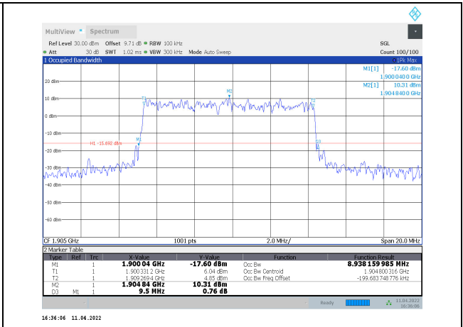
1-N2-PC3-15-10-H-1-CP-QPSK-Outer_Full-50@0-Ant1-8.938-9.500-≤10-PASS
