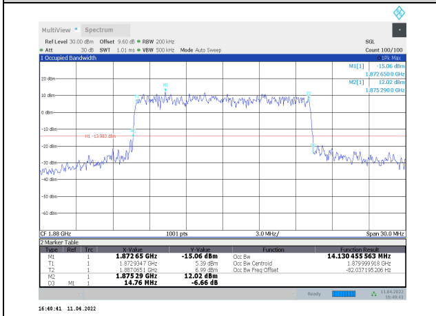
1-N2-PC3-15-15-M-2-CP-16QAM-Outer_Full-79@0-Ant1-14.13-14.760-≤15-PASS
