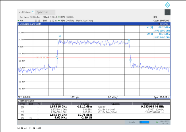
1-N2-PC3-15-10-M-2-CP-16QAM-Outer_Full-52@0-Ant1-9.254-9.620-≤10-PASS
