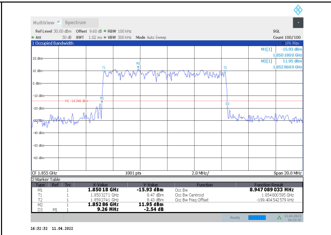
1-N2-PC3-15-10-L-7-DFT-16QAM-Outer_Full-50@0-Ant1-8.947-9.260-≤10-PASS
