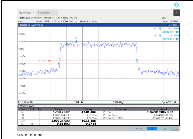
1-N2-PC3-15-10-H-2-CP-16QAM-Outer_Full-52@0-Ant1-9.262-9.580-≤10-PASS
