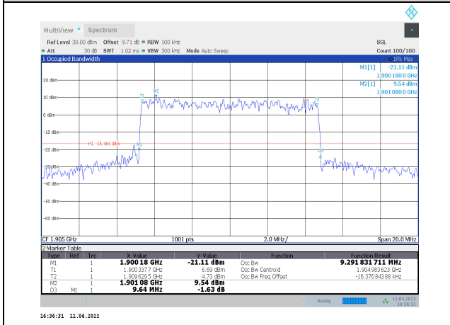
1-N2-PC3-15-10-H-4-CP-256QAM-Outer_Full-52@0-Ant1-9.292-9.640-≤10-PASS
