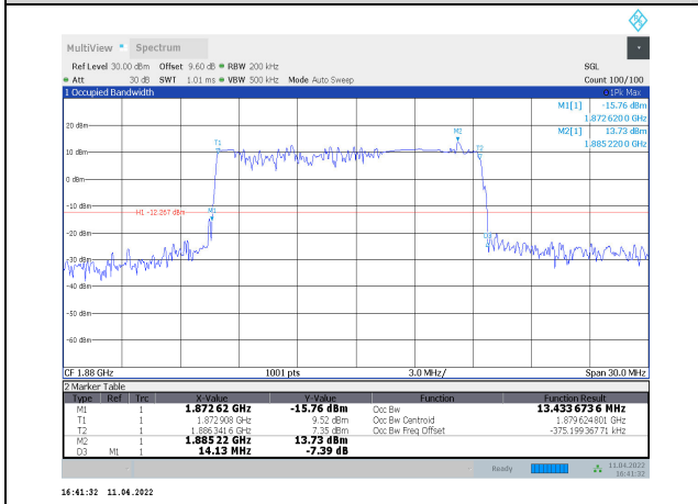
1-N2-PC3-15-15-M-8-DFT-64QAM-Outter_Full-75@0-Ant1-13.434-14.130-≤15-PASS
