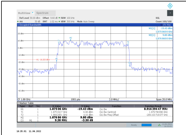
1-N2-PC3-15-10-M-9-DFT-256QAM-Outer_Full-50 @0-Ant1-8.916-9.380-≤10-PASS
