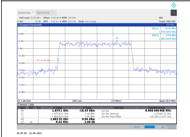
1-N2-PC3-15-10-M-1-CP-QPSK-Outer_Full-50@0-Ant1-8.968-9.440-≤10-PASS
