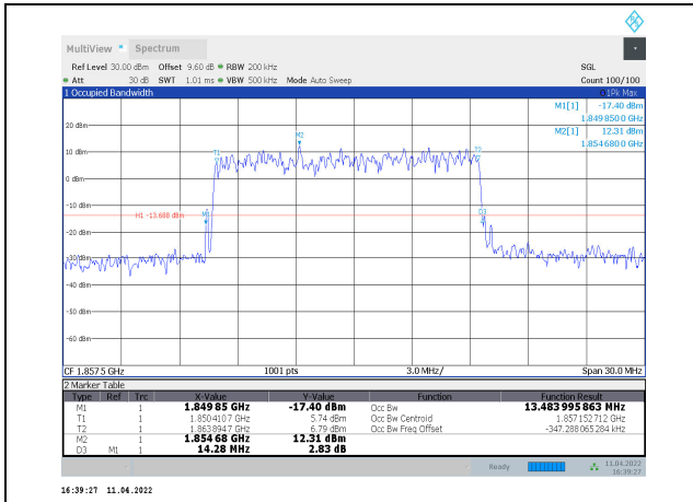
1-N2-PC3-15-15-L-9-DFT-256QAM-Outer_Full-75 @0-Ant1-13.484-14.280-≤15-PASS
