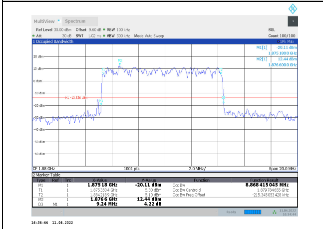
1-N2-PC3-15-10-M-7-DFT-16QAM-Outer_Full-50@0-Ant1-8.868-9.240-≤10-PASS
