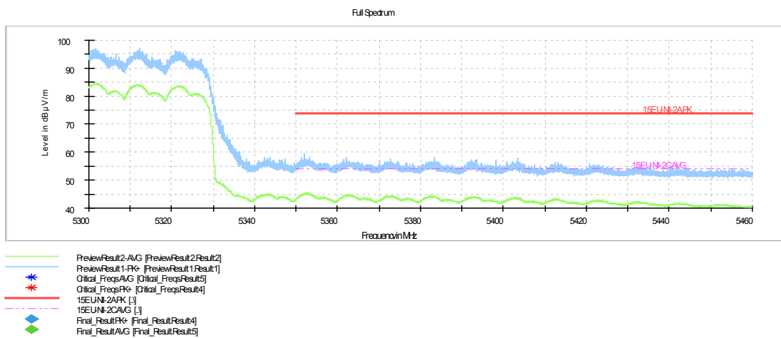
Fig.42 Band Edges (802.11ax-HT160 Ch50-R, 5250MHz)
