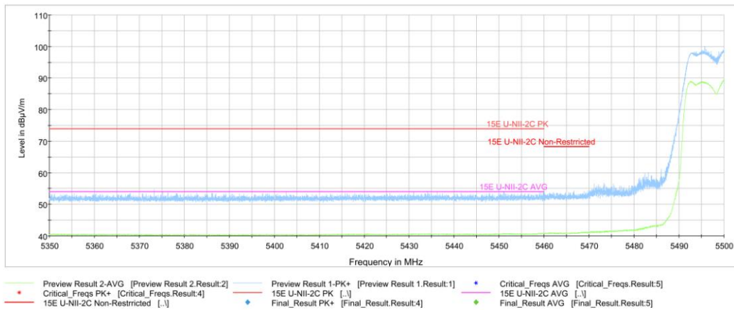
Fig.11 Band Edges (802.11n-HT40 Ch102, 5510MHz)
