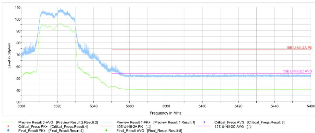
Fig.30 Band Edges (802.11ax-HT20 Ch64, 5320MHz)
