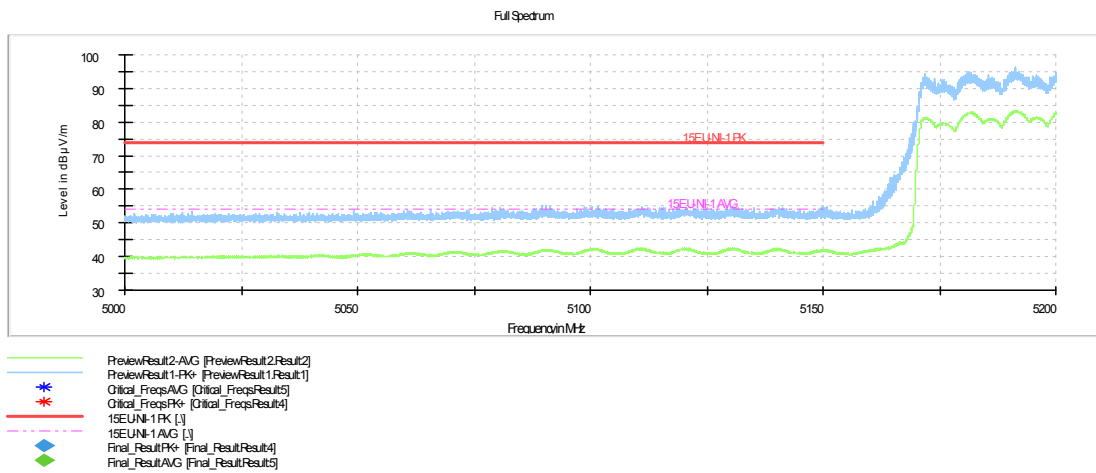
Fig.41 Band Edges (802.11ax-HT160 Ch50-L, 5250MHz)
