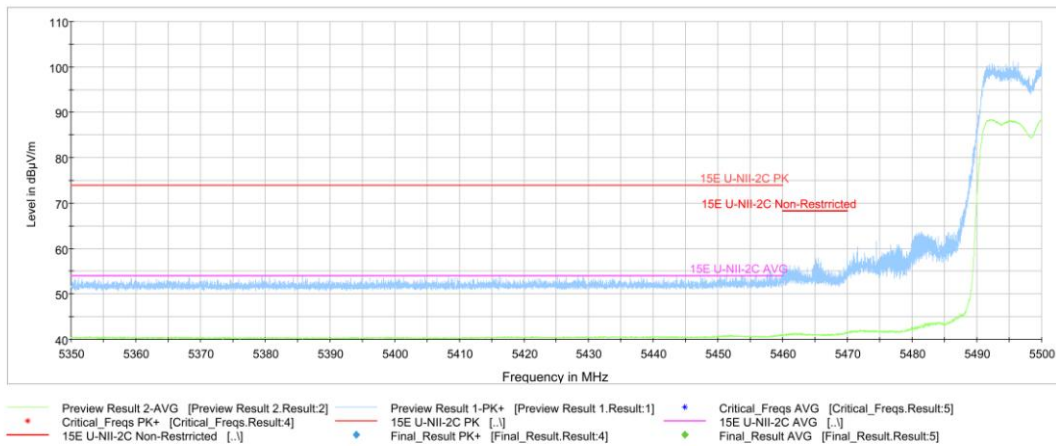
Fig.35 Band Edges (802.11ax-HT40 Ch102, 5510MHz)
