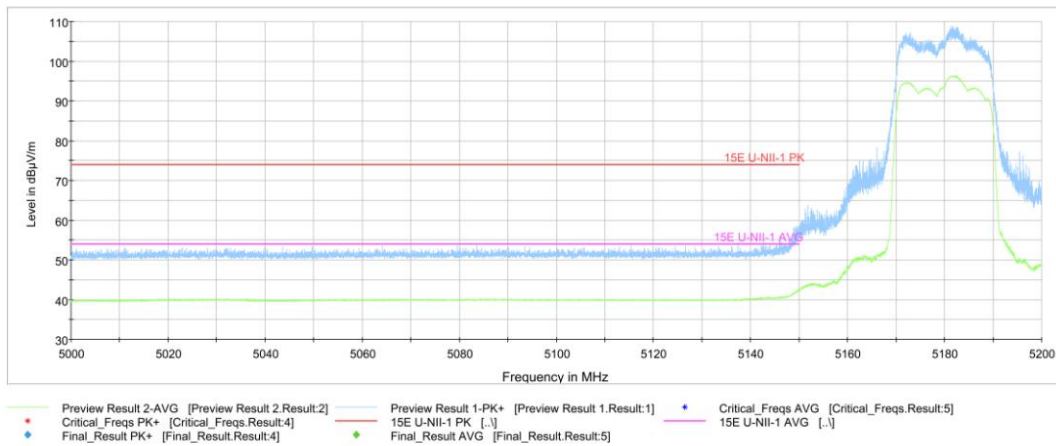
Fig.29 Band Edges (802.11ax-HT20 Ch36, 5180MHz)
