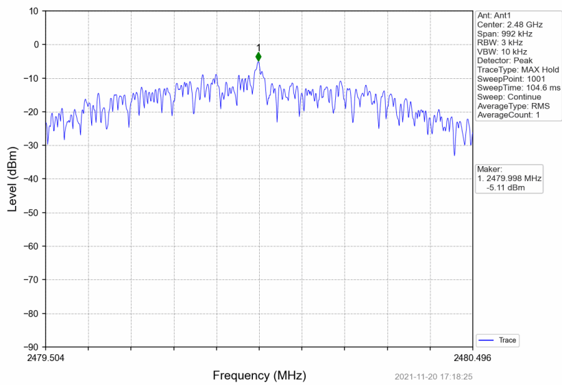
1M_HCH_2480MHz_DataRate=_ Ant1_NTNV
