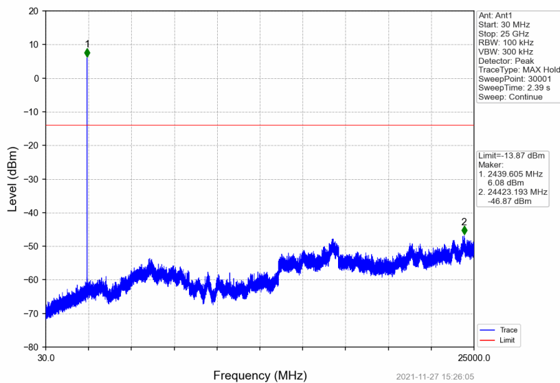
1M_MCH_2440MHz_DataRate=_ Ant1_NTNV
