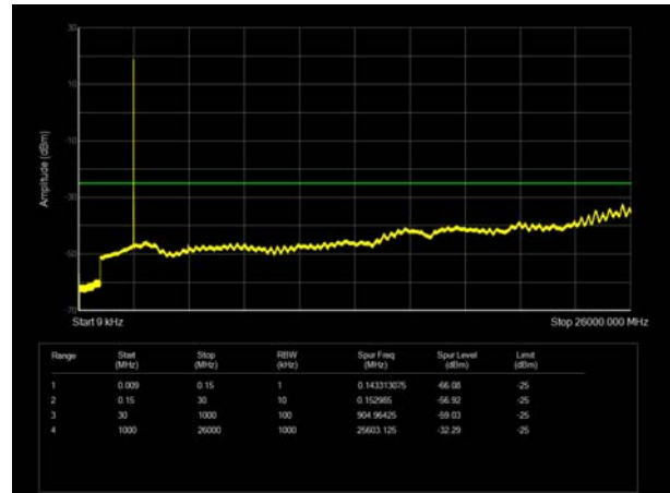
LTE Band 38 10MHz CH- Middle 9kHz~26GHz
