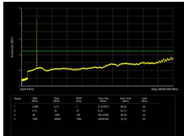
LTE Band 38 10MHz CH- High 9kHz~26GHz
