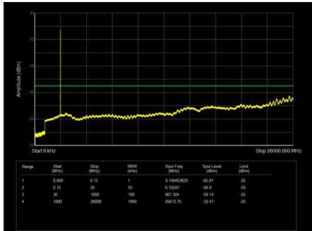
LTE Band 38 5MHz CH- Middle 9kHz~26GHz
