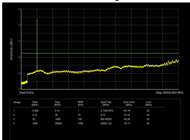
LTE Band 38 5MHz CH-High 9kHz~26GHz
