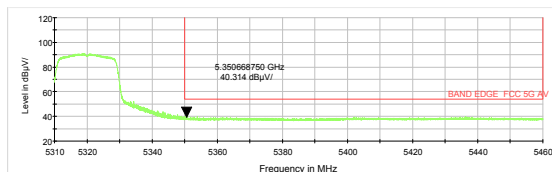
802.11n HT40-Channel 62: Peak
