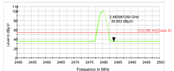
3DH5-Channel 78: Average
