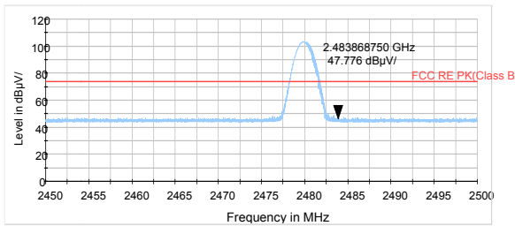
DH5-Channel 78: Peak
