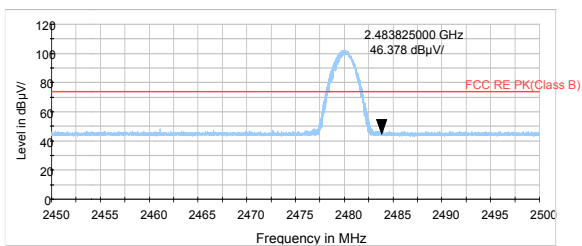
3DH5-Channel 78: Peak
