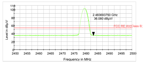
DH5-Channel 78: Average
