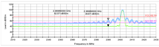
Bluetooth LE (1M) Channel 0 Peak+ Average
