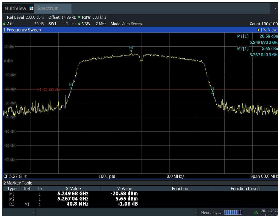
Fig.23 Occupied 26dB Bandwidth (802.11n-HT40, 5270MHz)
