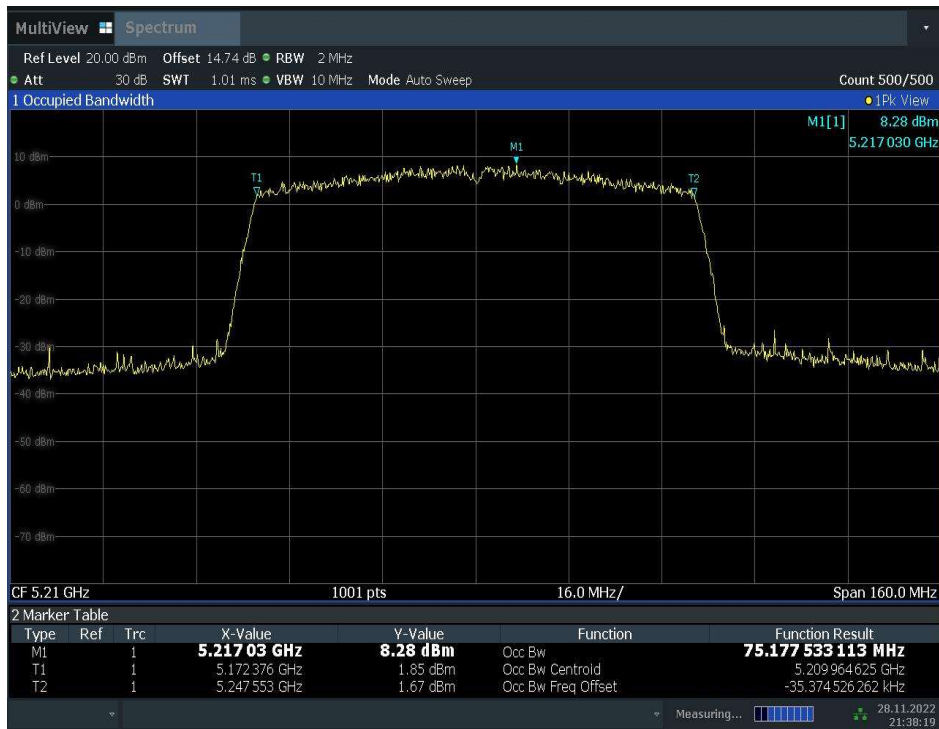
Fig.42 99% Occupied bandwidth (802.11ac-VHT80, 5210MHz)
