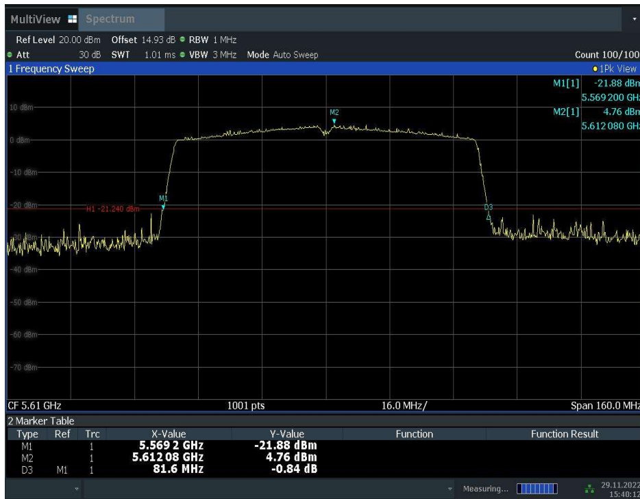
Fig.32 Occupied 26dB Bandwidth (802. 11ac-VHT80, 5610MHz)
