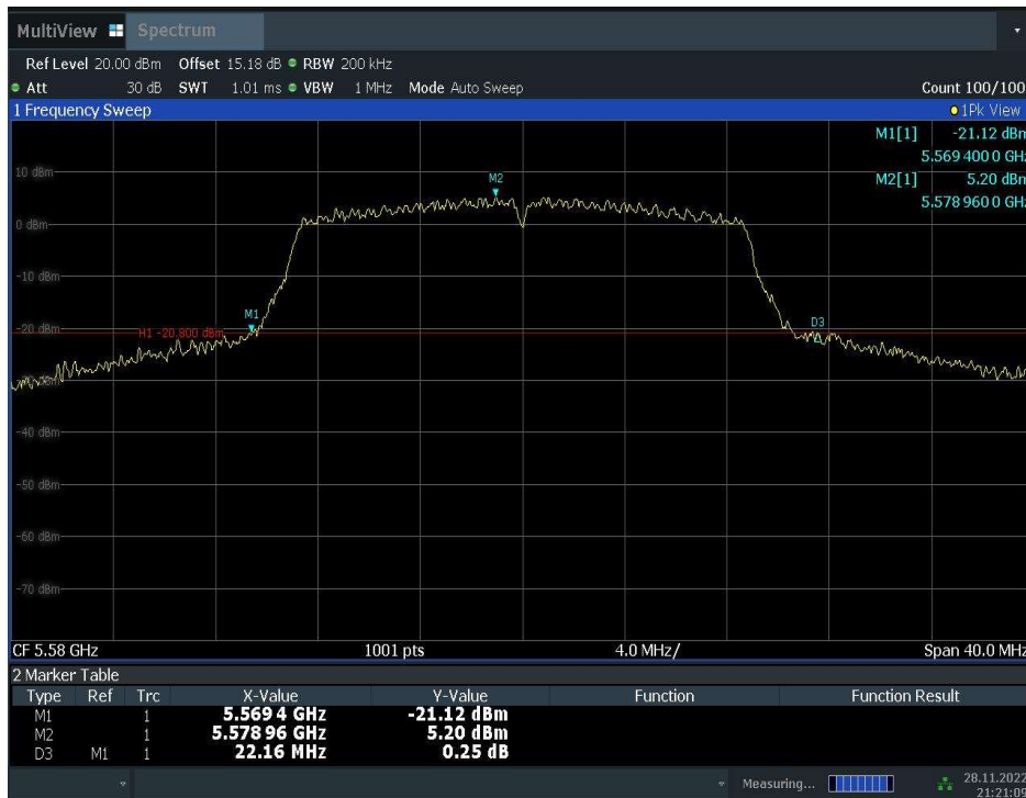
Fig.18 Occupied 26dB Bandwidth (802. 11ac-VHT20, 5580MHz)
