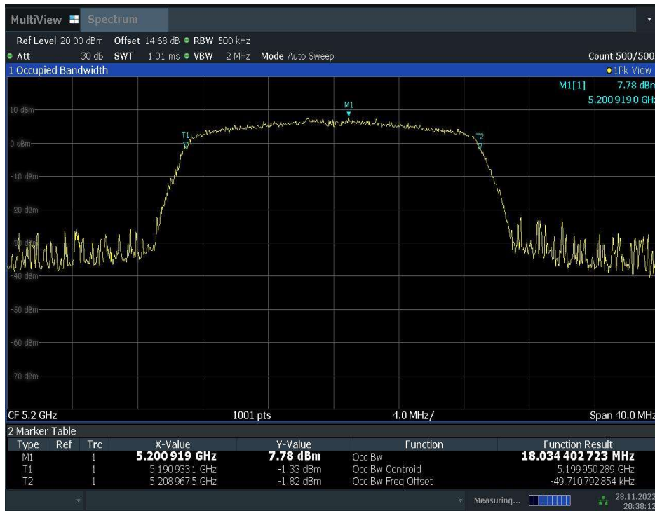
Fig.38 99% Occupied bandwidth (802.11ac-VHT20, 5200MHz)
