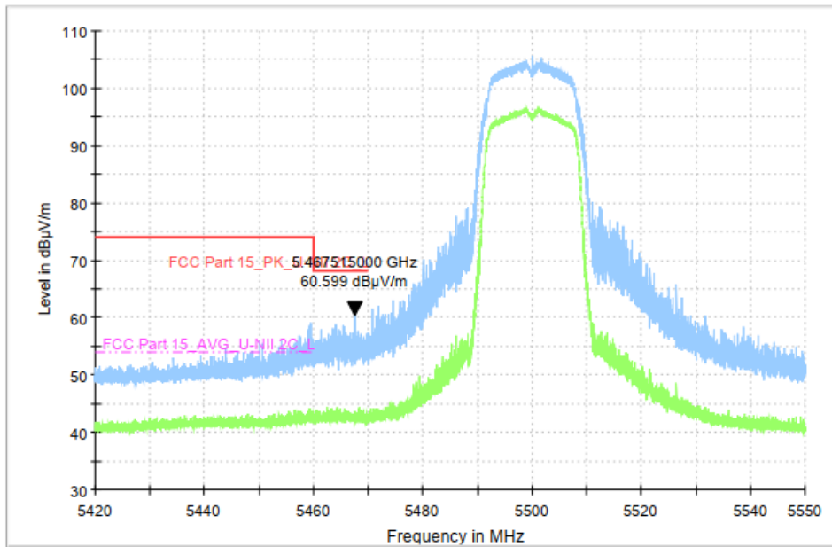
Fig. 3 Band Edges (802.11a, CH100 5500MHz)
