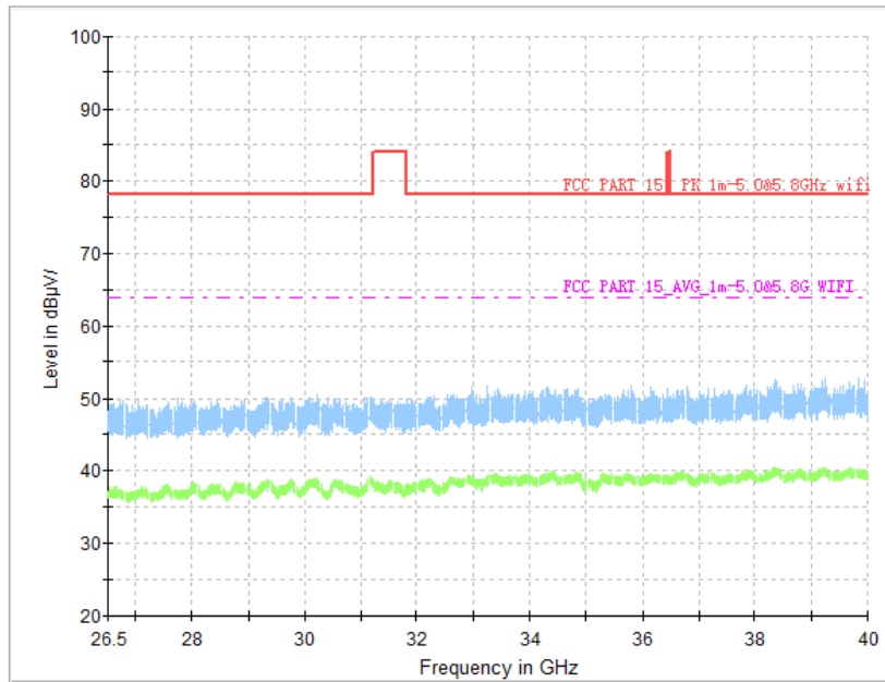
Fig. 46 Transmitter Spurious Emission (All channel, 26.5GHz~40GHz)
