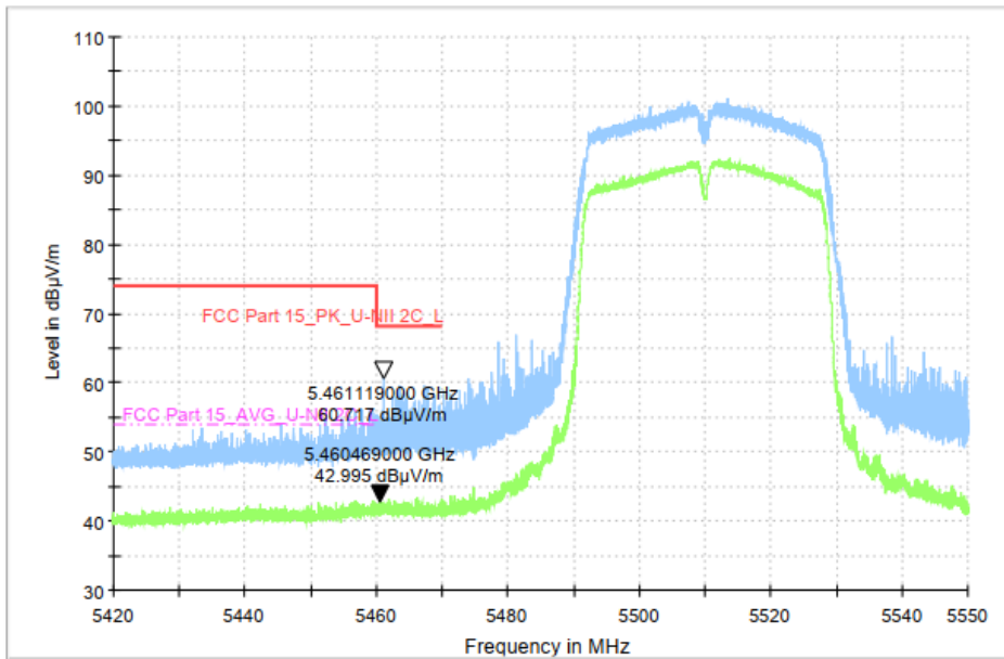
Fig. 9 Band Edges (802.11ac-VHT40, CH102 5510MHz)
