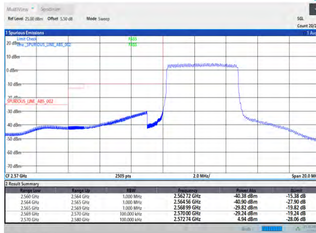
Band38-5MHz-QPSK-37775-25RB#0
