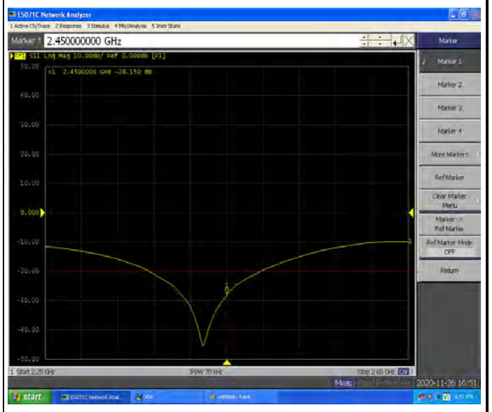
Return Loss-Head
