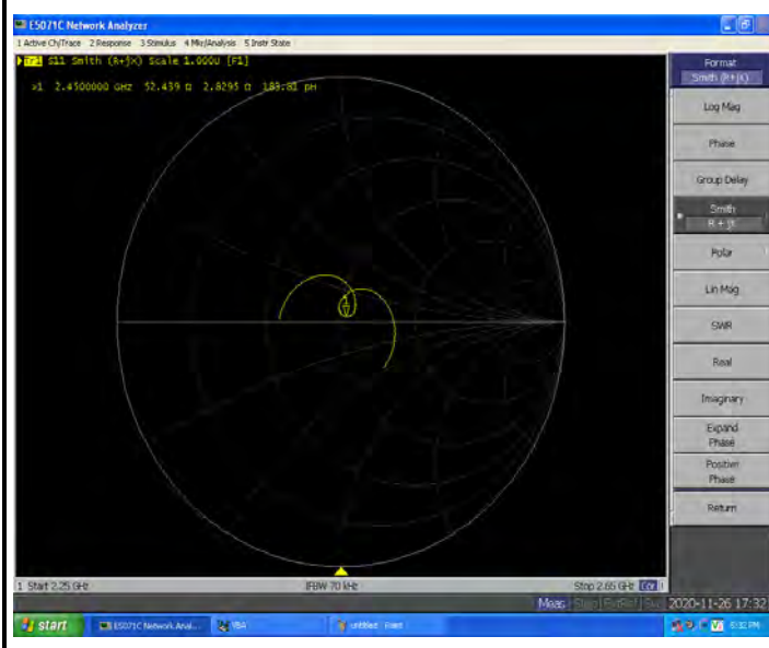
Impedance Test-Head
