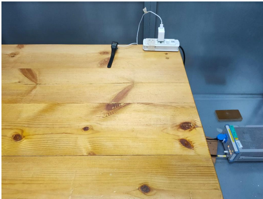
8. Conducted Emission (Part 15C, Bluetooth)
