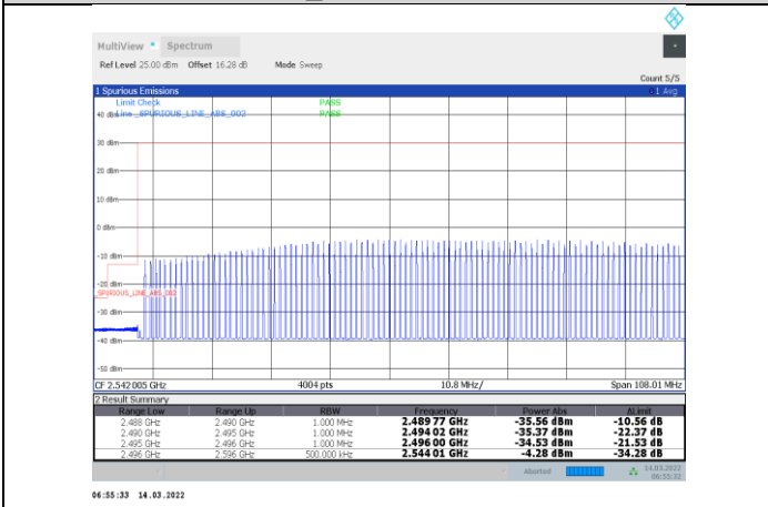
1-N41-PC3-30-100-L-31-CP-OFDM 64QAM-Outer_Full-273@0-Ant1-PASS
