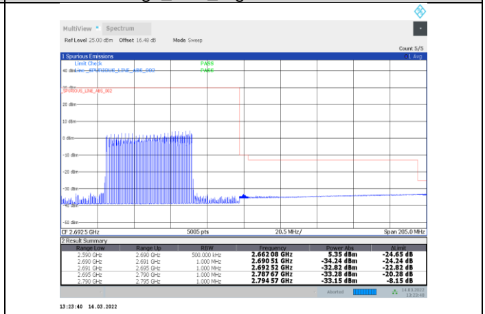
1-N41-PC3-30-100-H-4-DFT-s-OFDM PI/2 BPSK-Inner_Full-135@67-Ant1-PASS
