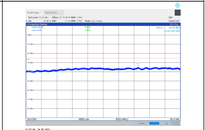
1-N41-PC3-30-60-M-3-CP-OFDM QPSK-Outer_Full-162 @0-18000-26500-Ant1--34.29--25-PASS
