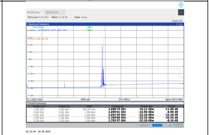
1-N41-PC3-30-100-H-2-DFT-s-OFDM PI/2 BPSK-Edge_1RB_Right-1@272-Ant1-PASS
