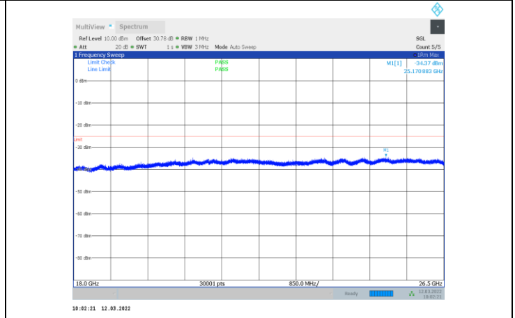
1-N41-PC3-30-20-L-3-CP-OFDM QPSK-Outter_Full-51 @0-18000-26500-Ant1--34.37--25-PASS
