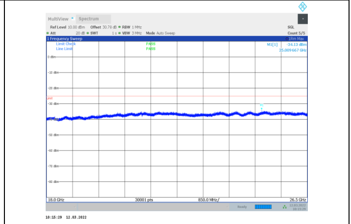
1-N41-PC3-30-20-H-2-CP-OFDM QPSK-Edge_1RB_Right-1 @50-18000-26500-Ant1--34.13--25-PASS
