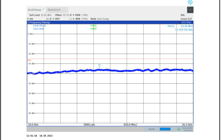
1-N41-PC3-30-60-H-1-CP-OFDM QPSK-Edge_1RB_Left-1 @0-18000-26500-Ant1--34.48--25-PASS
