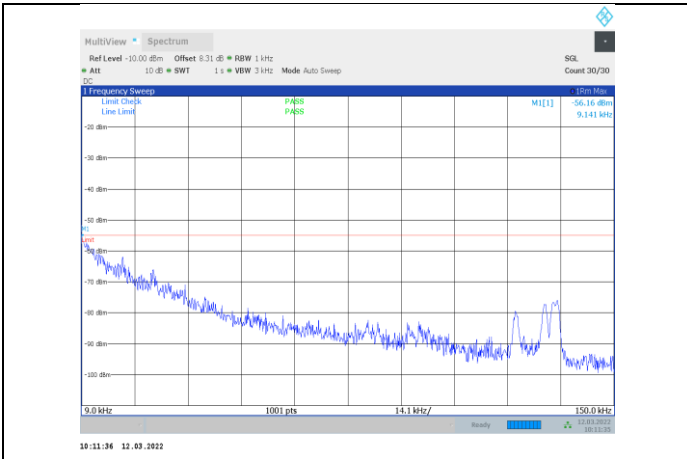
1-N41-PC3-30-20-H-1-CP-OFDM QPSK-Edge_1RB_Left-1 @0-0.009-0.15-Ant1--56.16--55-PASS
