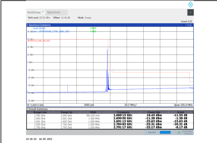
1-N41-PC3-30-100-H-22-CP-OFDM QPSK-Edge_1RB_Right-1@272-Ant1-PASS
