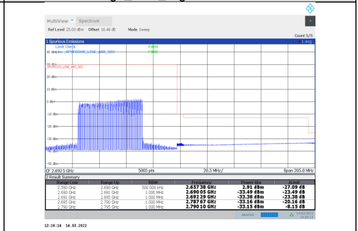
1-N41-PC3-30-100-H-12-DFT-s-OFDM 16QAM-Inner_Full-135@67-Ant1-PASS
