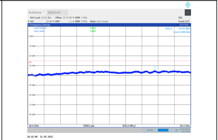
1-N41-PC3-30-20-H-1-CP-OFDM QPSK-Edge_1RB_Left-1 @0-18000-26500-Ant1--34.55--25-PASS
