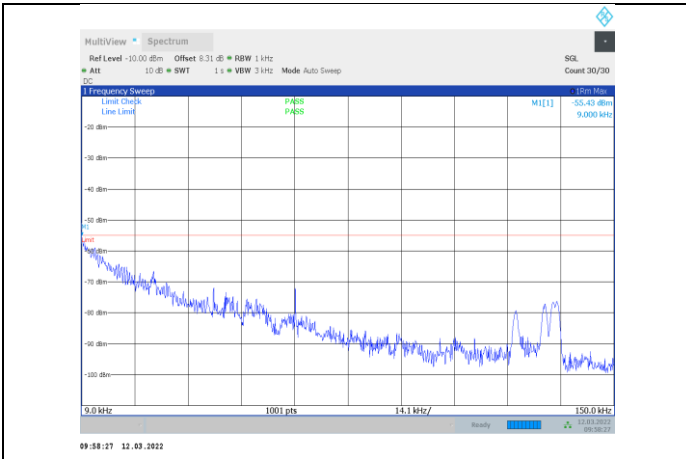
1-N41-PC3-30-20-L-2-CP-OFDM QPSK-Edge_1RB_Right-1 @50-0.009-0.15-Ant1--55.43--55-PASS
