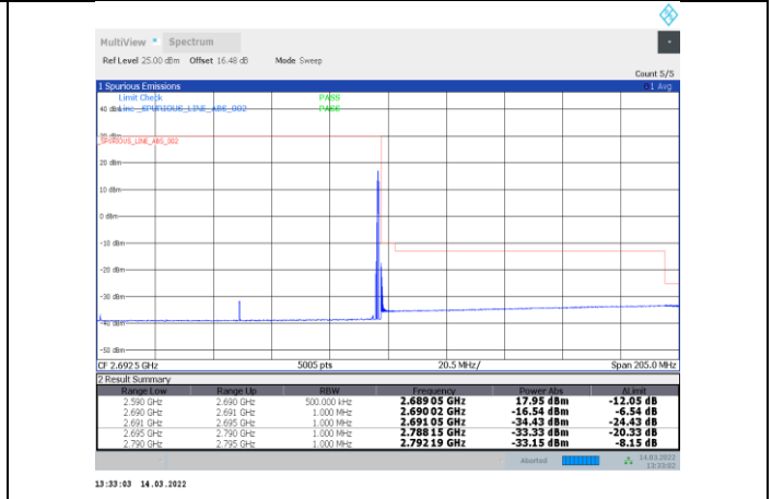
1-N41-PC3-30-100-H-34-CP-OFDM 256QAM-Edge_1RB_Right-1@272-Ant1-PASS
