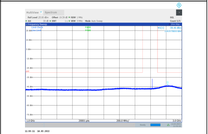
1-N41-PC3-30-60-M-2-CP-OFDM QPSK-Edge_1RB_Right-1 @161-1000-3000-Ant1--38.46--25-PASS
