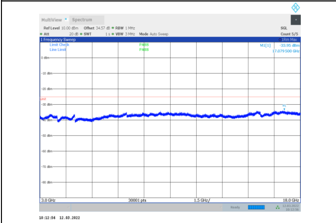
1-N41-PC3-30-20-H-1-CP-OFDM QPSK-Edge_1RB_Left-1 @0-3000-18000-Ant1--33.95--25-PASS
