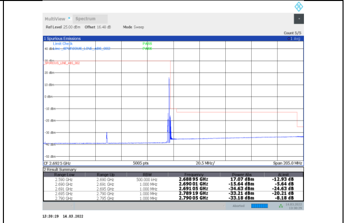
1-N41-PC3-30-100-H-26-CP-OFDM 16QAM-Edge_1RB_Right-1@272-Ant1-PASS
