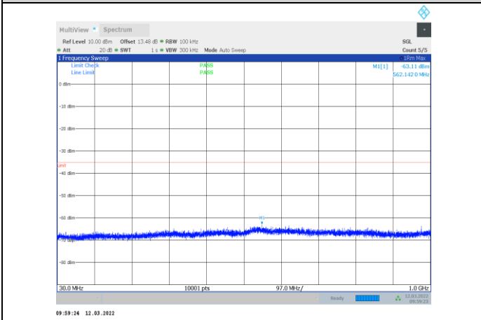
1-N41-PC3-30-20-L-2-CP-OFDM QPSK-Edge_1RB_Right-1 @50-30-1000-Ant1--63.11--35-PASS
