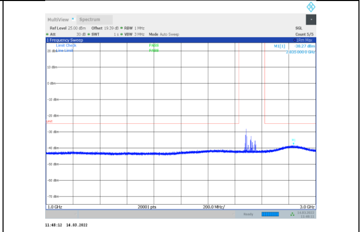
1-N41-PC3-30-60-L-3-CP-OFDM QPSK-Outer_Full-162 @0-1000-3000-Ant1--38.27--25-PASS
