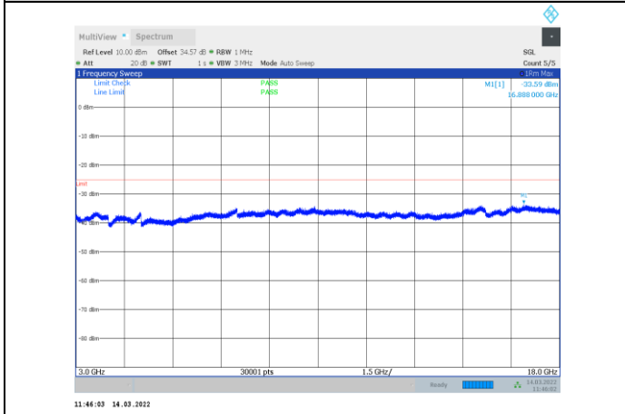
1-N41-PC3-30-60-L-2-CP-OFDM QPSK-Edge_1RB_Right-1 @161-3000-18000-Ant1--33.59--25-PASS
