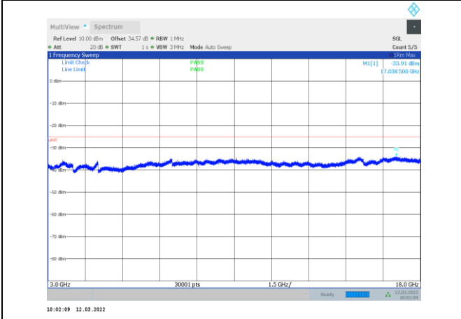
1-N41-PC3-30-20-L-3-CP-OFDM QPSK-Outter_Full-51 @0-3000-18000-Ant1--33.91--25-PASS
