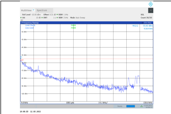
1-N41-PC3-30-20-M-3-CP-OFDM QPSK-Outter_Full-51 @0-0.009-0.15-Ant1--55.82--55-PASS
