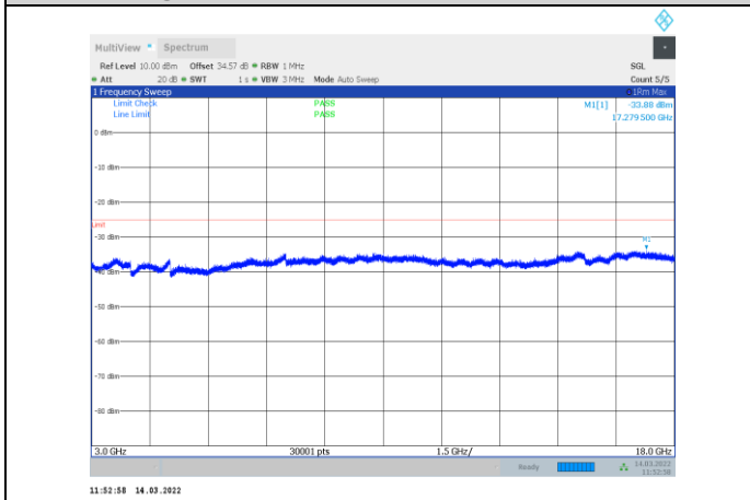
1-N41-PC3-30-60-M-1-CP-OFDM QPSK-Edge_1RB_Left-1 @0-3000-18000-Ant1--33.88--25-PASS
