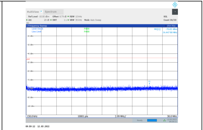
1-N41-PC3-30-20-L-2-CP-OFDM QPSK-Edge_1RB_Right-1 @50-0.15-30-Ant1--75.02--45-PASS
