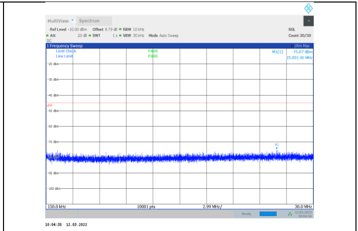
1-N41-PC3-30-20-M-1-CP-OFDM QPSK-Edge_1RB_Left-1 @0-0.15-30-Ant1--75.07--45-PASS
