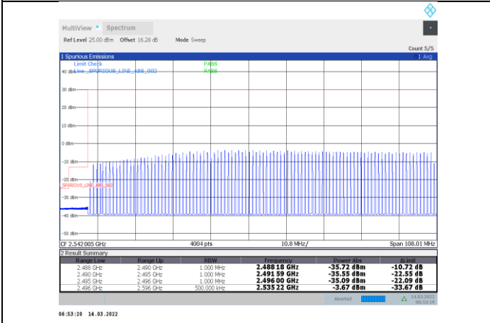
1-N41-PC3-30-100-L-23-CP-OFDM QPSK-Outer_Full-273@0-Ant1-PASS
