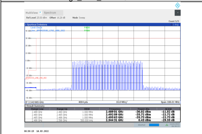
1-N41-PC3-30-100-L-12-DFT-s-OFDM 16QAM-Inner_Full-135@67-Ant1-PASS
