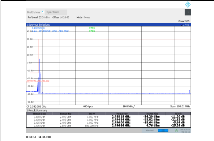
1-N41-PC3-30-100-L-33-CP-OFDM 256QAM-Edge_1RB_Left-1@0-Ant1-PASS
