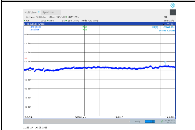
1-N41-PC3-30-60-M-2-CP-OFDM QPSK-Edge_1RB_Right-1 @161-3000-18000-Ant1--33.64--25-PASS
