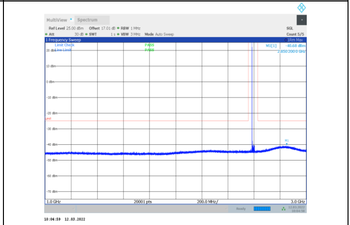
1-N41-PC3-30-20-M-1-CP-OFDM QPSK-Edge_1RB_Left-1 @0-1000-3000-Ant1--40.68--25-PASS
