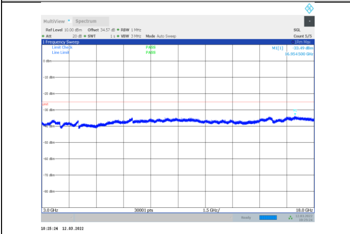
1-N41-PC3-30-20-H-3-CP-OFDM QPSK-Outter_Full-51 @0-3000-18000-Ant1--33.49--25-PASS
