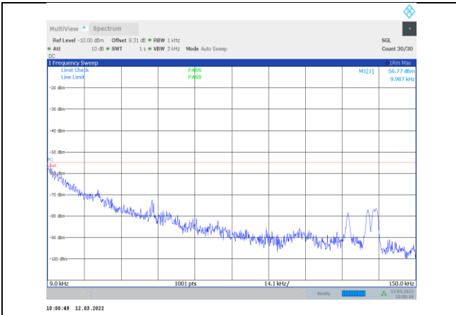
1-N41-PC3-30-20-L-3-CP-OFDM QPSK-Outter_Full-51 @0-0.009-0.15-Ant1--56.77--55-PASS
