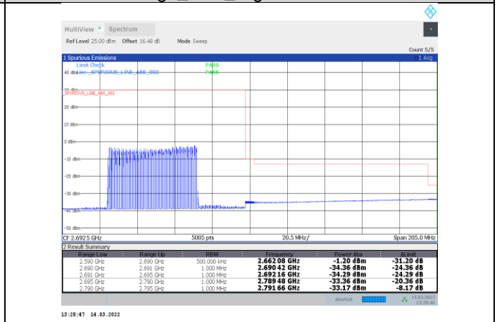
1-N41-PC3-30-100-H-20-DFT-s-OFDM 256QAM-Inner_Full-135@67-Ant1-PASS
