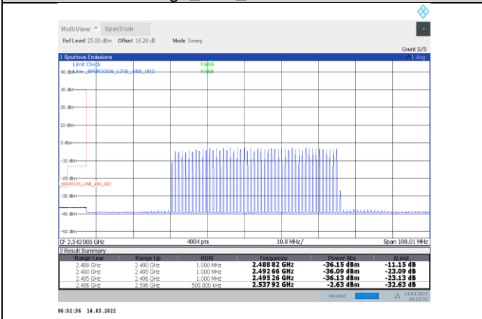
1-N41-PC3-30-100-L-20-DFT-s-OFDM 256QAM-Inner_Full-135@67-Ant1-PASS
