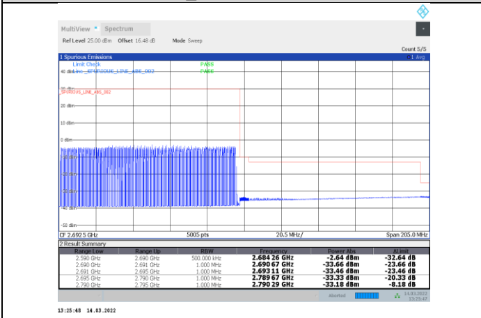
1-N41-PC3-30-100-H-11-DFT-s-OFDM 16QAM-Outer_Full-270@0-Ant1-PASS
