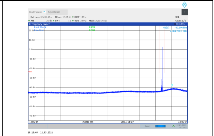
1-N41-PC3-30-20-H-2-CP-OFDM QPSK-Edge_1RB_Right-1 @50-1000-3000-Ant1--40.69--25-PASS
