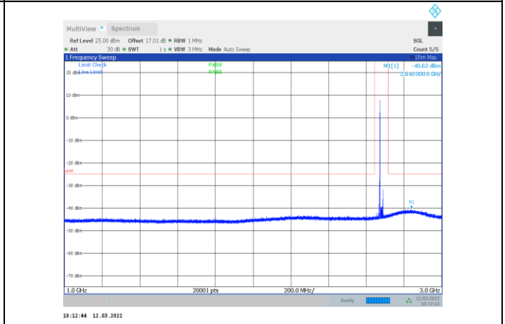
1-N41-PC3-30-20-H-1-CP-OFDM QPSK-Edge_1RB_Left-1 @0-1000-3000-Ant1--40.62--25-PASS
