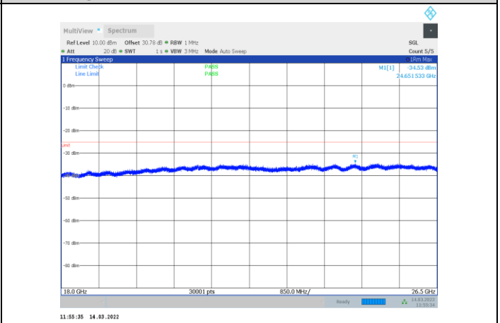
1-N41-PC3-30-60-M-2-CP-OFDM QPSK-Edge_1RB_Right-1 @161-18000-26500-Ant1--34.53--25-PASS
