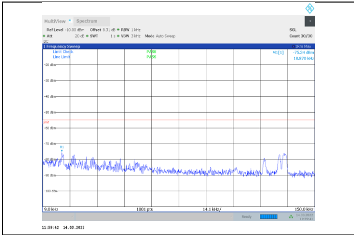
1-N41-PC3-30-60-H-1-CP-OFDM QPSK-Edge_1RB_Left-1 @0-0.009-0.15-Ant1--75.34--55-PASS
