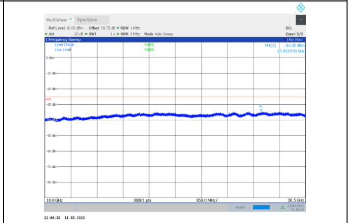
1-N41-PC3-30-60-L-2-CP-OFDM QPSK-Edge_1RB_Right-1 @161-18000-26500-Ant1--34.42--25-PASS
