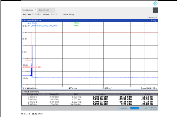
1-N41-PC3-30-100-L-17-DFT-s-OFDM 256QAM-Edge_1RB_Left-1@0-Ant1-PASS
