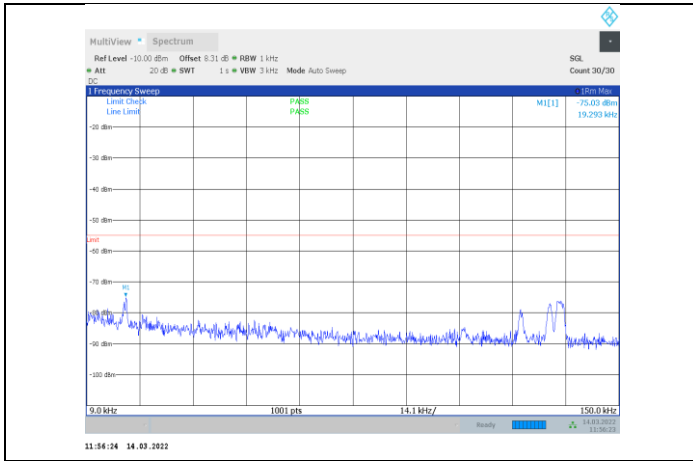
1-N41-PC3-30-60-M-3-CP-OFDM QPSK-Outer_Full-162 @0-0.009-0.15-Ant1--75.03--55-PASS
