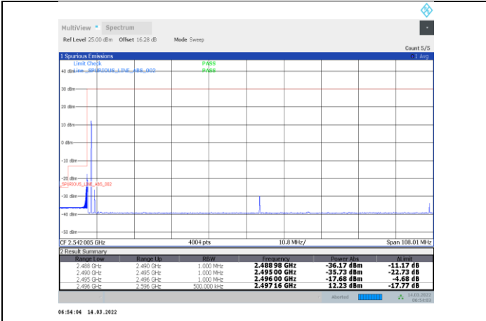
1-N41-PC3-30-100-L-25-CP-OFDM 16QAM-Edge_1RB_Left-1@0-Ant1-PASS
