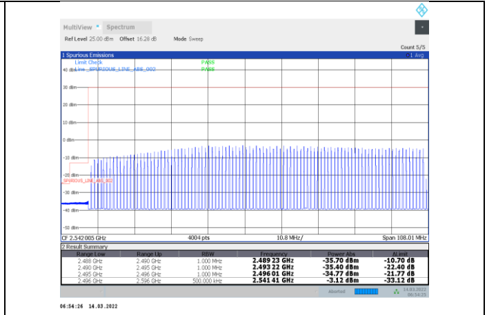
1-N41-PC3-30-100-L-27-CP-OFDM 16QAM-Outer_Full-273@0-Ant1-PASS
