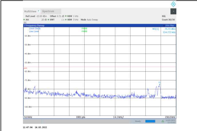
1-N41-PC3-30-60-L-3-CP-OFDM QPSK-Outer_Full-162 @0-0.009-0.15-Ant1--75.72--55-PASS
