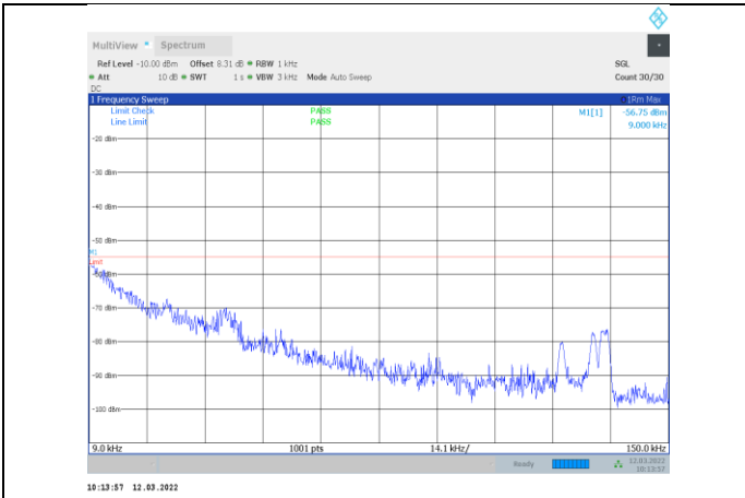
1-N41-PC3-30-20-H-2-CP-OFDM QPSK-Edge_1RB_Right-1 @50-0.009-0.15-Ant1--56.75--55-PASS
