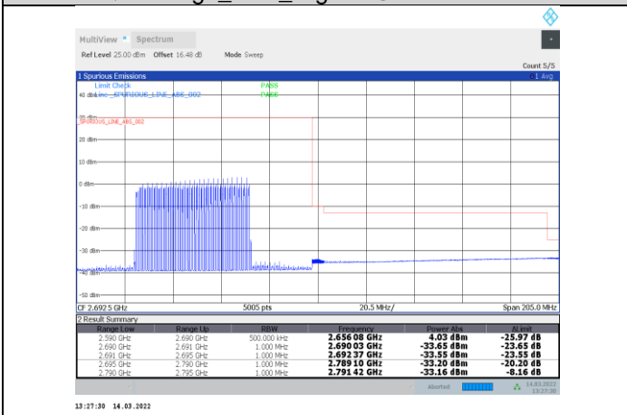
1-N41-PC3-30-100-H-16-DFT-s-OFDM 64QAM-Inner_Full-135@67-Ant1-PASS
