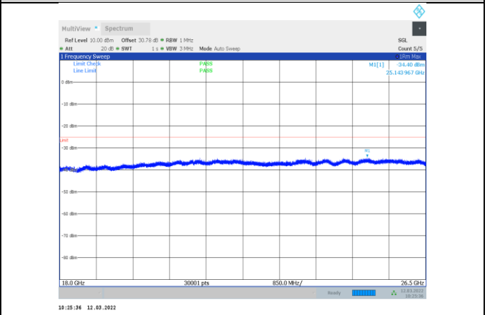
1-N41-PC3-30-20-H-3-CP-OFDM QPSK-Outter_Full-51 @0-18000-26500-Ant1--34.40--25-PASS
