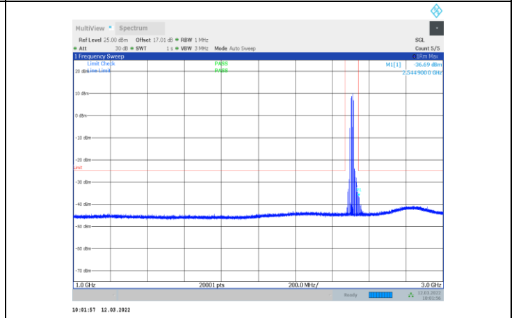
1-N41-PC3-30-20-L-3-CP-OFDM QPSK-Outter_Full-51 @0-1000-3000-Ant1--36.69--25-PASS
