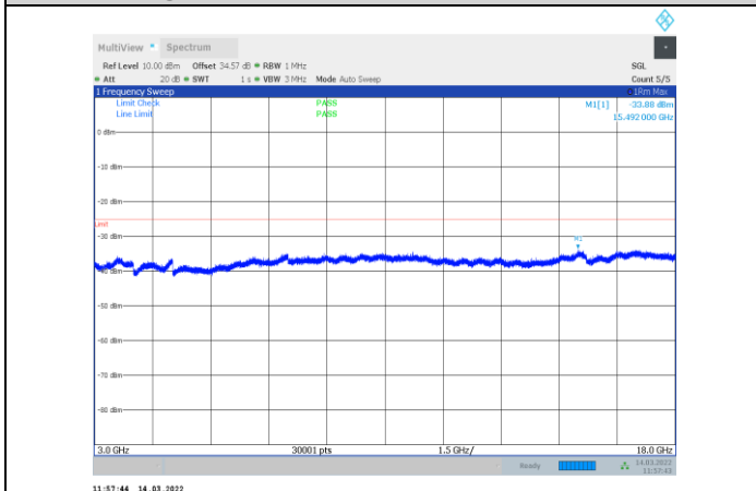
1-N41-PC3-30-60-M-3-CP-OFDM QPSK-Outer_Full-162 @0-3000-18000-Ant1--33.88--25-PASS
