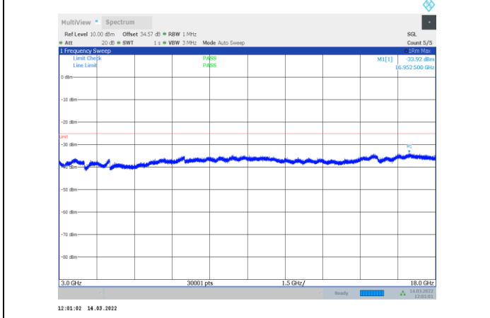
1-N41-PC3-30-60-H-1-CP-OFDM QPSK-Edge_1RB_Left-1 @0-3000-18000-Ant1--33.92--25-PASS
