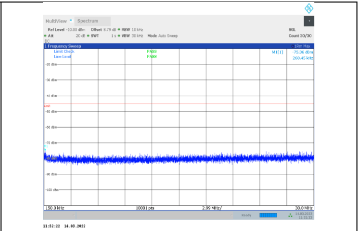
1-N41-PC3-30-60-M-1-CP-OFDM QPSK-Edge_1RB_Left-1 @0-0.15-30-Ant1--75.36--45-PASS
