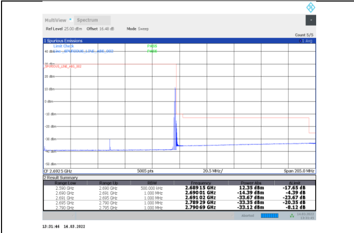
1-N41-PC3-30-100-H-30-CP-OFDM 64QAM-Edge_1RB_Right-1@272-Ant1-PASS
