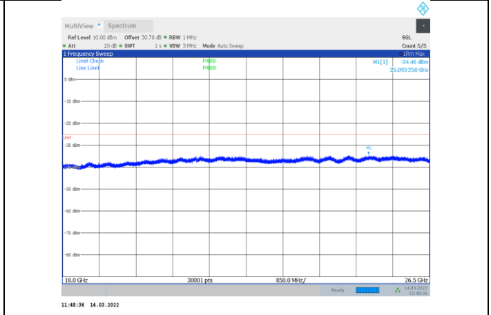
1-N41-PC3-30-60-L-3-CP-OFDM QPSK-Outer_Full-162 @0-18000-26500-Ant1--34.46--25-PASS
