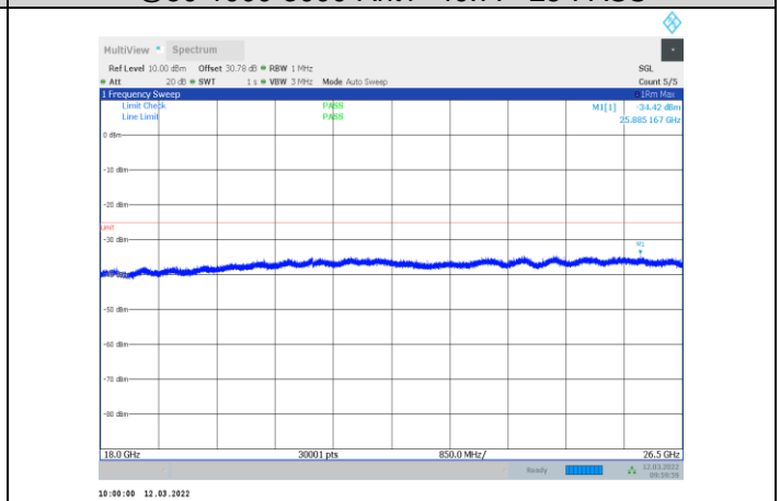
1-N41-PC3-30-20-L-2-CP-OFDM QPSK-Edge_1RB_Right-1 @50-18000-26500-Ant1--34.42--25-PASS
