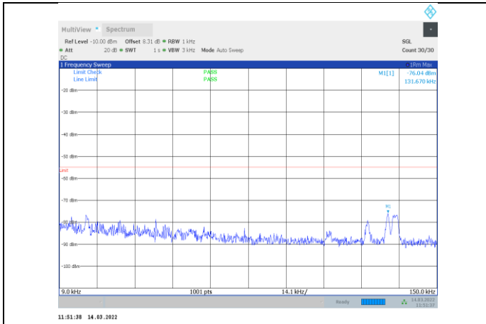
1-N41-PC3-30-60-M-1-CP-OFDM QPSK-Edge_1RB_Left-1 @0-0.009-0.15-Ant1--76.04--55-PASS
