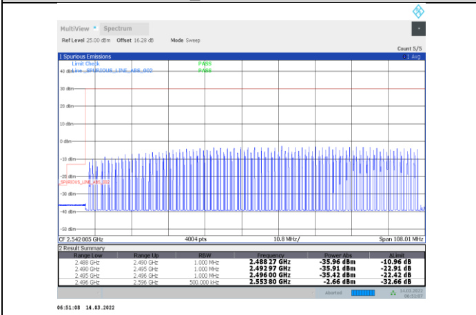
1-N41-PC3-30-100-L-15-DFT-s-OFDM 64QAM-Outer_Full-270@0-Ant1-PASS
