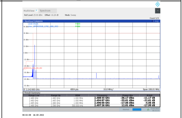
1-N41-PC3-30-100-L-21-CP-OFDM QPSK-Edge_1RB_Left-1@0-Ant1-PASS
