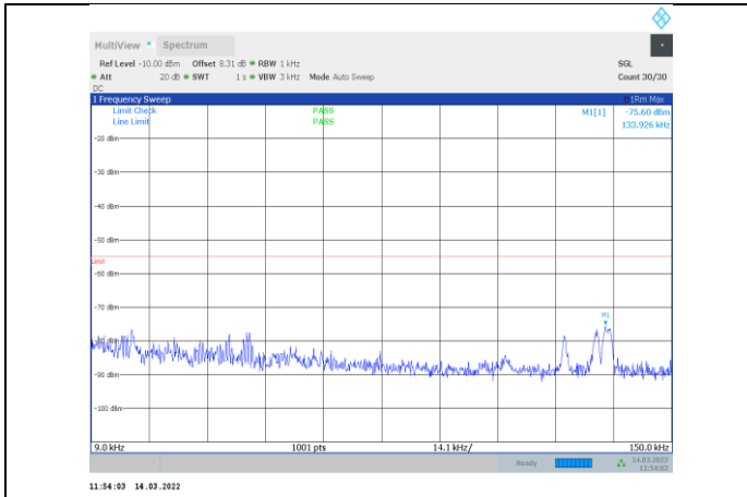
1-N41-PC3-30-60-M-2-CP-OFDM QPSK-Edge_1RB_Right-1 @161-0.009-0.15-Ant1--75.60--55-PASS
