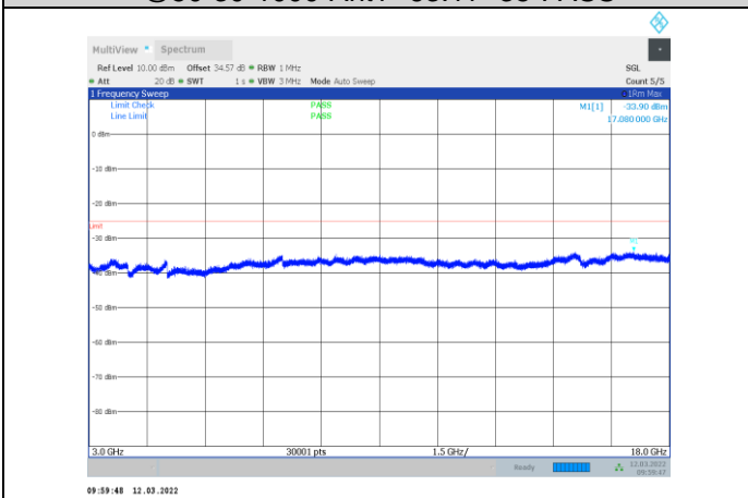
1-N41-PC3-30-20-L-2-CP-OFDM QPSK-Edge_1RB_Right-1 @50-3000-18000-Ant1--33.90--25-PASS
