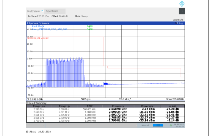
1-N41-PC3-30-100-H-28-CP-OFDM 16QAM-Inner_Full-137@68-Ant1-PASS
