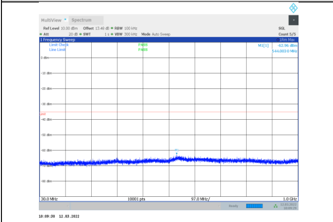
1-N41-PC3-30-20-M-3-CP-OFDM QPSK-Outter_Full-51 @0-30-1000-Ant1--62.96--35-PASS
