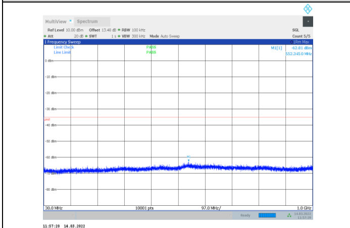
1-N41-PC3-30-60-M-3-CP-OFDM QPSK-Outer_Full-162 @0-30-1000-Ant1--62.81--35-PASS
