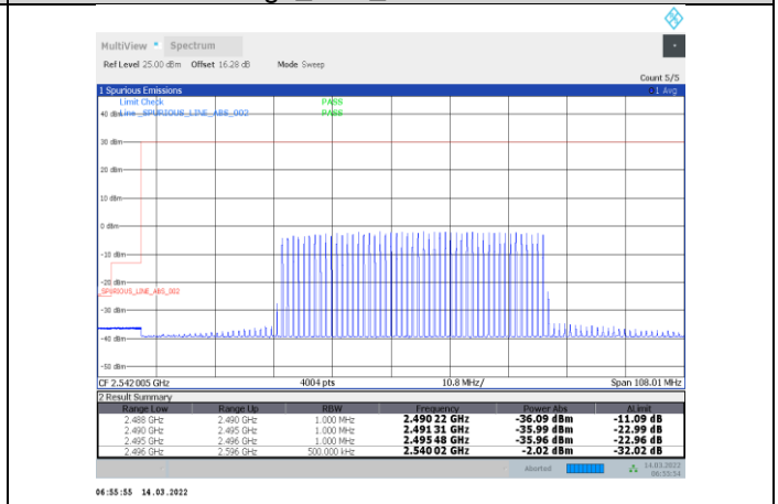
1-N41-PC3-30-100-L-32-CP-OFDM 64QAM-Inner_Full-137@68-Ant1-PASS
