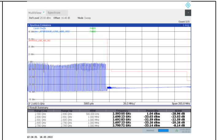
1-N41-PC3-30-100-H-7-DFT-s-OFDM QPSK-Outer_Full-270@0-Ant1-PASS
