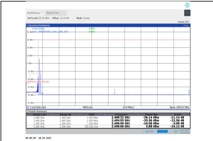
1-N41-PC3-30-100-L-9-DFT-s-OFDM 16QAM-Edge_1RB_Left-1@0-Ant1-PASS
