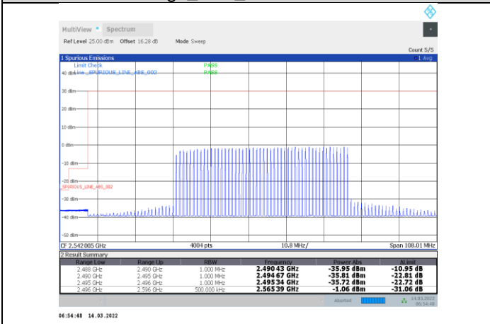
1-N41-PC3-30-100-L-28-CP-OFDM 16QAM-Inner_Full-137@68-Ant1-PASS
