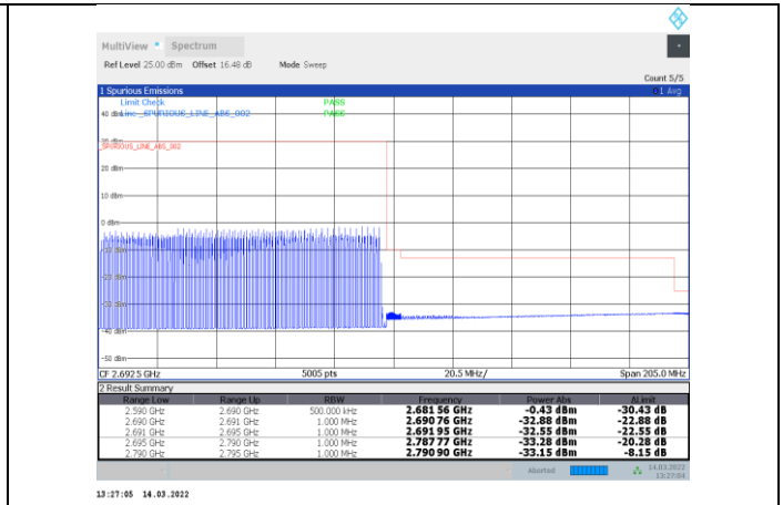
1-N41-PC3-30-100-H-15-DFT-s-OFDM 64QAM-Outer_Full-270@0-Ant1-PASS
