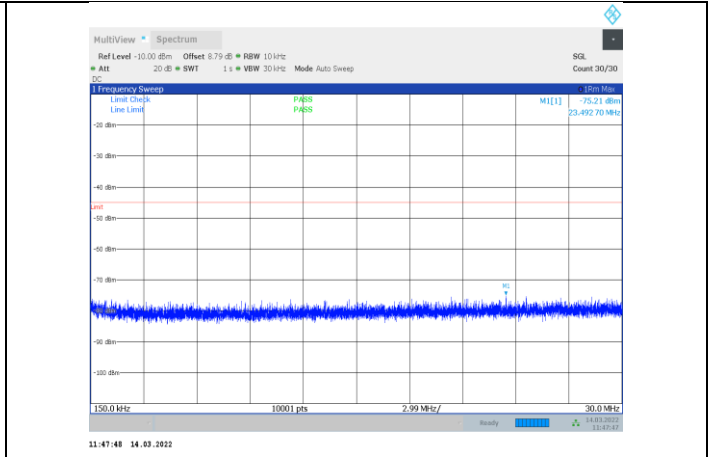
1-N41-PC3-30-60-L-3-CP-OFDM QPSK-Outer_Full-162 @0-0.15-30-Ant1--75.21--45-PASS
