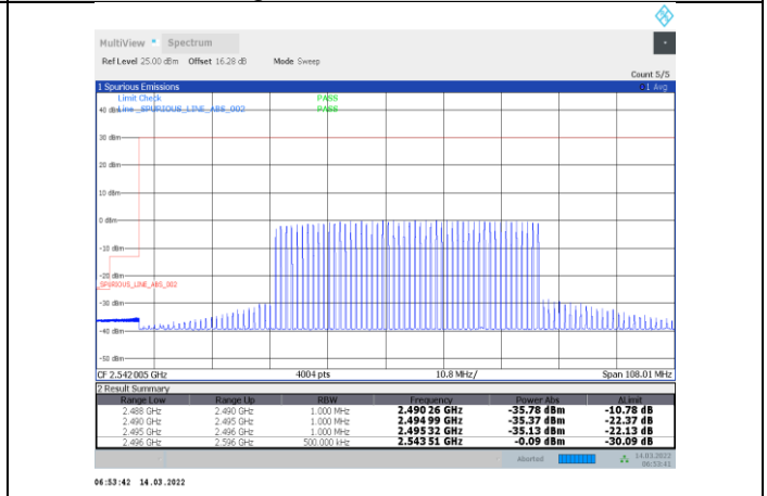
1-N41-PC3-30-100-L-24-CP-OFDM QPSK-Inner_Full-137@68-Ant1-PASS
