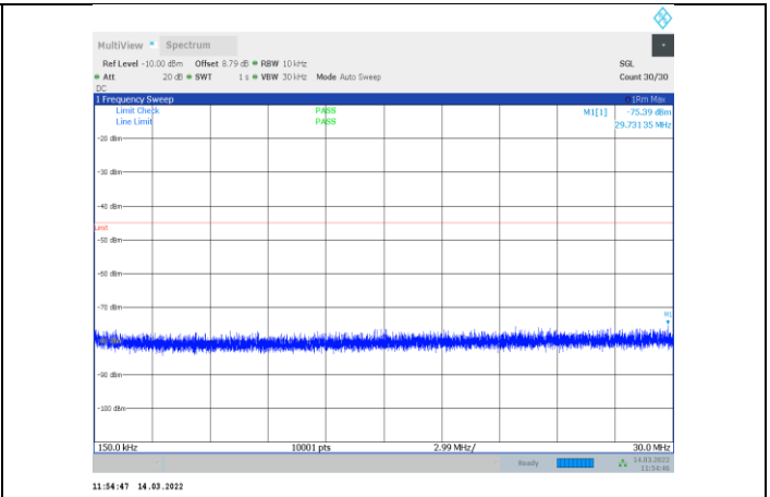
1-N41-PC3-30-60-M-2-CP-OFDM QPSK-Edge_1RB_Right-1 @161-0.15-30-Ant1--75.39--45-PASS
