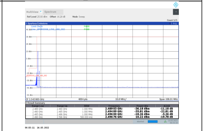
1-N41-PC3-30-100-L-29-CP-OFDM 64QAM-Edge_1RB_Left-1@0-Ant1-PASS
