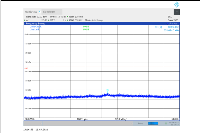
1-N41-PC3-30-20-H-2-CP-OFDM QPSK-Edge_1RB_Right-1 @50-30-1000-Ant1--63.25--35-PASS
