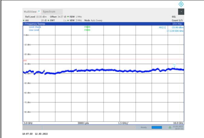
1-N41-PC3-30-20-M-2-CP-OFDM QPSK-Edge_1RB_Right-1 @50-3000-18000-Ant1--33.90--25-PASS
