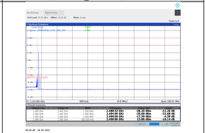
1-N41-PC3-30-100-L-13-DFT-s-OFDM 64QAM-Edge_1RB_Left-1@0-Ant1-PASS
