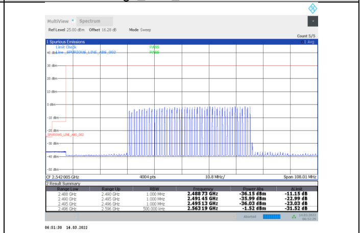
1-N41-PC3-30-100-L-16-DFT-s-OFDM 64QAM-Inner_Full-135@67-Ant1-PASS
