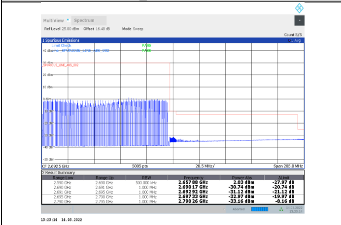
1-N41-PC3-30-100-H-3-DFT-s-OFDM PI/2 BPSK-Outer_Full-270@0-Ant1-PASS
