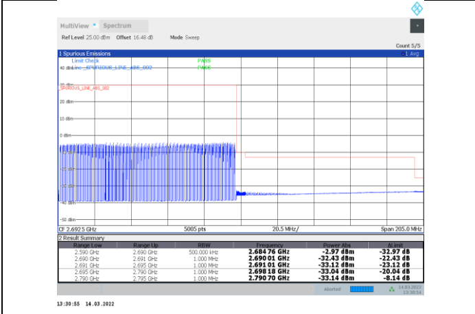
1-N41-PC3-30-100-H-27-CP-OFDM 16QAM-Outer_Full-273@0-Ant1-PASS
