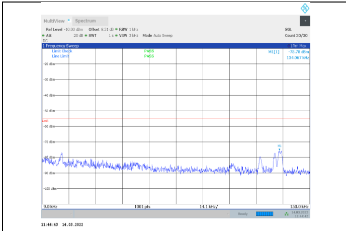
1-N41-PC3-30-60-L-2-CP-OFDM QPSK-Edge_1RB_Right-1 @161-0.009-0.15-Ant1--75.78--55-PASS
