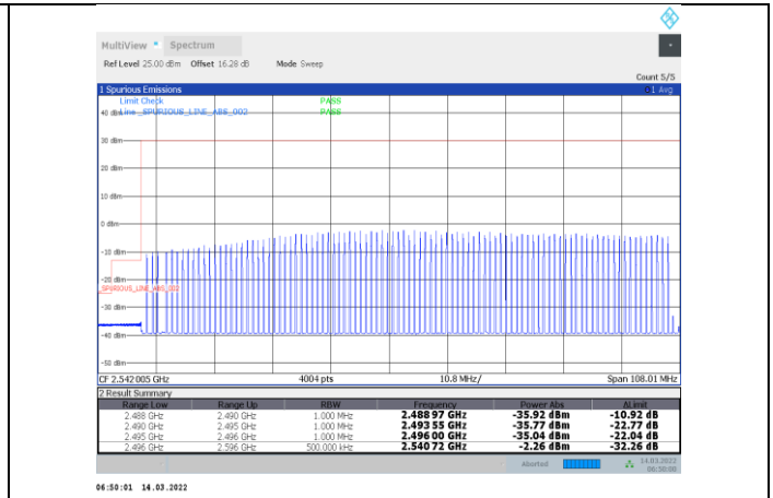
1-N41-PC3-30-100-L-11-DFT-s-OFDM 16QAM-Outer_Full-270@0-Ant1-PASS
