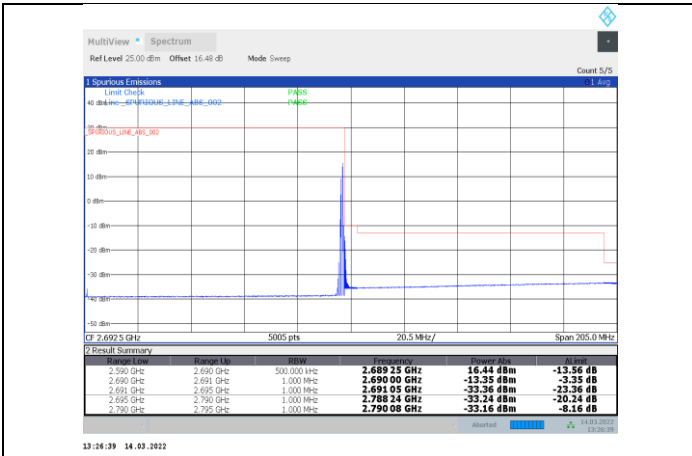
1-N41-PC3-30-100-H-14-DFT-s-OFDM 64QAM-Edge_1RB_Right-1@272-Ant1-PASS
