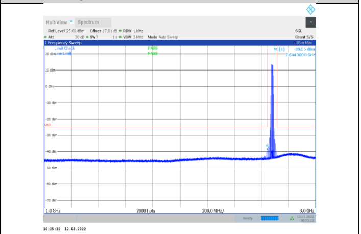
1-N41-PC3-30-20-H-3-CP-OFDM QPSK-Outter_Full-51 @0-1000-3000-Ant1--39.55--25-PASS
