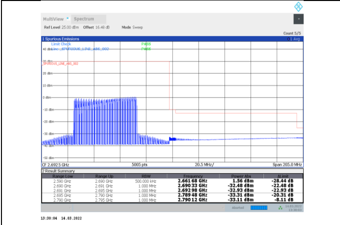
1-N41-PC3-30-100-H-24-CP-OFDM QPSK-Inner_Full-137@68-Ant1-PASS
