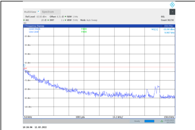
1-N41-PC3-30-20-H-3-CP-OFDM QPSK-Outter_Full-51 @0-0.009-0.15-Ant1--55.90--55-PASS
