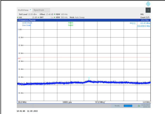
1-N41-PC3-30-20-L-3-CP-OFDM QPSK-Outter_Full-51 @0-30-1000-Ant1--63.42--35-PASS
