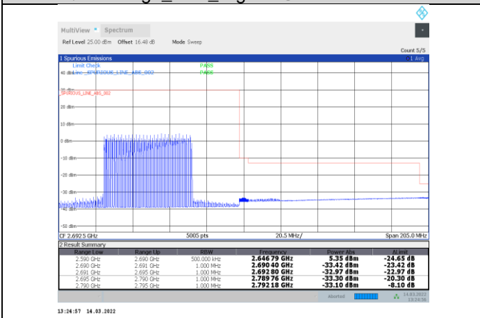
1-N41-PC3-30-100-H-8-DFT-s-OFDM QPSK-Inner_Full-135@67-Ant1-PASS
