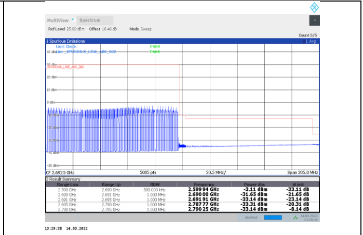
1-N41-PC3-30-100-H-23-CP-OFDM QPSK-Outer_Full-273@0-Ant1-PASS
