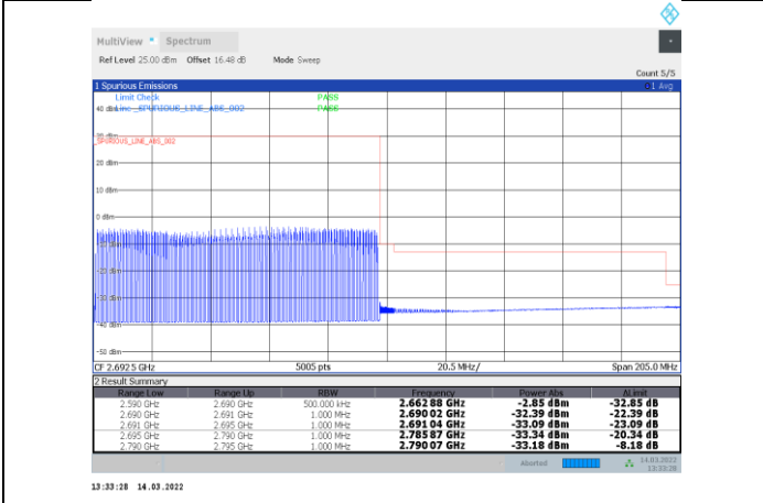
1-N41-PC3-30-100-H-32-CP-OFDM 64QAM-Inner_Full-137@68-Ant1-PASS
