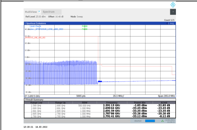
1-N41-PC3-30-100-H-19-DFT-s-OFDM 256QAM-Outer_Full-270@0-Ant1-PASS
