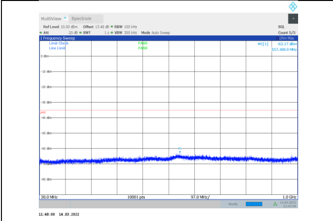
1-N41-PC3-30-60-L-3-CP-OFDM QPSK-Outer_Full-162 @0-30-1000-Ant1--63.17--35-PASS
