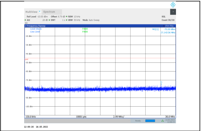
1-N41-PC3-30-60-H-1-CP-OFDM QPSK-Edge_1RB_Left-1 @0-0.15-30-Ant1--75.50--45-PASS
