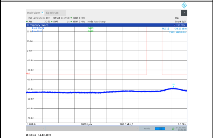
1-N41-PC3-30-60-M-1-CP-OFDM QPSK-Edge_1RB_Left-1 @0-1000-3000-Ant1--38.19--25-PASS
