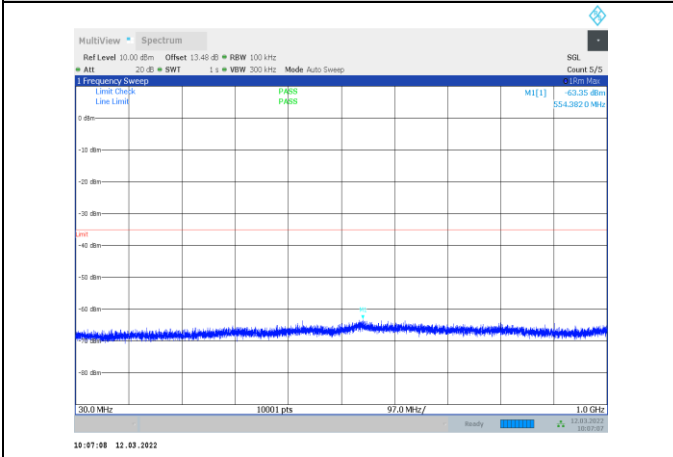
1-N41-PC3-30-20-M-2-CP-OFDM QPSK-Edge_1RB_Right-1 @50-30-1000-Ant1--63.35-- 35-PASS
