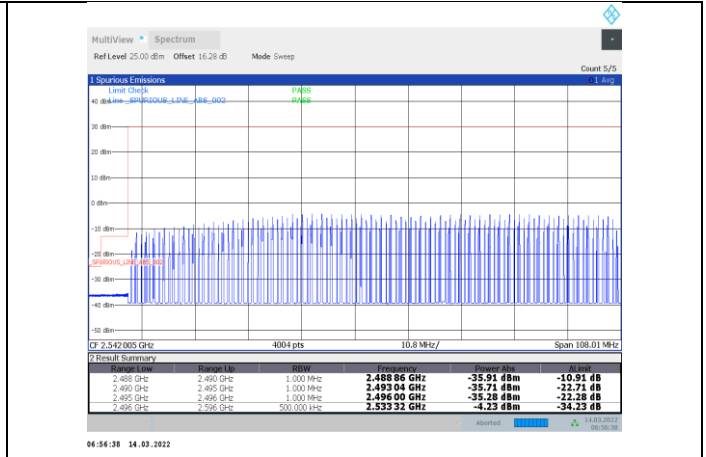
1-N41-PC3-30-100-L-35-CP-OFDM 256QAM-Outer_Full-273@0-Ant1-PASS
