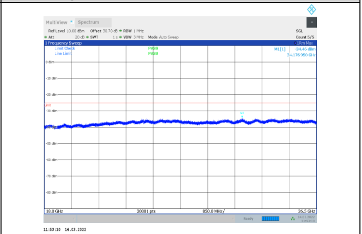
1-N41-PC3-30-60-M-1-CP-OFDM QPSK-Edge_1RB_Left-1 @0-18000-26500-Ant1--34.46--25-PASS
