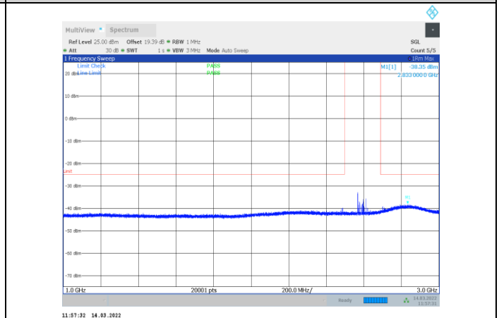
1-N41-PC3-30-60-M-3-CP-OFDM QPSK-Outer_Full-162 @0-1000-3000-Ant1--38.35--25-PASS
