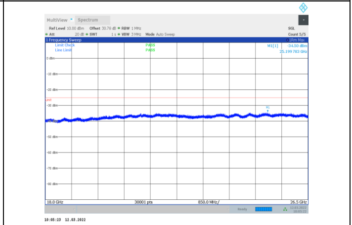
1-N41-PC3-30-20-M-1-CP-OFDM QPSK-Edge_1RB_Left-1 @0-18000-26500-Ant1--34.50--25-PASS
