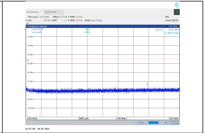
1-N41-PC3-30-60-M-3-CP-OFDM QPSK-Outer_Full-162 @0-0.15-30-Ant1--75.63--45-PASS
