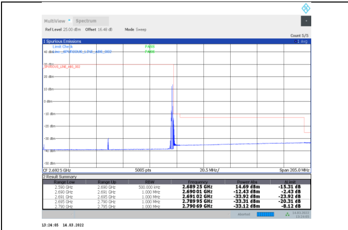
1-N41-PC3-30-100-H-6-DFT-s-OFDM QPSK-Edge_1RB_Right-1@272-Ant1-PASS
