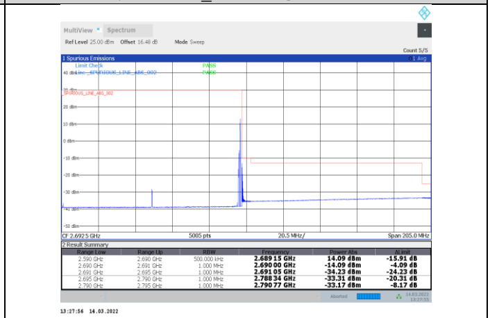
1-N41-PC3-30-100-H-18-DFT-s-OFDM 256QAM-Edge_1RB_Right-1@272-Ant1-PASS
