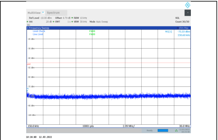
1-N41-PC3-30-20-H-3-CP-OFDM QPSK-Outter_Full-51 @0-0.15-30-Ant1--75.33--45-PASS
