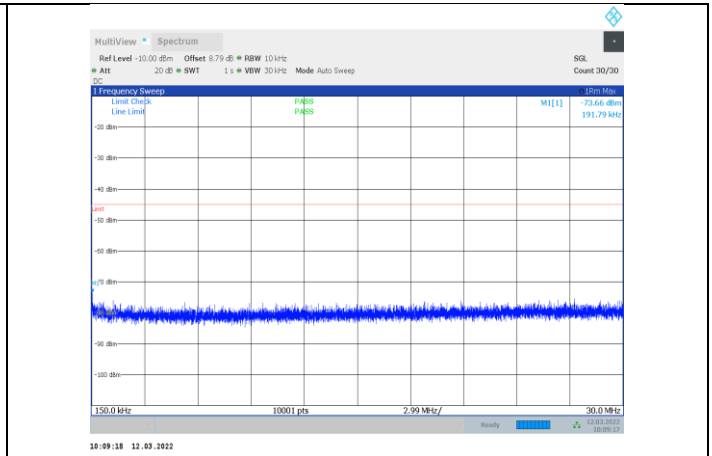
1-N41-PC3-30-20-M-3-CP-OFDM QPSK-Outter_Full-51 @0-0.15-30-Ant1--73.66--45-PASS
