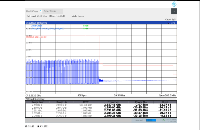
1-N41-PC3-30-100-H-31-CP-OFDM 64QAM-Outer_Full-273@0-Ant1-PASS
