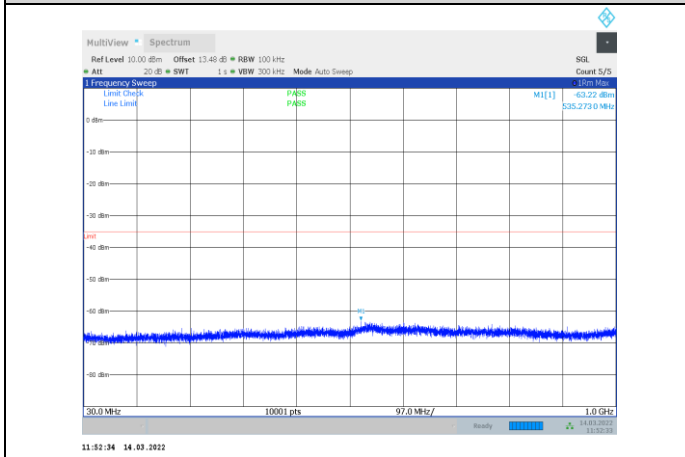
1-N41-PC3-30-60-M-1-CP-OFDM QPSK-Edge_1RB_Left-1 @0-30-1000-Ant1--63.22--35-PASS
