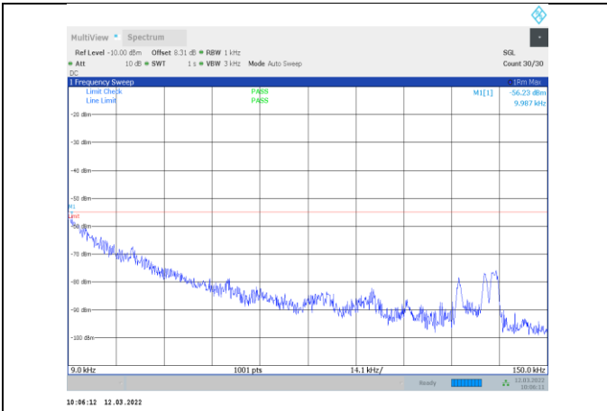
1-N41-PC3-30-20-M-2-CP-OFDM QPSK-Edge_1RB_Right-1 @50-0.009-0.15-Ant1--56.23--55-PASS
