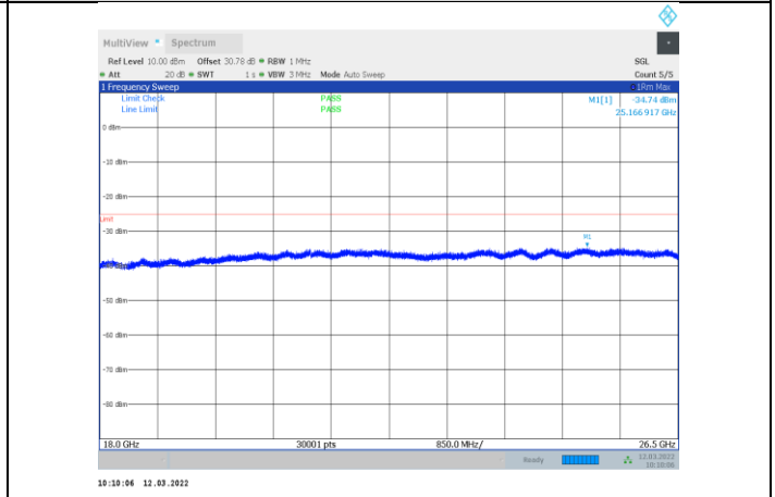
1-N41-PC3-30-20-M-3-CP-OFDM QPSK-Outter_Full-51 @0-18000-26500-Ant1--34.74--25-PASS
