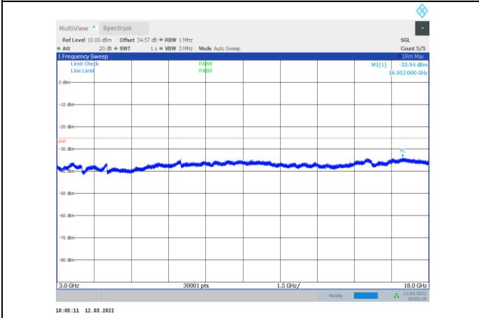
1-N41-PC3-30-20-M-1-CP-OFDM QPSK-Edge_1RB_Left-1 @0-3000-18000-Ant1--33.94--25-PASS
