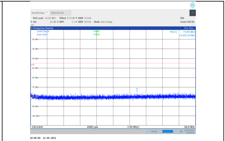
1-N41-PC3-30-20-M-2-CP-OFDM QPSK-Edge_1RB_Right-1 @50-0.15-30-Ant1--74.89--45-PASS
