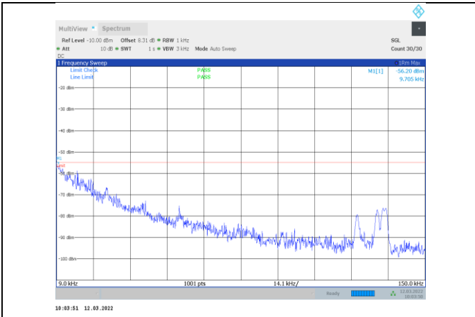
1-N41-PC3-30-20-M-1-CP-OFDM QPSK-Edge_1RB_Left-1 @0-0.009-0.15-Ant1--56.20--55-PASS
