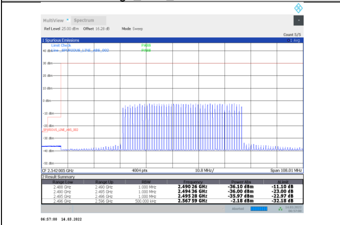
1-N41-PC3-30-100-L-36-CP-OFDM 256QAM-Inner_Full-137@68-Ant1-PASS
