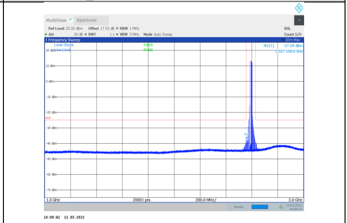
1-N41-PC3-30-20-M-3-CP-OFDM QPSK-Outter_Full-51 @0-1000-3000-Ant1--37.39--25-PASS
