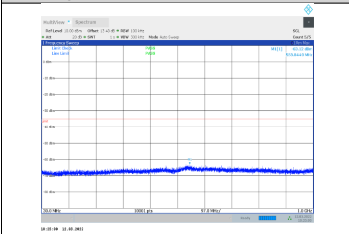
1-N41-PC3-30-20-H-3-CP-OFDM QPSK-Outter_Full-51 @0-30-1000-Ant1--63.12--35-PASS
