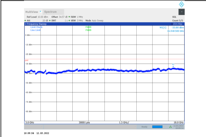
1-N41-PC3-30-20-M-3-CP-OFDM QPSK-Outter_Full-51 @0-3000-18000-Ant1--33.80--25-PASS
