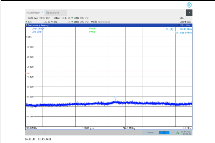
1-N41-PC3-30-20-H-1-CP-OFDM QPSK-Edge_1RB_Left-1 @0-30-1000-Ant1--63.43--35-PASS
