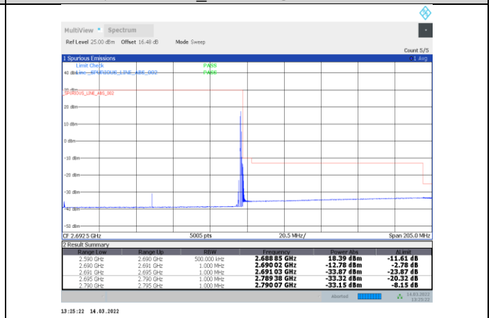
1-N41-PC3-30-100-H-10-DFT-s-OFDM 16QAM-Edge_1RB_Right-1@272-Ant1-PASS
