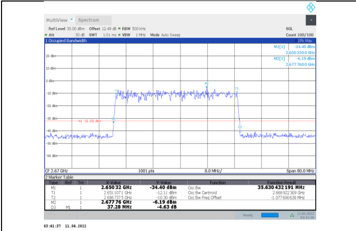
1-N41-PC3-30-40-H-7-CP-64QAM-Outer_Full-106@0-A nt1-35.63-37.280-≤40-PASS
