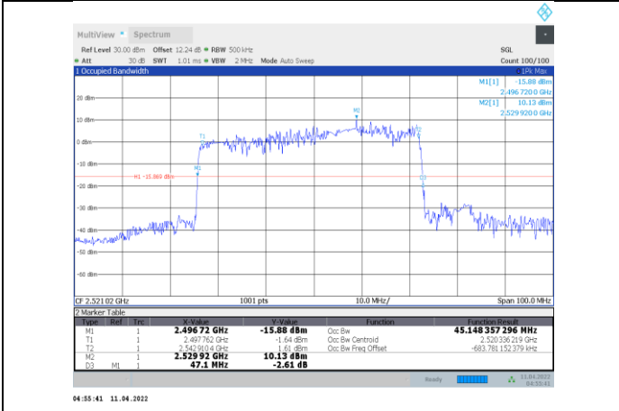
1-N41-PC3-30-50-L-8-CP-256QAM-Outer_Full-133@0- Ant1-45.148-47.100-≤50-PASS
