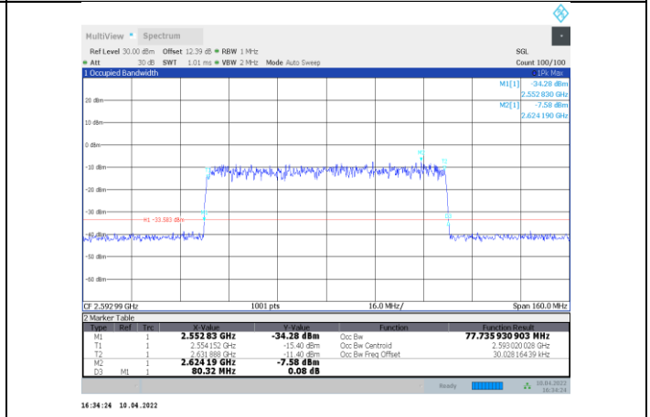
1-N41-PC3-30-80-M-4-DFT-64QAM-Outer_Full-216@0- Ant1-77.736-80.320-≤80-PASS
