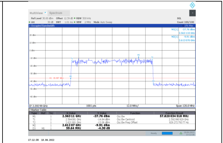
1-N41-PC3-30-60-M-5-CP-QPSK-Outer_Full-162@0-An t1-57.82-59.640-≤60-PASS
