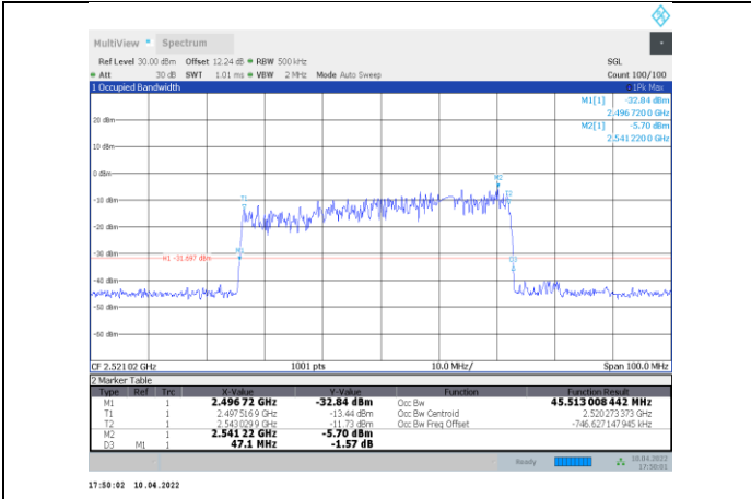
1-N41-PC3-30-50-L-6-CP-16QAM-Outer_Full-133@0-A Ant1-45.513-47.100-≤50-PASS
