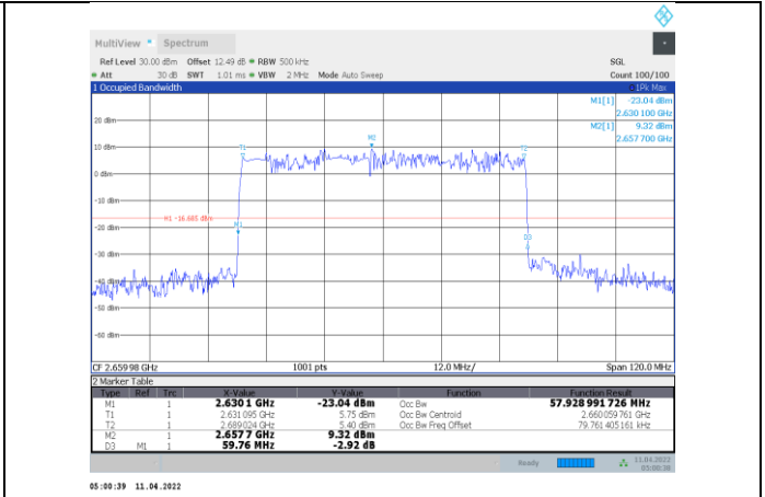
1-N41-PC3-30-60-H-8-CP-256QAM-Outer_Full-162@0- Ant1-57.929-59.760-≤60-PASS
