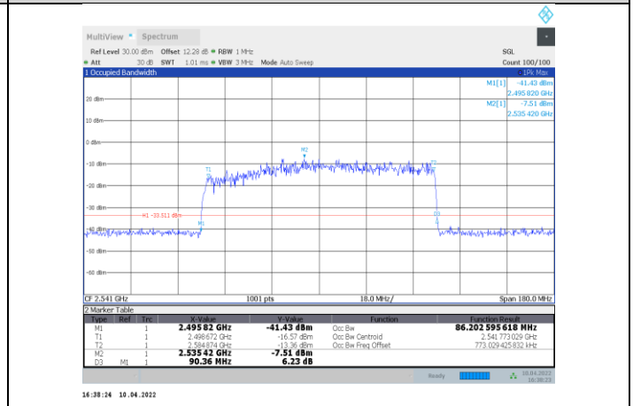
1-N41-PC3-30-90-L-4-DFT-64QAM-Outer_Full-240@0-A nt1-86.203-90.360-≤90-PASS
