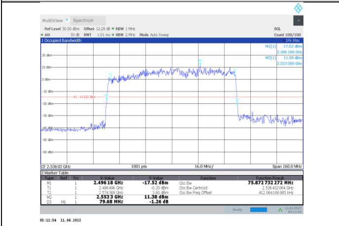
1-N41-PC3-30-80-L-8-CP-256QAM-Outer_Full-217@0- Ant1-75.873-79.680-≤80-PASS
