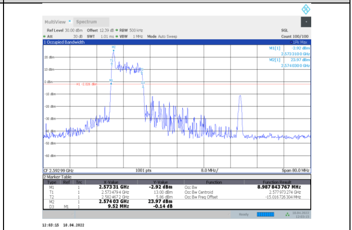
1-N41-PC3-30-40-M-1-DFT-QPSK-Outer_Full-100@0-A Ant1-8.988-9.520-≤40-PASS
