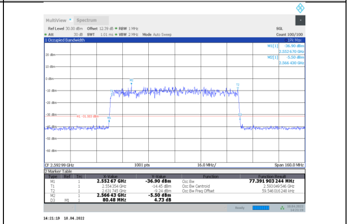
1-N41-PC3-30-80-M-2-DFT-PI2BPSK-Outer_Full-217@0- Ant1-77.392-80.480-≤80-PASS
