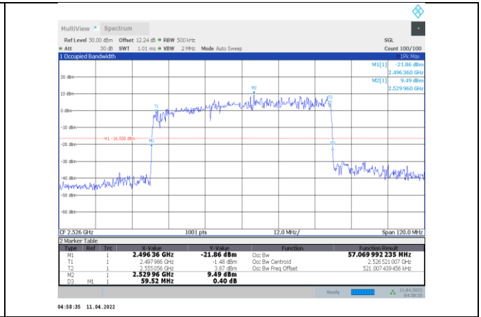
1-N41-PC3-30-60-L-8-CP-256QAM-Outer_Full-162@0-A Ant1-57.07-59.520-≤60-PASS
