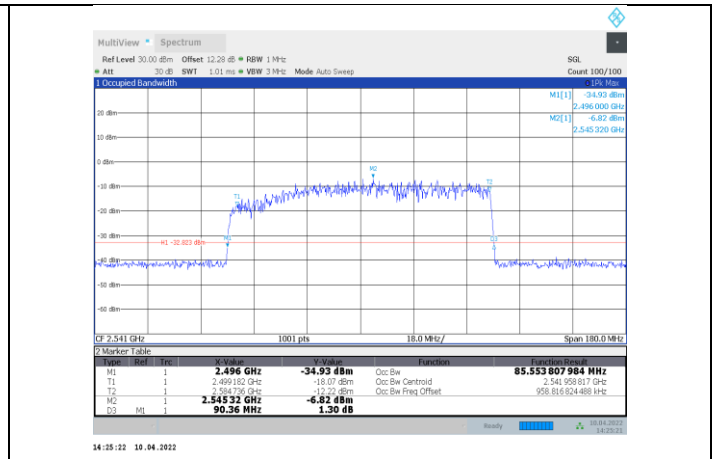
1-N41-PC3-30-90-L-2-DFT-PI2BPSK-Outer_Full-245@0 -Ant1-85.554-90.360-≤90-PASS
