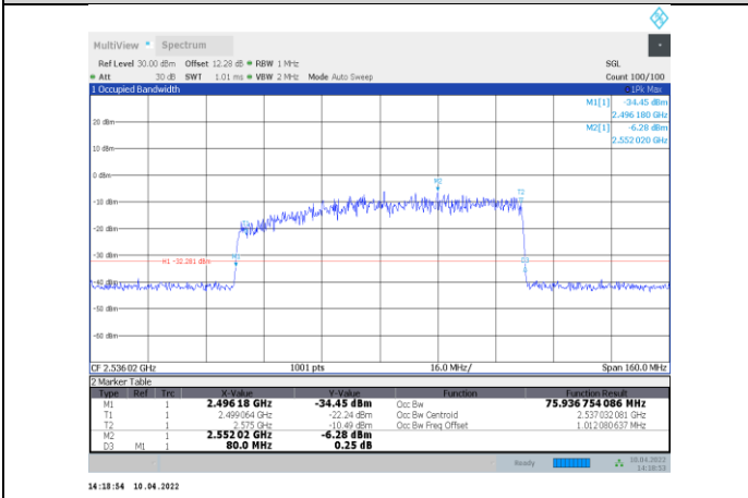
1-N41-PC3-30-80-L-2-DFT-PI2BPSK-Outer_Full-217@0-A Ant1-75.937-80.000-≤80-PASS
