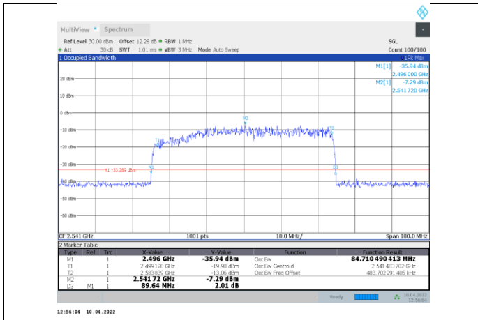
1-N41-PC3-30-90-L-1-DFT-QPSK-Outer_Full-240@0-A nt1-84.71-89.640-≤90-PASS
