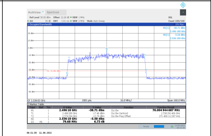
1-N41-PC3-30-80-L-7-CP-64QAM-Outer_Full-217@0-A nt1-76.005-79.680-≤80-PASS
