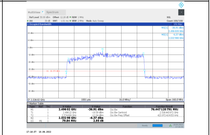
1-N41-PC3-30-80-L-5-CP-QPSK-Outer_Full-217@0-Ant 1-76.447-79.840-≤80-PASS
