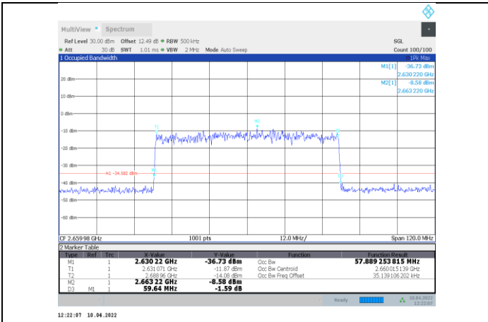
1-N41-PC3-30-60-H-1-DFT-QPSK-Outer_Full-162@0-A nt1-57.889-59.640-≤60-PASS
