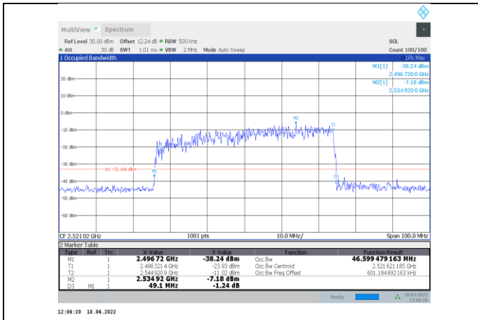
1-N41-PC3-30-50-L-1-DFT-QPSK-Outer_Full-128@0-A nt1-46.599-49.100-≤50-PASS
