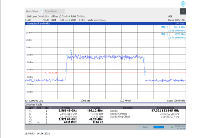
1-N41-PC3-30-50-M-1-DFT-QPSK-Outer_Full-128@0- Ant1-47.321-49.000-≤50-PASS
