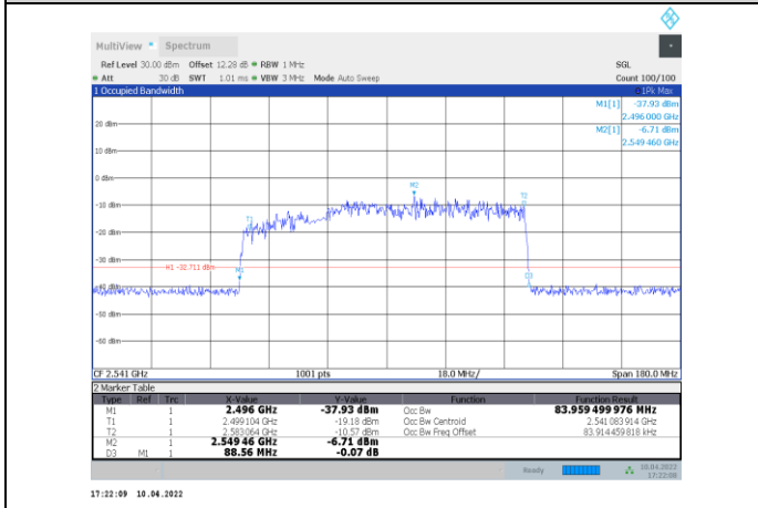
1-N41-PC3-30-90-L-5-CP-QPSK-Outer_Full-245@0-An t1-83.959-88.560-≤90-PASS
