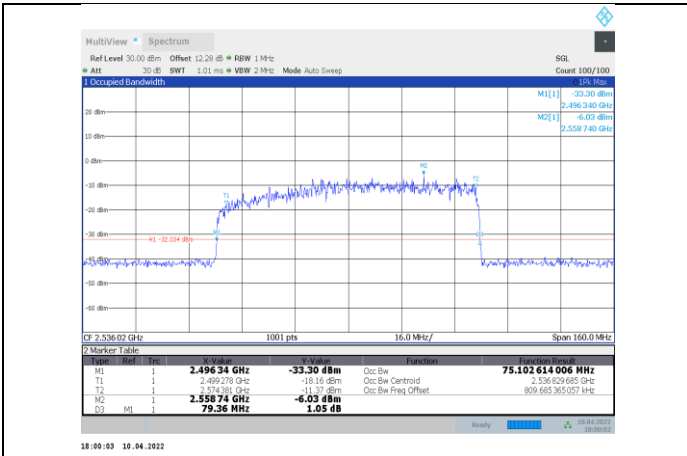
1-N41-PC3-30-80-L-6-CP-16QAM-Outer_Full-217@0-A Ant1-75.103-79.360-≤80-PASS
