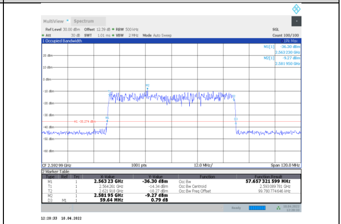
1-N41-PC3-30-60-M-1-DFT-QPSK-Outer_Full-162@0-A Ant1-57.657-59.640-≤60-PASS
