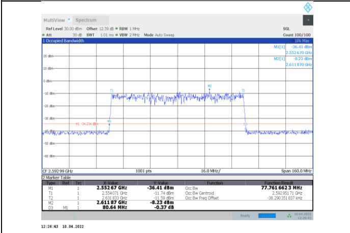
1-N41-PC3-30-80-M-1-DFT-QPSK-Outer_Full-216@0- Ant1-77.762-80.640-≤80-PASS
