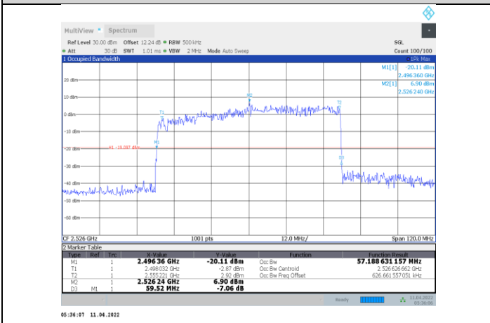
1-N41-PC3-30-60-L-9-DFT-256QAM-Outer_Full-162@0-A Ant1-57.189-59.520-≤60-PASS
