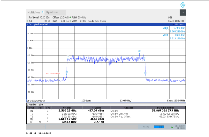
1-N41-PC3-30-60-M-2-DFT-PI2BPSK-Outer_Full-162@0-A Ant1-57.867-59.520-≤60-PASS
