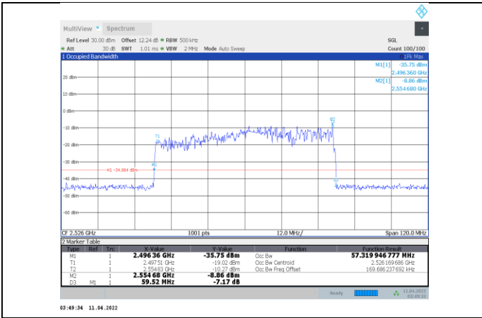
1-N41-PC3-30-60-L-7-CP-64QAM-Outer_Full-162@0-A nt1-57.32-59.520-≤60-PASS
