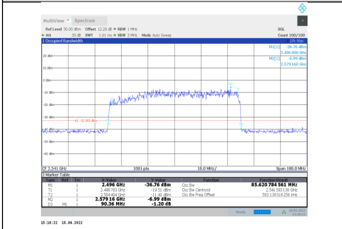
1-N41-PC3-30-90-L-3-DFT-16QAM-Outer_Full-240@0-A Ant1-85.621-90.360-≤90-PASS
