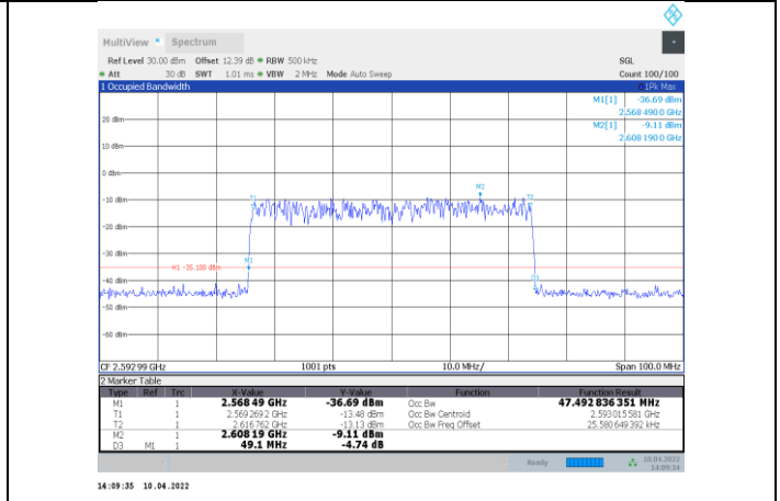
1-N41-PC3-30-50-M-2-DFT-PI2BPSK-Outer_Full-133@0- Ant1-47.493-49.100-≤50-PASS
