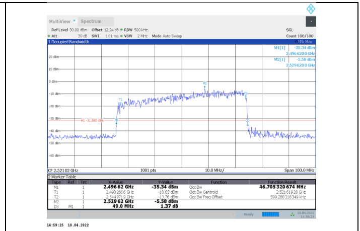
1-N41-PC3-30-50-L-3-DFT-16QAM-Outer_Full-128@0-A Ant1-46.705-49.000-≤50-PASS
