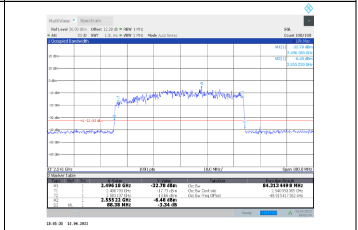
1-N41-PC3-30-90-L-6-CP-16QAM-Outer_Full-245@0-A nt1-84.313-88.380-≤90-PASS
