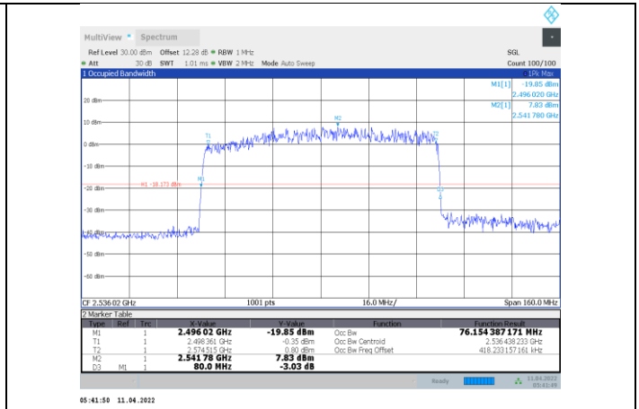
1-N41-PC3-30-80-L-9-DFT-256QAM-Outer_Full-216@0- Ant1-76.154-80.000-≤80-PASS
