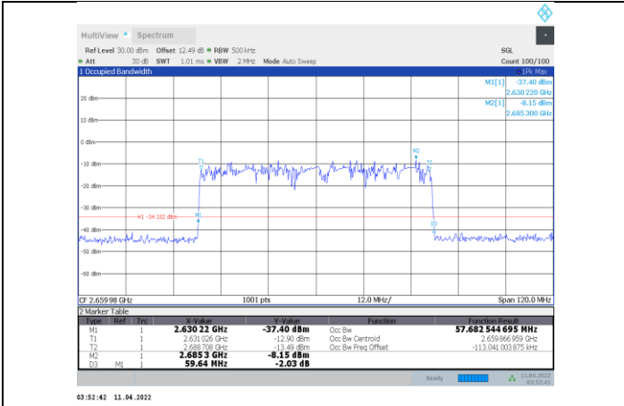
1-N41-PC3-30-60-H-7-CP-64QAM-Outer_Full-162@0-A nt1-57.683-59.640-≤60-PASS
