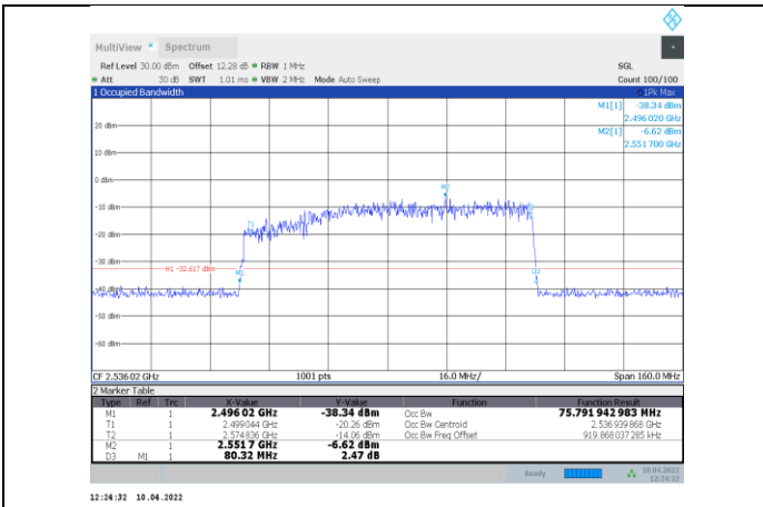
1-N41-PC3-30-80-L-1-DFT-QPSK-Outer_Full-216@0-A nt1-75.792-80.320-≤80-PASS
