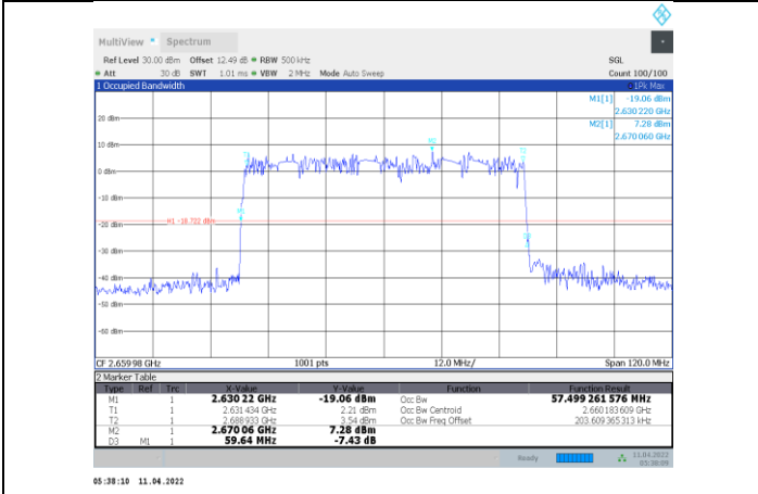
1-N41-PC3-30-60-H-9-DFT-256QAM-Outer_Full-162@0 -Ant1-57.499-59.640-≤60-PASS
