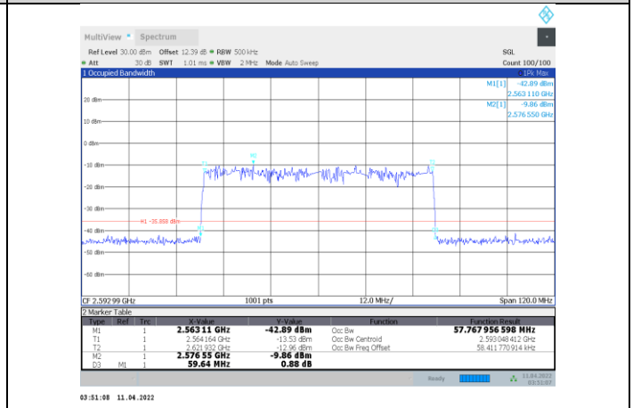
1-N41-PC3-30-60-M-7-CP-64QAM-Outer_Full-162@0-A nt1-57.768-59.640-≤60-PASS
