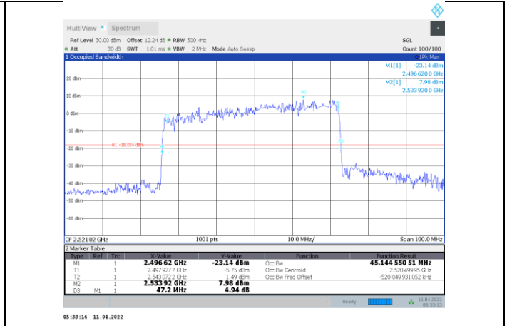
1-N41-PC3-30-50-L-9-DFT-256QAM-Outer_Full-128@0- Ant1-45.145-47.200-≤50-PASS
