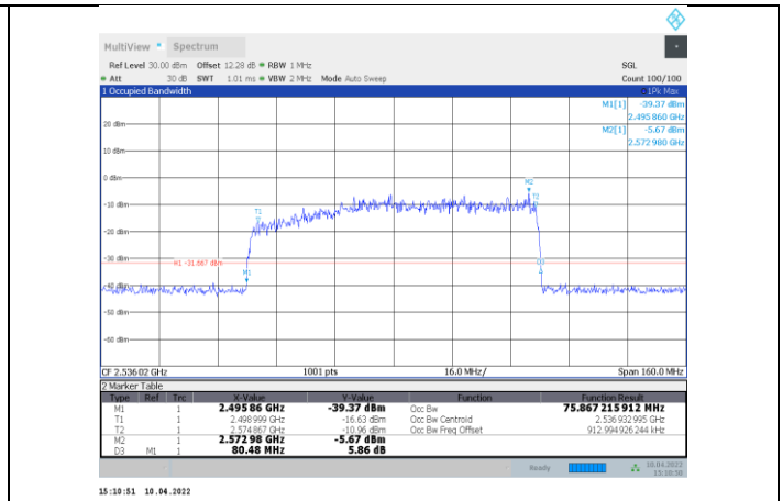
1-N41-PC3-30-80-L-3-DFT-16QAM-Outer_Full-216@0-A Ant1-75.867-80.480-≤80-PASS
