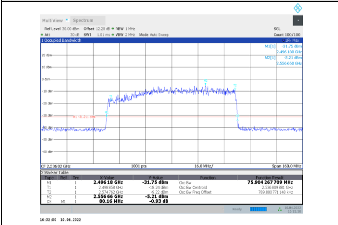
1-N41-PC3-30-80-L-4-DFT-64QAM-Outer_Full-216@0-A Ant1-75.904-80.160-≤80-PASS
