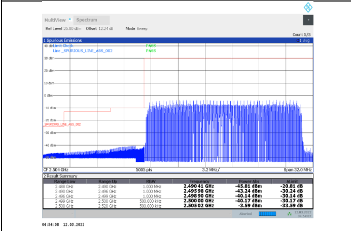
1-N7-PC3-15-20-L-15-DFT-s-OFDM 64QAM-Outer_Full-100@0-Ant1-PASS
