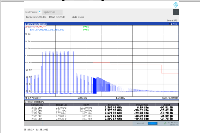
1-N7-PC3-15-20-H-32-CP-OFDM 64QAM-Inner_Full-53@26-Ant1-PASS
