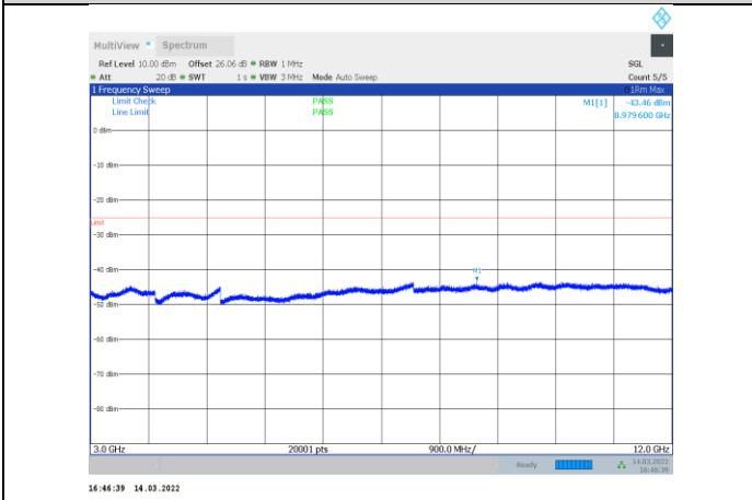
1-N7-PC3-15-15-M-2-CP-QPSK-Edge_1RB_Right-1@7 8-3000-12000-Ant1--43.46--25-PASS
