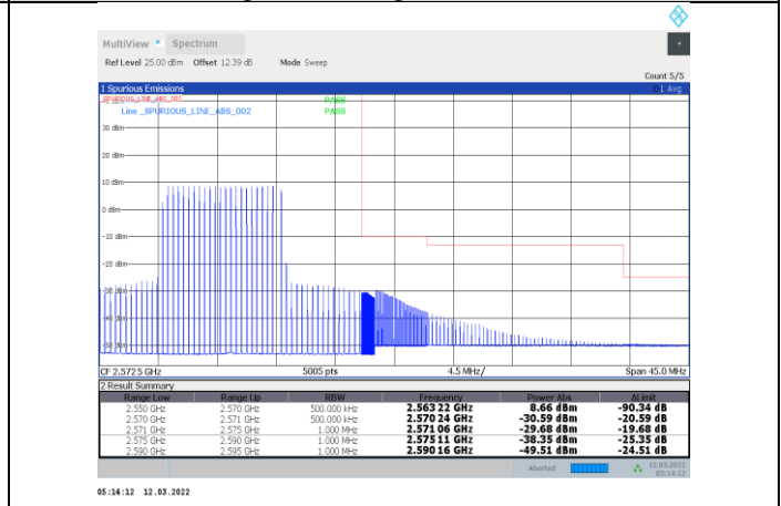
1-N7-PC3-15-20-H-12-DFT-s-OFDM 16QAM-Inner_Full-50@25-Ant1-PASS
