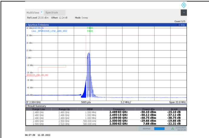
1-N7-PC3-15-20-L-25-CP-OFDM 16QAM-Edge_1RB_Left-1@0-Ant1-PASS
