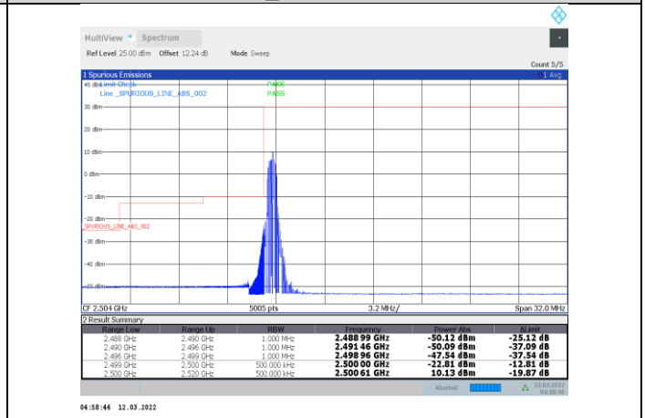
1-N7-PC3-15-20-L-29-CP-OFDM 64QAM-Edge_1RB_Left-1@0-Ant1-PASS
