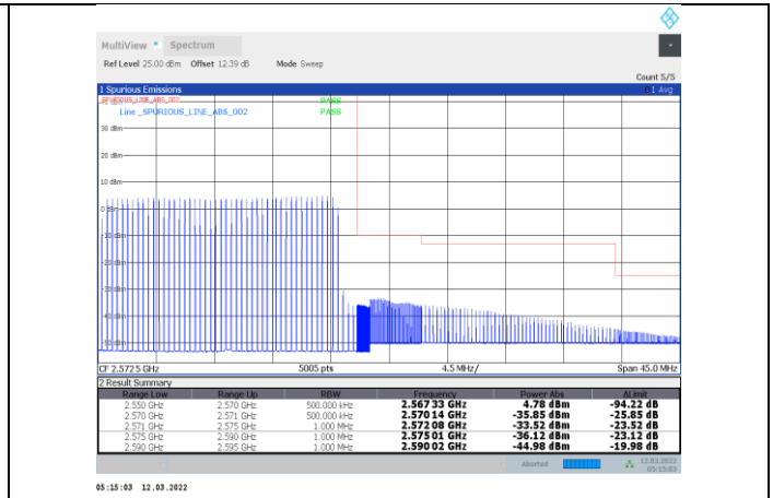
1-N7-PC3-15-20-H-15-DFT-s-OFDM 64QAM-Outer_Full-100@0-Ant1-PASS
