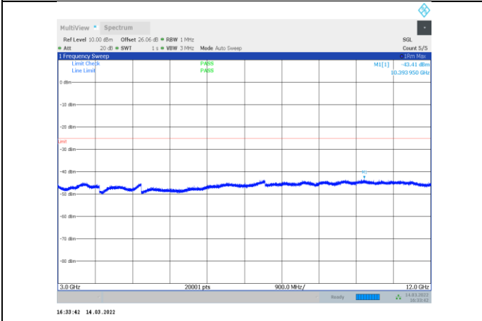
1-N7-PC3-15-5-M-3-CP-QPSK-Outer_Full-25@0-3000- 12000-Ant1--43.41--25-PASS
