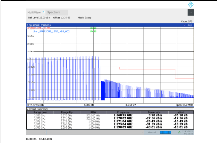
1-N7-PC3-15-20-H-27-CP-OFDM 16QAM-Outer_Full-106@0-Ant1-PASS
