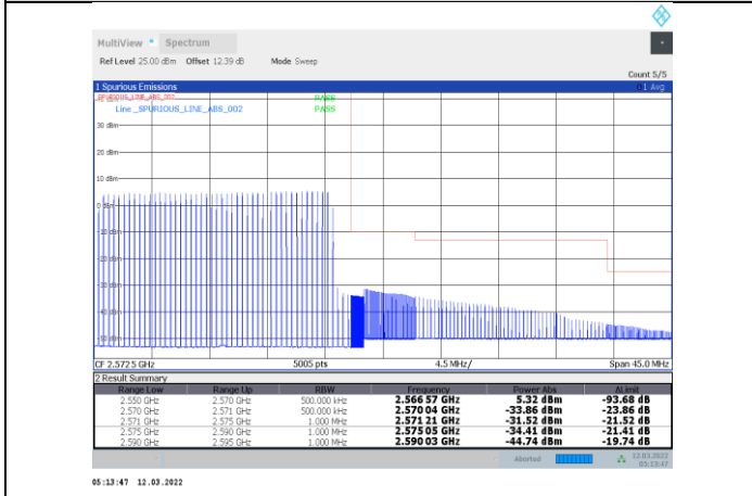
1-N7-PC3-15-20-H-11-DFT-s-OFDM 16QAM-Outer_Full-100@0-Ant1-PASS
