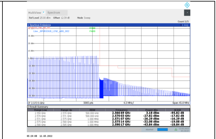
1-N7-PC3-15-20-H-31-CP-OFDM 64QAM-Outer_Full-106@0-Ant1-PASS
