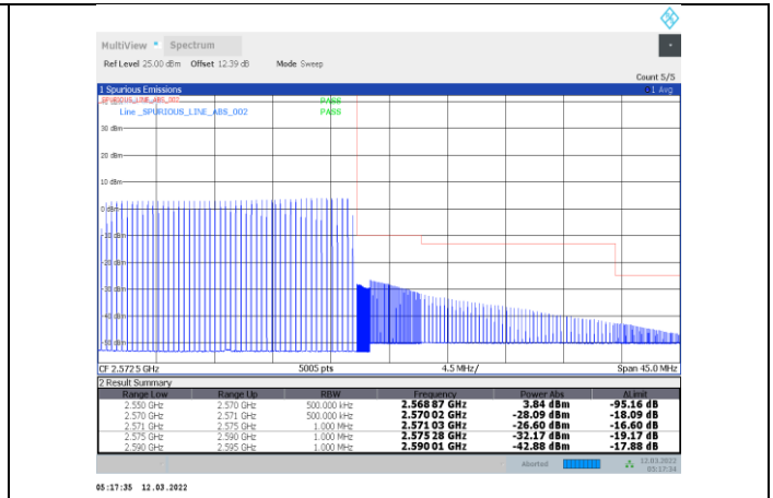
1-N7-PC3-15-20-H-23-CP-OFDM QPSK-Outer_Full-106@0-Ant1-PASS
