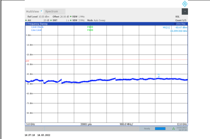
1-N7-PC3-15-5-H-2-CP-QPSK-Edge_1RB_Right-1@24 -3000-12000-Ant1--43.47--25-PASS
