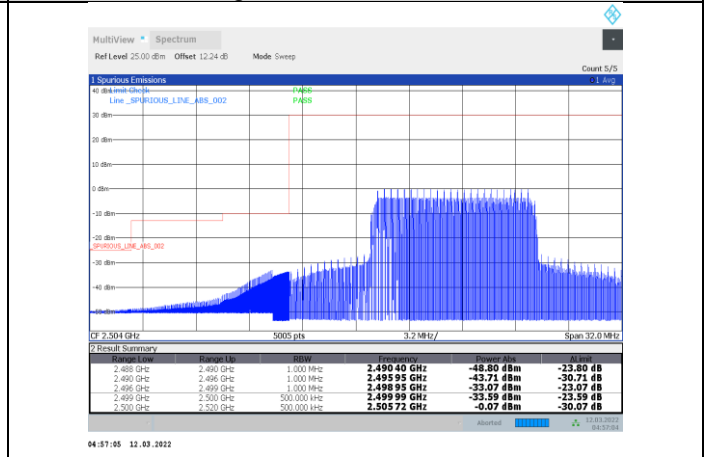
1-N7-PC3-15-20-L-24-CP-OFDM QPSK-Inner_Full-53@26-Ant1-PASS
