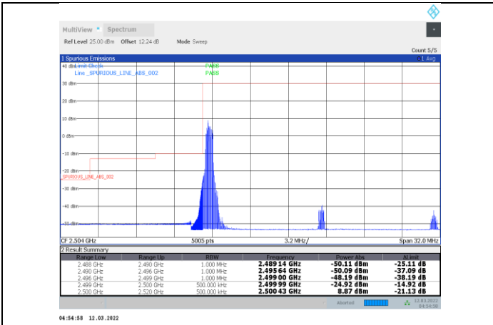
1-N7-PC3-15-20-L-17-DFT-s-OFDM 256QAM-Edge_1RB_Left-1@0-Ant1-PASS
