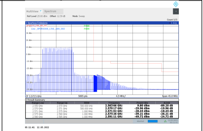
1-N7-PC3-15-20-H-4-DFT-s-OFDM PI/2 BPSK-Inner_Full-50@25-Ant1-PASS
