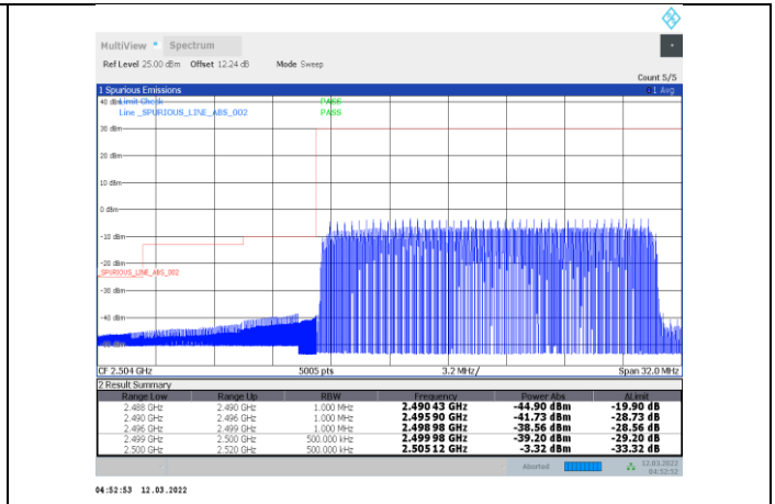
1-N7-PC3-15-20-L-11-DFT-s-OFDM 16QAM-Outer_Full-100@0-Ant1-PASS
