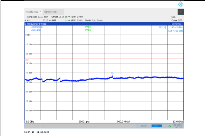
1-N7-PC3-15-5-L-2-CP-QPSK-Edge_1RB_Right-1@24 -3000-12000-Ant1--43.47--25-PASS
