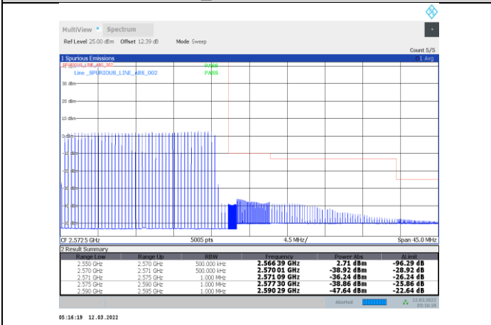
1-N7-PC3-15-20-H-19-DFT-s-OFDM 256QAM-Outer_Full-100@0-Ant1-PASS
