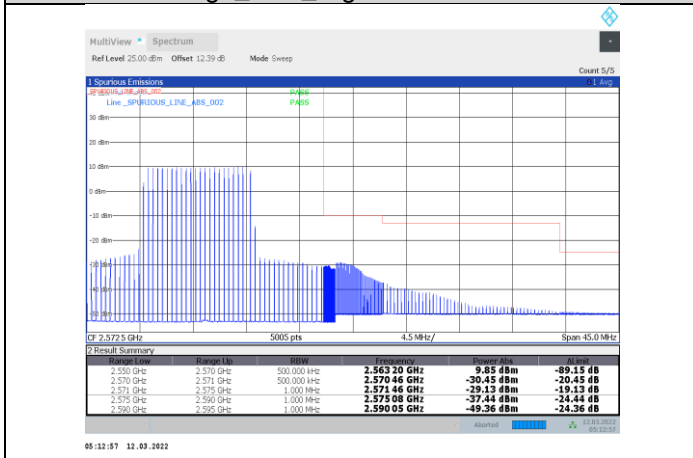
1-N7-PC3-15-20-H-8-DFT-s-OFDM QPSK-Inner_Full-50@25-Ant1-PASS
