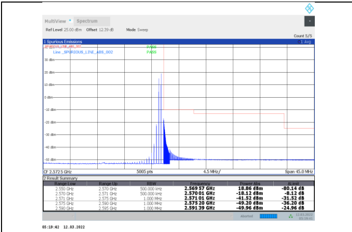
1-N7-PC3-15-20-H-30-CP-OFDM 64QAM-Edge_1RB_Right-1@105-Ant1-PASS
