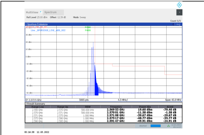
1-N7-PC3-15-20-H-14-DFT-s-OFDM 64QAM-Edge_1RB_Right-1@105-Ant1-PASS
