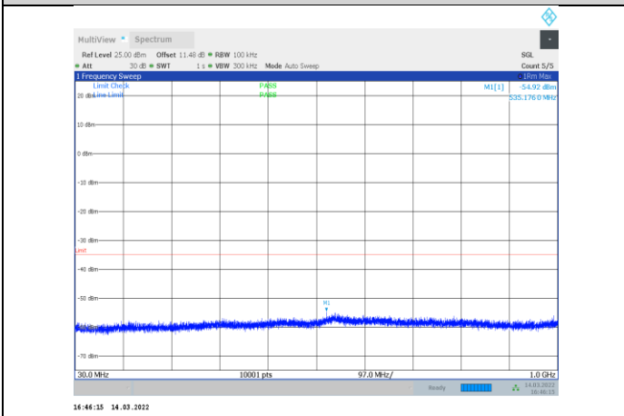
1-N7-PC3-15-15-M-2-CP-QPSK-Edge_1RB_Right-1@7 8-30-1000-Ant1--54.92--35-PASS
