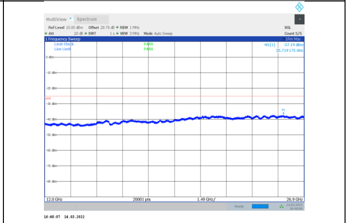
1-N7-PC3-15-15-M-3-CP-QPSK-Outter_Full-79@0-1200 0-26900-Ant1--37.19--25-PASS
