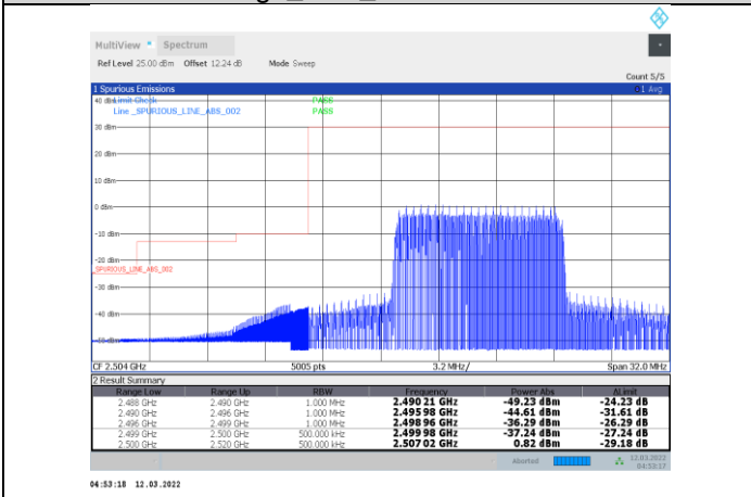
1-N7-PC3-15-20-L-12-DFT-s-OFDM 16QAM-Inner_Full-50@25-Ant1-PASS
