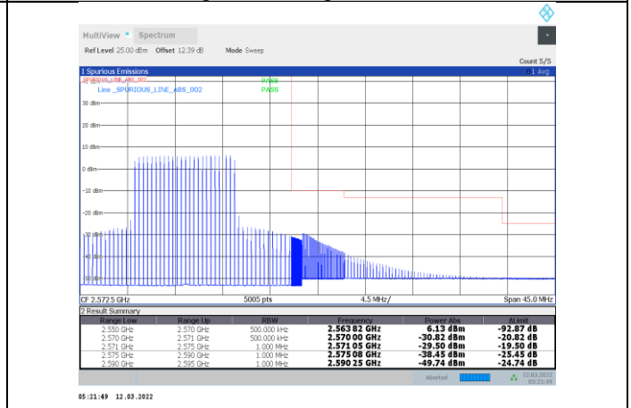
1-N7-PC3-15-20-H-36-CP-OFDM 256QAM-Inner_Full-53@26-Ant1-PASS
