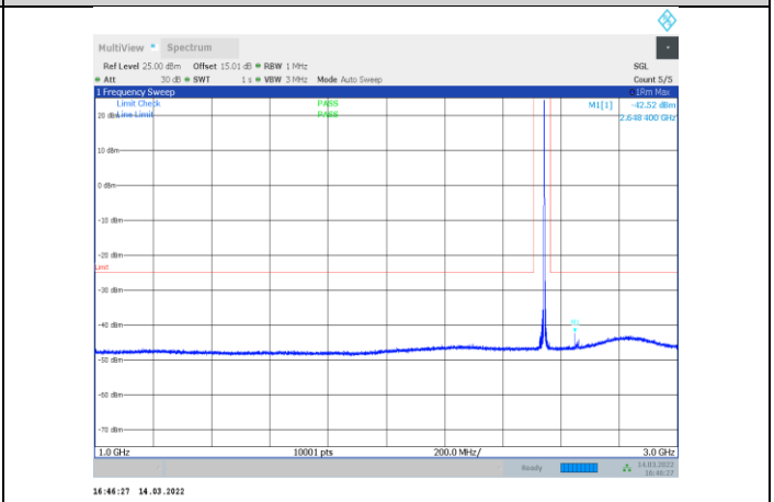
1-N7-PC3-15-15-M-2-CP-QPSK-Edge_1RB_Right-1@7 8-1000-3000-Ant1--42.52--25-PASS
