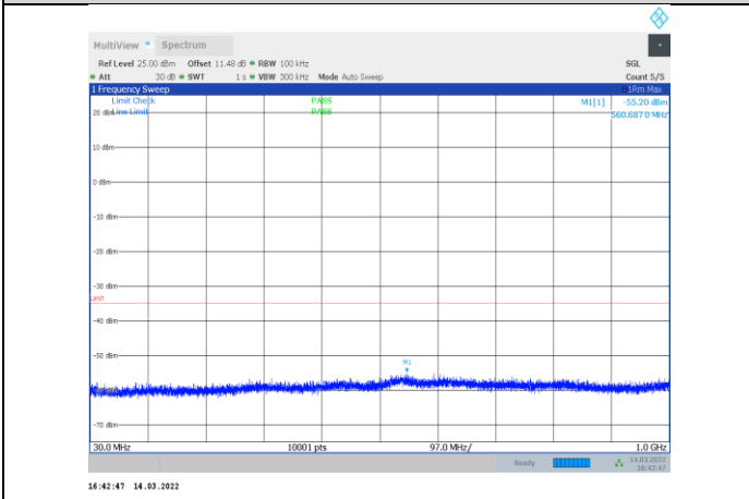
1-N7-PC3-15-15-L-3-CP-QPSK-Outter_Full-79@0-30-1 000-Ant1--55.20--35-PASS
