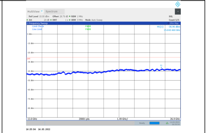
1-N7-PC3-15-5-M-3-CP-QPSK-Outer_Full-25@0-12000- 26900-Ant1--36.96--25-PASS
