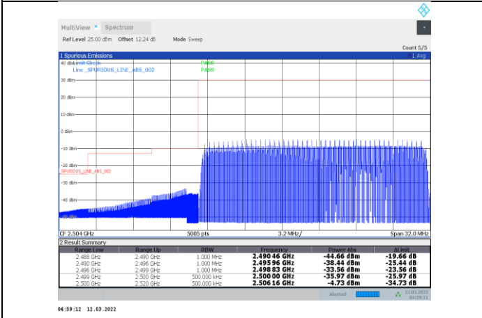
1-N7-PC3-15-20-L-31-CP-OFDM 64QAM-Outer_Full-106@0-Ant1-PASS
