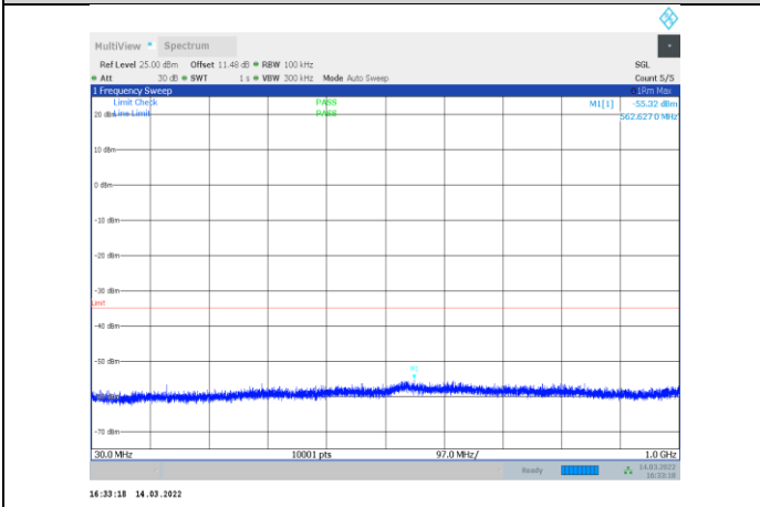
1-N7-PC3-15-5-M-3-CP-QPSK-Outer_Full-25@0-30-10 00-Ant1--55.32--35-PASS
