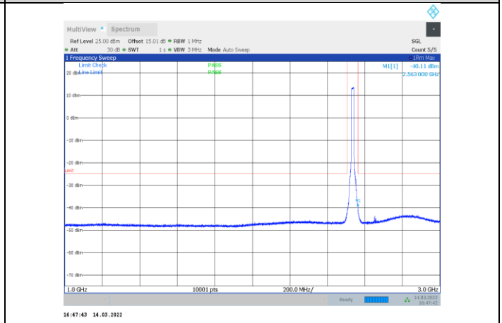
1-N7-PC3-15-15-M-3-CP-QPSK-Outter_Full-79@0-1000- 3000-Ant1--40.11--25-PASS
