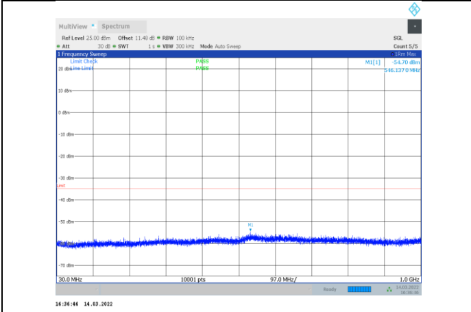
1-N7-PC3-15-5-H-2-CP-QPSK-Edge_1RB_Right-1@24 -30-1000-Ant1--54.70--35-PASS
