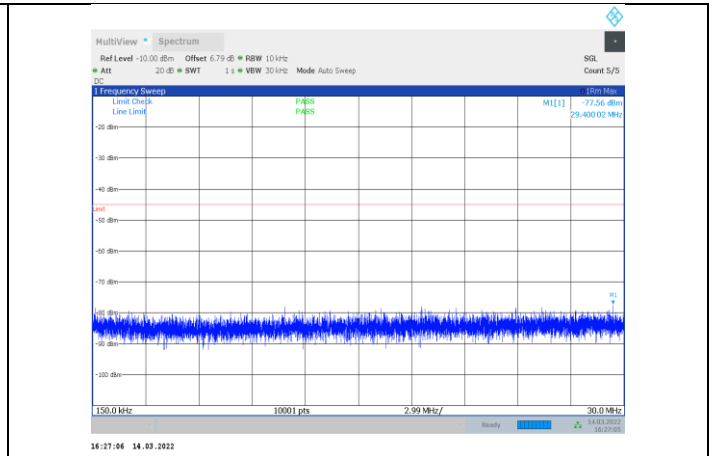
1-N7-PC3-15-5-L-2-CP-QPSK-Edge_1RB_Right-1@24 -0.15-30-Ant1--77.56--45-PASS
