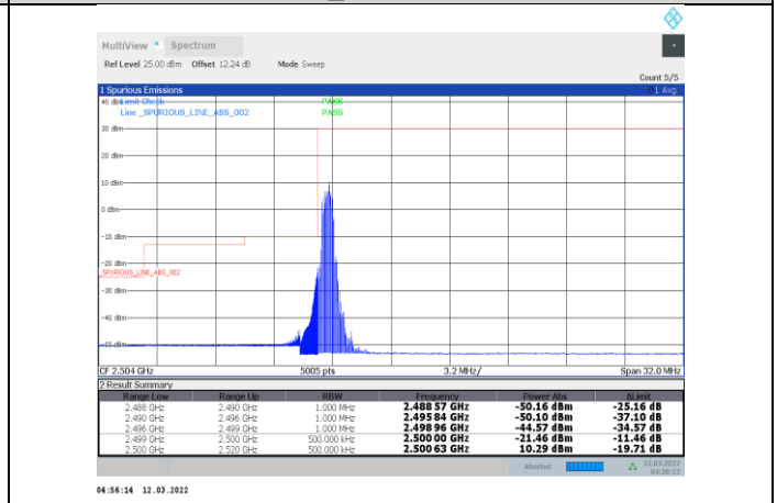
1-N7-PC3-15-20-L-21-CP-OFDM QPSK-Edge_1RB_Left-1@0-Ant1-PASS
