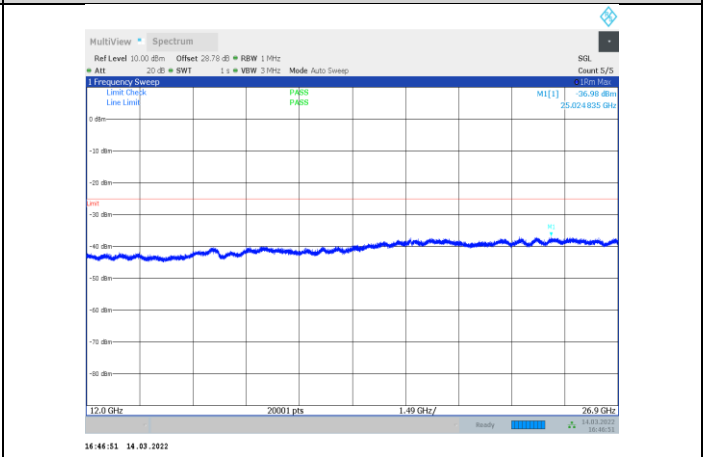
1-N7-PC3-15-15-M-2-CP-QPSK-Edge_1RB_Right-1@7 8-12000-26900-Ant1--36.98--25-PASS
