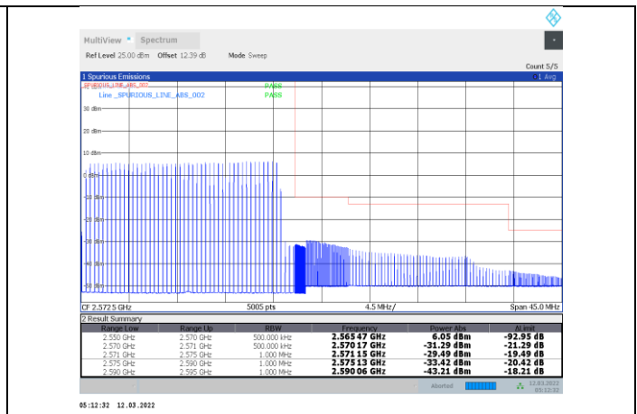
1-N7-PC3-15-20-H-7-DFT-s-OFDM QPSK-Outer_Full-100@0-Ant1-PASS
