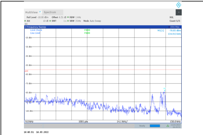
1-N7-PC3-15-15-M-2-CP-QPSK-Edge_1RB_Right-1@7 8-0.009-0.15-Ant1--78.85--55-PASS
