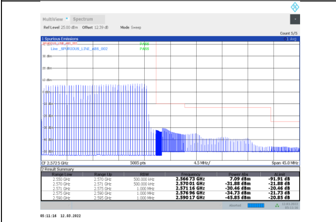
1-N7-PC3-15-20-H-3-DFT-s-OFDM PI/2 BPSK-Outer_Full-100@0-Ant1-PASS
