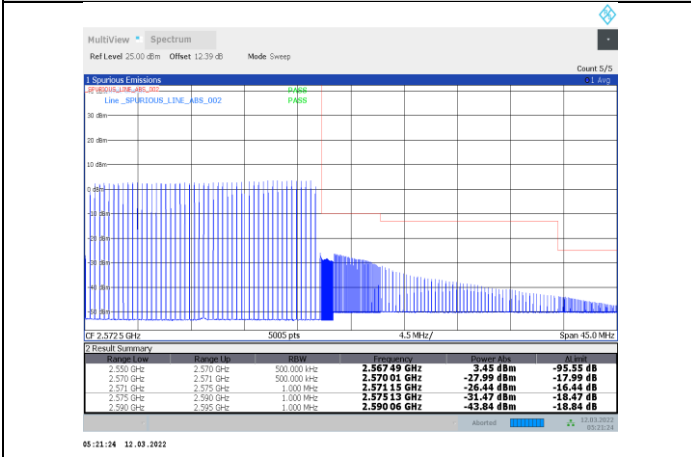
1-N7-PC3-15-20-H-35-CP-OFDM 256QAM-Outer_Full-106@0-Ant1-PASS
