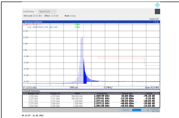
1-N7-PC3-15-20-H-6-DFT-s-OFDM QPSK-Edge_1RB_Right-1@105-Ant1-PASS
