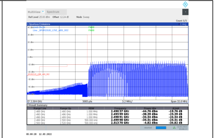
1-N7-PC3-15-20-L-35-CP-OFDM 256QAM-Outer_Full-106@0-Ant1-PASS
