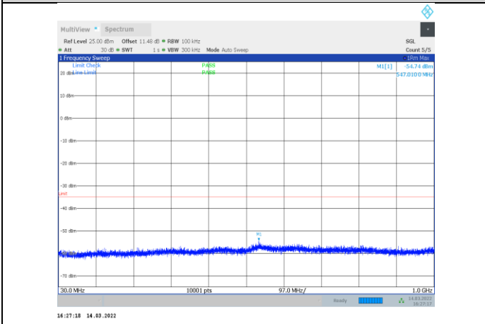
1-N7-PC3-15-5-L-2-CP-QPSK-Edge_1RB_Right-1@24 -30-1000-Ant1--54.74--35-PASS
