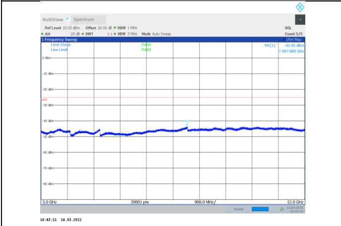
1-N7-PC3-15-15-L-3-CP-QPSK-Outter_Full-79@0-3000 -12000-Ant1--43.45--25-PASS
