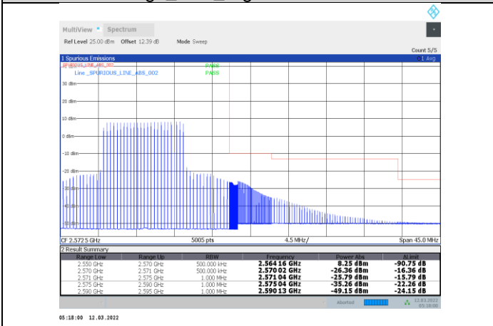
1-N7-PC3-15-20-H-24-CP-OFDM QPSK-Inner_Full-53@26-Ant1-PASS
