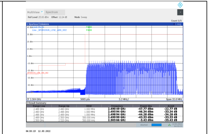
1-N7-PC3-15-20-L-19-DFT-s-OFDM 256QAM-Outer_Full-100@0-Ant1-PASS
