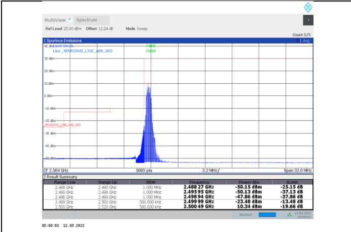
1-N7-PC3-15-20-L-33-CP-OFDM 256QAM-Edge_1RB_Left-1@0-Ant1-PASS
