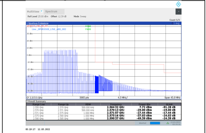
1-N7-PC3-15-20-H-28-CP-OFDM 16QAM-Inner_Full-53@26-Ant1-PASS
