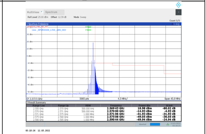
1-N7-PC3-15-20-H-26-CP-OFDM 16QAM-Edge_1RB_Right-1@105-Ant1-PASS
