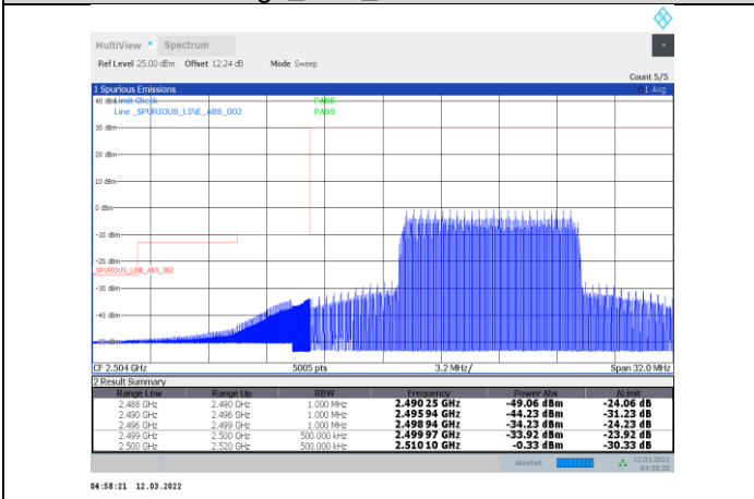
1-N7-PC3-15-20-L-28-CP-OFDM 16QAM-Inner_Full-53@26-Ant1-PASS
