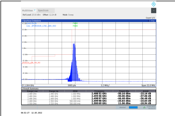
1-N7-PC3-15-20-L-9-DFT-s-OFDM 16QAM-Edge_1RB_Left-1@0-Ant1-PASS
