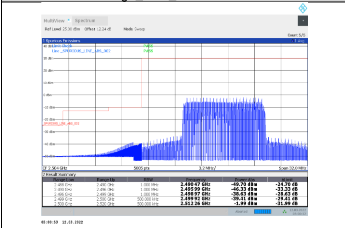
1-N7-PC3-15-20-L-36-CP-OFDM 256QAM-Inner_Full-53@26-Ant1-PASS
