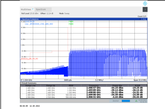
1-N7-PC3-15-20-L-23-CP-OFDM QPSK-Outer_Full-106@0-Ant1-PASS
