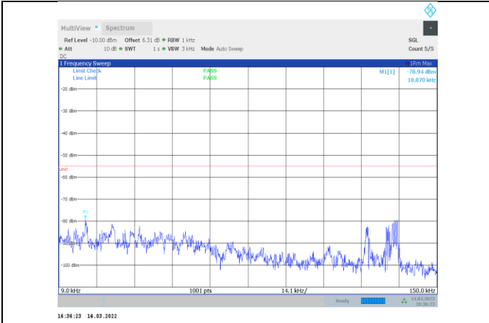
1-N7-PC3-15-5-H-2-CP-QPSK-Edge_1RB_Right-1@24 -0.009-0.15-Ant1--78.94--55-PASS
