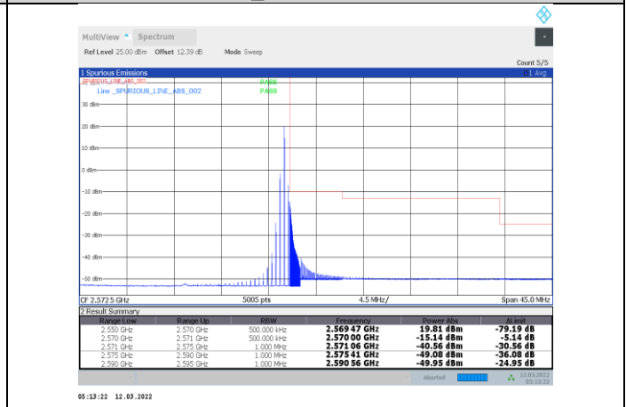
1-N7-PC3-15-20-H-10-DFT-s-OFDM 16QAM-Edge_1RB_Right-1@105-Ant1-PASS
