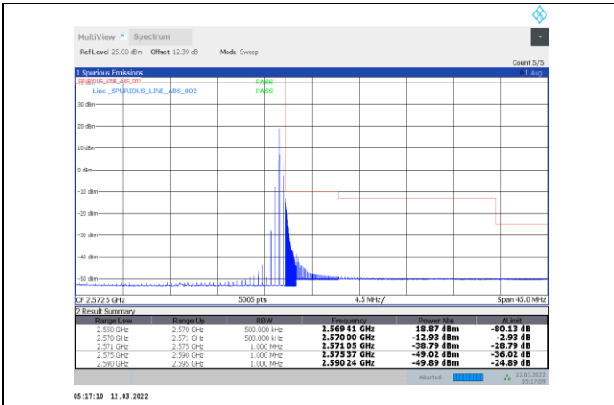
1-N7-PC3-15-20-H-22-CP-OFDM QPSK-Edge_1RB_Right-1@105-Ant1-PASS
