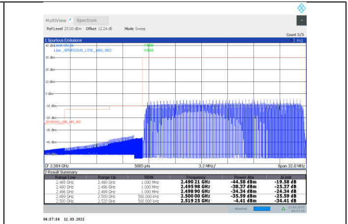
1-N7-PC3-15-20-L-27-CP-OFDM 16QAM-Outer_Full-106@0-Ant1-PASS
