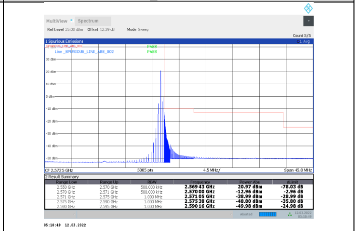
1-N7-PC3-15-20-H-2-DFT-s-OFDM PI/2 BPSK-Edge_1RB_Right-1@105-Ant1-PASS
