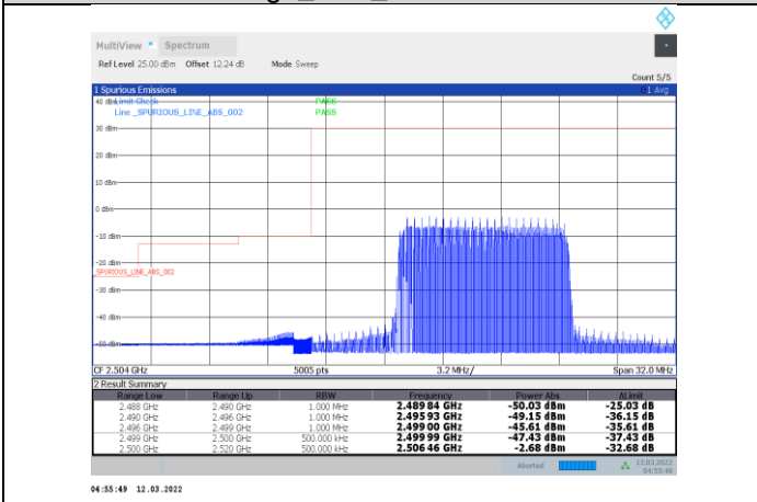
1-N7-PC3-15-20-L-20-DFT-s-OFDM 256QAM-Inner_Full-50@25-Ant1-PASS
