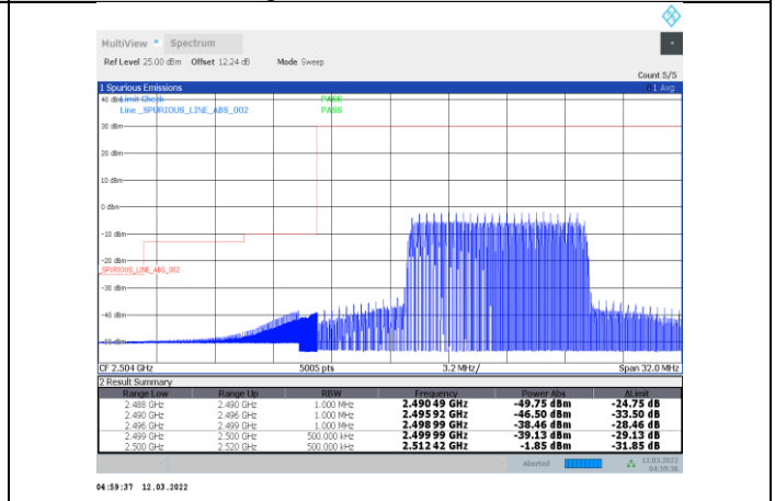
1-N7-PC3-15-20-L-32-CP-OFDM 64QAM-Inner_Full-53@26-Ant1-PASS
