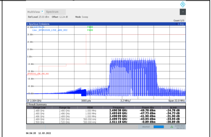
1-N7-PC3-15-20-L-16-DFT-s-OFDM 64QAM-Inner_Full-50@25-Ant1-PASS
