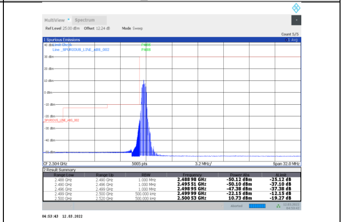
1-N7-PC3-15-20-L-13-DFT-s-OFDM 64QAM-Edge_1RB_Left-1@0-Ant1-PASS
