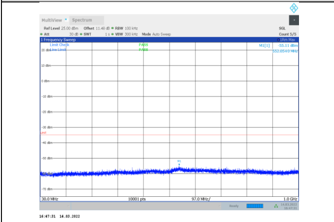
1-N7-PC3-15-15-M-3-CP-QPSK-Outter_Full-79@0-30-1 000-Ant1--55.11--35-PASS
