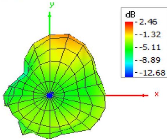
Figure A-3 Pattern at 2450 MHz
