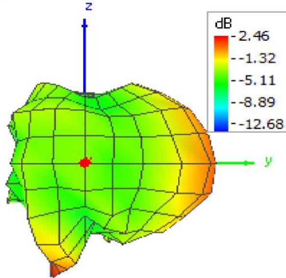
Figure A-4 Pattern at 2450 MHz
