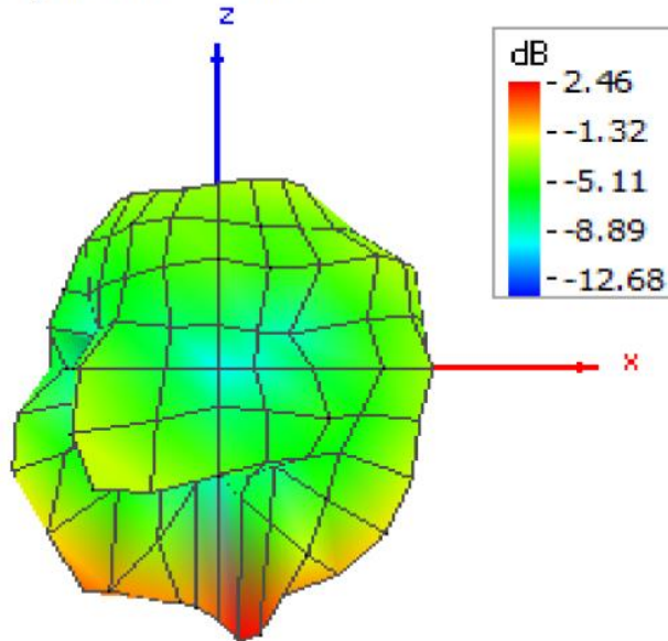
Figure A-5 Pattern at 2450 MHz
