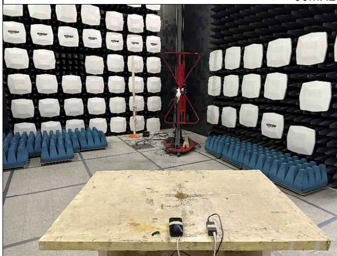
30MHz – 1GHz
